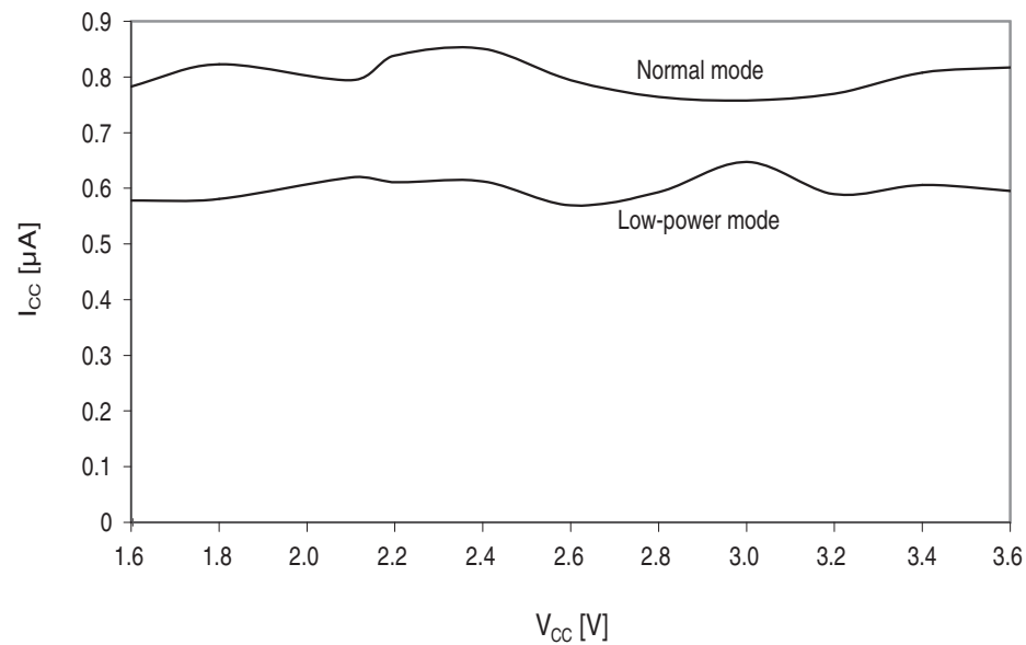
Figure 33-18. Power-save mode supply current vs. V_{CC} .
