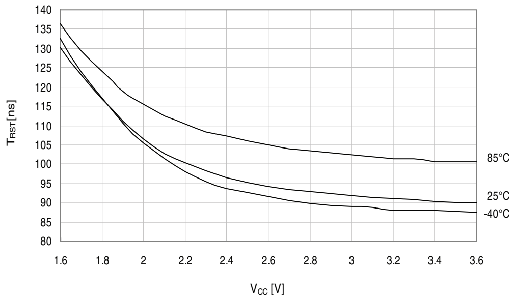
Figure 33-57. Minimum Reset pin pulse width vs. V_{CC} .
