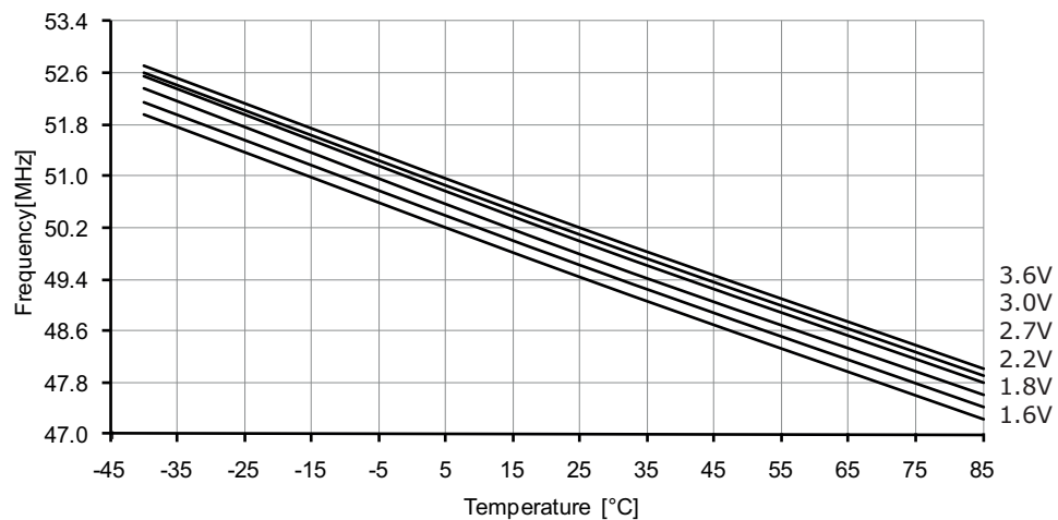
Figure 33-235. 48MHz internal oscillator frequency vs. temperature. DFLL disabled.
