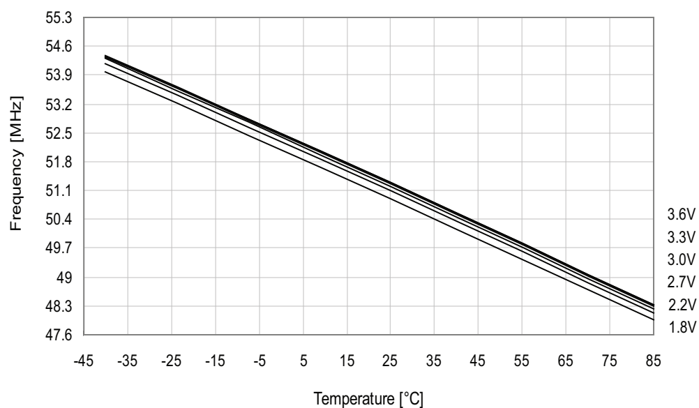
Figure 33-74. 48MHz internal oscillator frequency vs. temperature.
