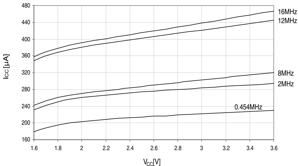
Figure 33-260. Standby supply current vs. V_{CC} .
