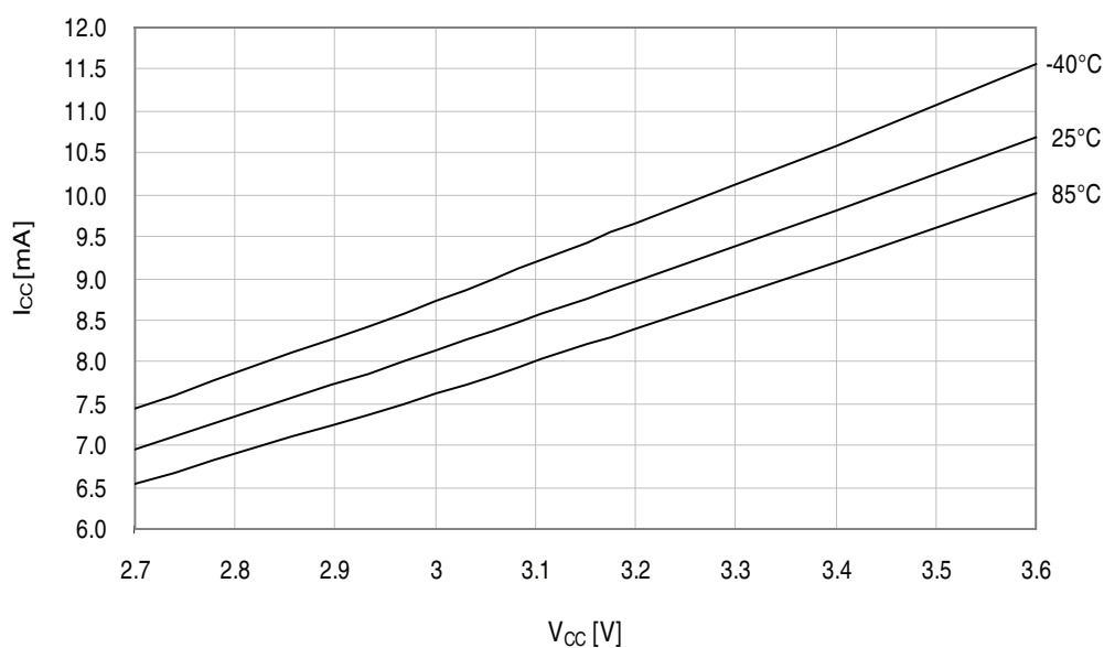
Figure 33-86. Active mode supply current vs. V_{CC} .
