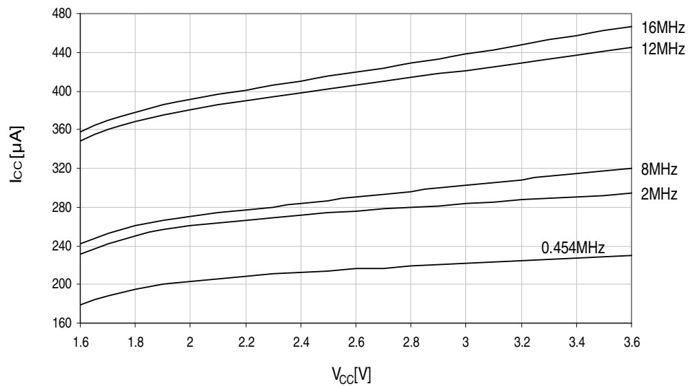
Figure 33-99. Standby supply current vs. V_{CC} .
