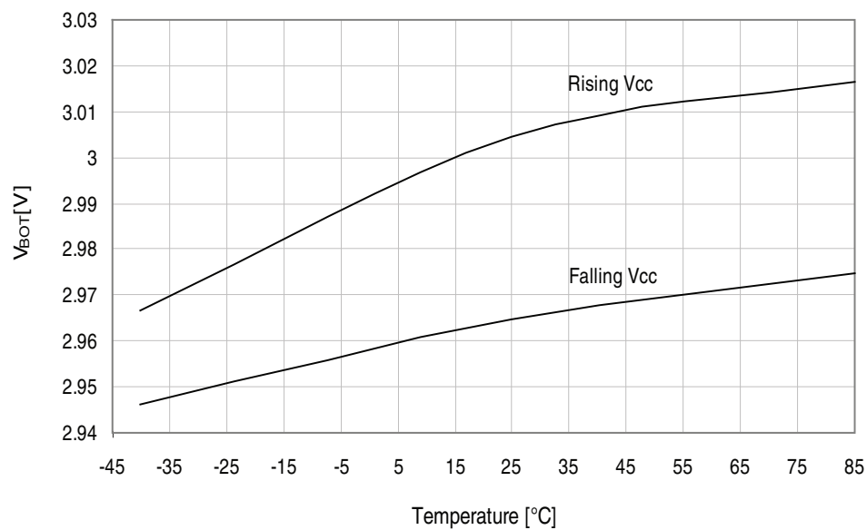
Figure 33-298. BOD thresholds vs. temperature.
