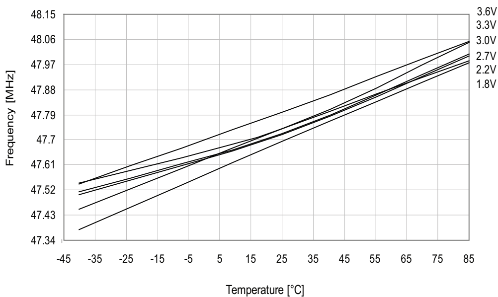
Figure 33-75. 48MHz internal oscillator frequency vs. temperature. DPLL enabled, from the 32.768kHz internal oscillator.
