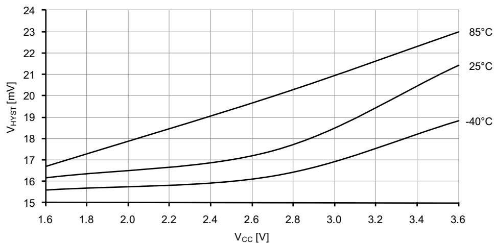
Figure 33-208. Analog comparator hysteresis vs. V_{CC} .
