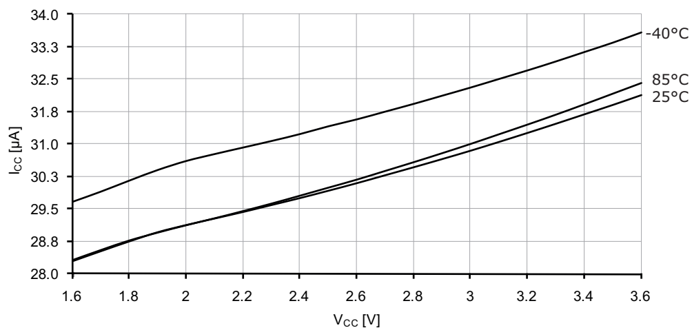
Figure 33-168. Idle mode supply current vs. V_{CC} .
