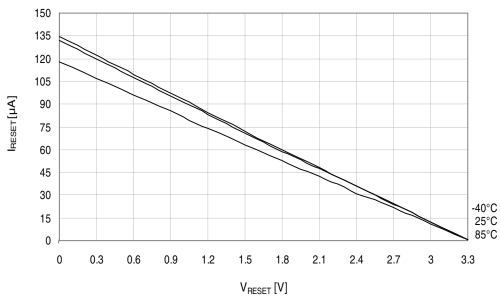
Figure 33-302. Reset pin pull-up resistor current vs. reset pin voltage.
