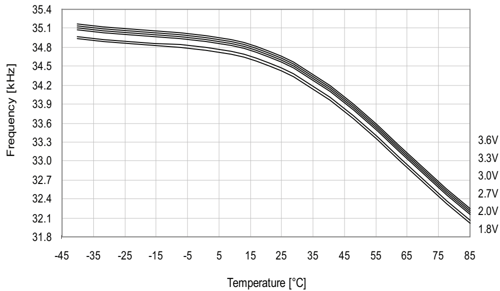
Figure 33-65.Ultra Low-Power internal oscillator frequency vs. temperature.
