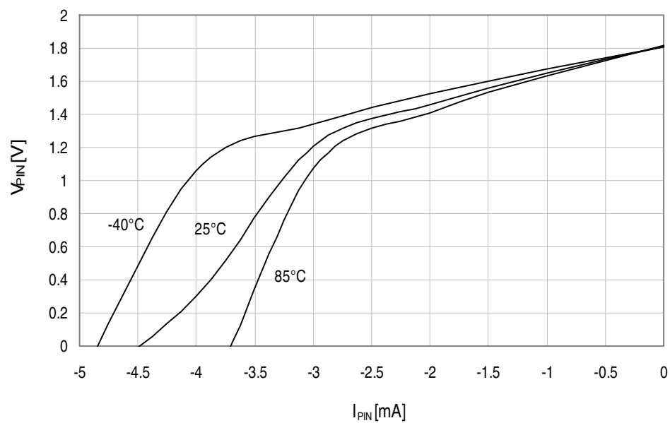
Figure 33-24. I/O pin output voltage vs. source current.
