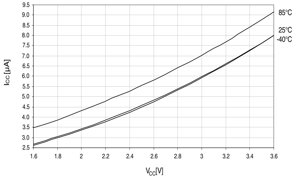
Figure 33-99. Standby supply current vs. V_{CC} .
