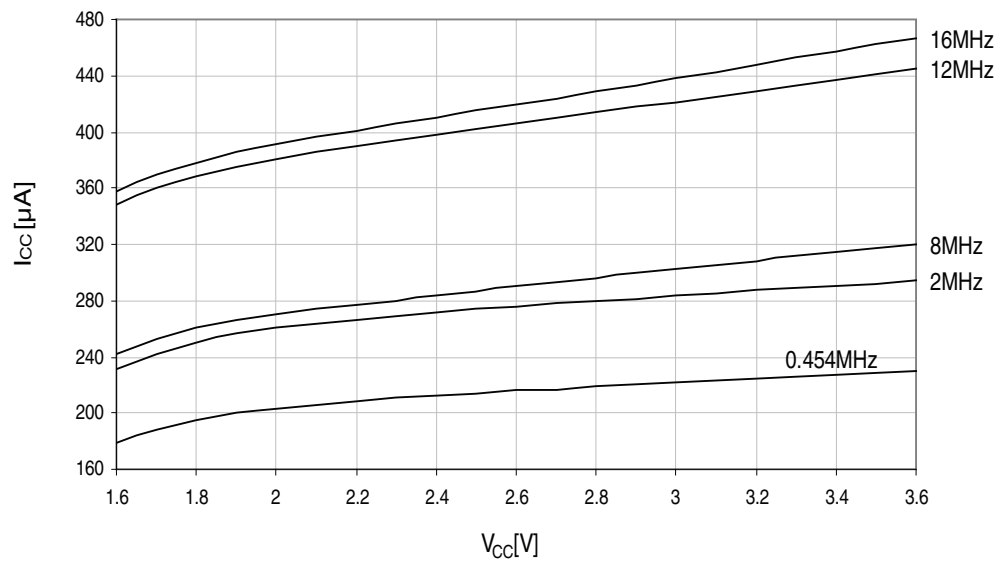
Figure 33-20. Standby supply current vs. V_{CC} .
