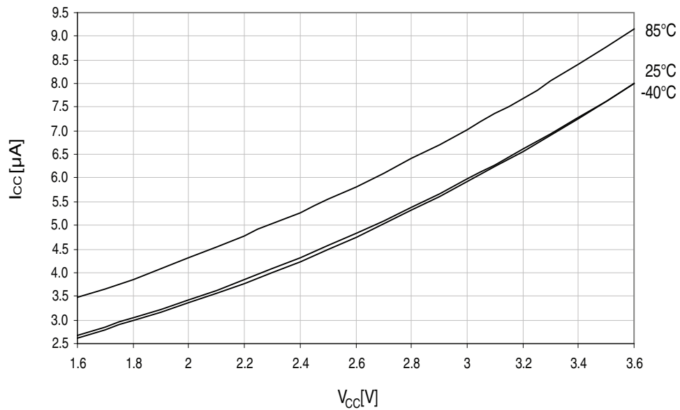
Figure 33-20. Standby supply current vs. V_{CC} .
