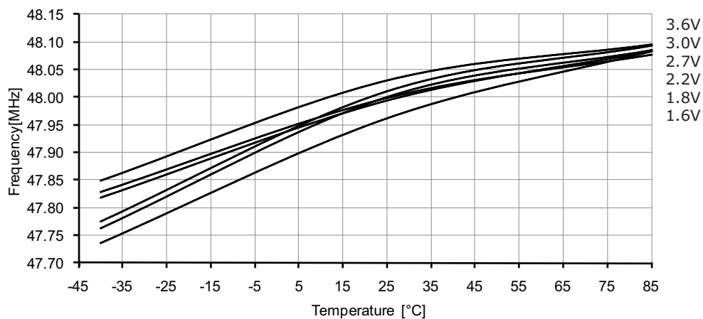
Figure 33-236. 48MHz internal oscillator frequency vs. temperature. DFLL enabled, from the 32.768kHz internal oscillator.
