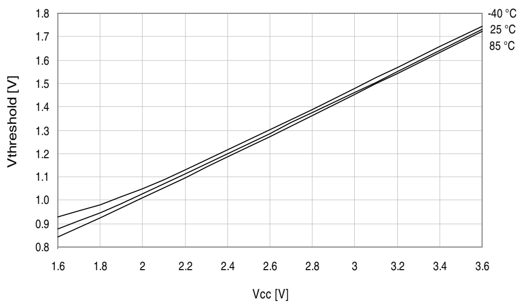
Figure 33-191. I/O pin input threshold voltage vs. V_{CC} .
