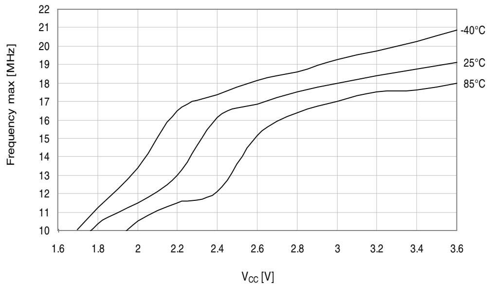
Figure 33-79. Maximum PDI frequency vs. V_{CC} .
