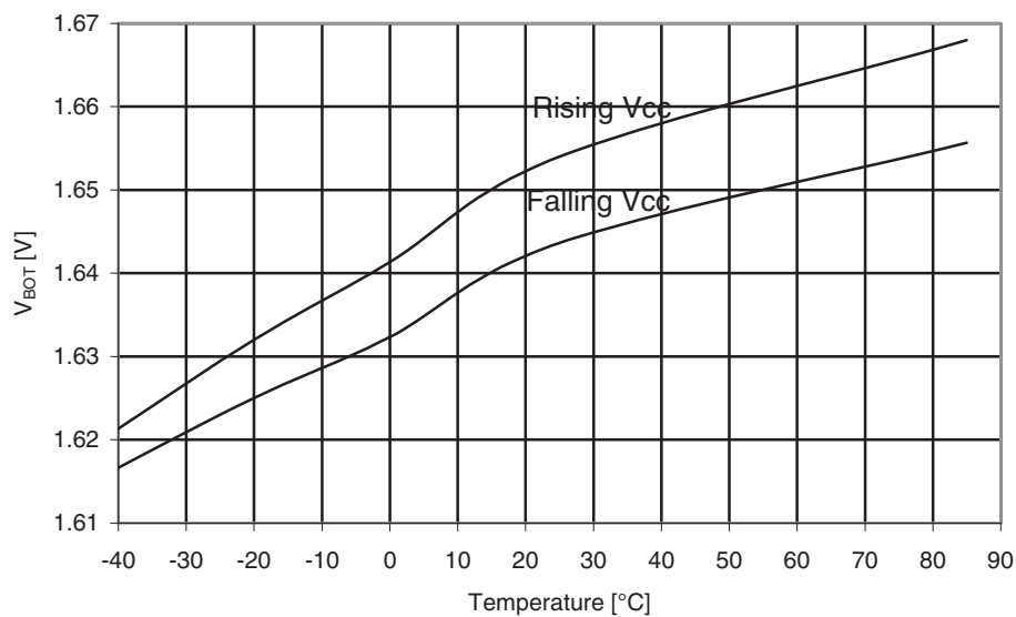
Figure 31-32. BOD Thresholds vs. Temperature BOD\ Level = 1.6V
