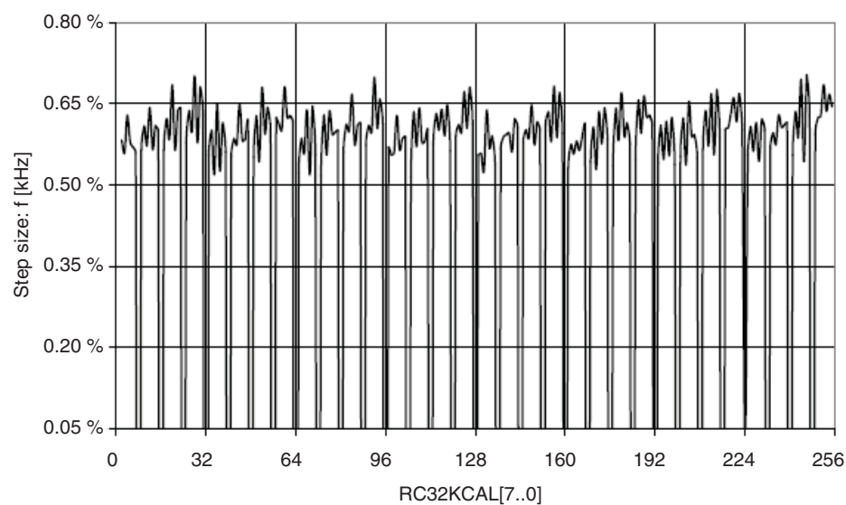
Figure 31-34. Internal 32.768 kHz Oscillator Calibration Step Size
