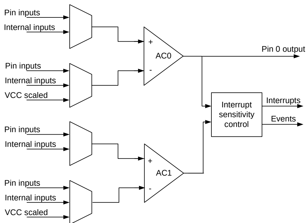
Figure 24-1. Analog comparator overview
