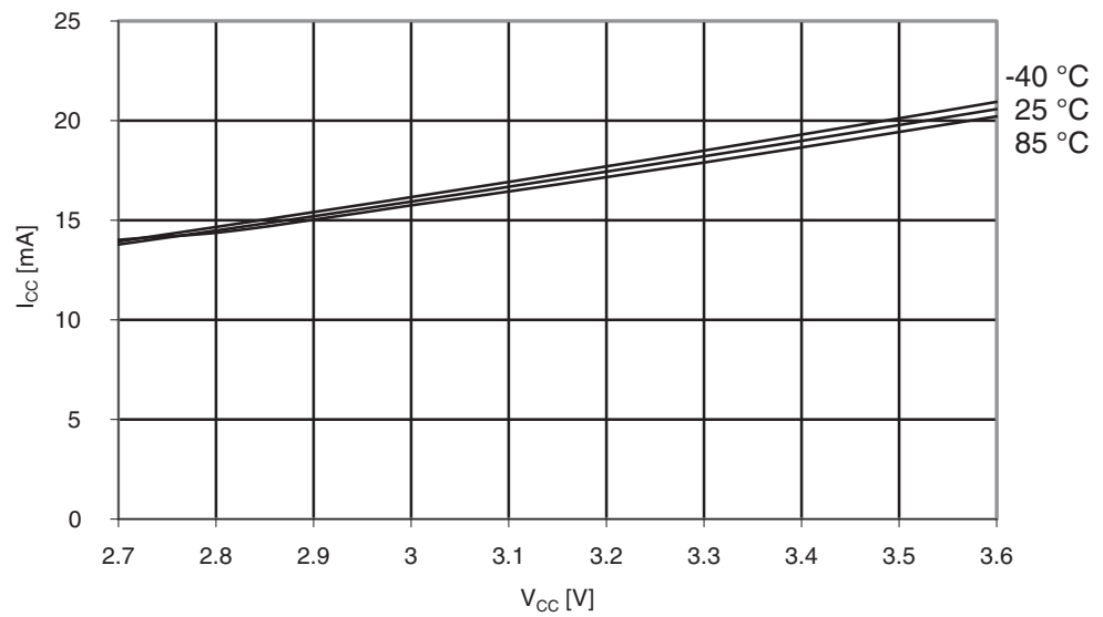
Figure 31-7. Active Supply Current vs. V_{CC}
