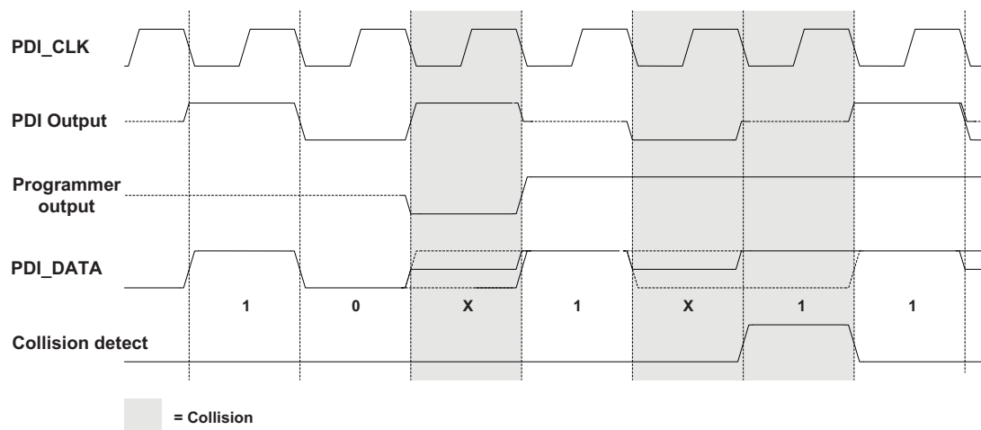
Figure 27-9. Drive contention and collision detection on the PDI_DATA line.
