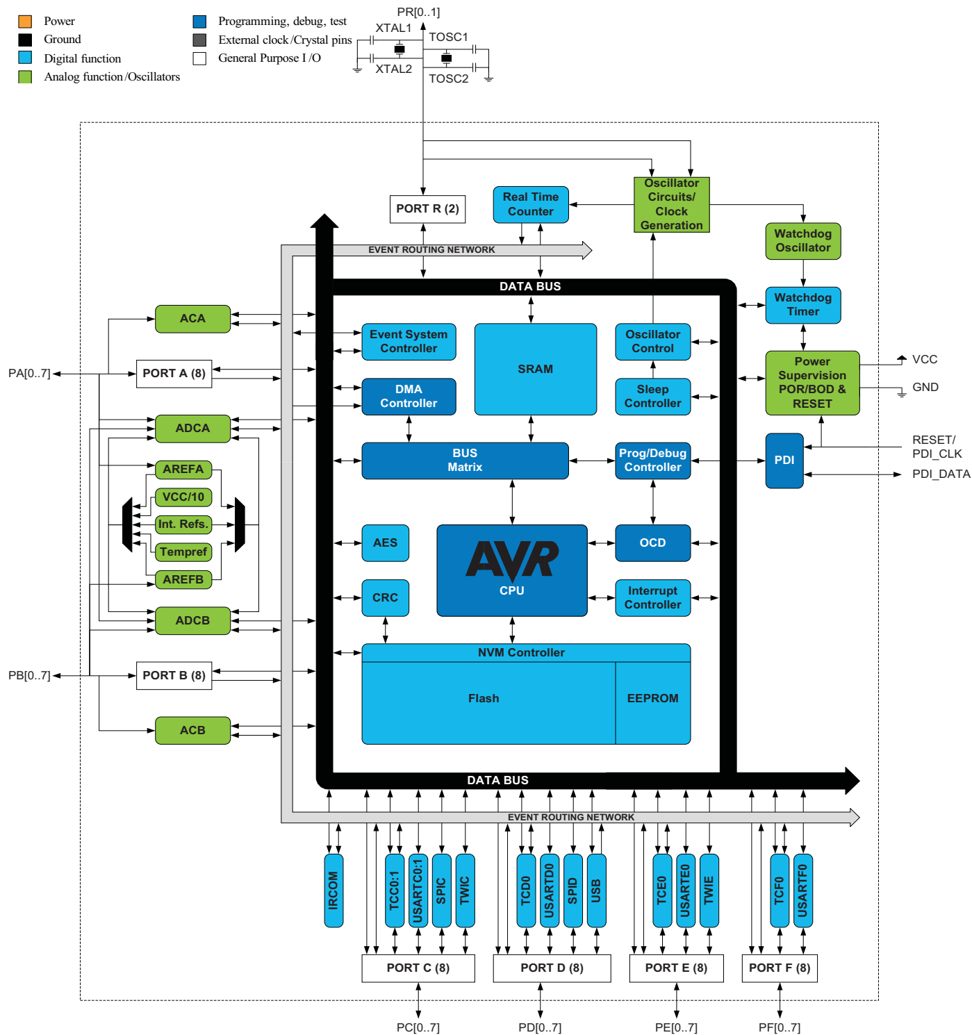
Figure 2-1. Atmel AVR XMEGA C block diagram.
