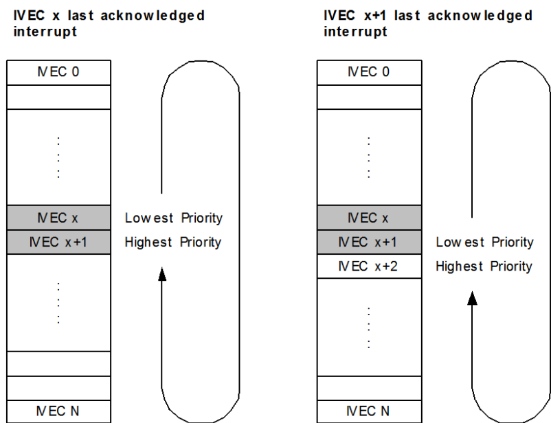
Figure 11-4. Round-robin scheduling.
