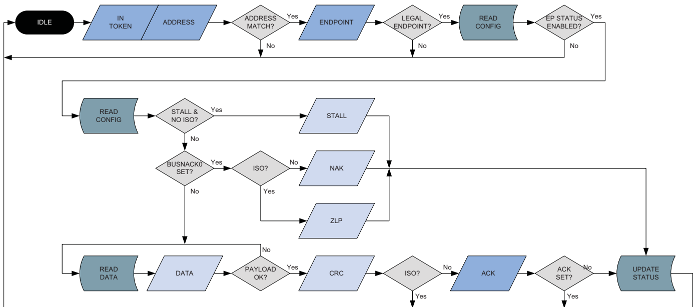
Figure 18-5. IN transaction.
