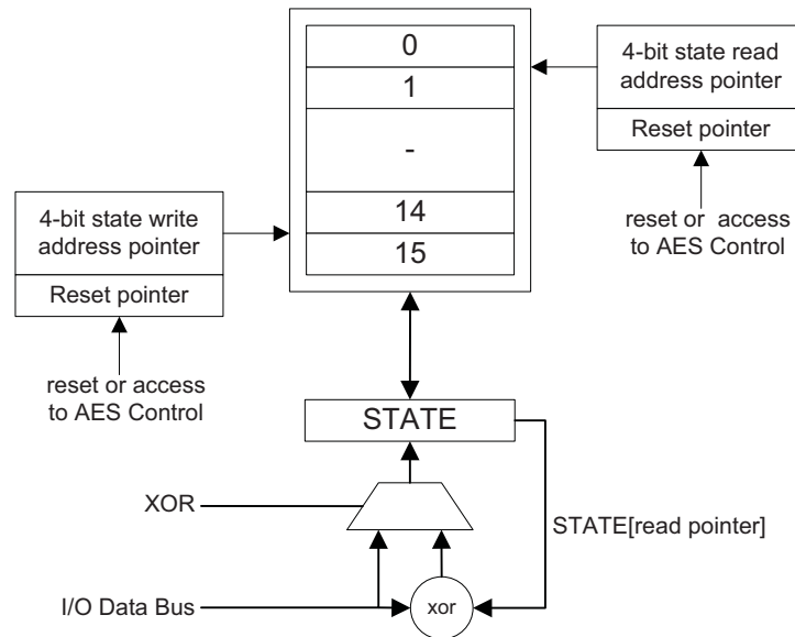
Figure 23-1. The state memory with pointers and register.
