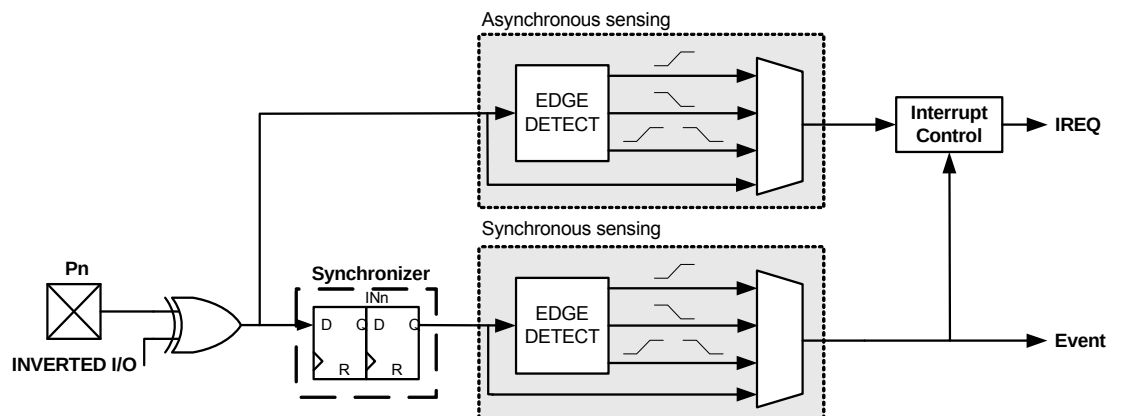
Figure 12-9. Input sensing.
