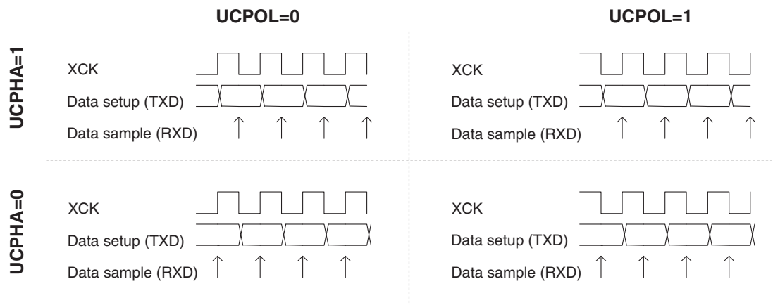
Figure 21-4. UCPHA and INVEN data transfer timing diagrams.
