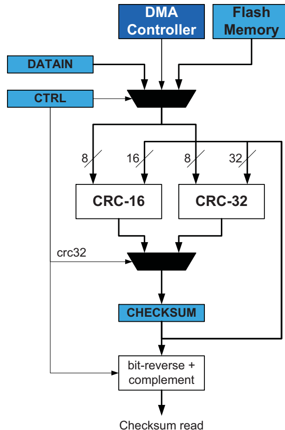
Figure 24-1. CRC generator block diagram.
