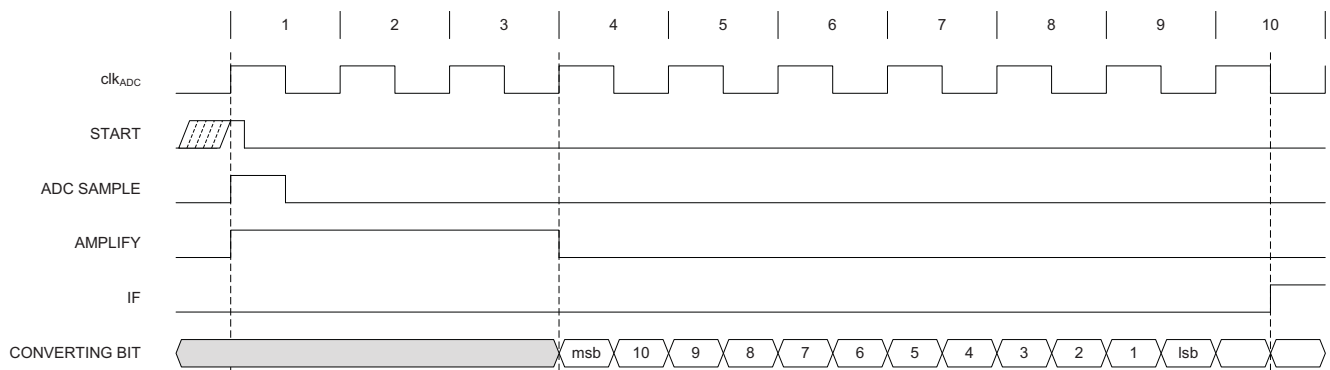
Figure 25-17. ADC timing for one single conversion with 64x gain.
