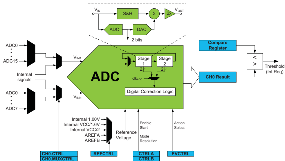
Figure 25-1. ADC overview.
