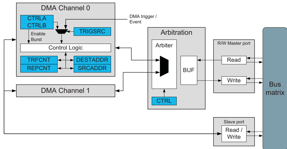
Figure 5-1. DMA Overview.
