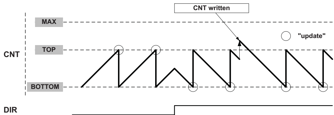
Figure 13-6. Normal operation.
