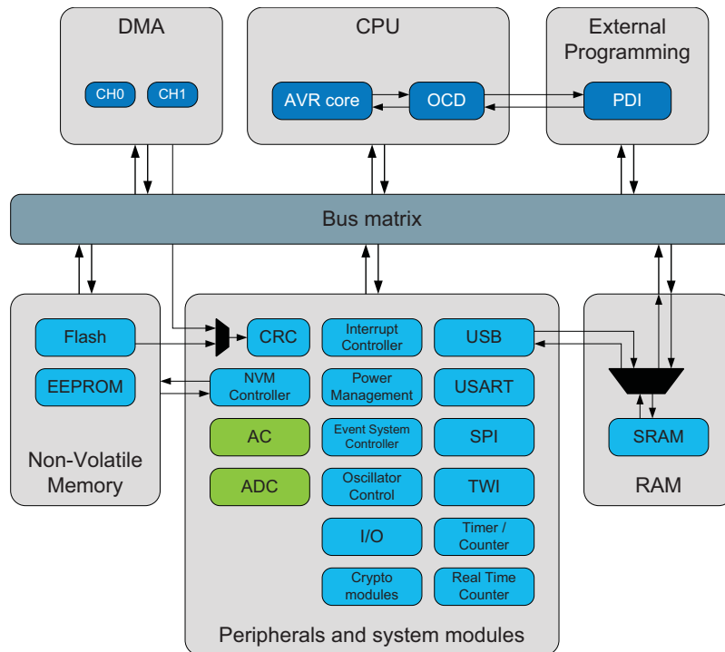
Figure 4-3. Bus access.
