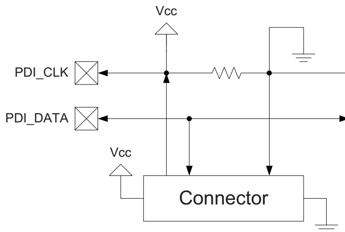
Figure 27-2. PDI connection.
