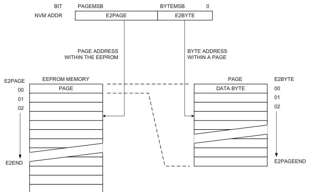
Figure 28-2. I/O mapped EEPROM addressing.
