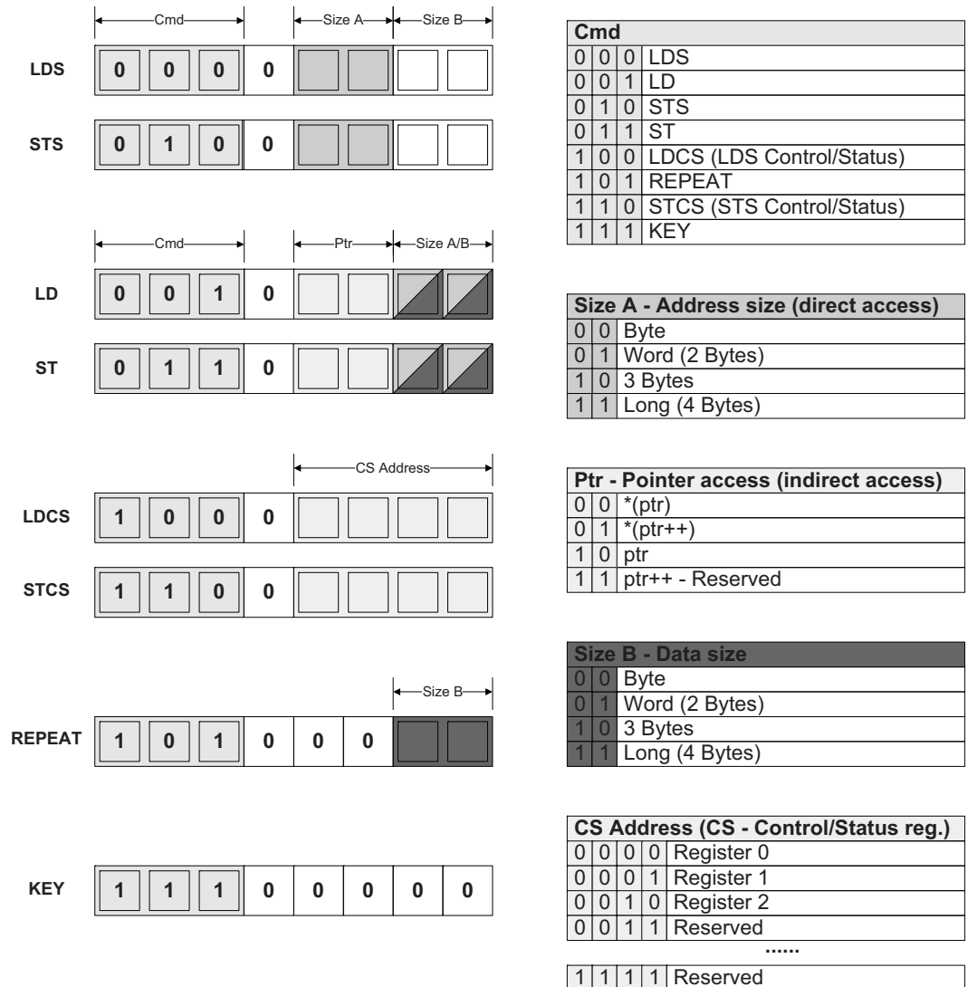
Figure 27-10. PDI instruction set summary.
