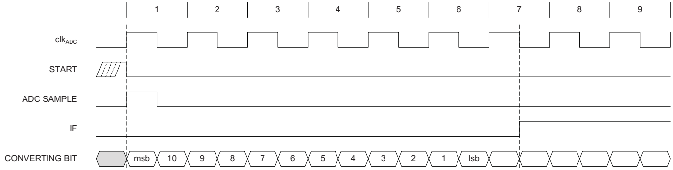
Figure 25-13. ADC timing for one single conversion without gain.
