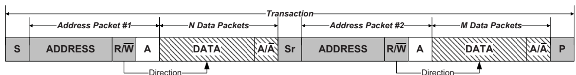
Figure 19-7. Combined Transaction.
