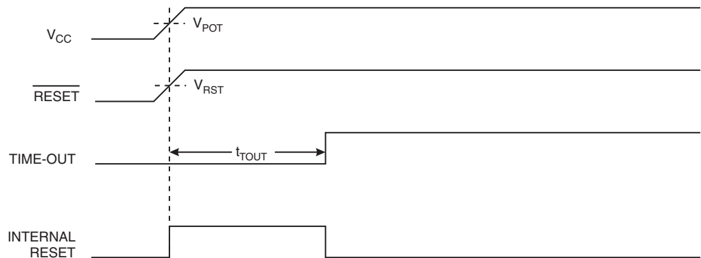
Figure 9-2. MCU startup, \overline{\text{RESET}} tied to V_{\text{CC}} .
