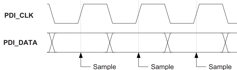
Figure 27-6. Changing and sampling of data.
