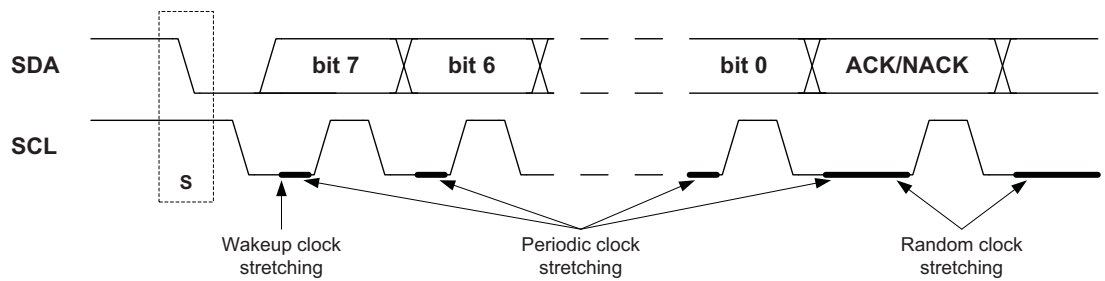
Figure 19-8. Clock stretching (1) .
