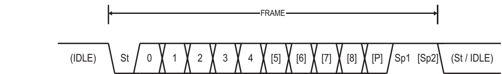
Figure 21-5. Frame formats.
