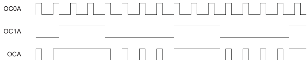
Figure 12-11. I/O timer/counter.
