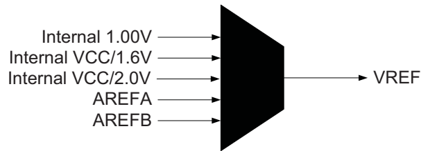
Figure 25-8. ADC voltage reference selection
