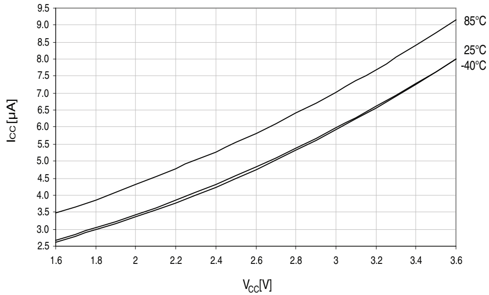
Figure 34-20. Standby supply current vs. V_{CC} .
