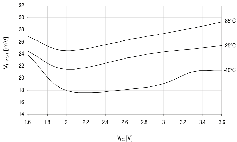
Figure 34-48. Analog comparator hysteresis vs. V_{CC} . High speed, large hysteresis.
