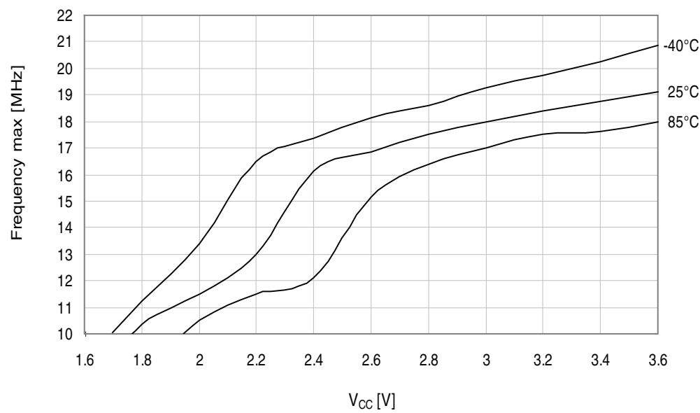
Figure 34-158. Maximum PDI frequency vs. V_{CC} .
