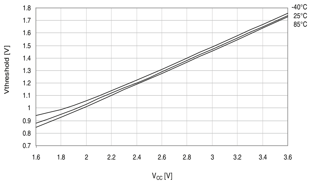
Figure 34-113. I/O pin input threshold voltage vs. V_{CC} .
