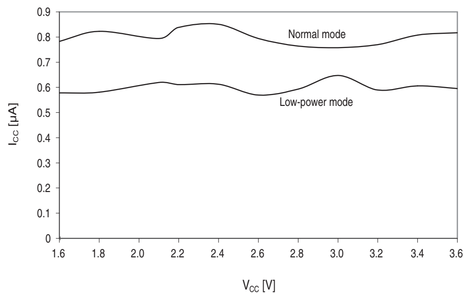
Figure 34-18. Power-save mode supply current vs. V_{CC} .
