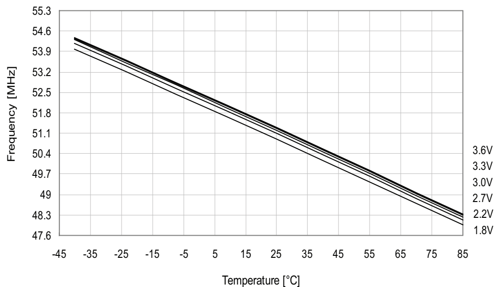
Figure 34-74. 48MHz internal oscillator frequency vs. temperature.
