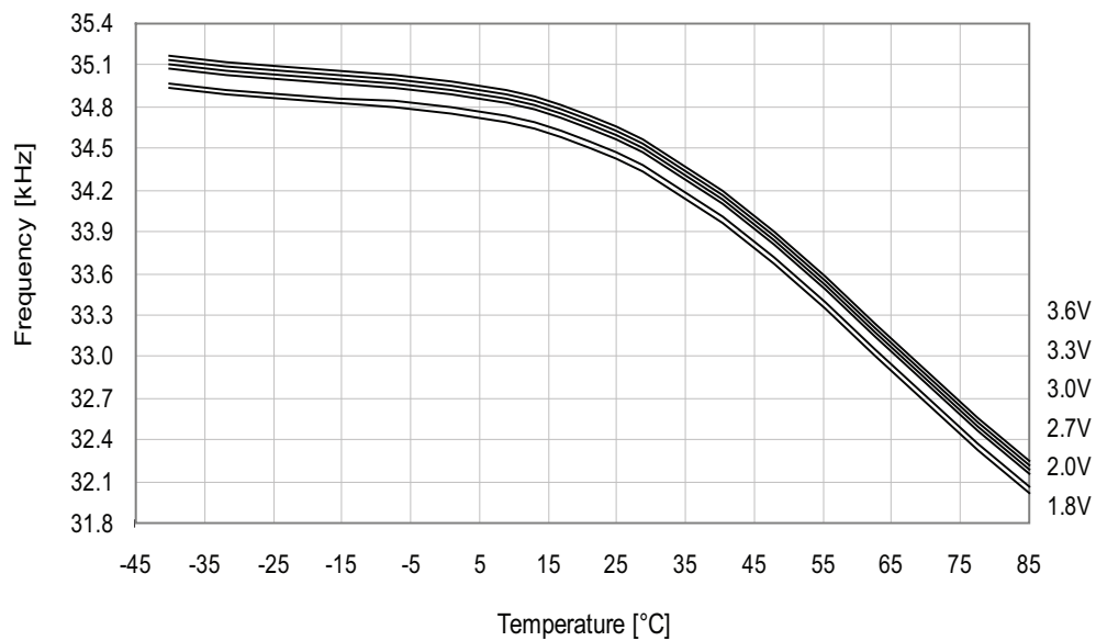
Figure 34-65.Ultra Low-Power internal oscillator frequency vs. temperature.
