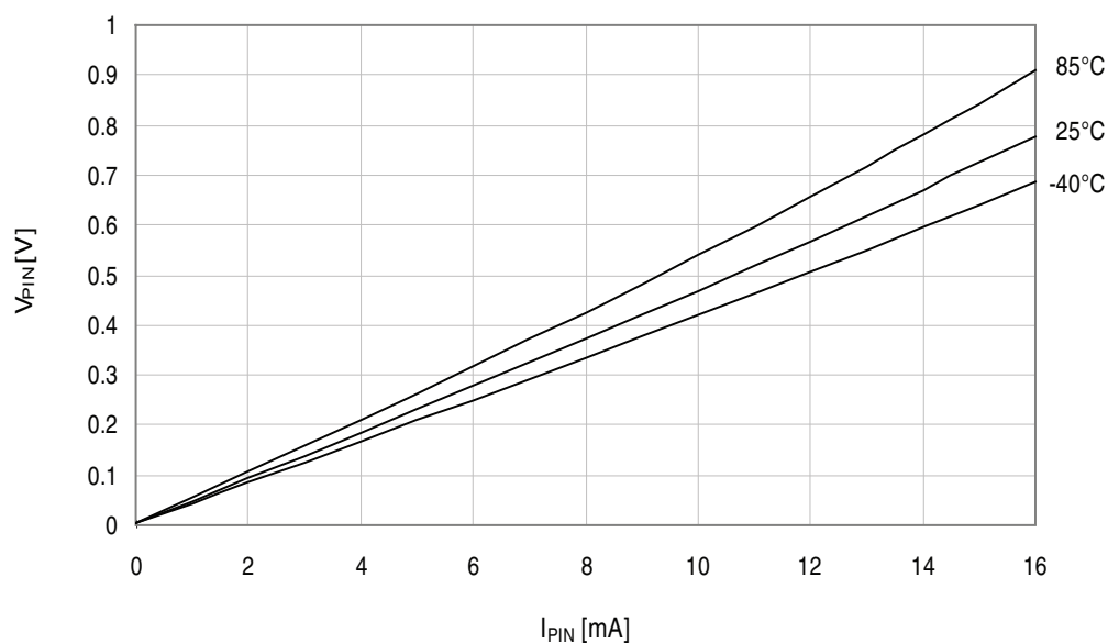
Figure 34-30. I/O pin output voltage vs. sink current.
