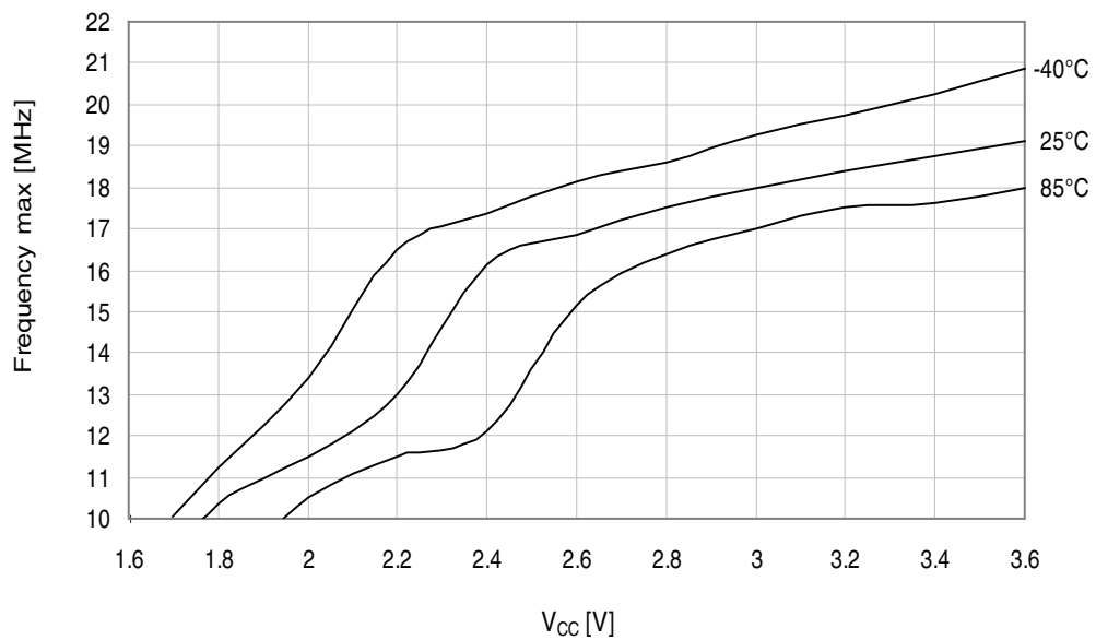
Figure 34-79. Maximum PDI frequency vs. V_{CC} .
