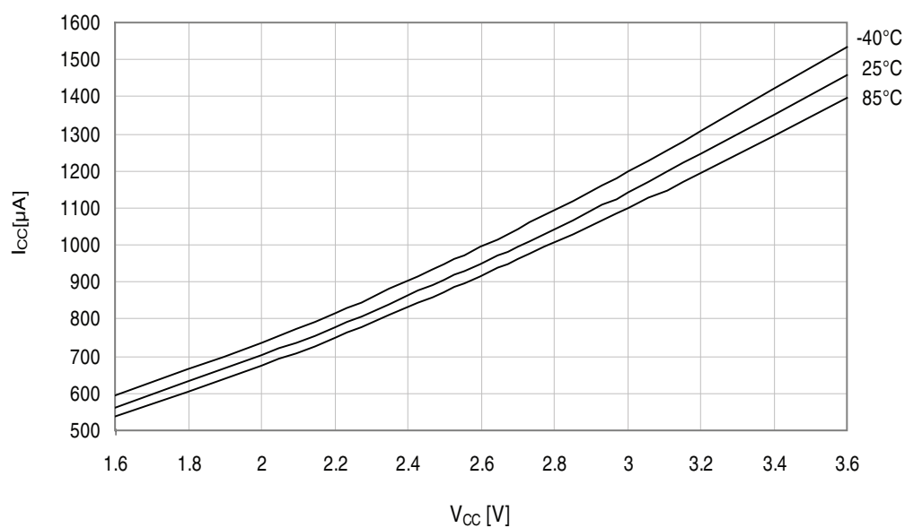
Figure 34-93. Idle mode current vs. V_{CC} .
