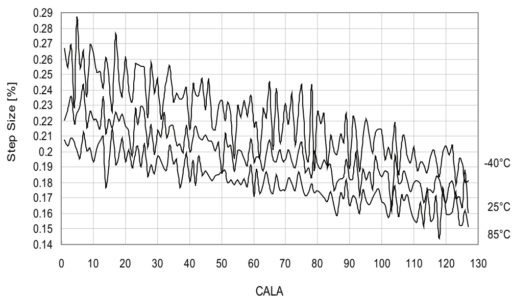
Figure 34-73. 32MHz internal oscillator CALA calibration step size.
