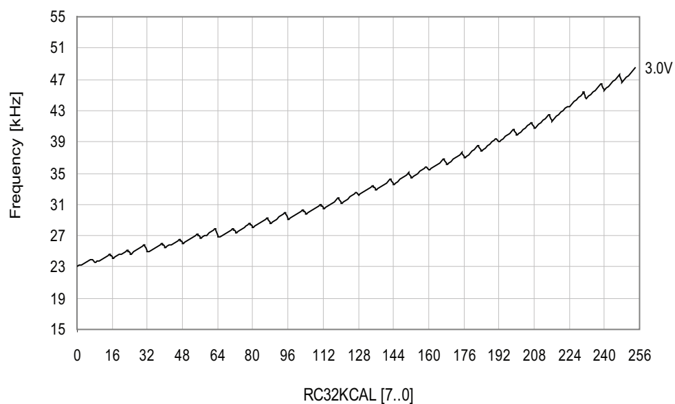
Figure 34-67. 32.768kHz internal oscillator frequency vs. calibration value.
