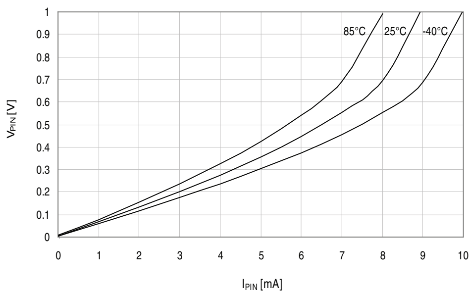
Figure 34-28. I/O pin output voltage vs. sink current.
