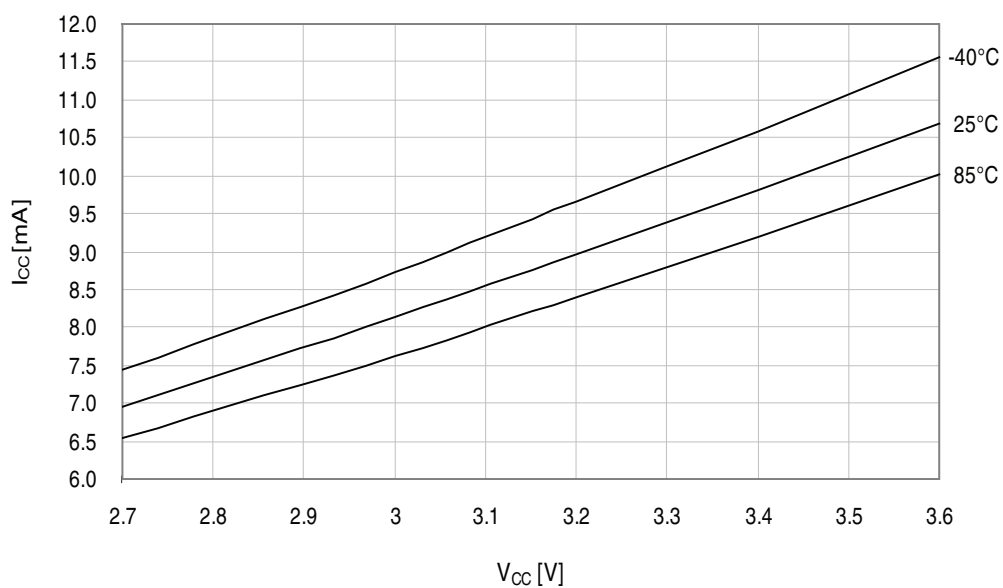
Figure 34-86. Active mode supply current vs. V_{CC} .
