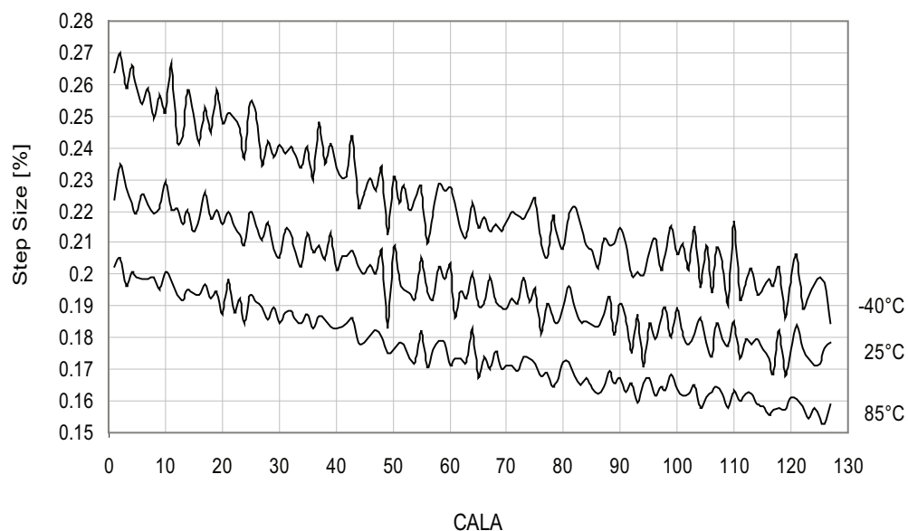
Figure 34-70. 2MHz internal oscillator CALA calibration step size.
