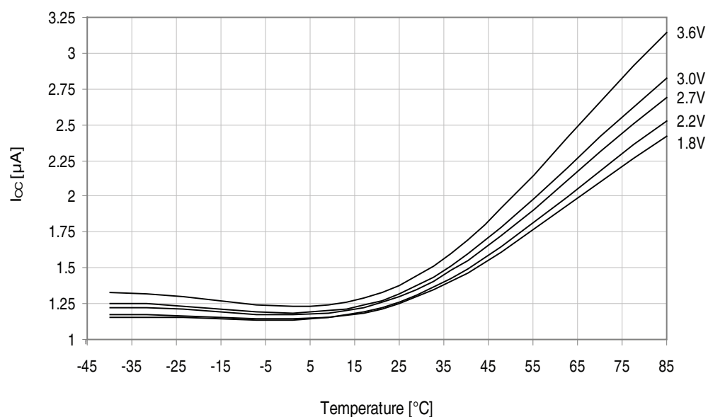
Figure 34-96. Power-down mode supply current vs. Temperature.
