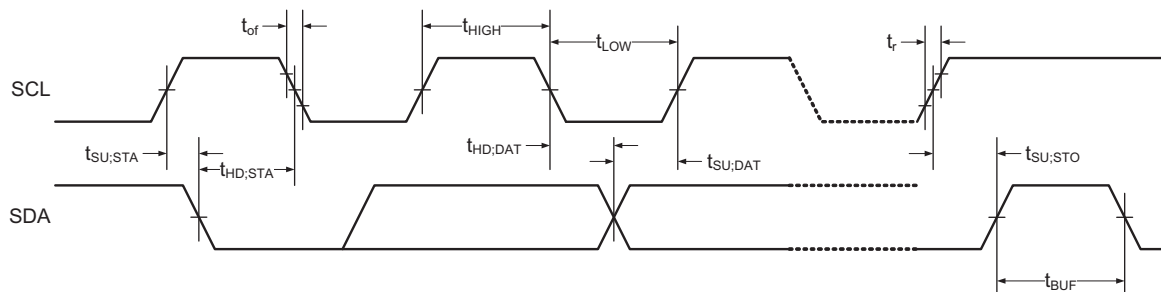
Figure 33-7. Two-wire interface bus timing.
