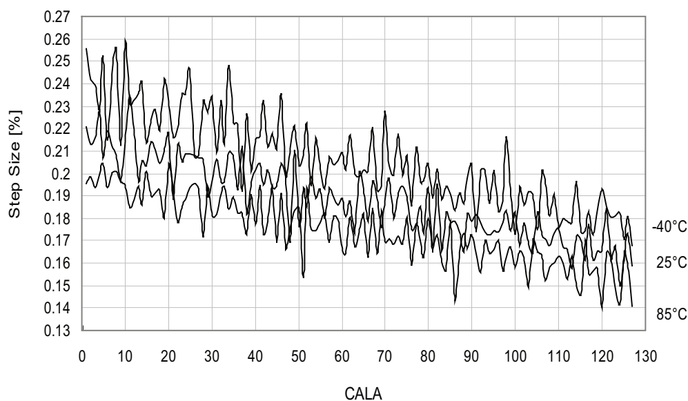
Figure 34-155. 48MHz internal oscillator CALA calibration step size. V_{CC} = 3.0V .
