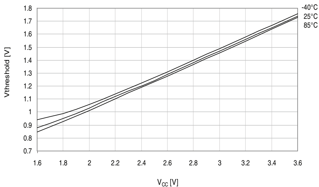
Figure 34-34. I/O pin input threshold voltage vs. V_{CC} .
