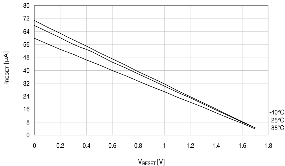
Figure 34-58. Reset pin pull-up resistor current vs. reset pin voltage.
