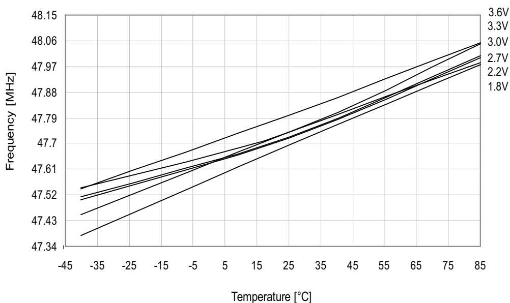
Figure 34-75. 48MHz internal oscillator frequency vs. temperature. DPLL enabled, from the 32.768kHz internal oscillator.
