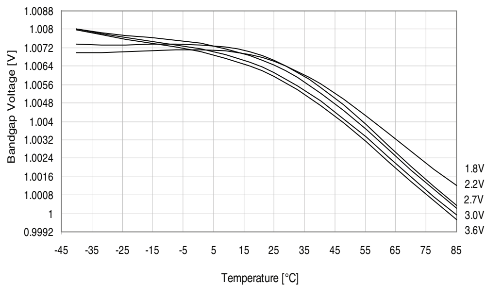
Figure 34-133. ADC Internal 1.0V reference vs. temperature.
