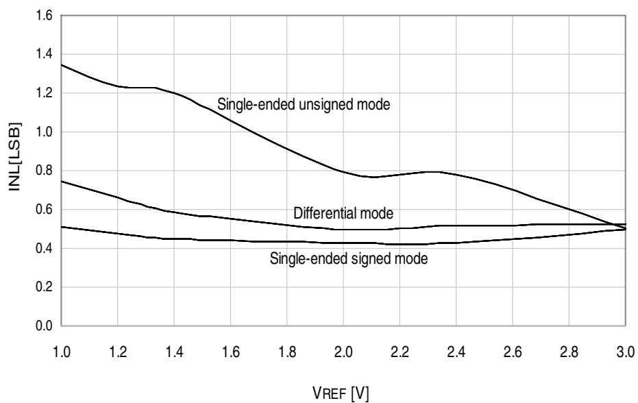
Figure 34-36. INL error vs. external V_{REF} .
