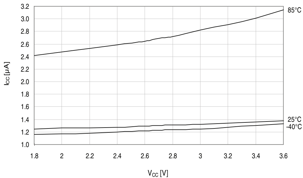
Figure 34-95. Power-down mode supply current vs. V_{CC} . Watchdog and sampled BOD enabled.
