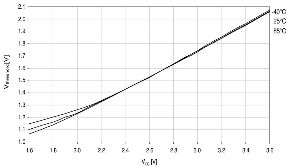
Figure 34-141. Reset pin input threshold voltage vs. V_{CC} .
