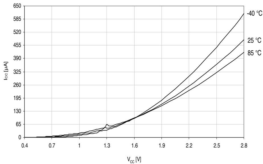
Figure 34-143. Power-on reset current consumption vs. V_{CC} . BOD level = 3.0V, enabled in sampled mode.
