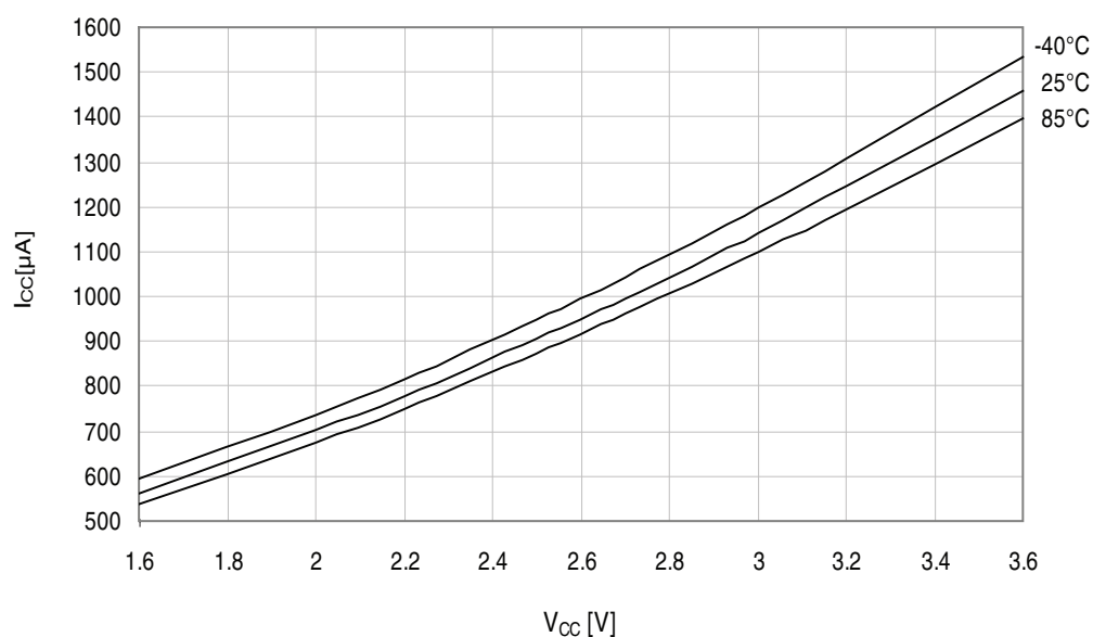
Figure 34-14. Idle mode current vs. V_{CC} .
