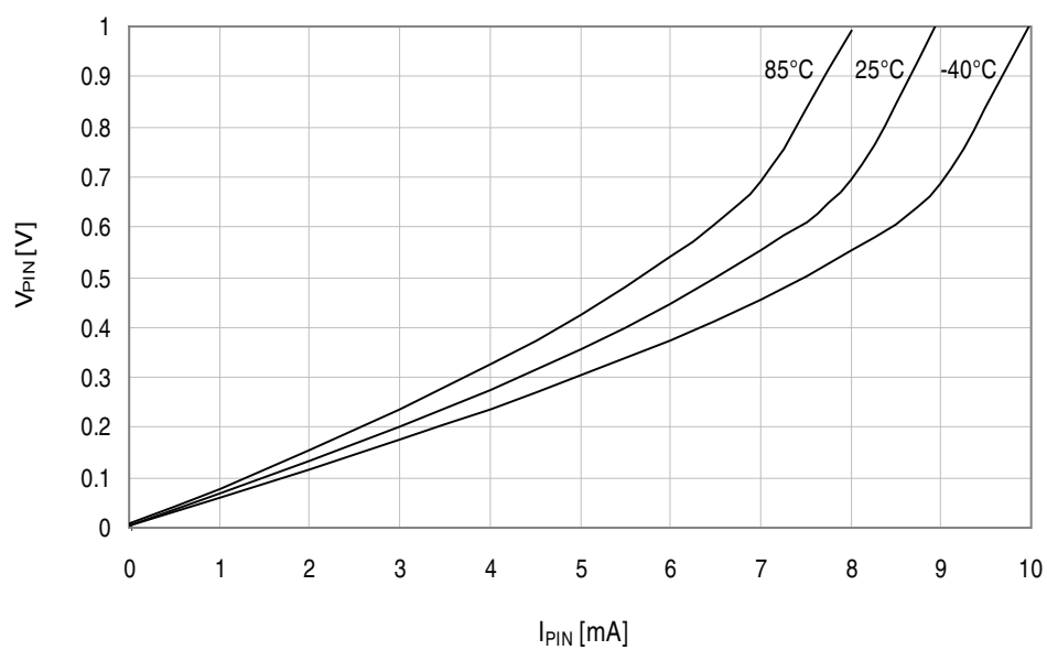
Figure 34-107. I/O pin output voltage vs. sink current.
