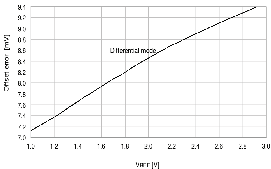
Figure 34-123. Offset error vs. V_{REF} .
