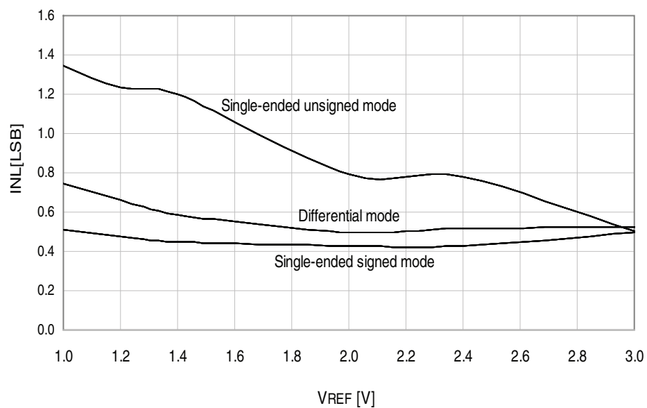
Figure 34-115. INL error vs. external V_{REF} .
