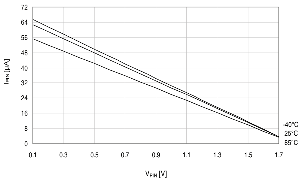
Figure 34-101. I/O pin pull-up resistor current vs. input voltage.
