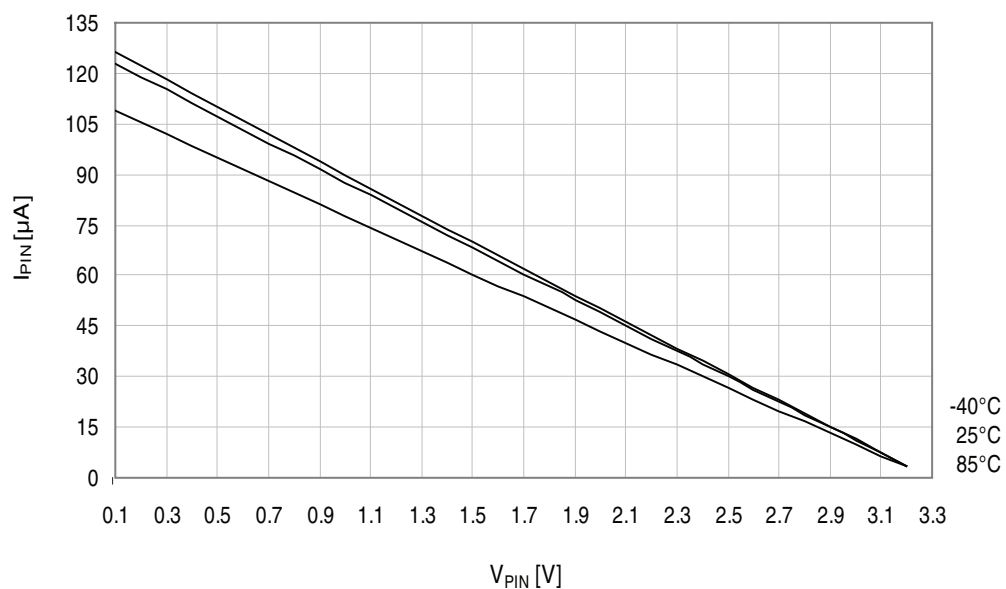
Figure 34-23. I/O pin pull-up resistor current vs. input voltage.
