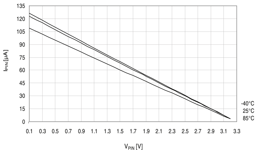
Figure 34-102. I/O pin pull-up resistor current vs. input voltage.
