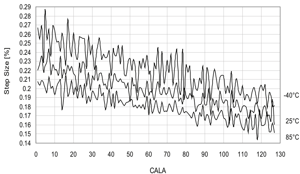
Figure 34-152. 32MHz internal oscillator CALA calibration step size.
