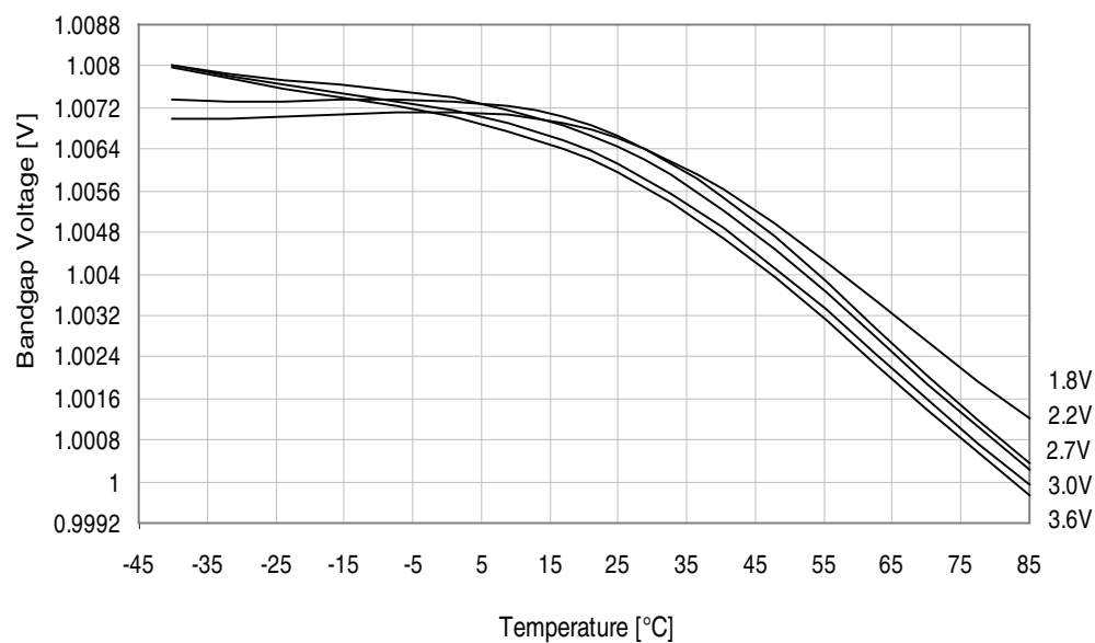
Figure 34-54. ADC Internal 1.0V reference vs. temperature.
