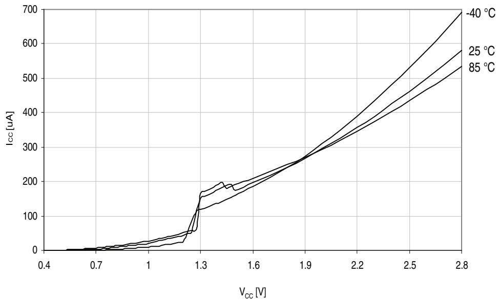
Figure 34-142. Power-on reset current consumption vs. V_{CC} . BOD level = 3.0V, enabled in continuous mode.
