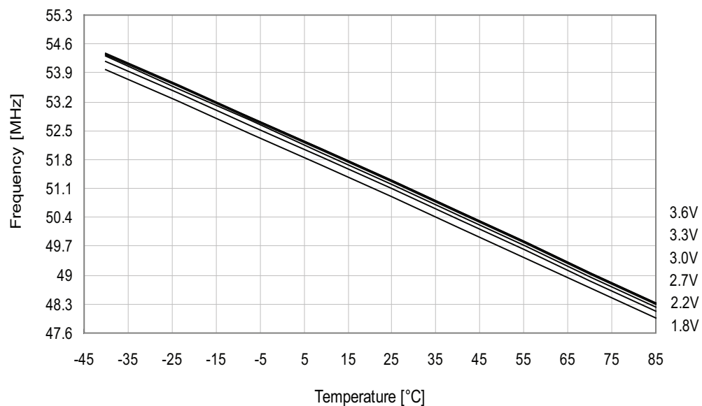
Figure 34-153. 48MHz internal oscillator frequency vs. temperature.
