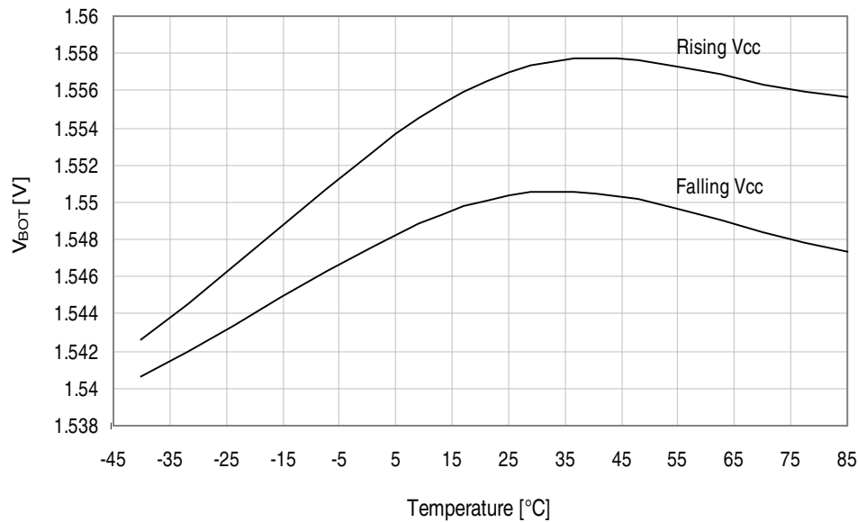
Figure 34-134. BOD thresholds vs. temperature. BOD level = 1.6V.
