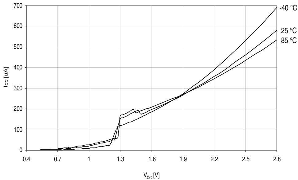
Figure 34-63. Power-on reset current consumption vs. V_{CC} . BOD level = 3.0V, enabled in continuous mode.
