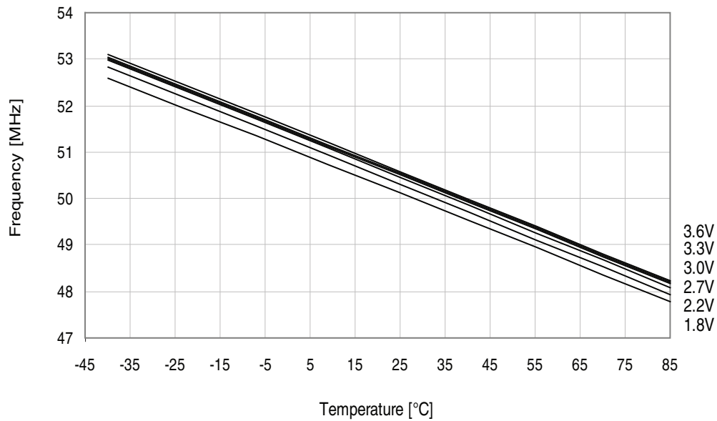
Figure 34-267. 48MHz internal oscillator frequency vs. temperature. DPLL enabled, from the 32.768kHz internal oscillator.
