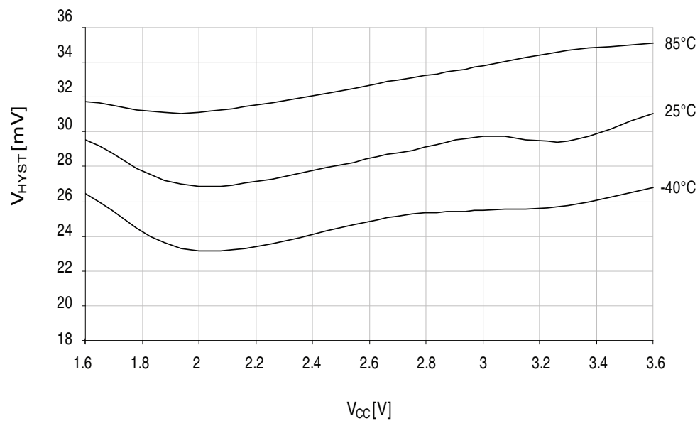
Figure 34-312. Analog comparator hysteresis vs. V_{CC} .
