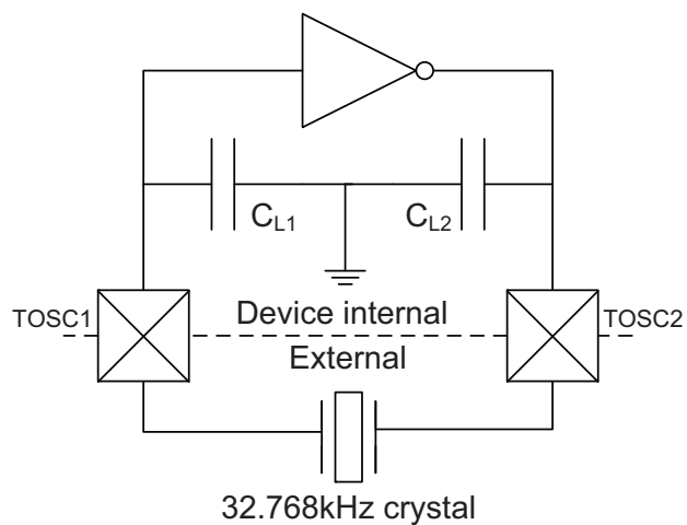
Figure 33-4. TOSC input capacitance.
