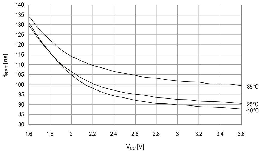
Figure 34-49. Minimum Reset pin pulse width vs. V_{CC} .
