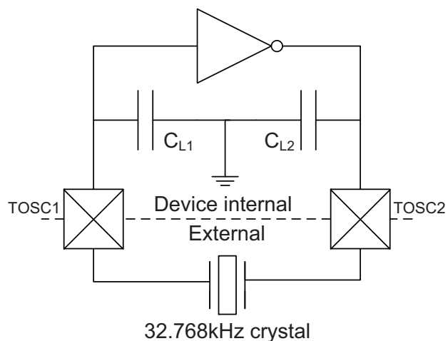
Figure 33-32. TOSC input capacitance.
