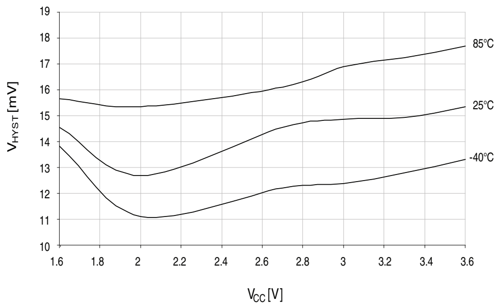
Figure 34-312. Analog comparator hysteresis vs. V_{CC} .
