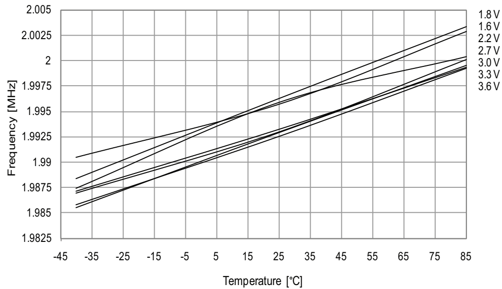
Figure 34-126. 2MHz internal oscillator frequency vs. temperature.
