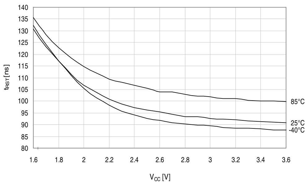
Figure 34-318. Minimum Reset pin pulse width vs. V_{CC} .
