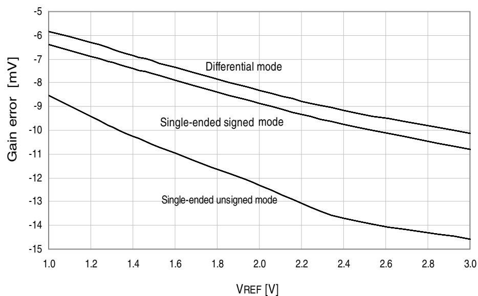
Figure 34-239.Gain error vs. V_{REF} . T = 25^{\circ}\text{C} , V_{CC} = 3.6\text{V} , ADC sample rate = 300ksps.
