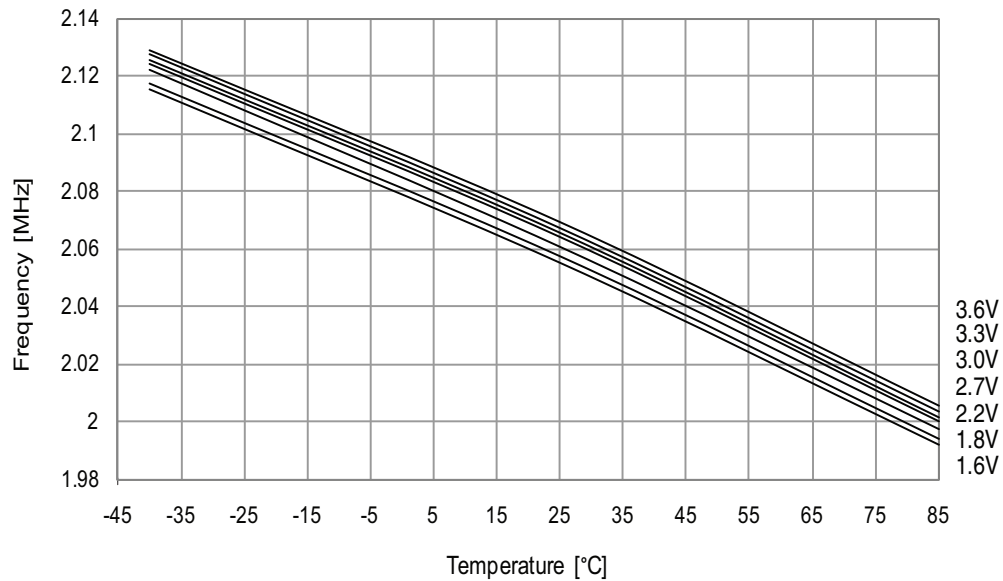
Figure 34-126. 2MHz internal oscillator frequency vs. temperature.
