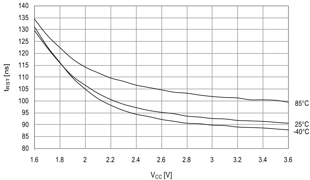
Figure 34-117. Minimum Reset pin pulse width vs. V_{CC} .
