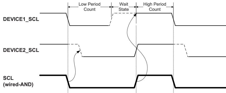
Figure 19-10. Clock synchronization.
