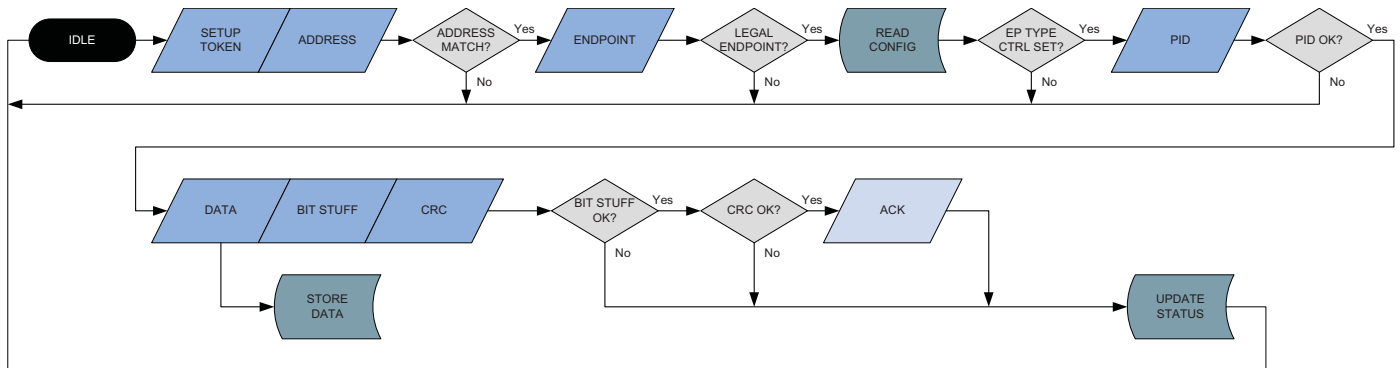
Figure 18-3. SETUP transaction.
