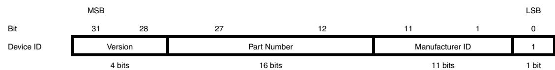
Figure 27-5. Device identification register.
