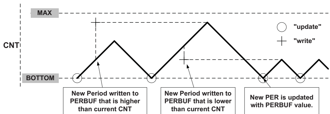
Figure 13-9. Changing the period using buffering.
