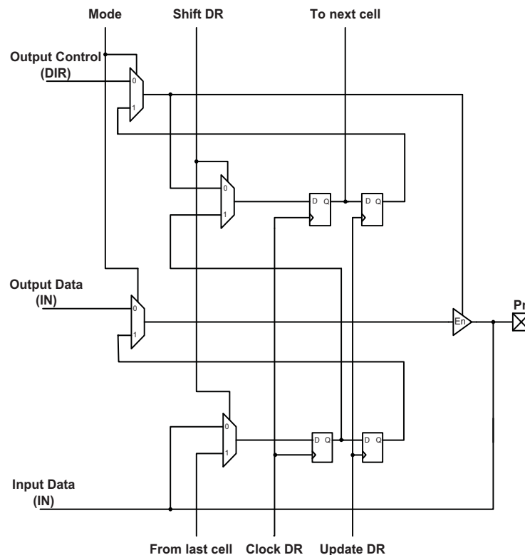
Figure 27-2. Boundary scan cell for bi-directional port pin.
