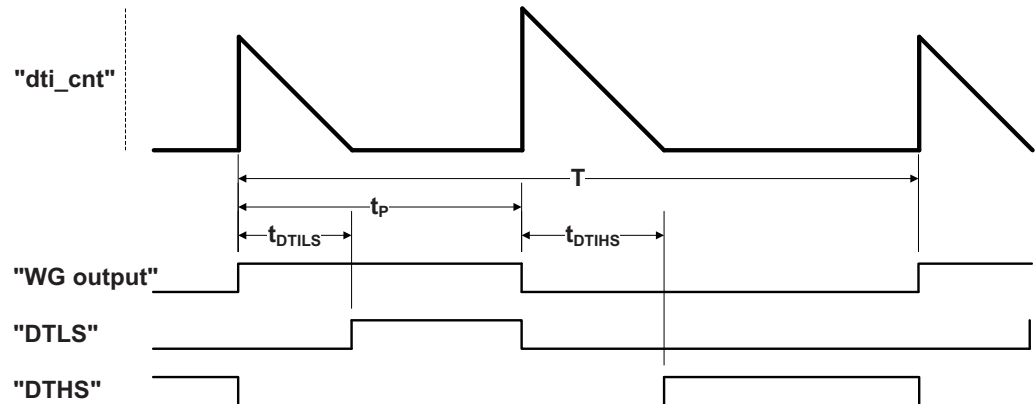
Figure 15-4. Dead-time generator timing diagram.
