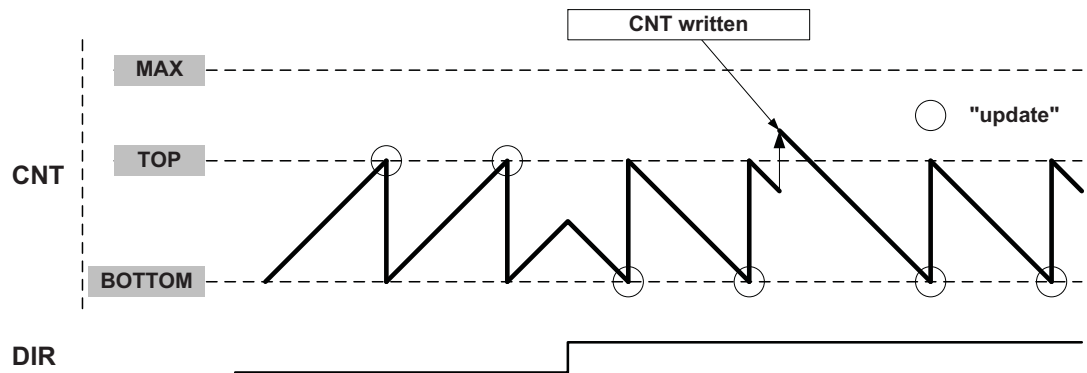
Figure 13-6. Normal operation.
