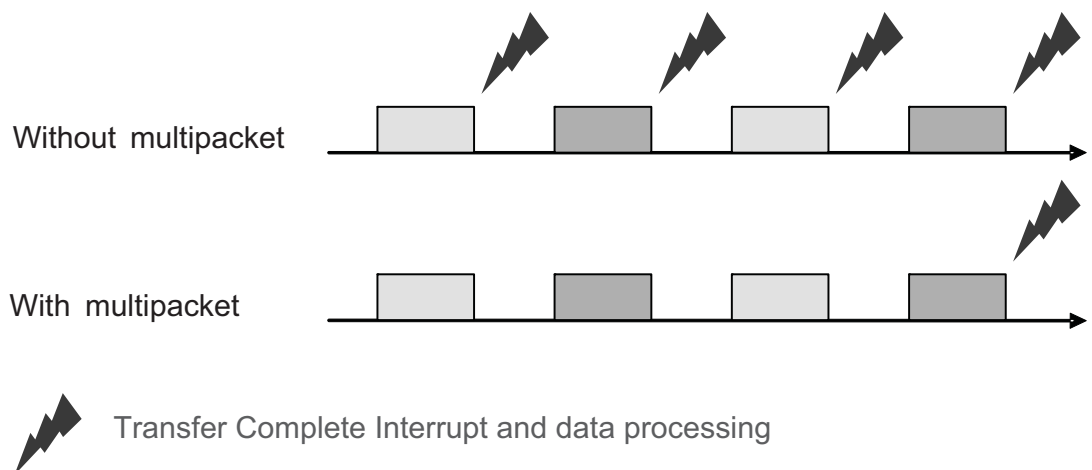
Figure 18-9. Multipacket overview.
