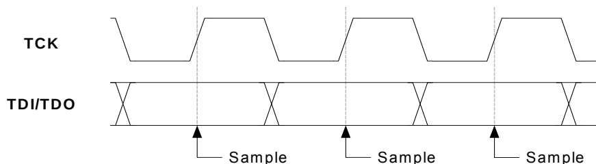
Figure 28-12. Changing and sampling data.
