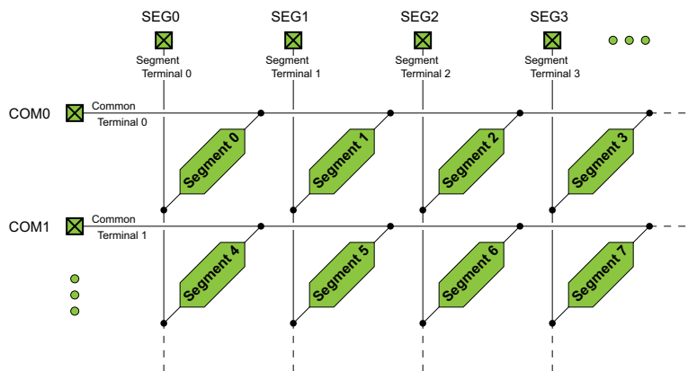
Figure 24-1. LCD Typical Connections
