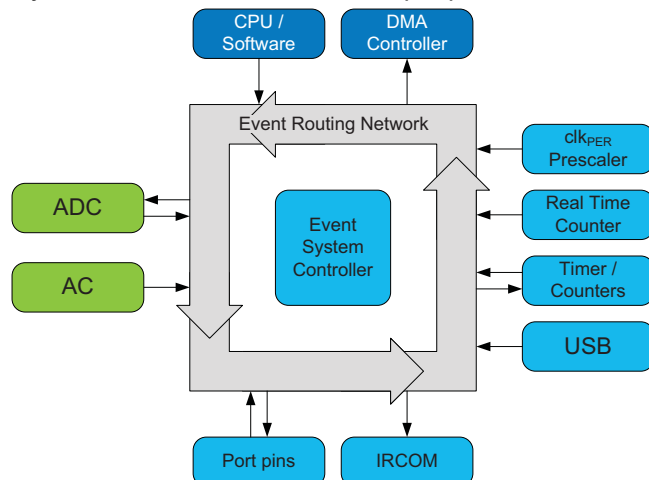
Figure 6-1. Event system overview and connected peripherals.
