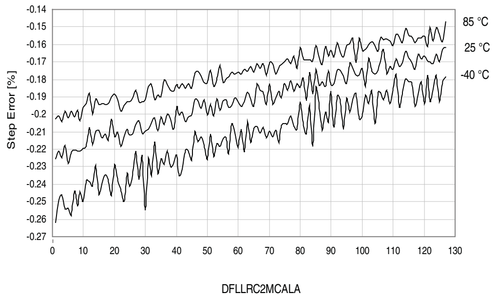
Figure 37-61. 2MHz internal oscillator CALB calibration step size.
