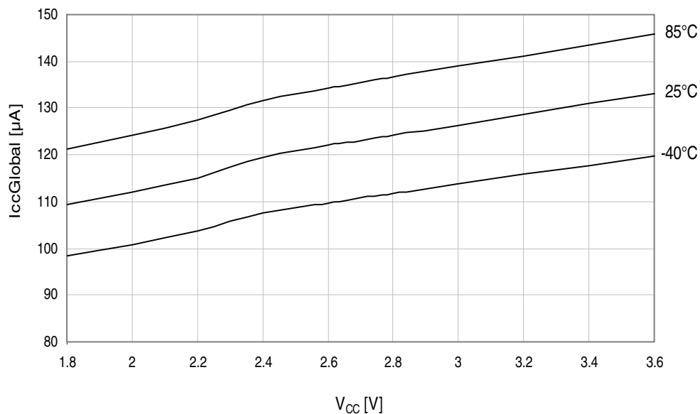
Figure 37-44. BOD current consumption vs. V_{CC} . Sampled mode, BOD level = 1.6V.
