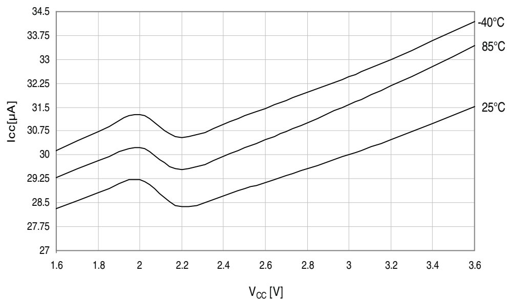
Figure 37-8. Idle mode supply current vs. V_{CC} . f_{SYS} = 2\text{MHz} internal oscillator.
