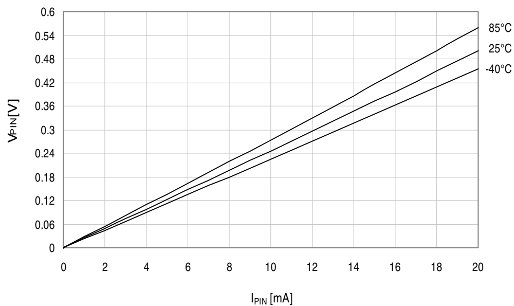
Figure 37-20. I/O pin output voltage vs. sink current. V_{CC} = 3.3V .
