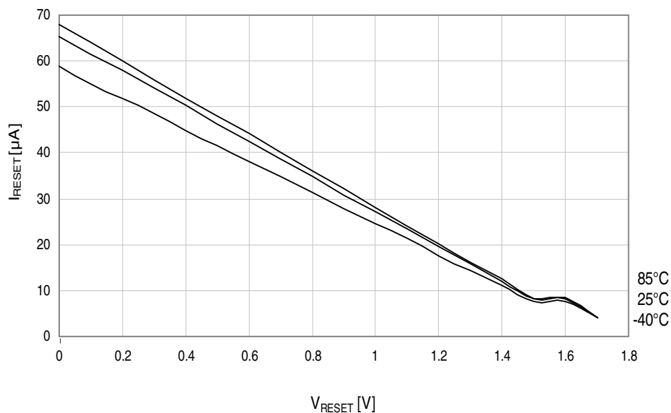
Figure 37-50. Reset pin pull-up resistor current vs. reset pin voltage. V_{CC} = 3.0V .
