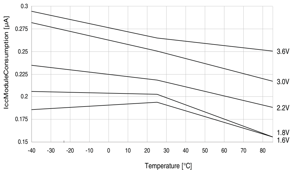
Figure 37-80. Psave vs. Temperature RTC, WDT, BOD sampled.
