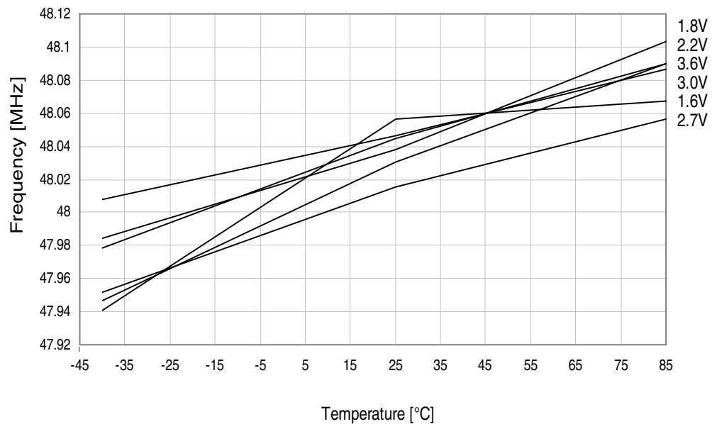
Figure 37-69. 48MHz internal oscillator frequency vs. temperature. DPLL enabled, from the 32.768kHz internal oscillator.
