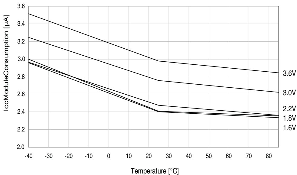
Figure 37-79. Psave LCD LP 32Hz vs. Temperature RTC, WDT, BOD sampled
