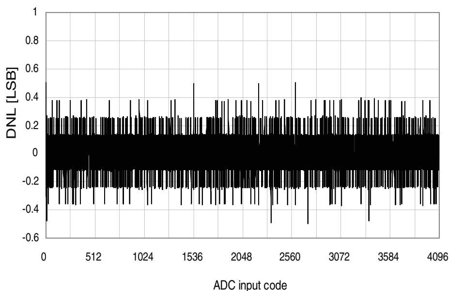
Figure 37-29. DNL error vs. input code.
