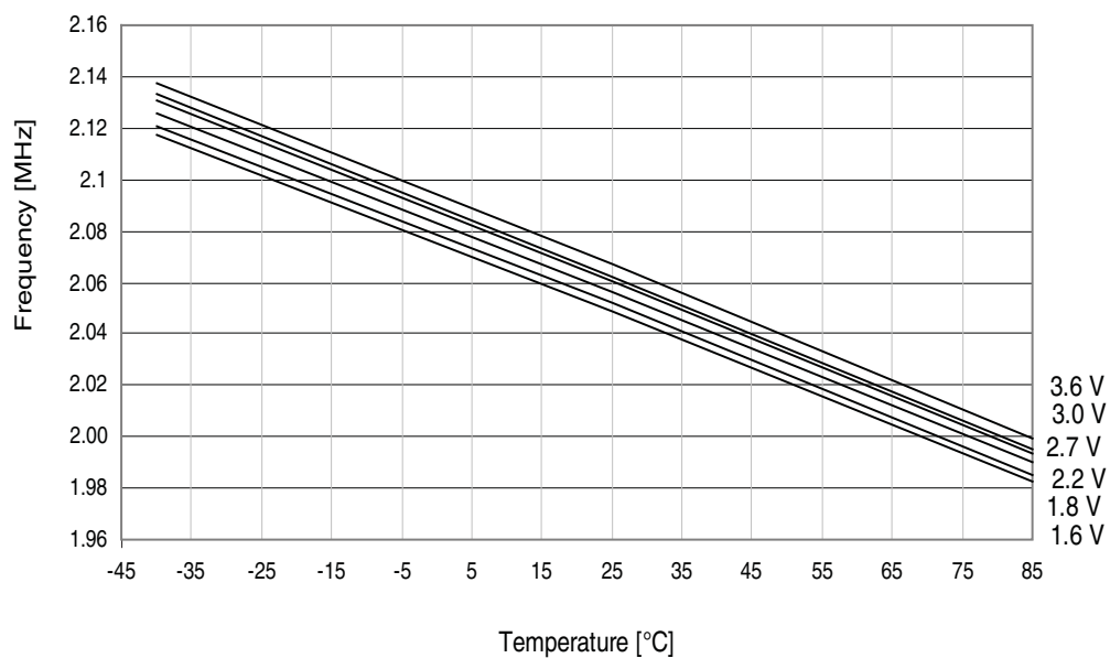
Figure 37-59. 2MHz internal oscillator frequency vs. temperature. DPLL enabled.
