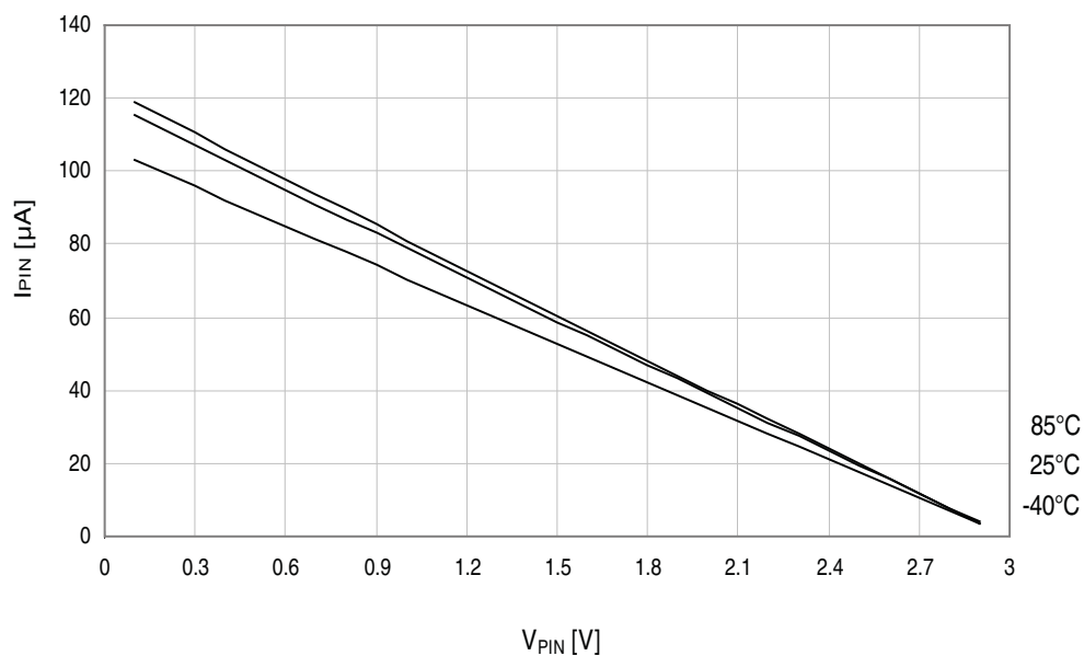
Figure 37-14. I/O pin pull-up resistor current vs. pin voltage. V_{CC} = 3.3V .
