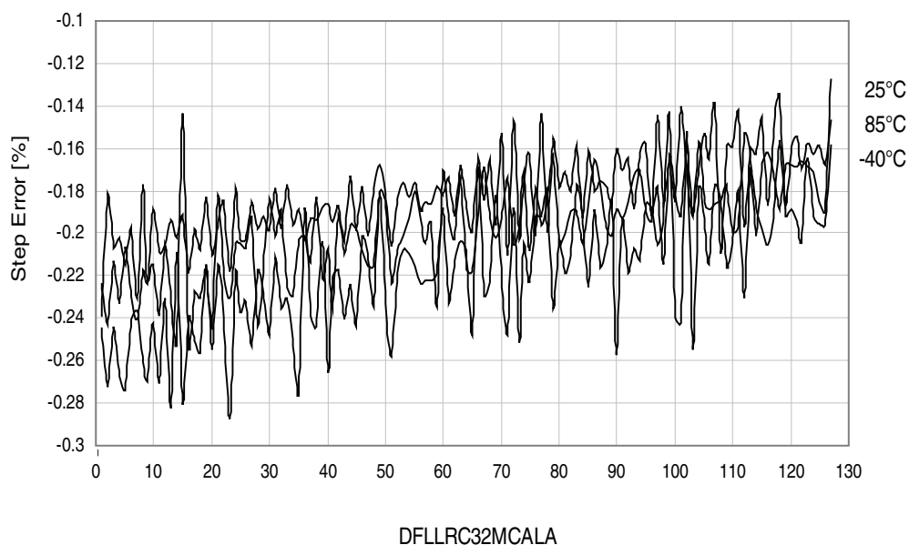
Figure 37-64. 32MHz internal oscillator CALA calibration step size. V_{CC} = 3.0V .
