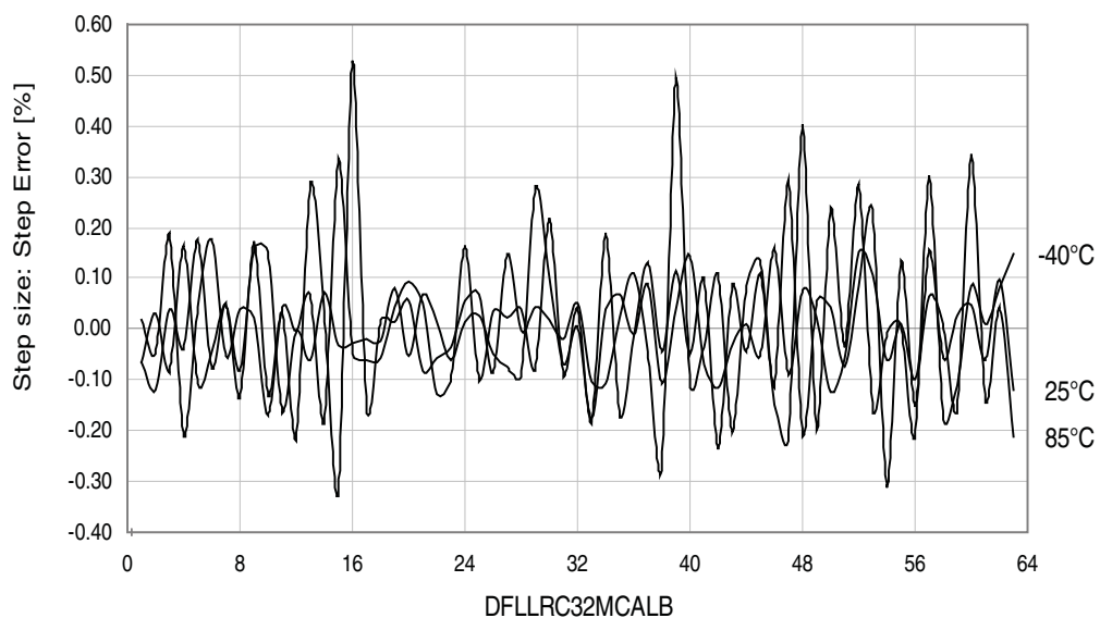
Figure 37-65. 32MHz internal oscillator CALB calibration step size. V_{CC} = 3.0V , CALA = mid value.
