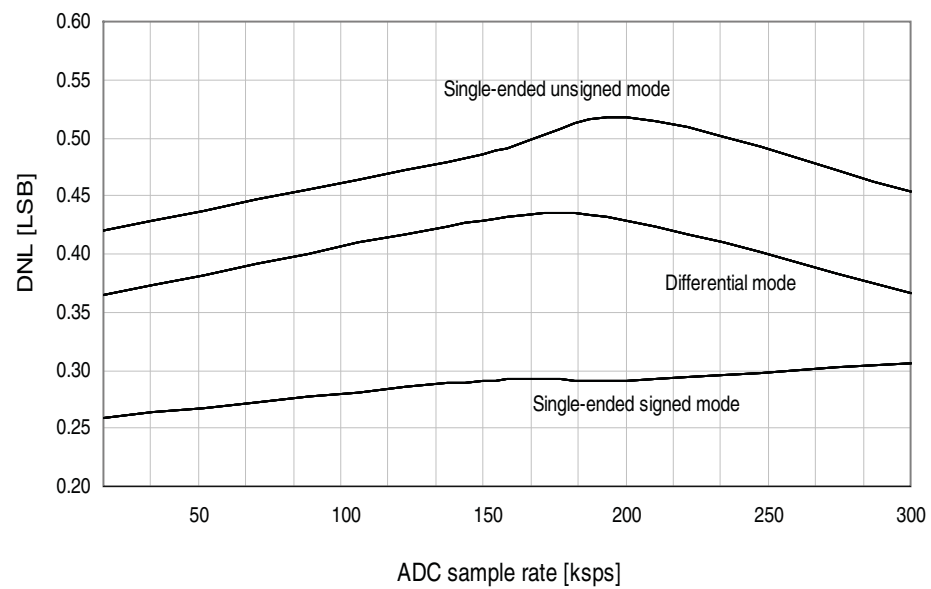
Figure 37-28. DNL error vs. sample rate. T = 25^{\circ}\text{C} , V_{CC} = 3.6\text{V} , V_{REF} = 3.0\text{V} external.
