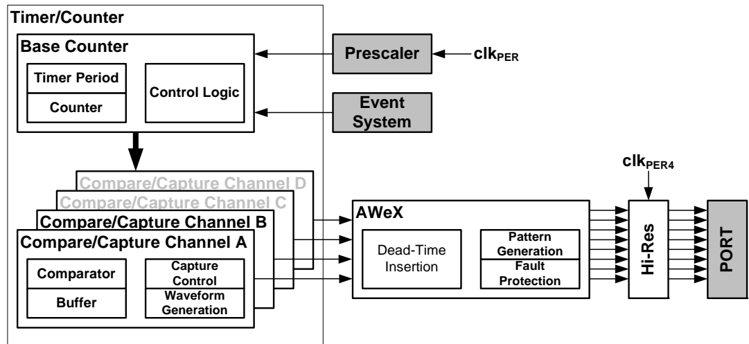
Figure 16-1. Overview of a Timer/Counter and closely related peripherals
