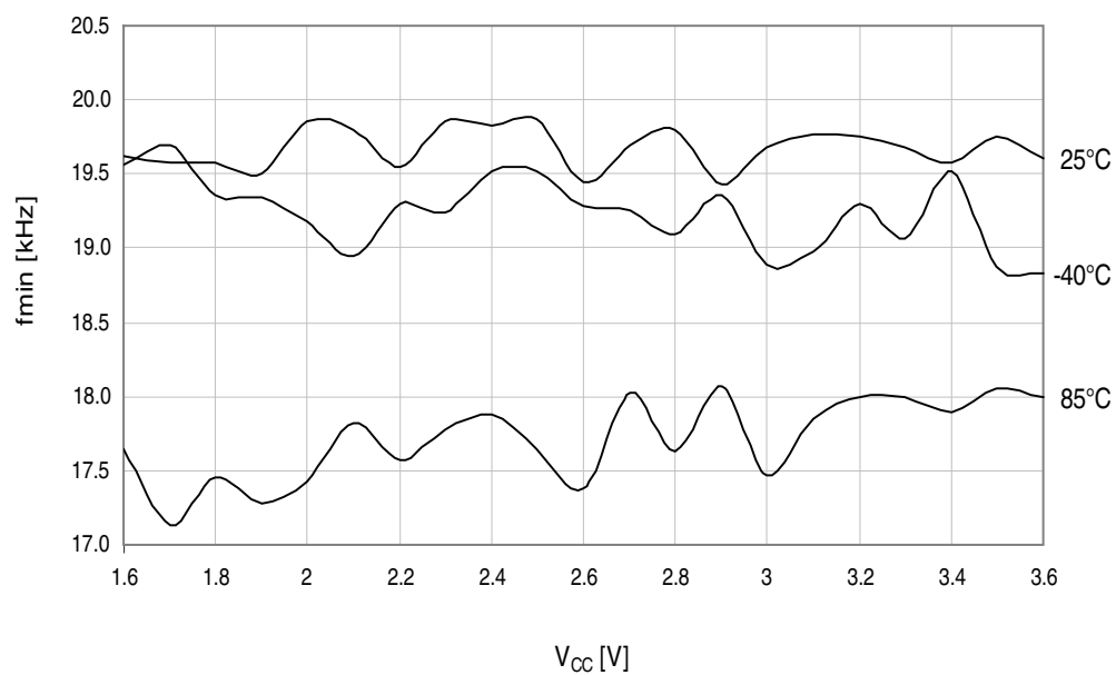
Figure 37-72. Maximum PDI frequency vs. V_{CC} .
