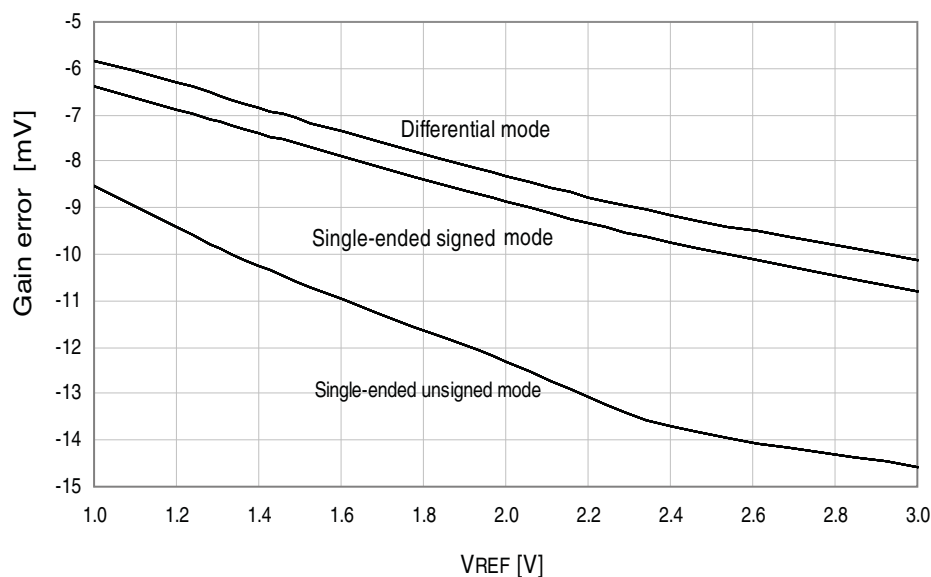
Figure 37-30. Gain error vs. V_{REF} .
