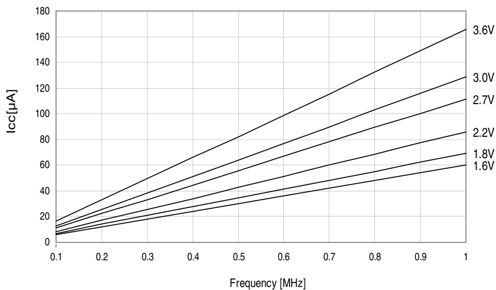
Figure 37-6. Idle mode supply current vs. frequency.
