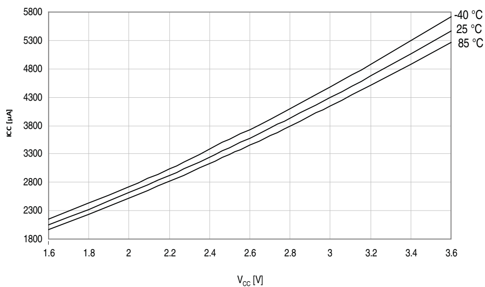
Figure 37-9. Idle mode current vs. V_{CC} . f_{SYS} = 32\text{MHz} internal oscillator.
