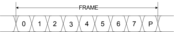
Figure 32-10.JTAG serial frame format
