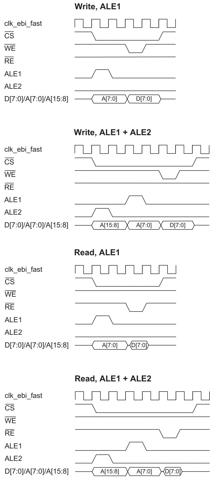
Figure 36-6. LPC 2- Port ALE12 CS
