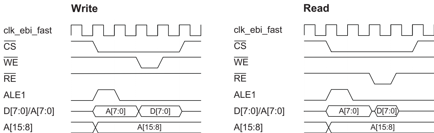
Figure 36-5. LPC 3- Port ALE1 CS
