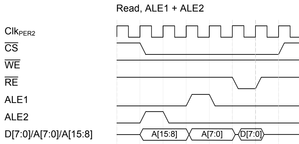
Figure 36-8. Read, ALE1 + ALE2
