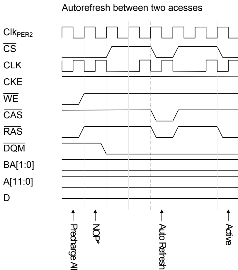
Figure 36-42. Autorefresh between two accesses
