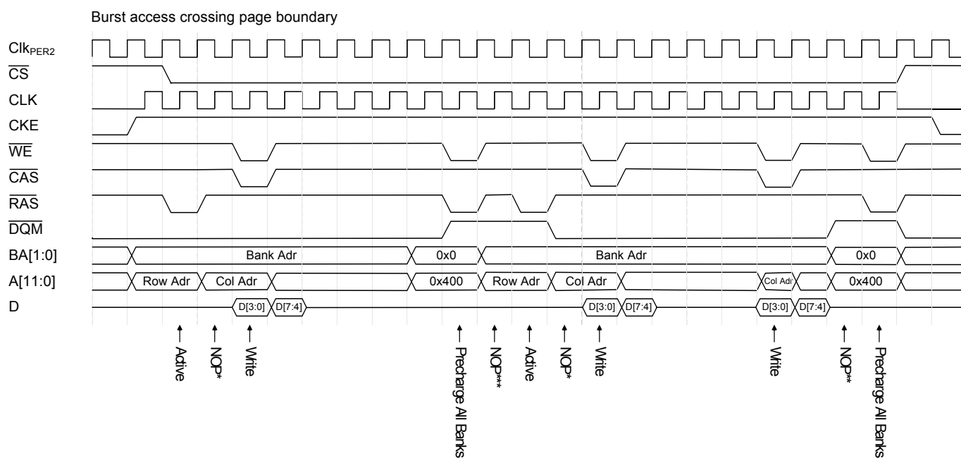
Figure 36-36. Burst access crossing page boundary
