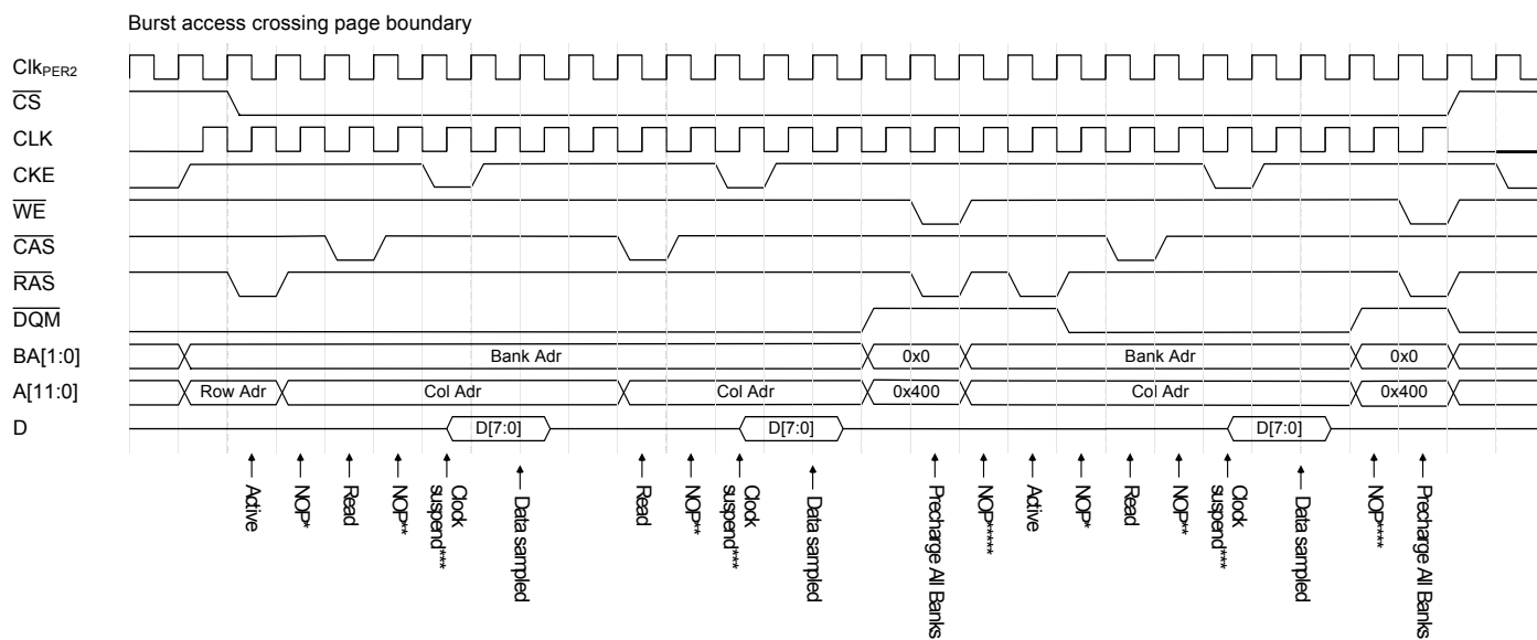
Figure 36-32. Burst access crossing page boundary
