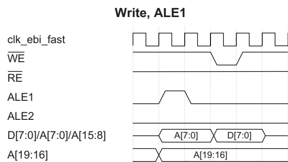
Figure 36-19.LPC 2 - Port ALE12 no CS
