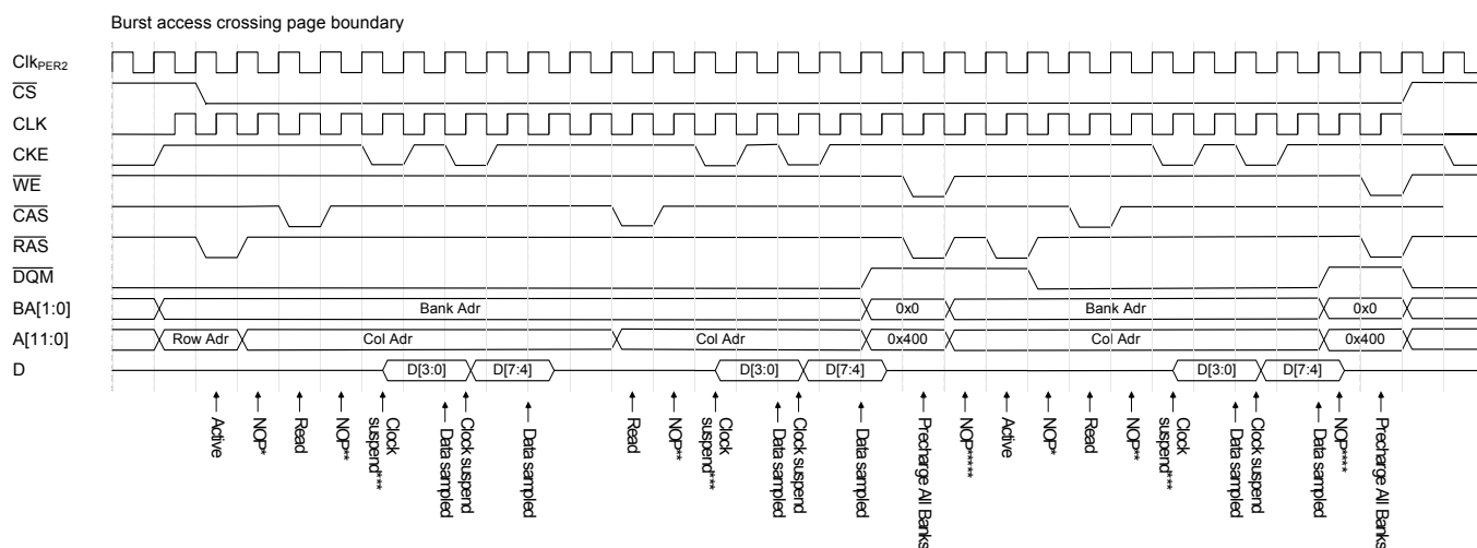
Figure 36-40. Burst access crossing page boundary
