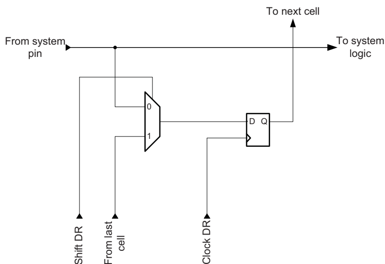
Figure 31-3. An observe-only input cell.
