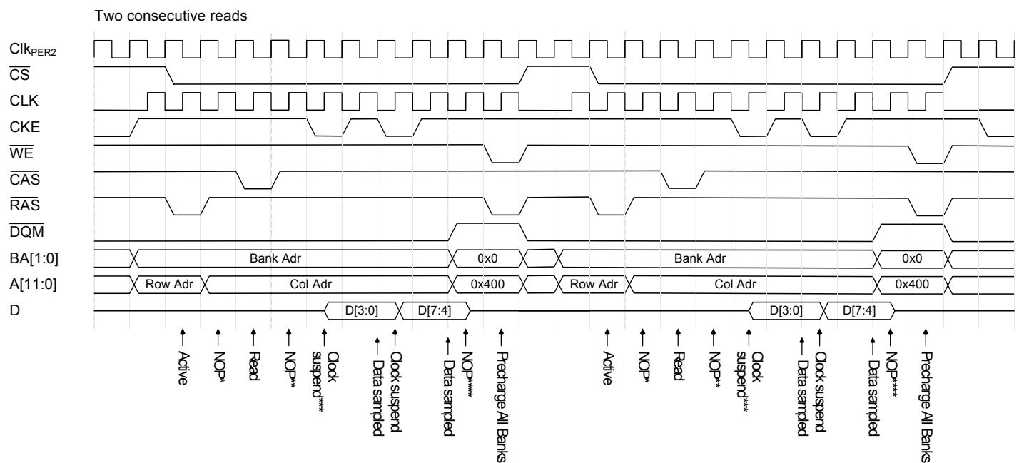
Figure 36-38. Two consecutive reads
