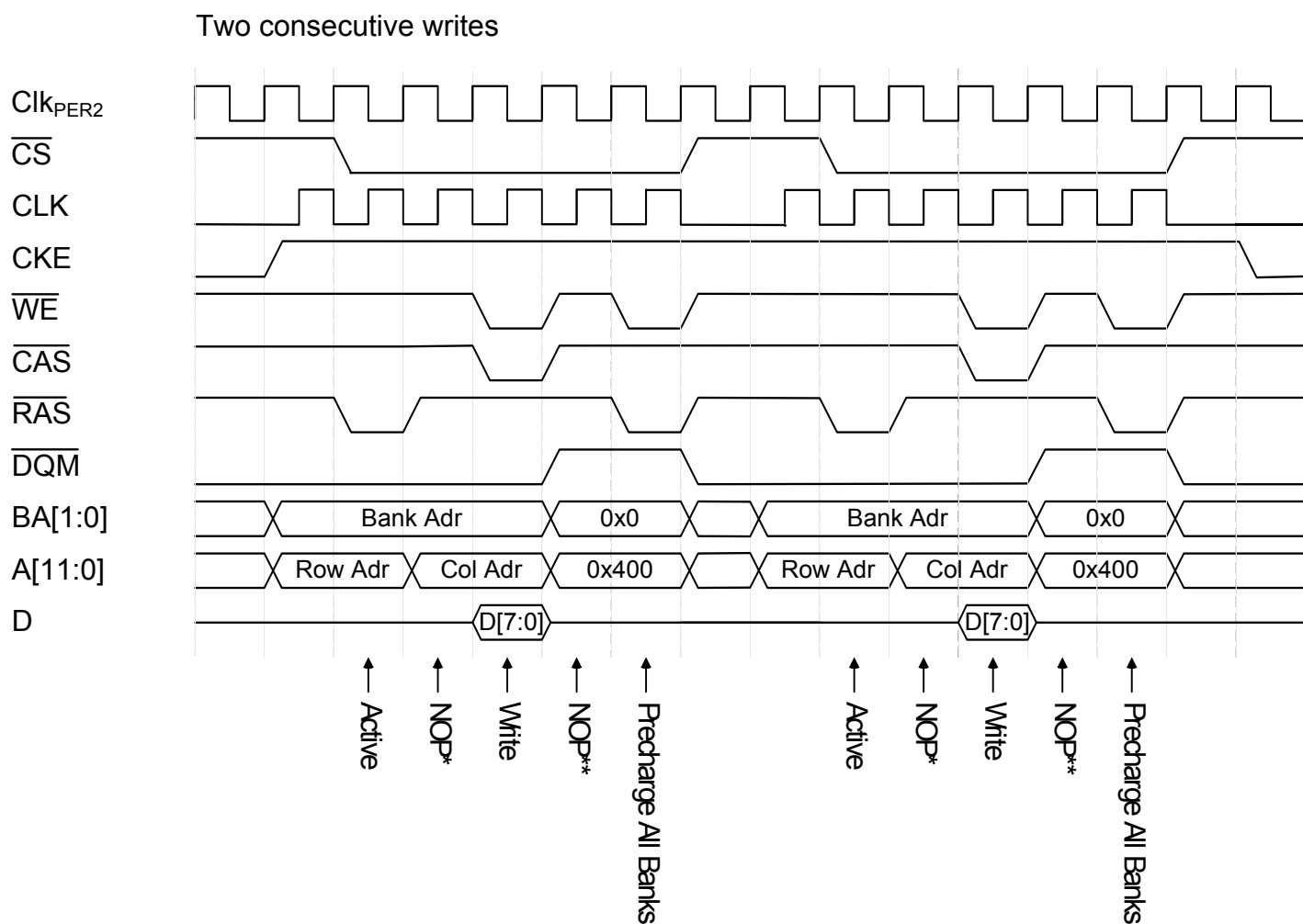
Figure 36-26. Two consecutive writes
