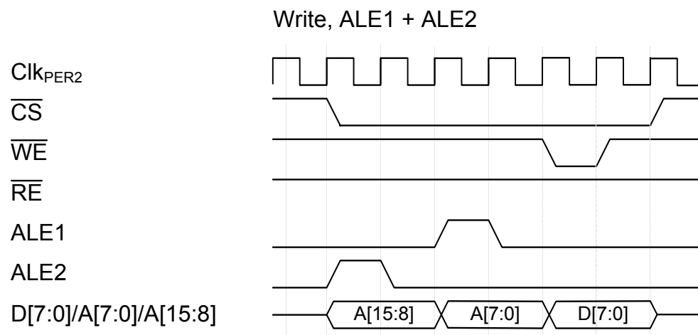
Figure 36-6. Write, ALE1 + ALE2
