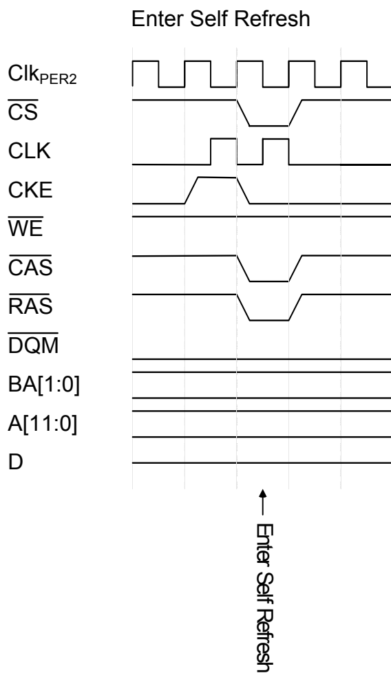
Figure 36-43. Enter Self Refresh
