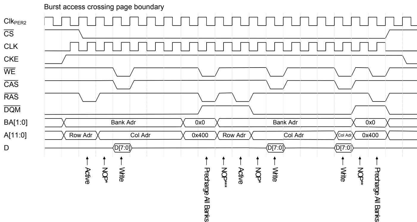
Figure 36-28. Burst access crossing page boundary
