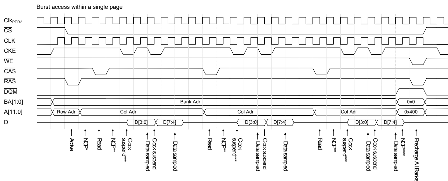
Figure 36-39. Burst access within a single page
