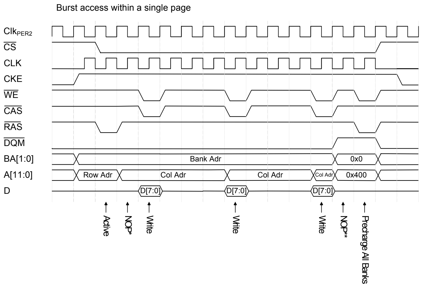
Figure 36-27. Burst access within a single page
