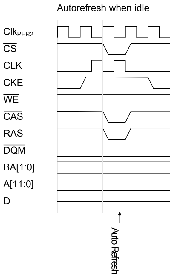
Figure 36-41. Autorefresh when idle
