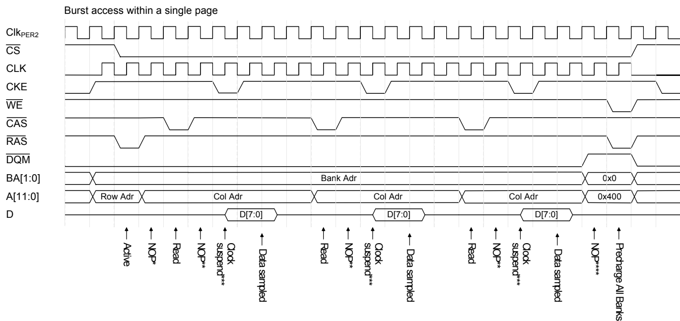
Figure 36-31. Burst access within a single page
