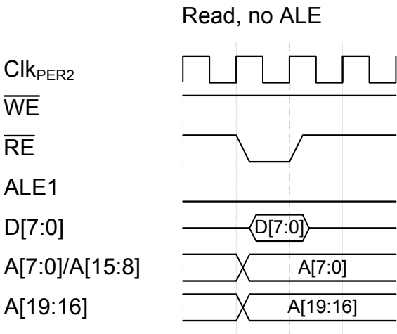
Figure 36-15. Read, no ALE
