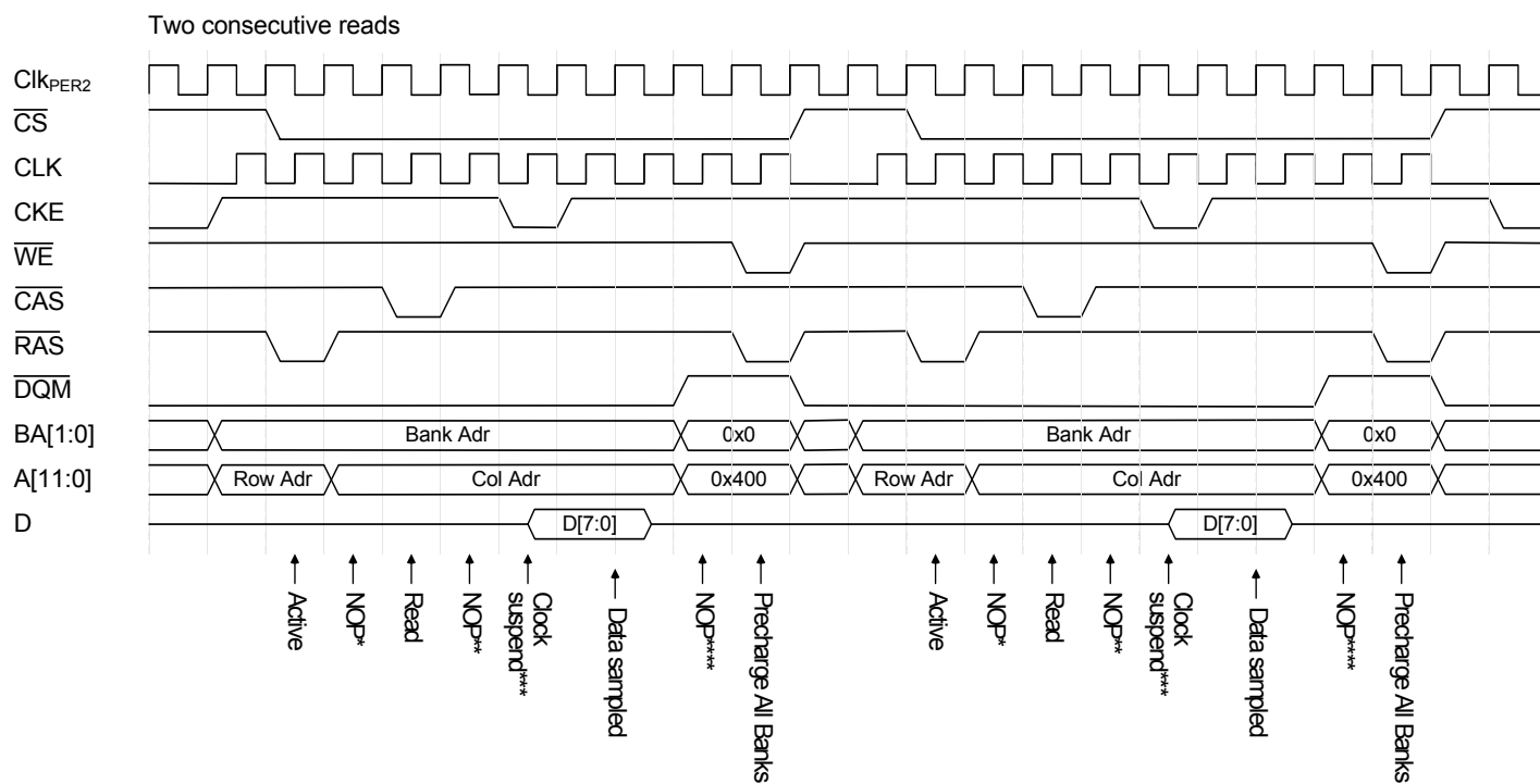
Figure 36-30. Two consecutive reads
