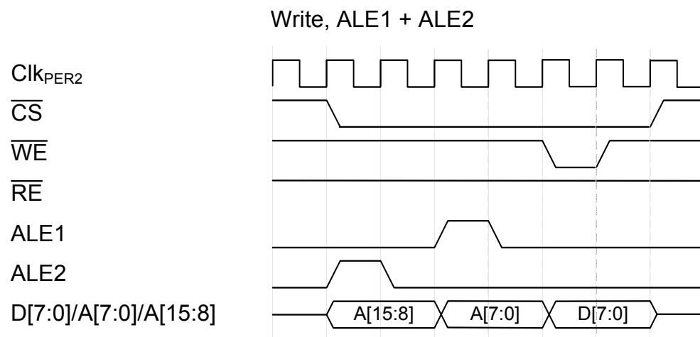
Figure 36-21. Write, ALE1 + ALE2
