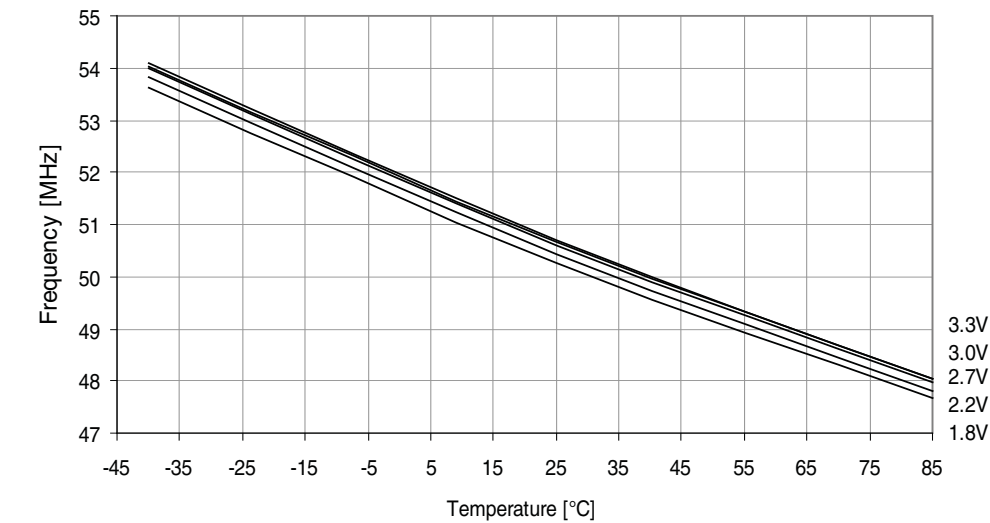
Figure 37-327. 48MHz internal oscillator frequency vs. temperature. DPLL disabled.
