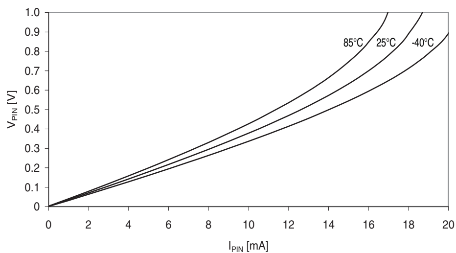
Figure 37-193. I/O pin output voltage vs. sink current.
