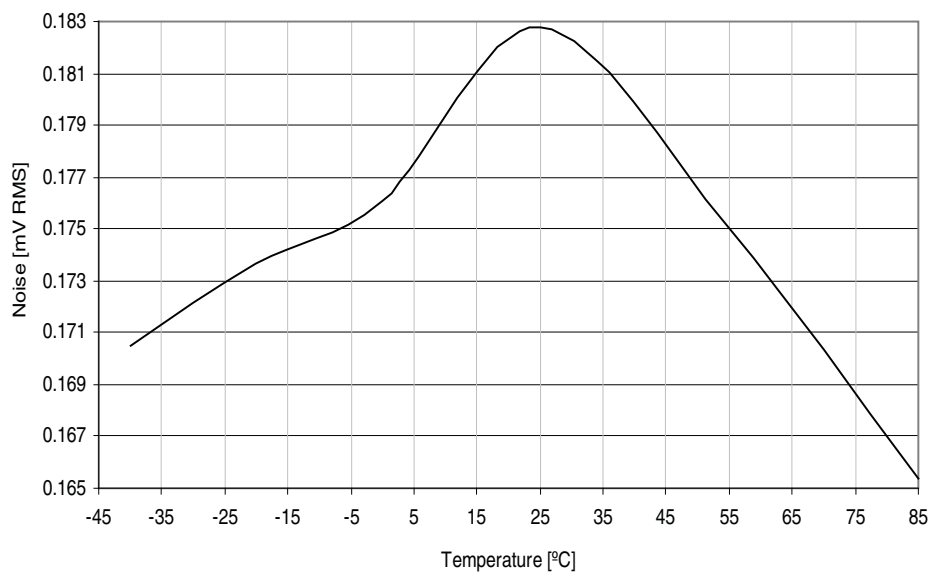
Figure 37-299. DAC noise vs. temperature. V_{CC} = 3.0\text{V} , V_{REF} = 2.4\text{V} .
