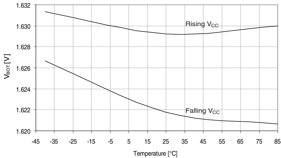
Figure 37-225. BOD thresholds vs. temperature. BOD level = 1.6V.
