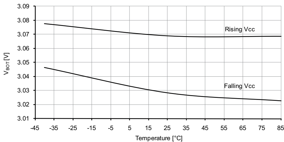
Figure 37-143. BOD thresholds vs. temperature.
