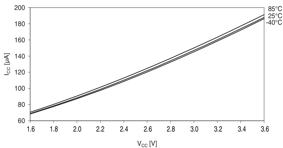
Figure 37-260. Idle mode supply current vs. V_{CC} .
