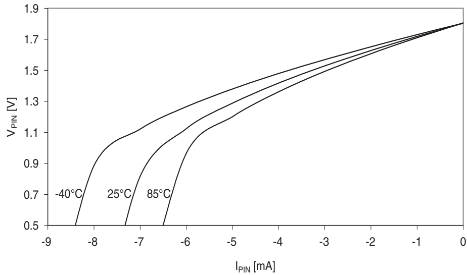
Figure 37-190. I/O pin output voltage vs. source current.
