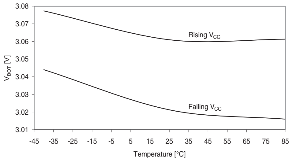
Figure 37-226. BOD thresholds vs. temperature. BOD level = 3.0V.
