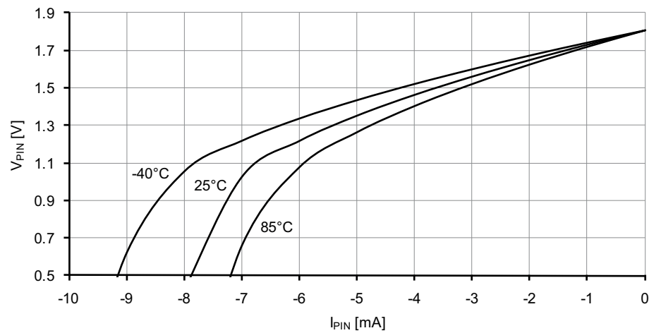
Figure 37-23. I/O pin output voltage vs. source current. V_{CC} = 1.8V .
