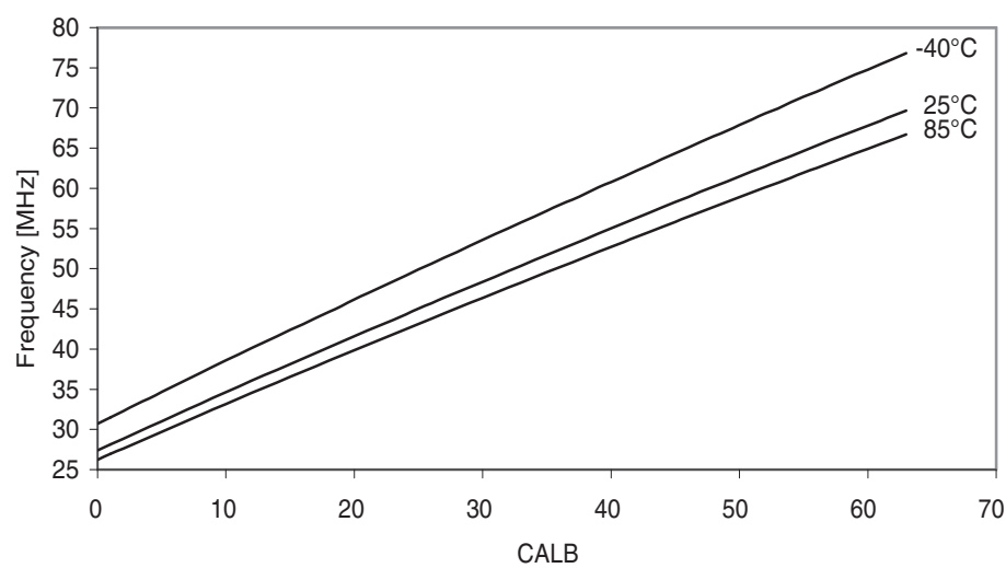
Figure 37-326. 32MHz internal oscillator frequency vs. CALB calibration value.
