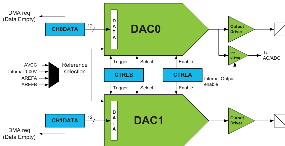
Figure 29-1. DAC overview.
