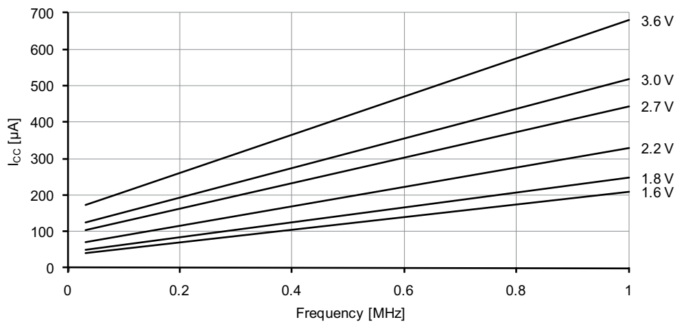
Figure 37-1. Active supply current vs. frequency. f_{SYS} = 0 - 1\text{MHz} external clock, T = 25^{\circ}\text{C} .
