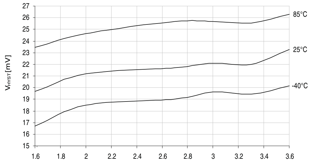
Figure 37-135. Analog comparator hysteresis vs. V_{CC} . Low power, small hysteresis.
