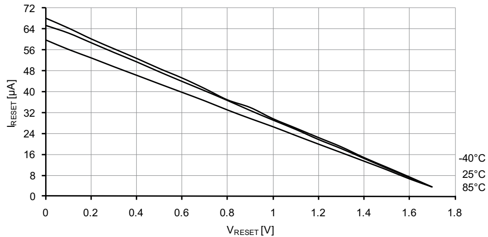
Figure 37-62. Reset pin pull-up resistor current vs. reset pin voltage. V_{CC} = 1.8V .
