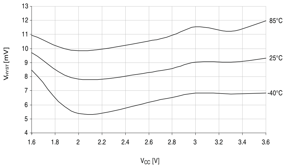
Figure 37-52. Analog comparator hysteresis vs. V_{CC} .
