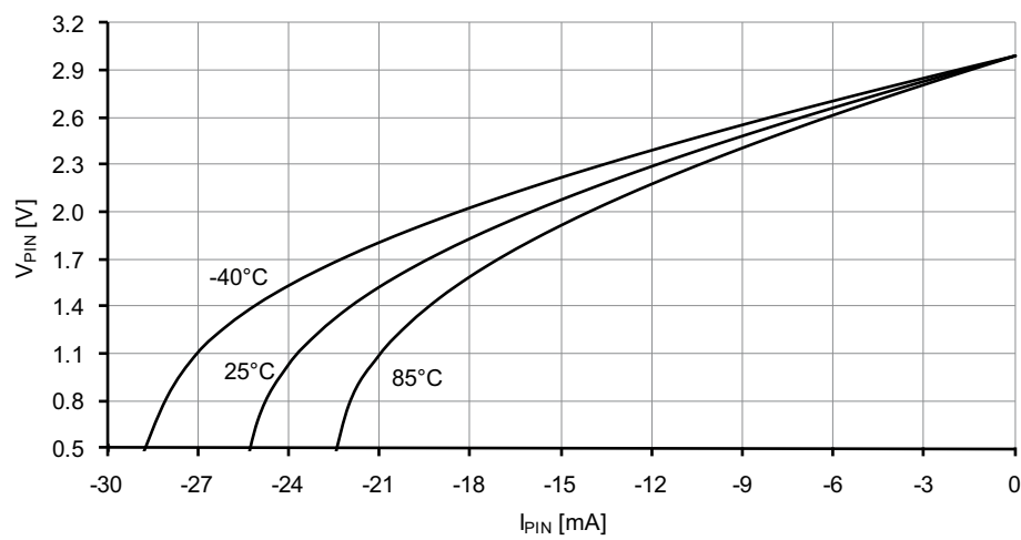
Figure 37-107. I/O pin output voltage vs. source current. V_{CC} = 3.0V .
