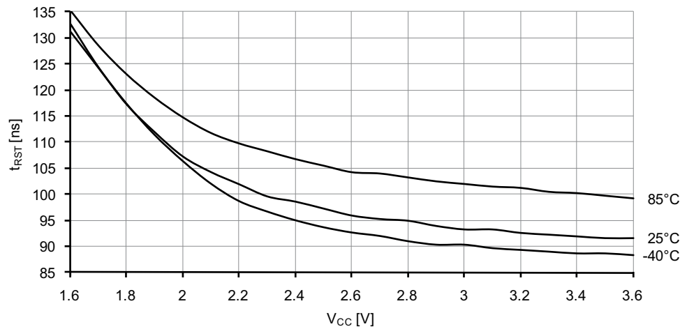
Figure 37-61. Minimum Reset pin pulse width vs. V_{CC} .
