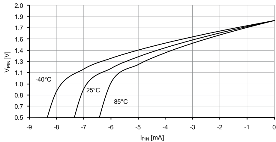
Figure 37-106. I/O pin output voltage vs. source current. V_{CC} = 1.8V .
