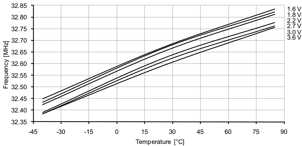
Figure 37-152. 32.768kHz internal oscillator frequency vs. temperature.
