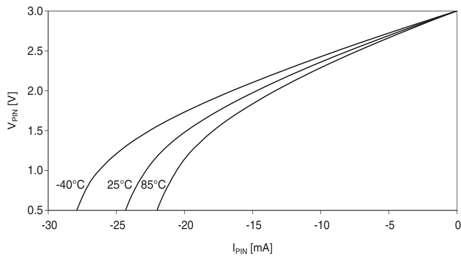
Figure 37-190. I/O pin output voltage vs. source current.
