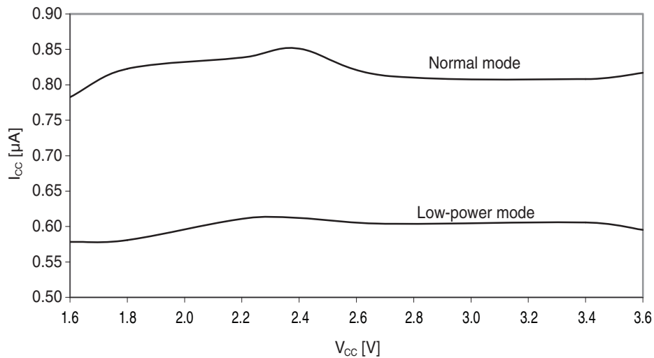
Figure 37-183. Power-save mode supply current vs. V_{CC} .
