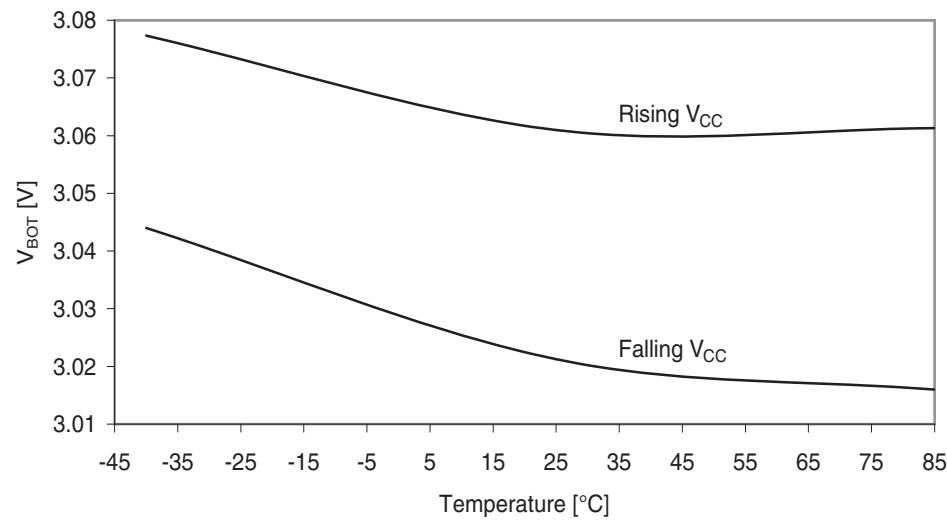
Figure 37-309. BOD thresholds vs. temperature.
