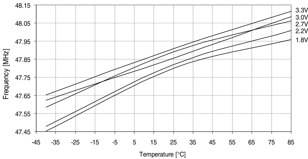
Figure 37-328. 48MHz internal oscillator frequency vs. temperature. DPLL enabled, from the 32.768kHz internal oscillator.
