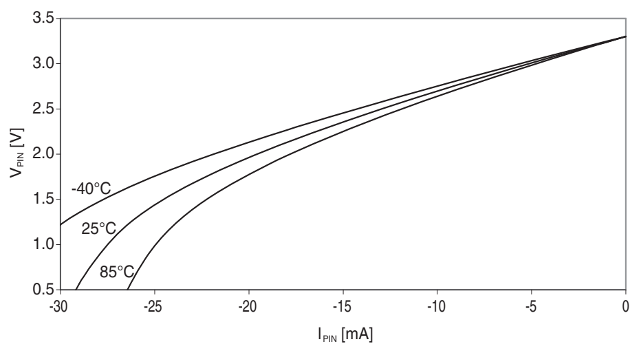
Figure 37-192. I/O pin output voltage vs. source current.
