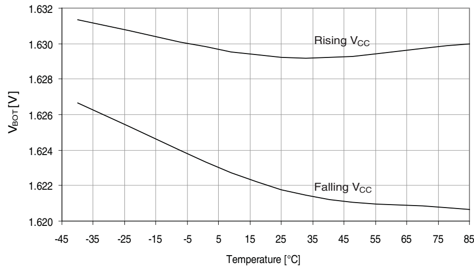
Figure 37-308. BOD thresholds vs. temperature.
