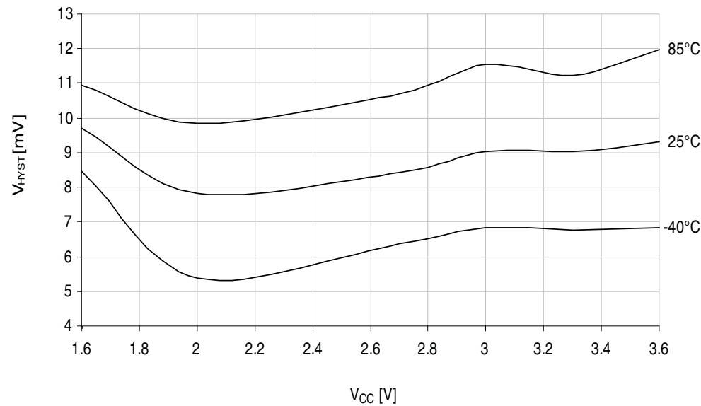
Figure 37-135. Analog comparator hysteresis vs. V_{CC} . Low power, small hysteresis.
