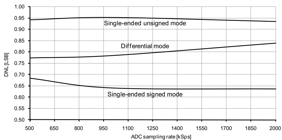
Figure 37-122. DNL error vs. sample rate.
