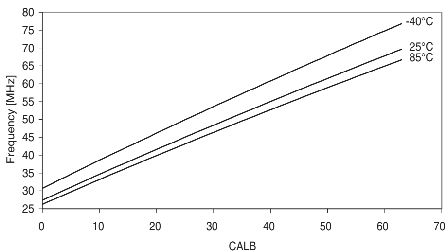
Figure 37-243. 32MHz internal oscillator frequency vs. CALB calibration value.
