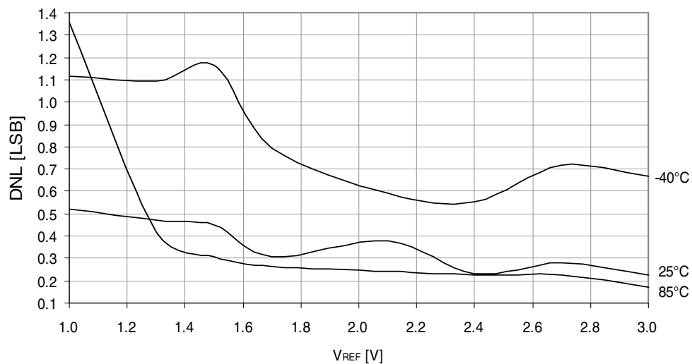
Figure 37-215. DNL error vs. V_{REF} . T = 25^{\circ}\text{C} , V_{CC} = 3.6\text{V} .
