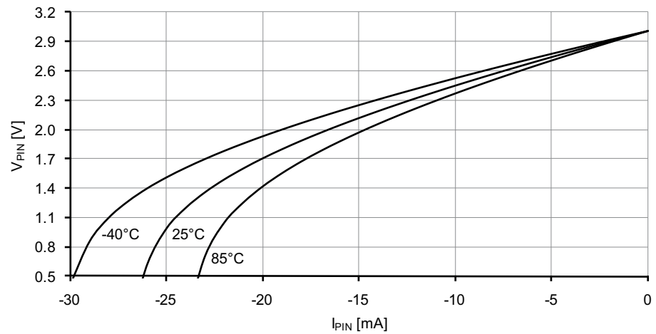
Figure 37-24. I/O pin output voltage vs. source current. V_{CC} = 3.0V .
