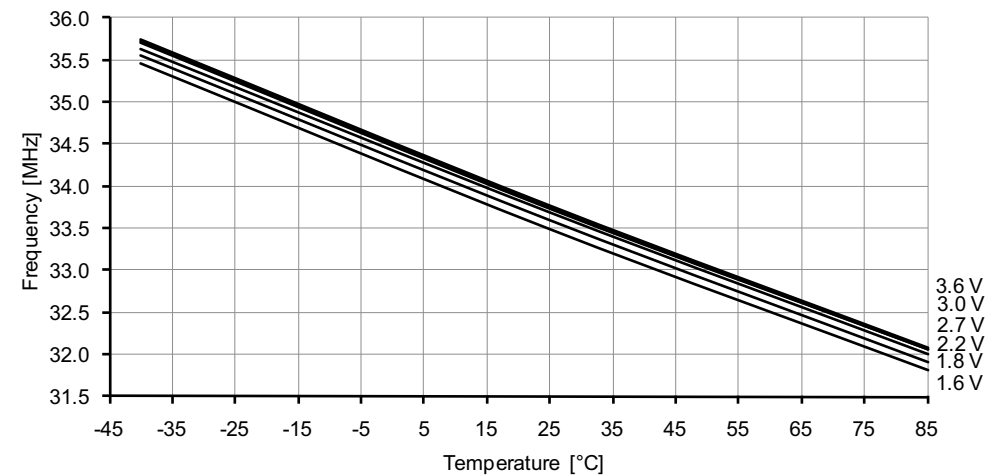
Figure 37-75. 32MHz internal oscillator frequency vs. temperature. DFLL enabled, from the 32.768kHz internal oscillator.
