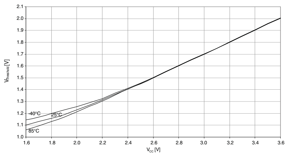
Figure 37-231. Reset pin input threshold voltage vs. V_{CC} .
