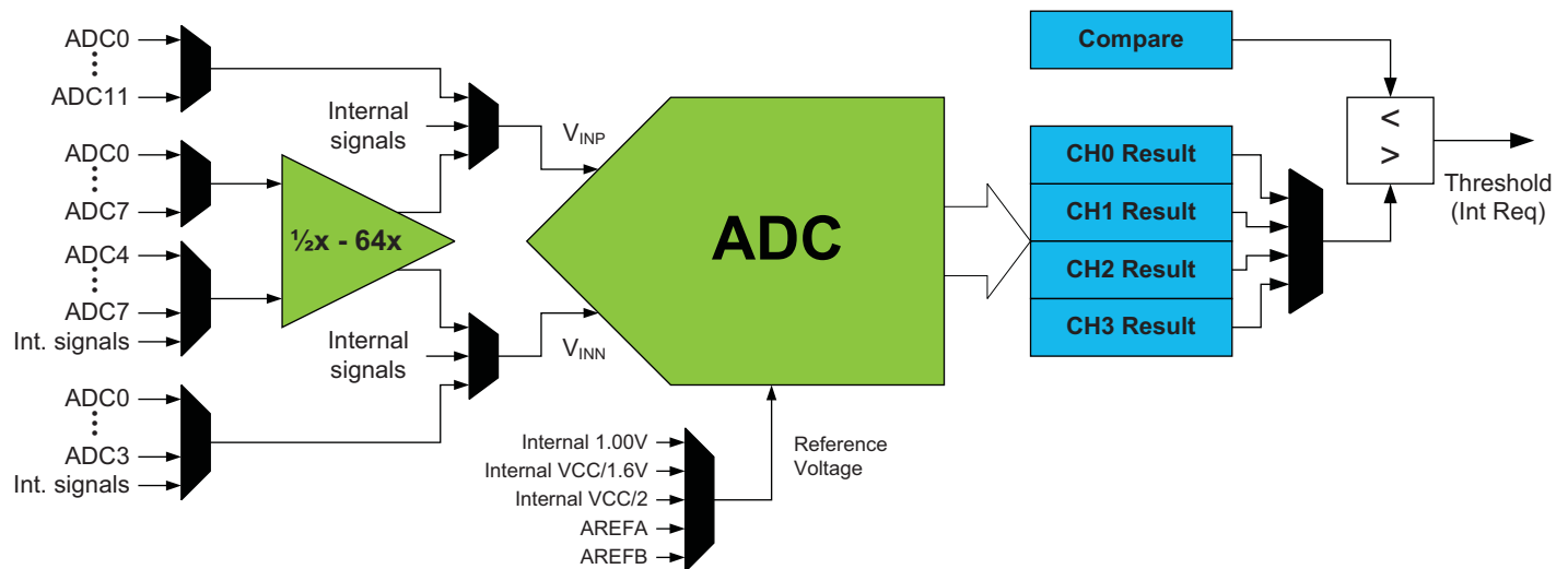
Figure 28-1. ADC overview.
