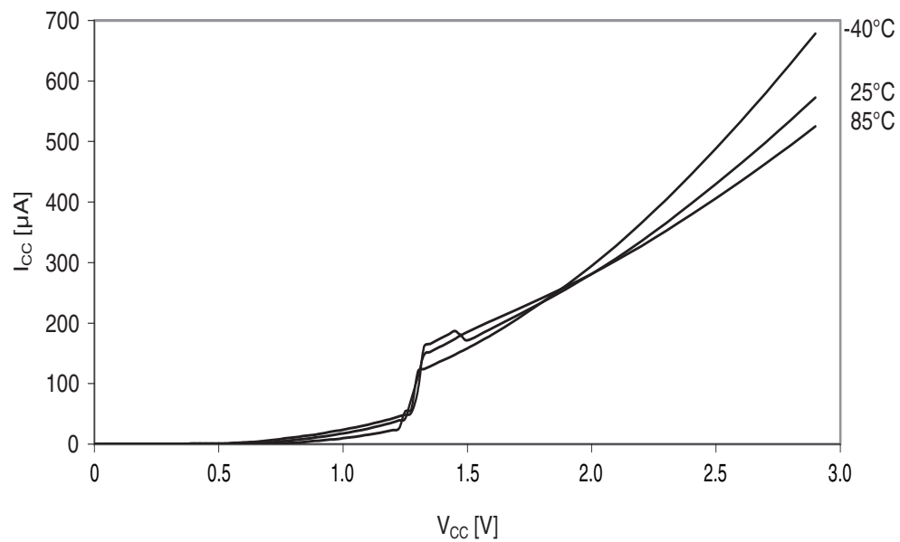
Figure 37-316. Power-on reset current consumption vs. V_{CC} .
