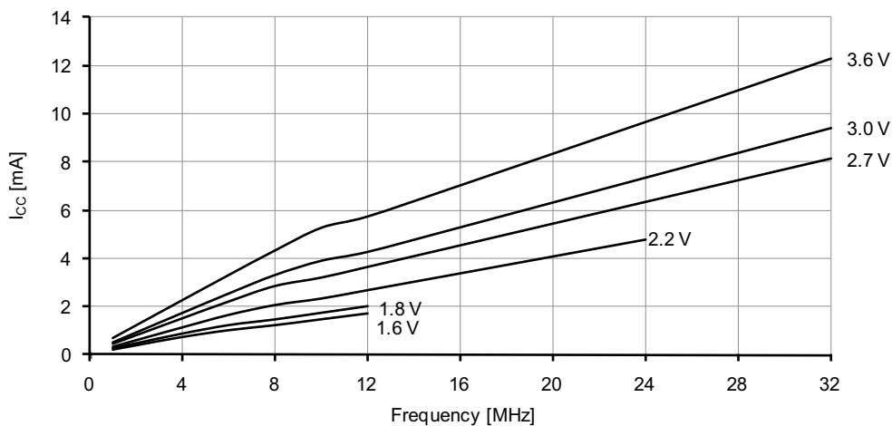
Figure 37-2. Active supply current vs. frequency. f_{SYS} = 1 - 32\text{MHz} external clock, T = 25^{\circ}\text{C} .
