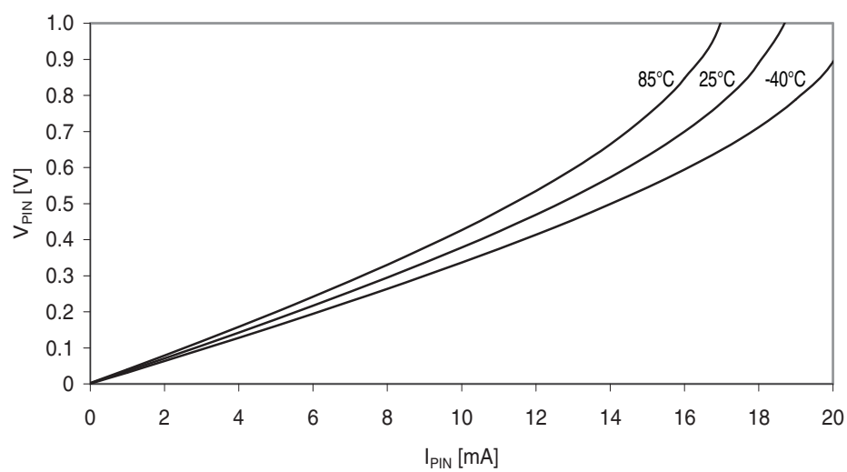
Figure 37-277. I/O pin output voltage vs. sink current.
