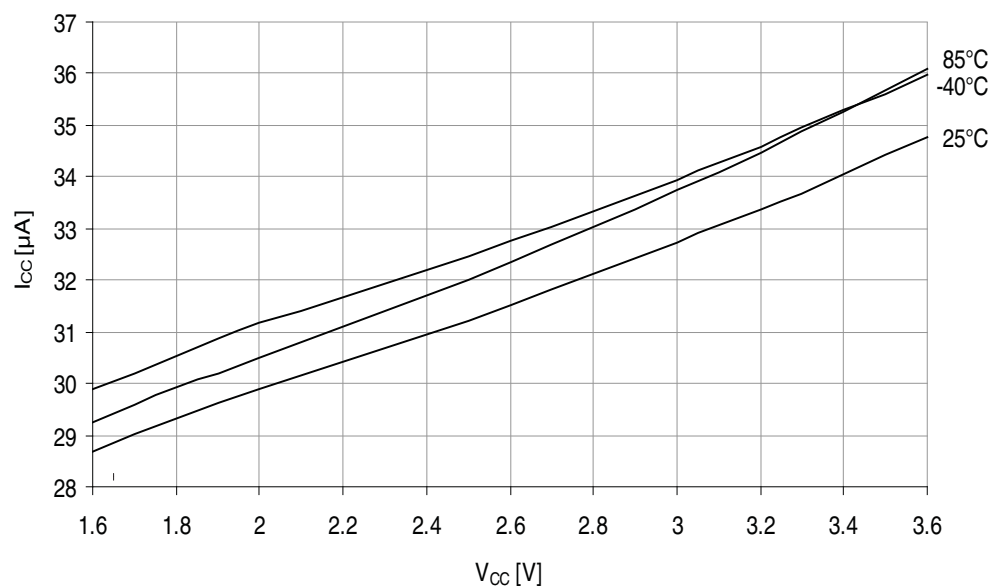
Figure 38-10. Idle mode supply current vs. V_{\text{CC}} .
