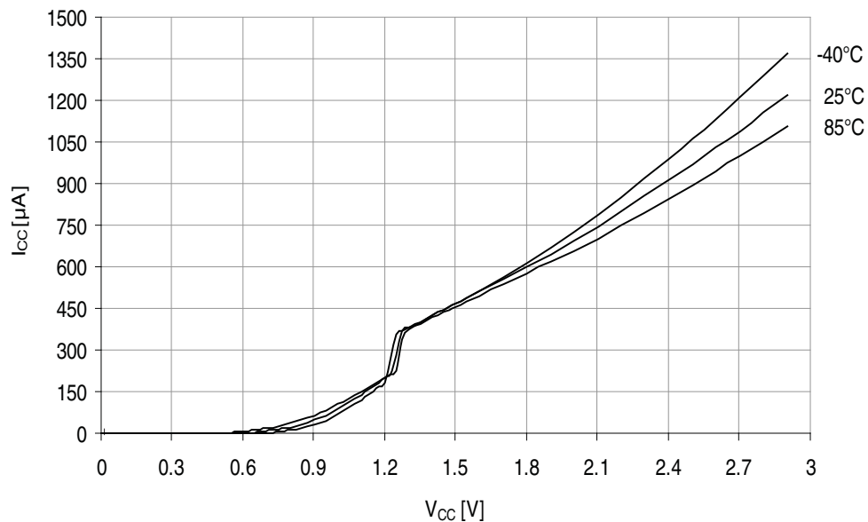
Figure 38-150. Power-on reset current consumption vs. V_{CC} .
