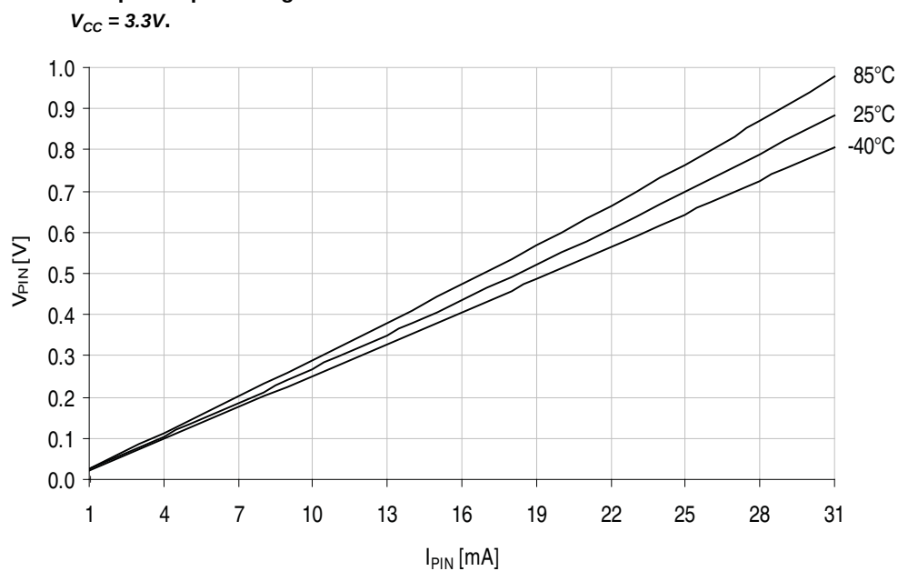
Figure 38-111. I/O pin output voltage vs. sink current.
