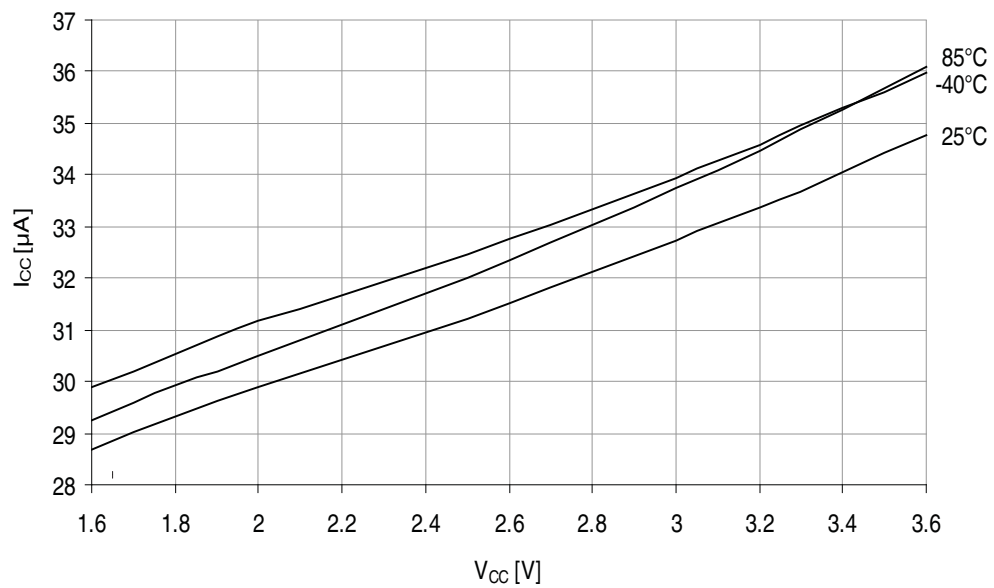
Figure 38-92. Idle mode supply current vs. V_{\text{CC}} .
