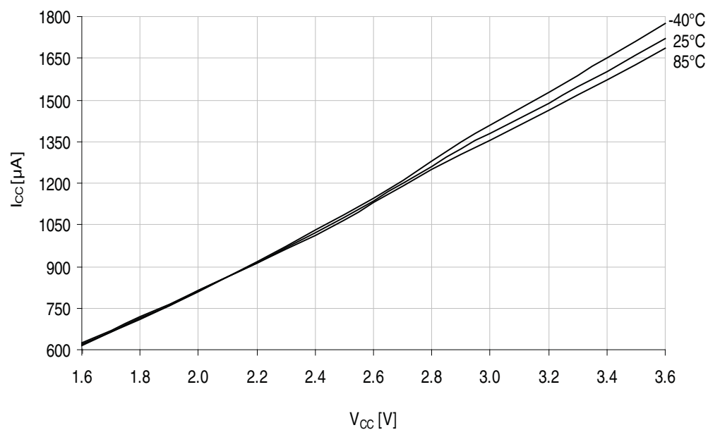
Figure 38-88. Active mode supply current vs. V_{CC} .
