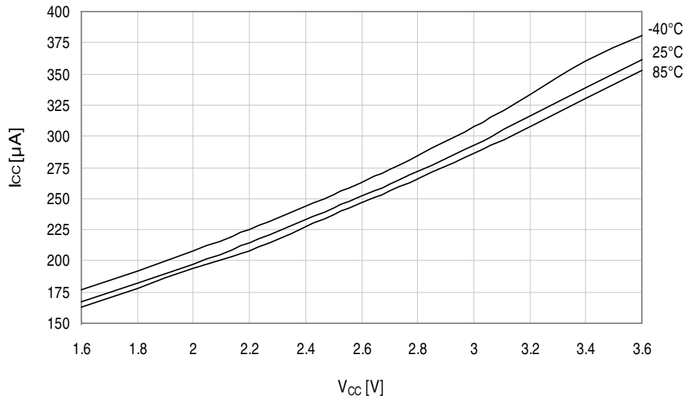
Figure 36-12. Idle mode supply current vs. V_{CC} .
