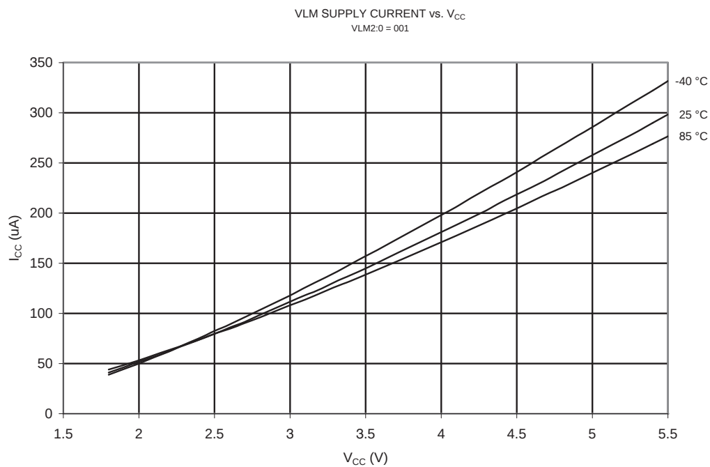
Figure 17-49. Temperature Dependence of VLM Current vs. V_{CC}
