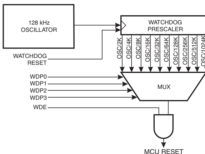
Figure 8-6. Watchdog Timer
