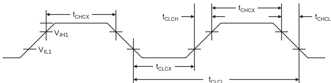
Figure 16-2. External Clock Drive Waveform
