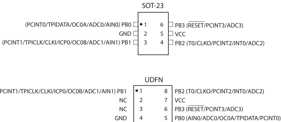
Figure 1-1. Pinout of ATtiny4/5/9/10
