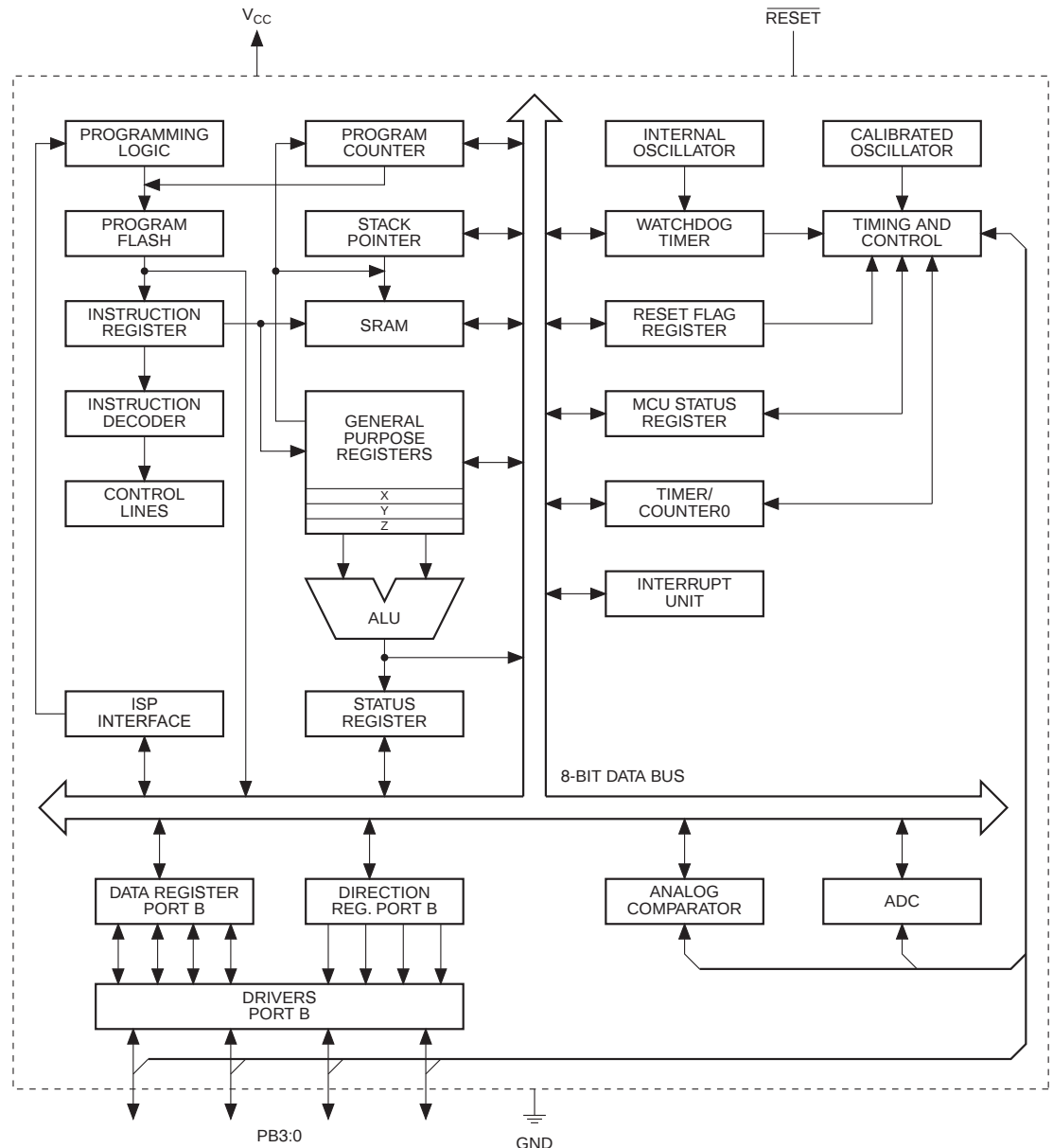
Figure 2-1. Block Diagram
