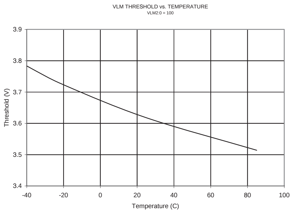
Figure 17-45. VLM3 Threshold of V_{CC} Level Monitorr2
