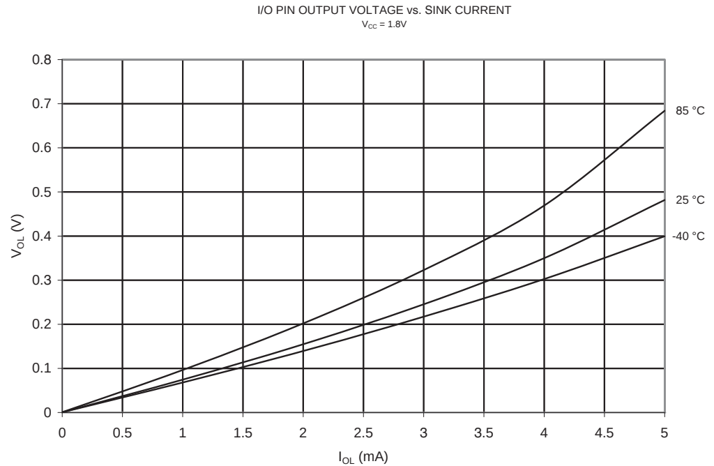
Figure 17-19. I/O Pin Output Voltage vs. Sink Current ( V_{CC} = 1.8V )
