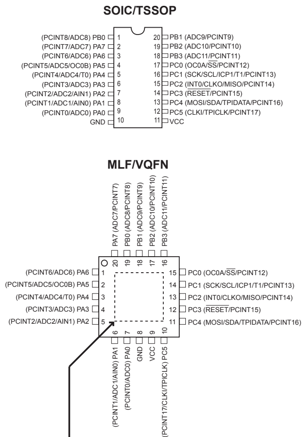
Figure 1-1. Pinout of ATtiny40
