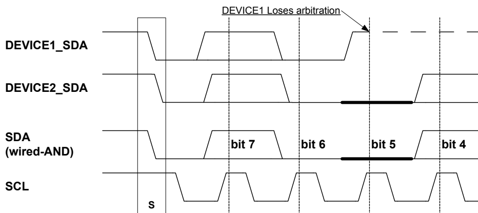
Figure 17-9. TWI Arbitration
