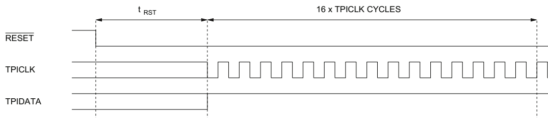
Figure 19-2. Sequence for enabling the Tiny Programming Interface
