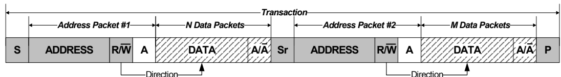
Figure 17-7. Combined Transaction
