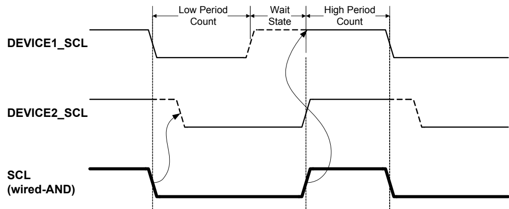
Figure 17-10. Clock Synchronization
