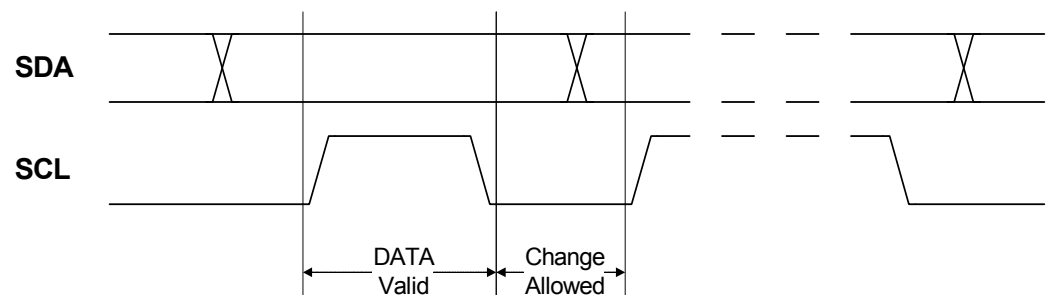
Figure 17-4. Data Validity
