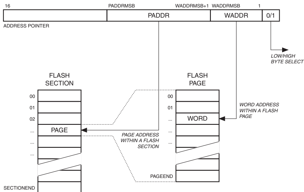
Figure 20-1. Addressing the Flash Memory
