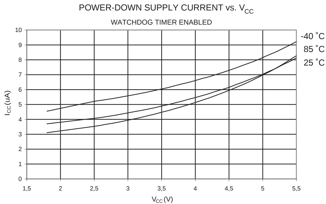
Figure 20-12. Power-down Supply Current vs. V_{CC} (Watchdog Timer Enabled)
