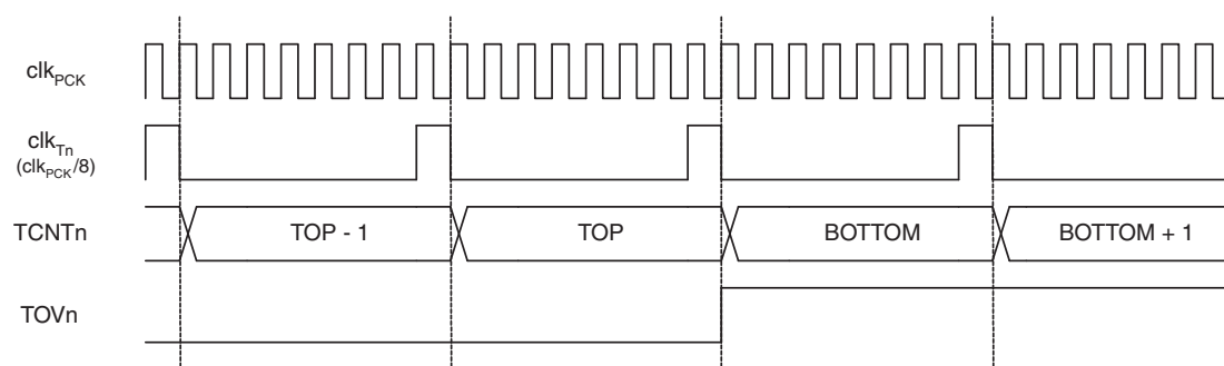
Figure 12-16. Timer/Counter Timing Diagram, with Prescaler ( f_{\text{clkT1}}/8 )
