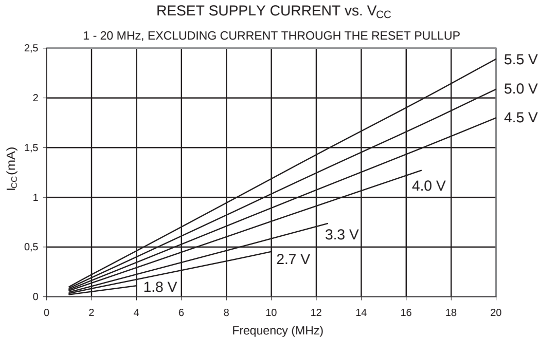
Figure 20-48. Reset Supply Current vs. Frequency (1 - 20 MHz, Excluding Current Through the Reset Pull-up)
