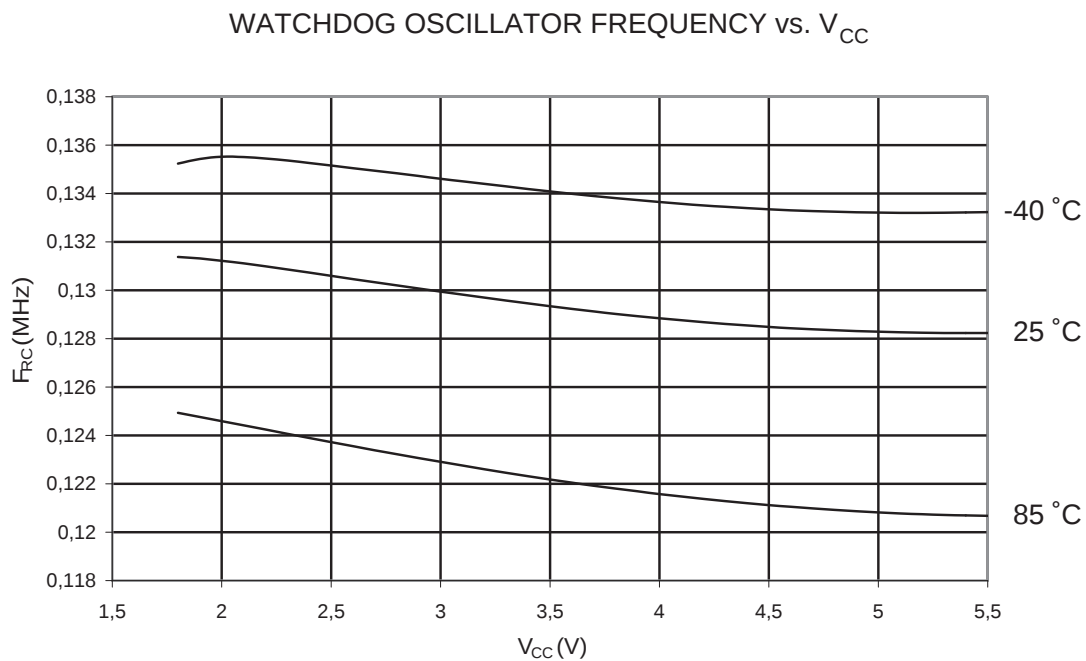
Figure 20-37. Watchdog Oscillator Frequency vs. V_{CC}
