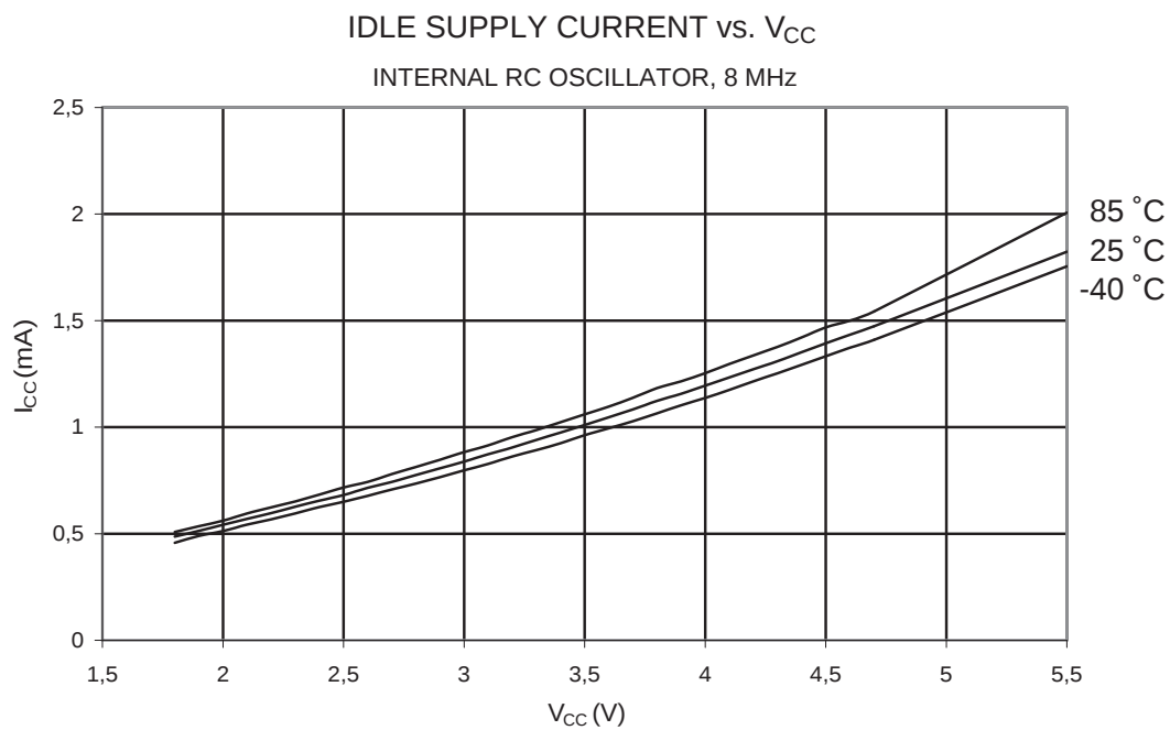
Figure 20-8. Idle Supply Current vs. V_{CC} (Internal RC Oscillator, 8 MHz)
