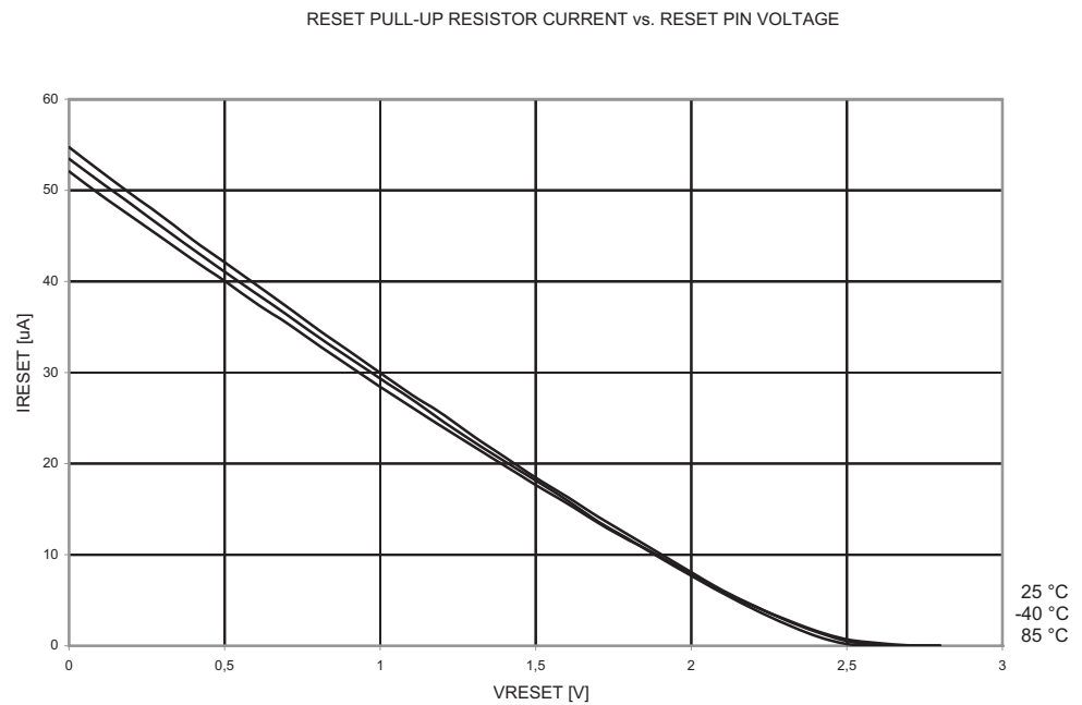
Figure 21-22. Reset Pull-up Resistor Current vs. Reset Pin Voltage ( V_{CC} = 2.7V )
