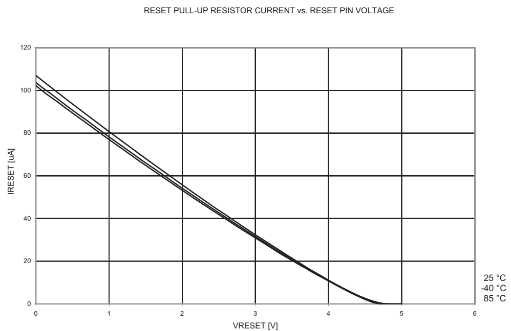
Figure 21-23. Reset Pull-up Resistor Current vs. Reset Pin Voltage ( V_{CC} = 5V )
