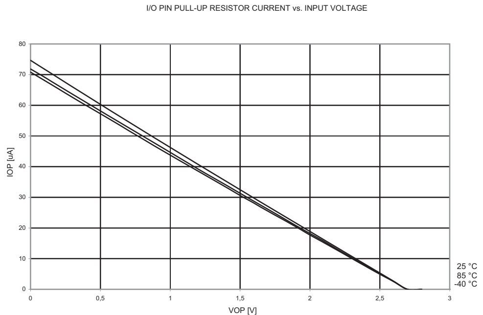
Figure 21-19. I/O Pin Pull-up Resistor Current vs. input Voltage ( V_{CC} = 2.7V )
