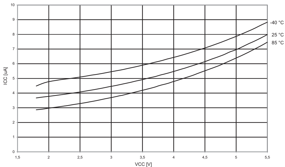
Figure 21-17. Brownout Detector Current vs. V_{CC}
