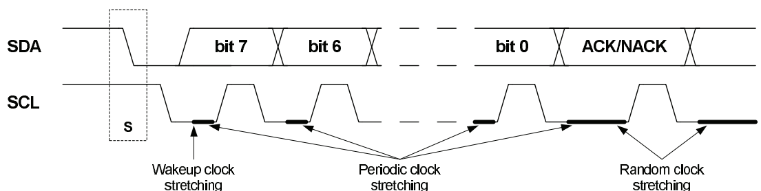
Figure 17-8. Clock Stretching
