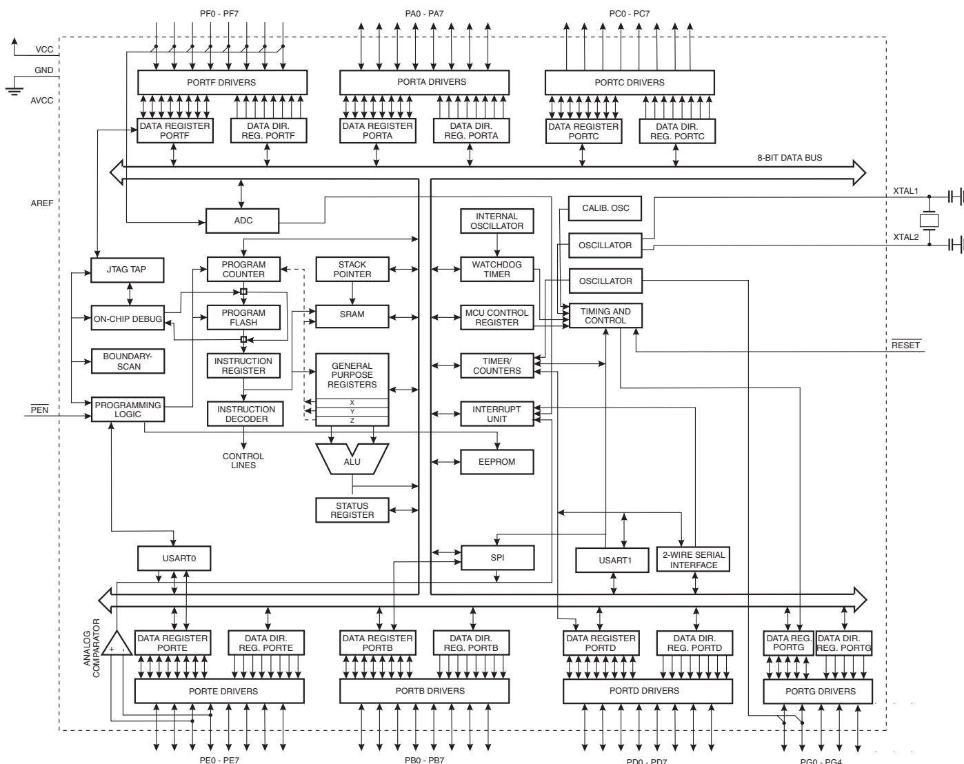
Figure 2-1. Block Diagram
