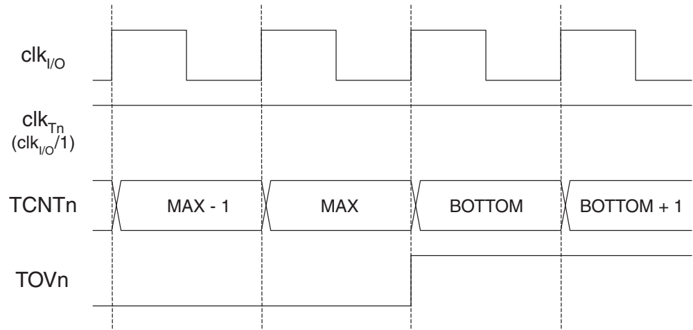
Figure 17-8. Timer/Counter Timing Diagram, no Prescaling
