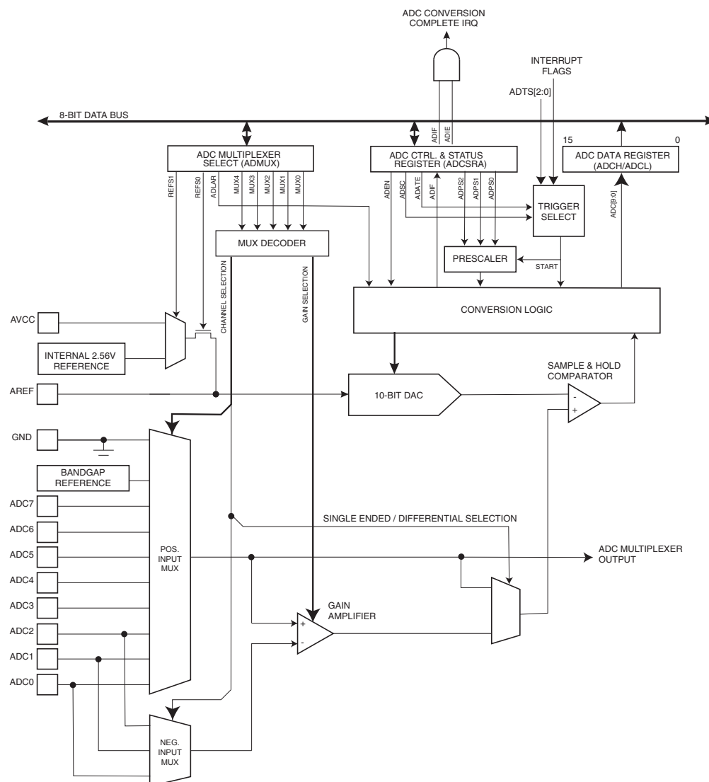
Figure 23-1. Analog to Digital Converter Block Schematic
