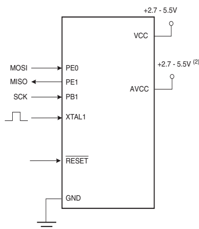
Figure 27-10. SPI Serial Programming and Verify (1)
