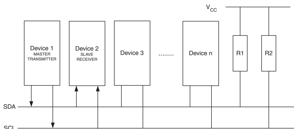
Figure 21-11. Data Transfer in Master Transmitter Mode
