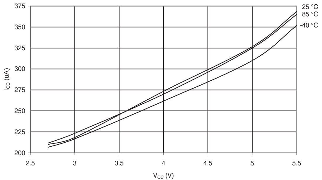
Figure 29-53. ADC Current vs. V_{CC} (ADC CLK = 50 kHz)
