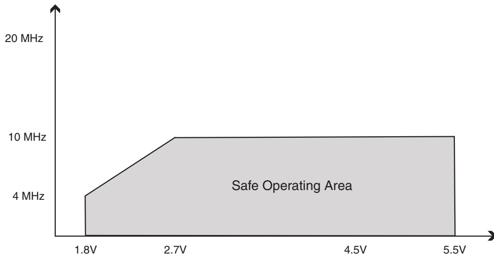
Figure 29-1. Maximum Frequency vs. V_{CC} , ATmega48P/88P/168PV
