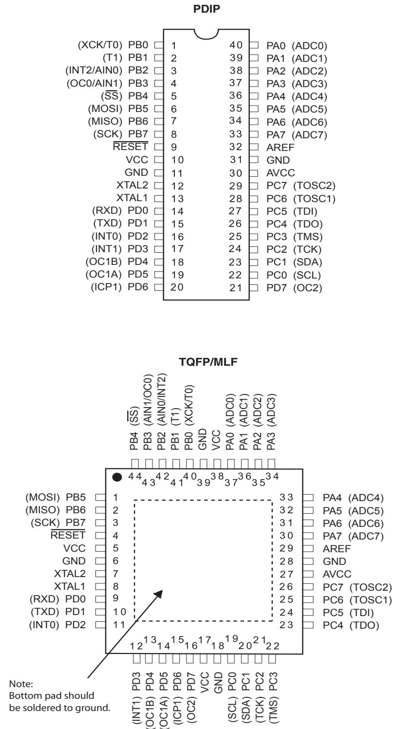
Figure 1-1. Pinout ATmega32A
