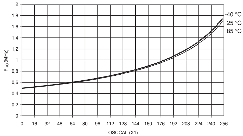
Figure 28-46. Calibrated 1MHz RC Oscillator Frequency vs. Oscal Value
