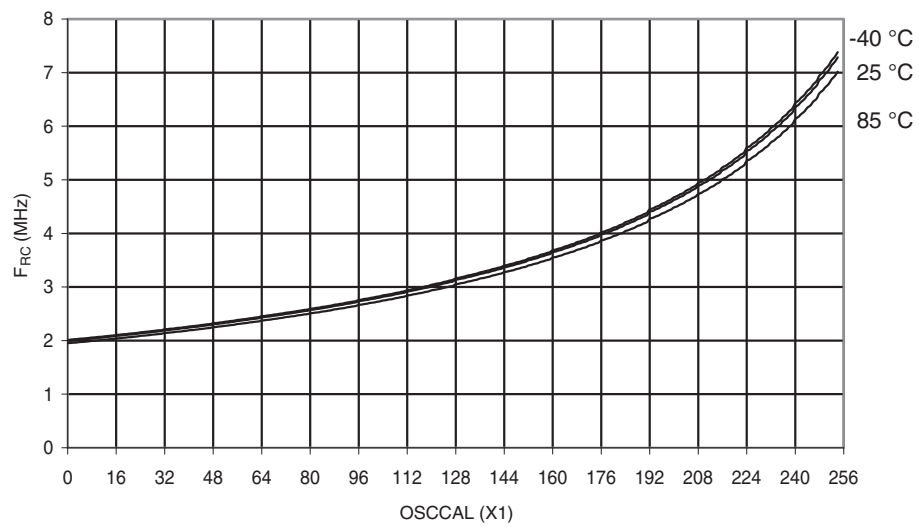
Figure 28-40. Calibrated 4MHz RC Oscillator Frequency vs. Oscal Value
