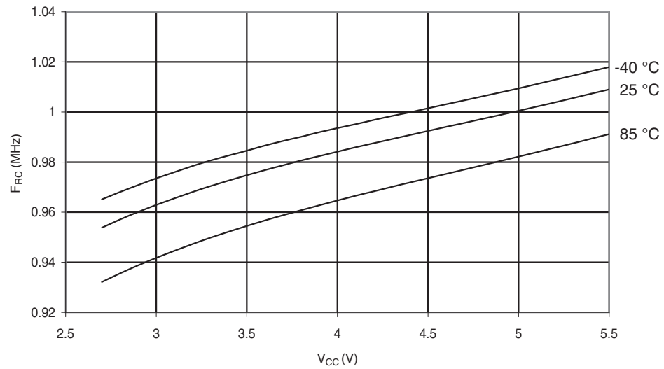
Figure 28-45. Calibrated 1MHz RC Oscillator Frequency vs. V_{CC}
