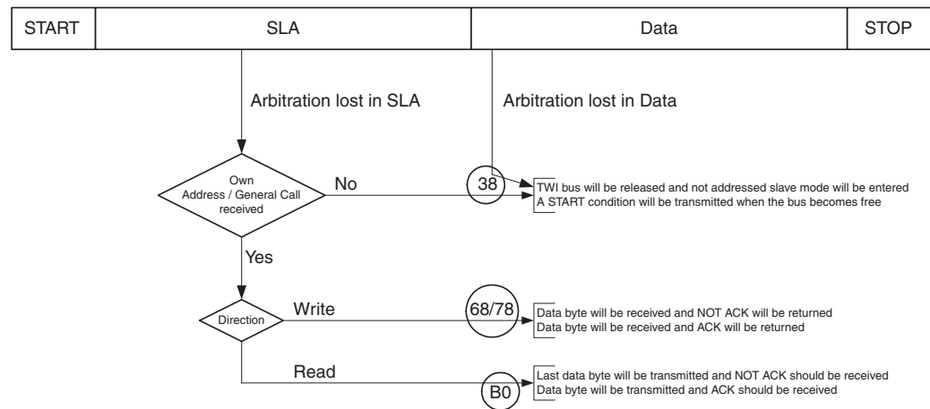
Figure 20-21. Possible Status Codes Caused by Arbitration
