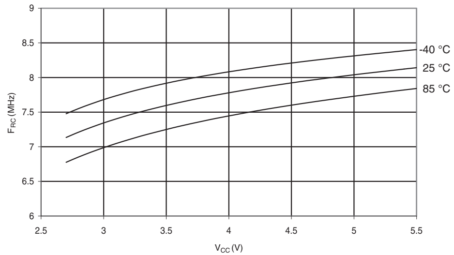
Figure 28-36. Calibrated 8MHz RC Oscillator Frequency vs. V_{CC}
