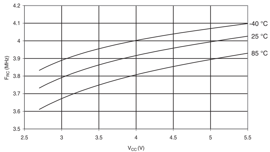
Figure 28-39. Calibrated 4MHz RC Oscillator Frequency vs. V_{CC}
