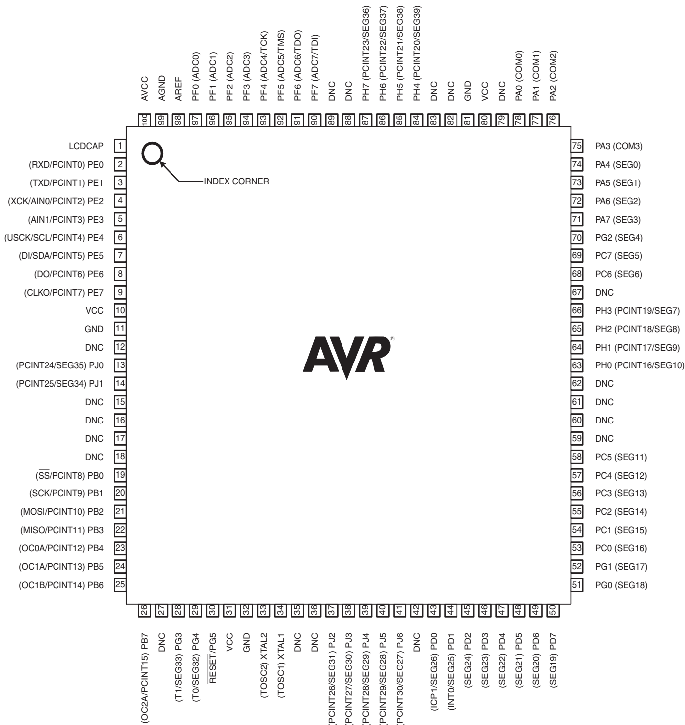
Figure 1-2. TQFP / Pinout ATmega3290P
