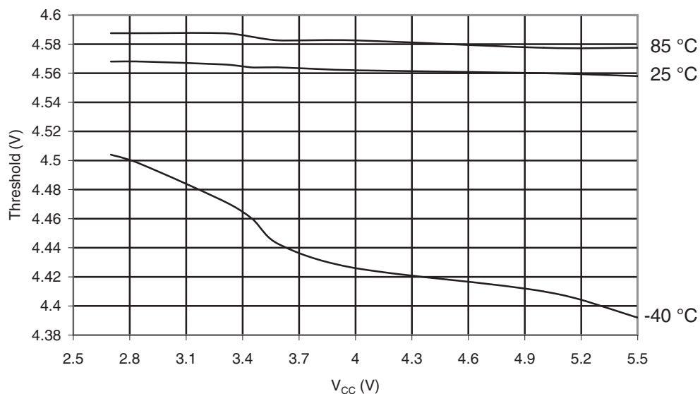
Figure 30-26. Vbus Pin Input Threshold Voltage vs. V_{CC} ( V_{IH} , IO Pin read as '1')
