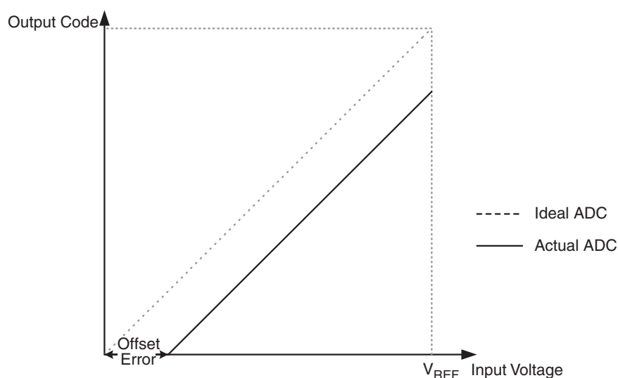
Figure 24-11. Offset Error
