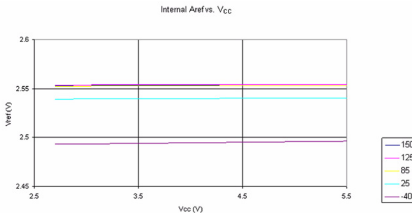
Figure 27-29. AREF Voltage versus V_{CC}
