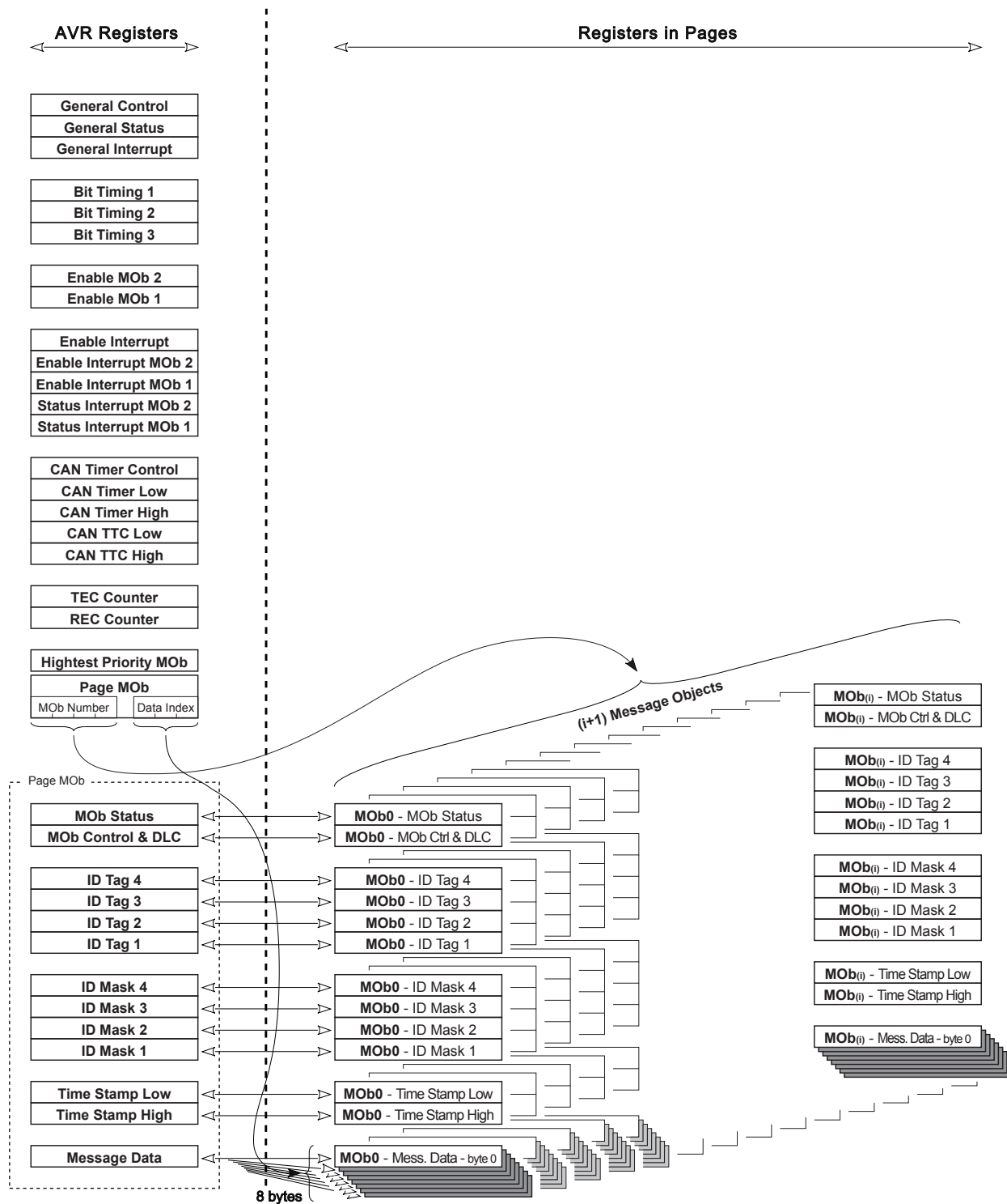
Figure 16-15. Registers Organization
