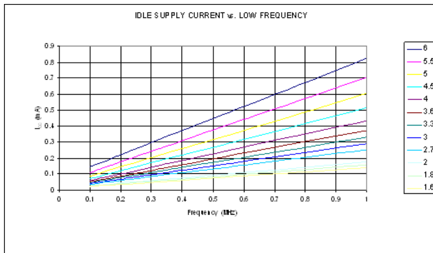
Figure 27-5. Idle Supply Current versus Frequency (0.1 - 1.0 MHz)
