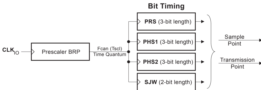
Figure 16-7. Sample and Transmission Point
