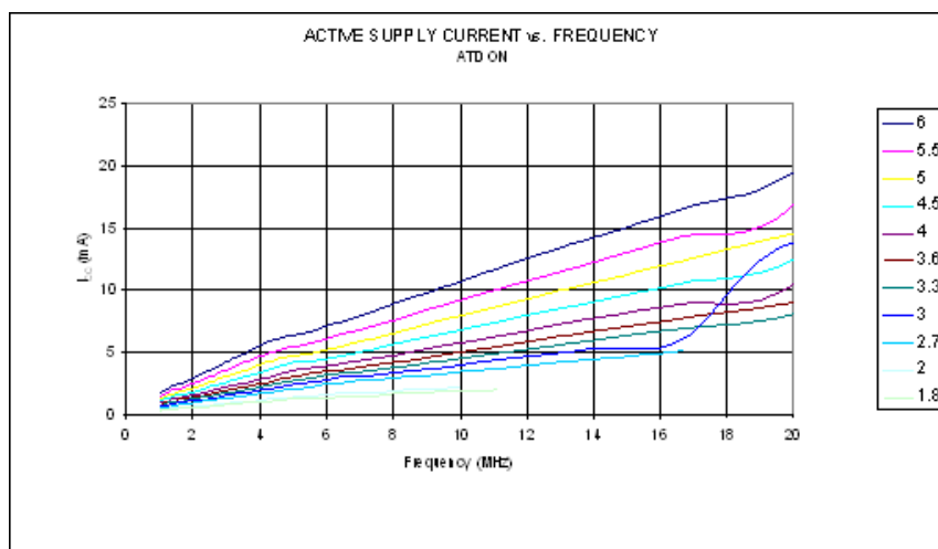
Figure 27-2. Active Supply Current versus Frequency (1 - 24 MHz)
