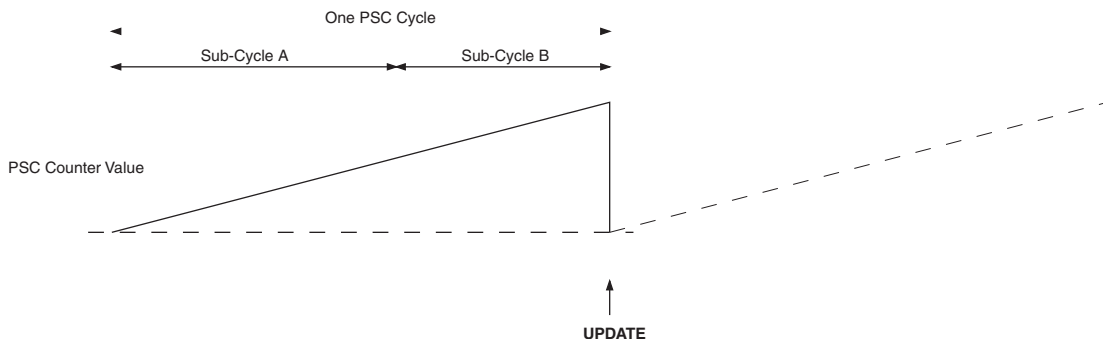
Figure 14-2. Cycle Presentation in One Ramp Mode
