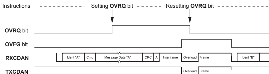
Figure 16-9. Overload Frame
