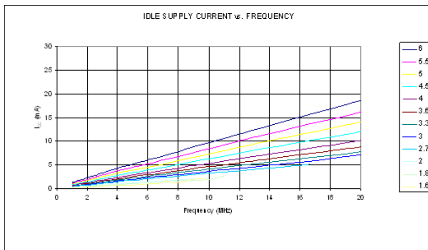
Figure 27-6. Idle Supply Current versus Frequency (1 - 24 MHz)
