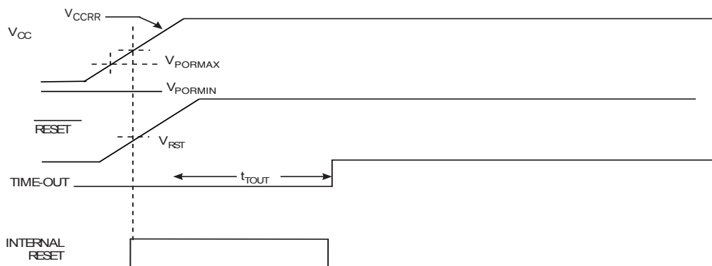
Figure 7-2. MCU Start-up, \overline{\text{RESET}} Tied to V_{CC}
