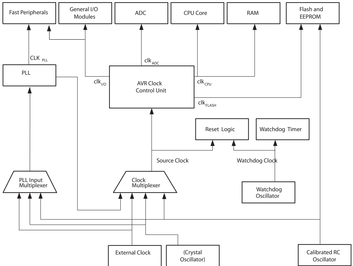
Figure 5-1. Clock Distribution
