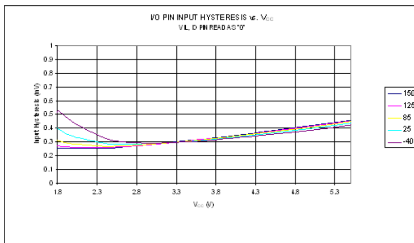
Figure 27-21. I/O Pin Input Hysteresis Voltage versus V_{CC}
