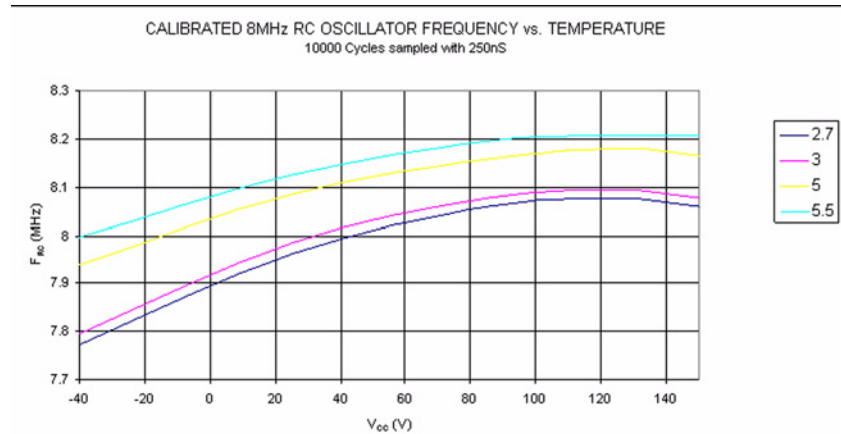
Figure 27-32. Calibrated 8 MHz RC Oscillator Frequency versus Temperature
