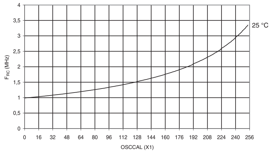
Figure 28-45. Calibrated 2MHz RC Oscillator Frequency vs. OSCCAL Value
