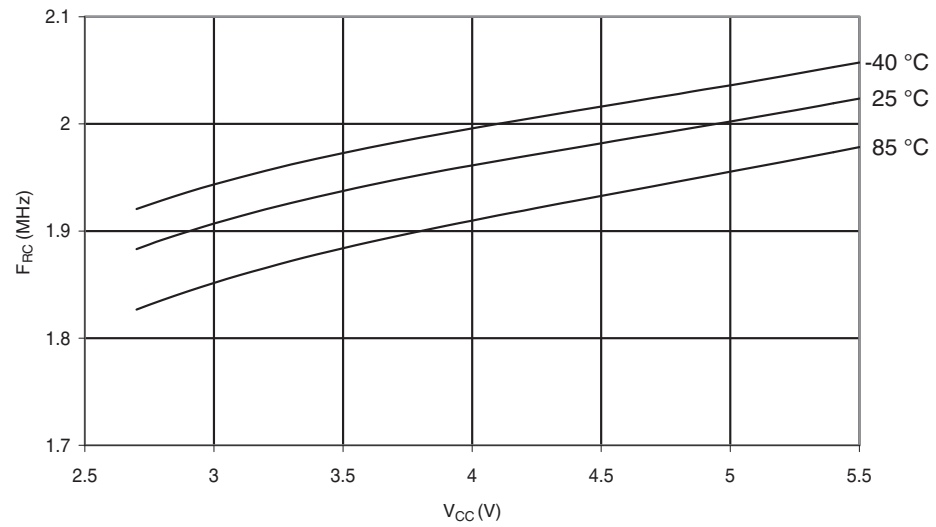
Figure 28-44. Calibrated 2MHz RC Oscillator Frequency vs. V_{CC}
