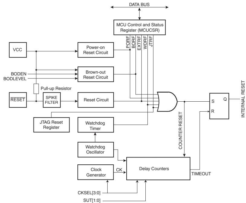
Figure 10-1. Reset Logic
