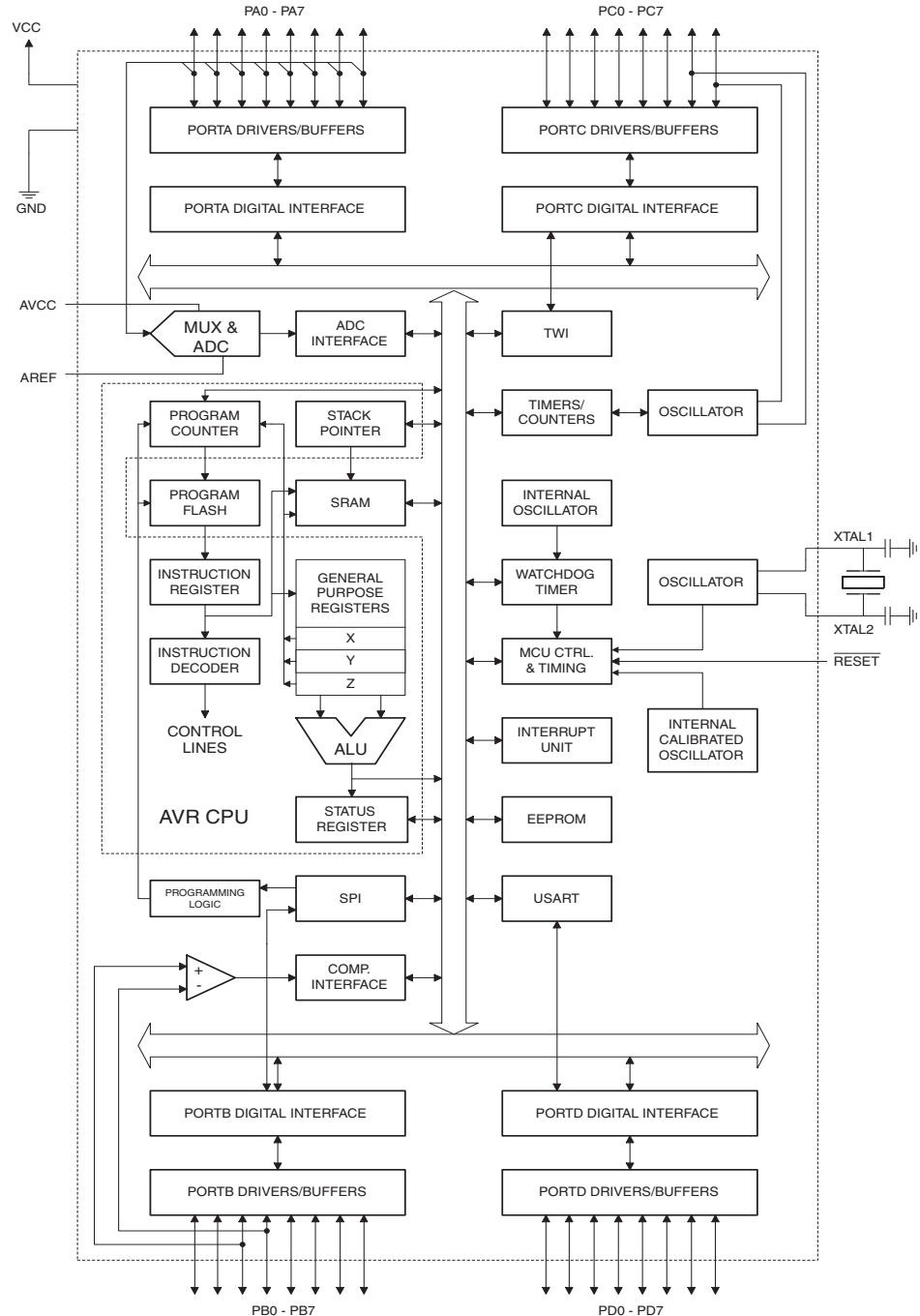
Figure 2-1. Block Diagram
