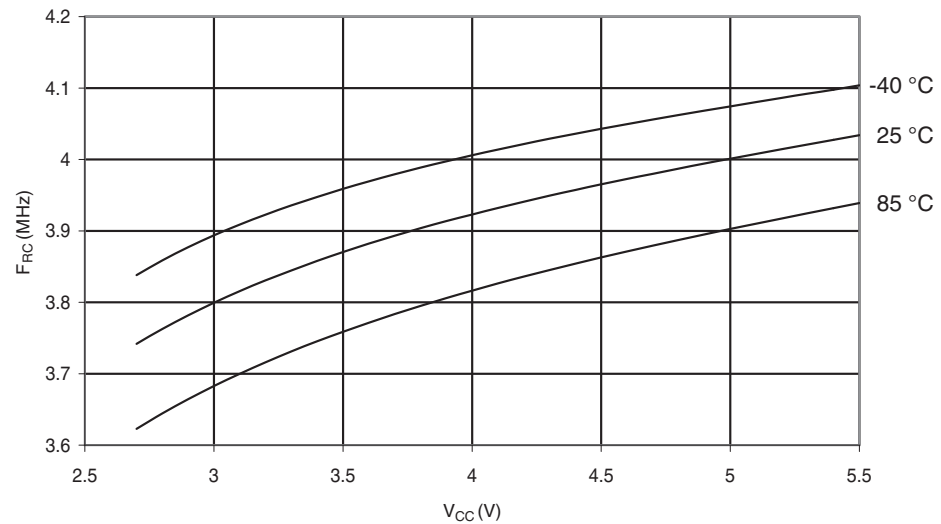
Figure 28-41. Calibrated 4MHz RC Oscillator Frequency vs. V_{CC}
