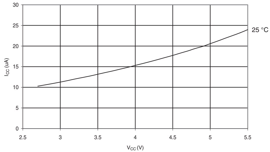
Figure 28-14. Idle Supply Current vs. V_{CC} (32kHz External Oscillator)
