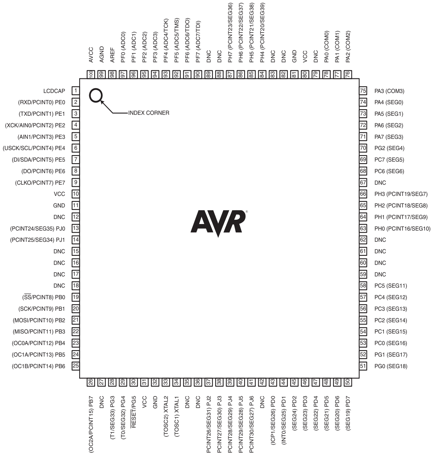
Figure 1-2. Pinout ATmega3290P/6490P
