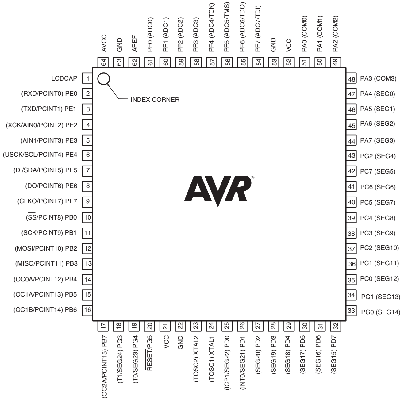
Figure 1-1. Pinout ATmega169PA/329P/649P
