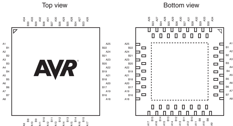
Figure 1-3. 64MC (DRQFN) Pinout ATmega169PA
