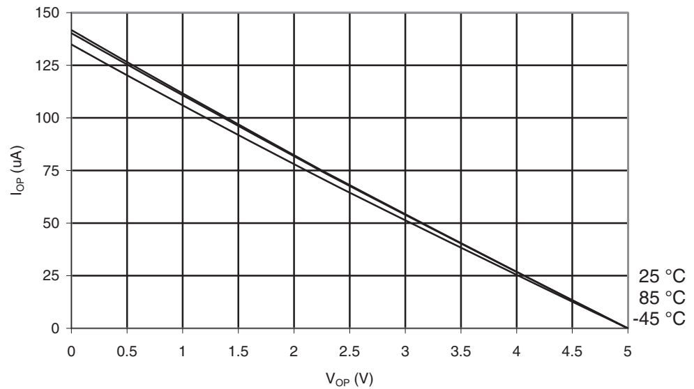
Figure 29-16. ATmega169PA: I/O Pin Pull-up Resistor Current vs. Input Voltage ( V_{CC} = 5V )
