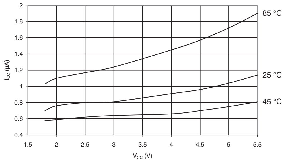
Figure 29-13. ATmega169PA: Power-save Supply Current vs. V_{CC} (Watchdog Timer Disabled)
