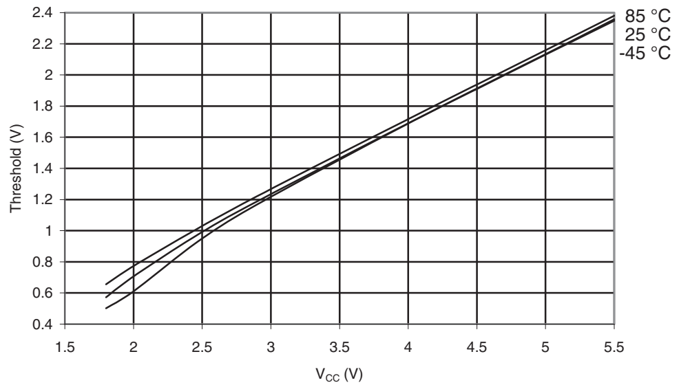
Figure 29-270. ATmega6490P: I/O Pin Input Threshold Voltage vs. V_{CC} ( V_{IL} , IO Pin Read as "0")
