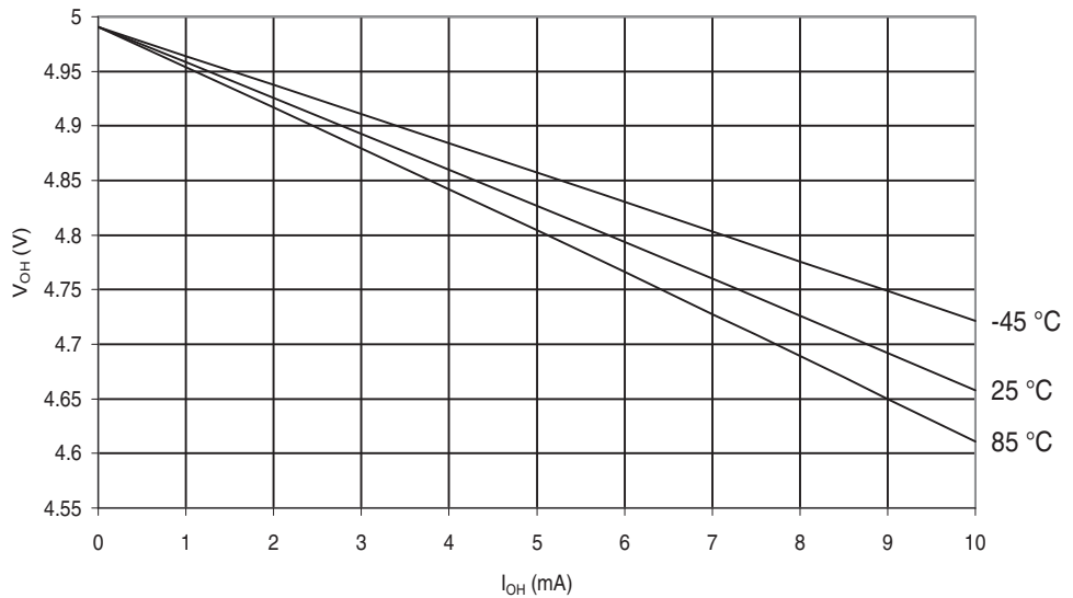
Figure 29-265. ATmega6490P : I/O Pin Output Voltage vs. Source Current, Port A,C,D,E,F,G ( V_{CC} = 5V )
