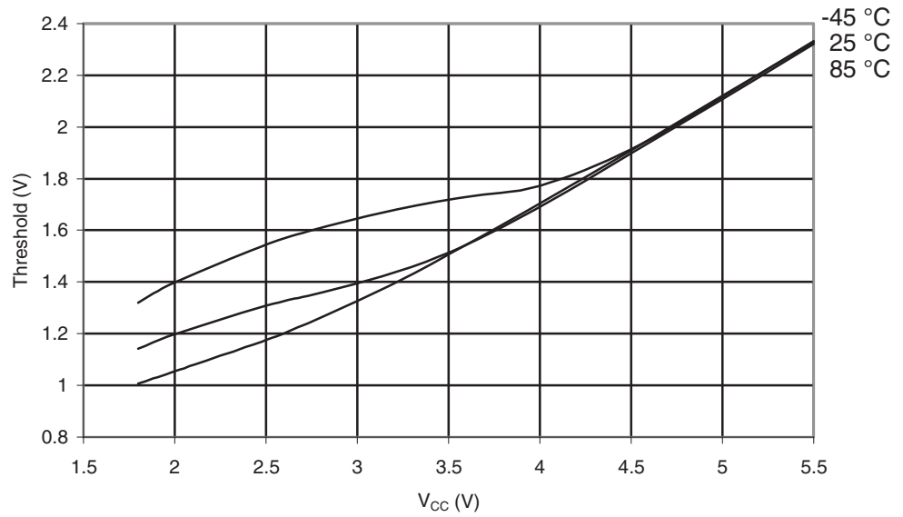
Figure 29-215. ATmega649P: Reset Input Threshold Voltage vs. V_{CC} ( V_{IH} , IO Pin Read as "1")
