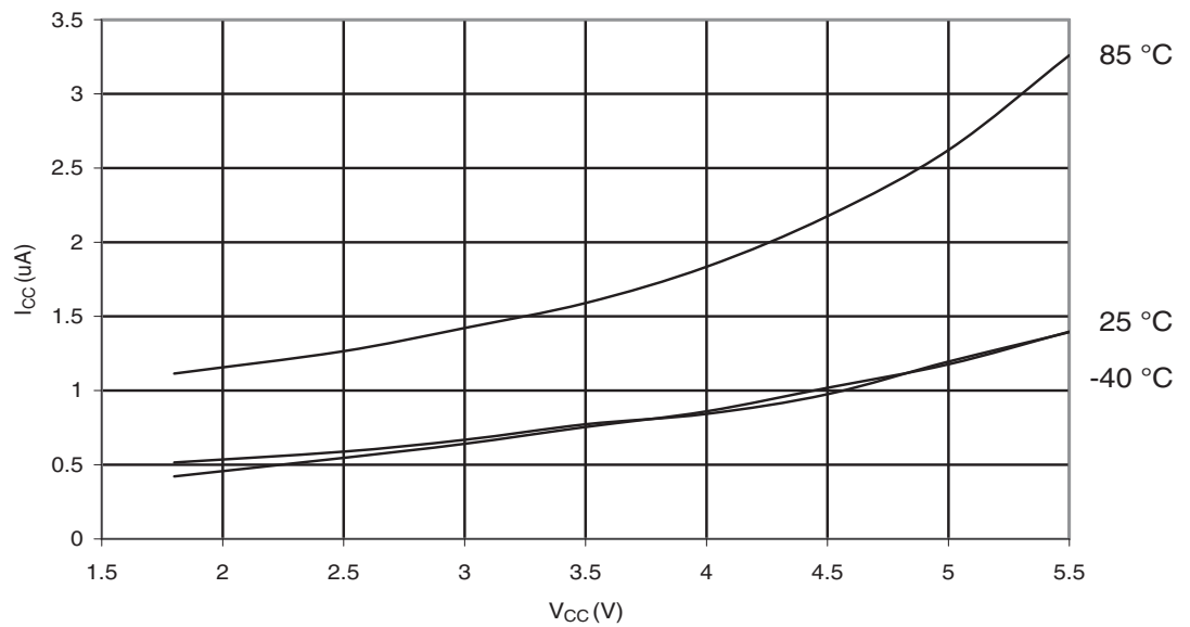
Figure 29-246. ATmega6490P: Power-save Supply Current vs. V_{CC} (Watchdog Timer Disabled)
