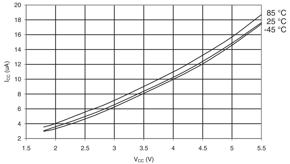
Figure 29-188. ATmega649P: Power-down Supply Current vs. V_{CC} (Watchdog Timer Enabled)
