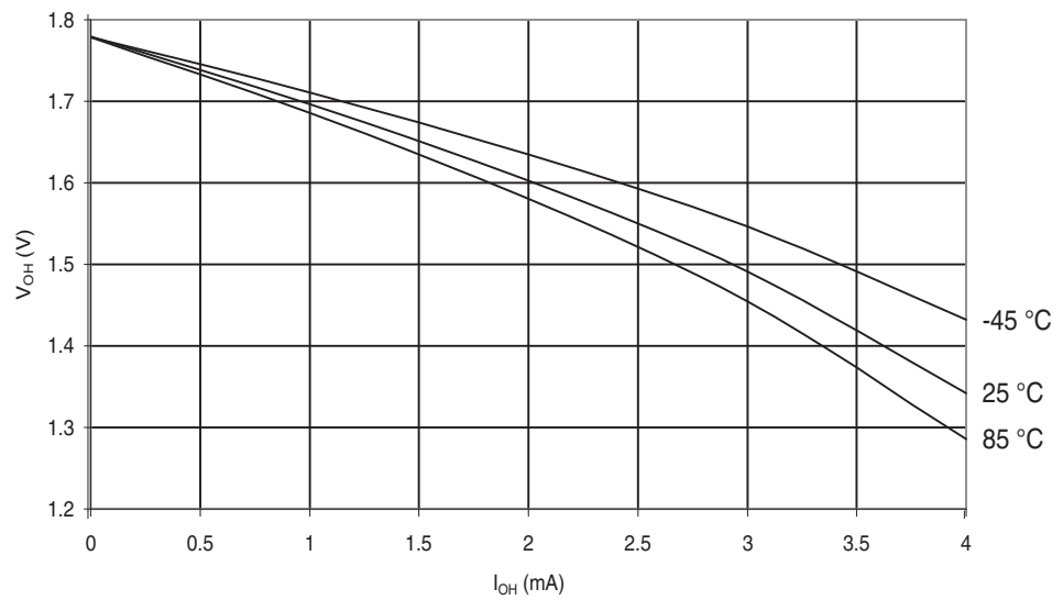
Figure 29-263. ATmega6490P: I/O Pin Output Voltage vs. Source Current, Port A,C,D,E,F,G ( V_{CC}=1.8V )
