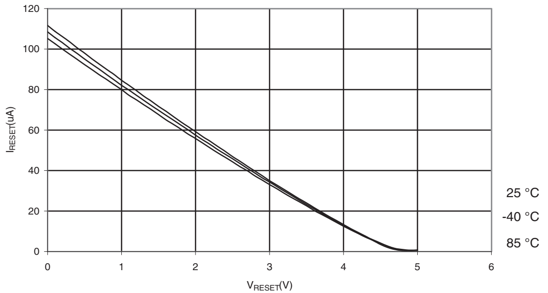
Figure 29-138. ATmega3290P: Reset Pull-up Resistor Current vs. Reset Pin Voltage ( V_{CC} = 5V )
