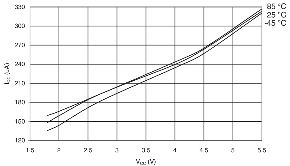
Figure 29-281. ATmega6490P: Active Supply Current with ADC at 50kHz vs. V_{CC}
