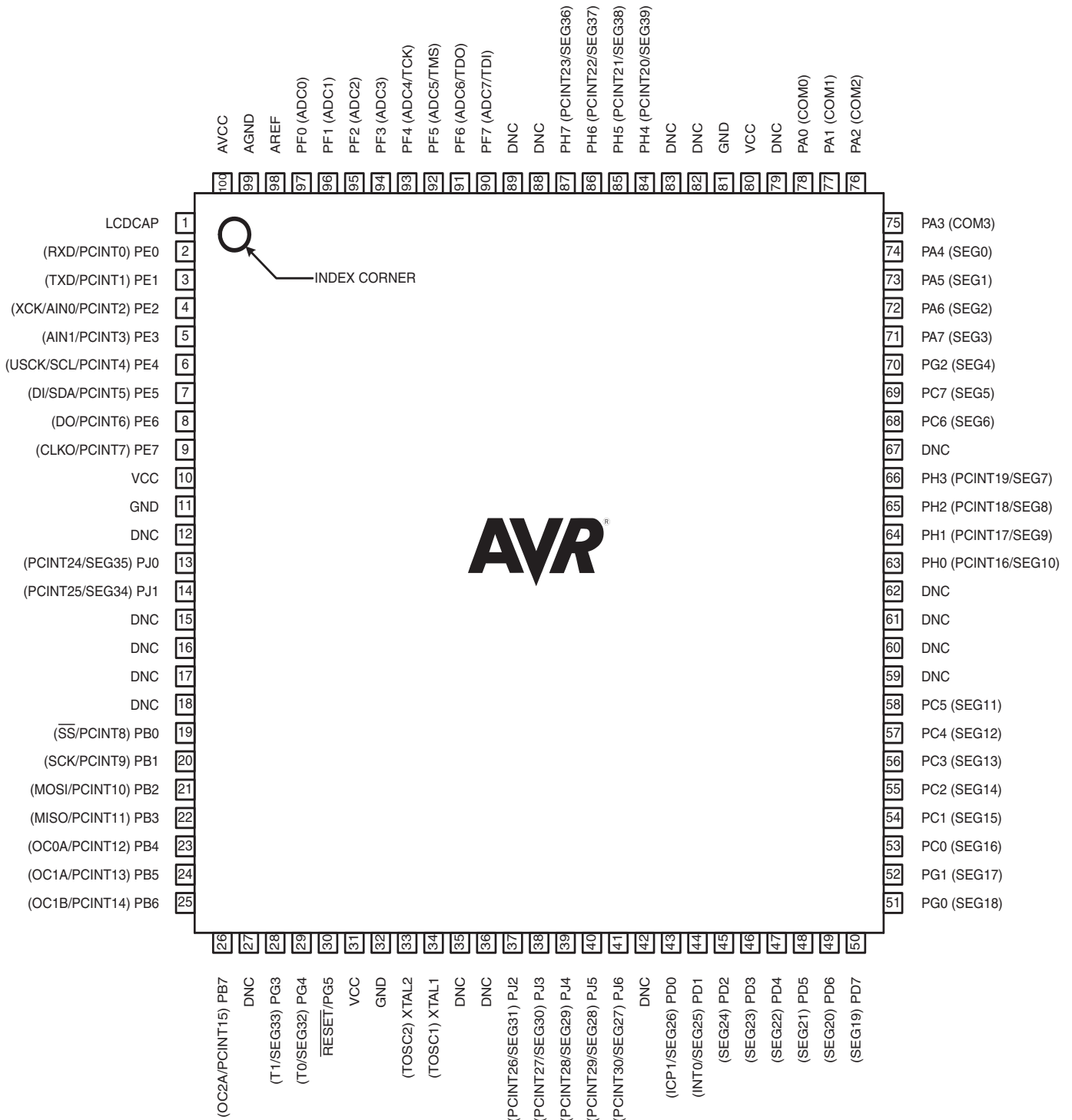
Figure 1-2. TQFP / Pinout ATmega3290P/6490P
