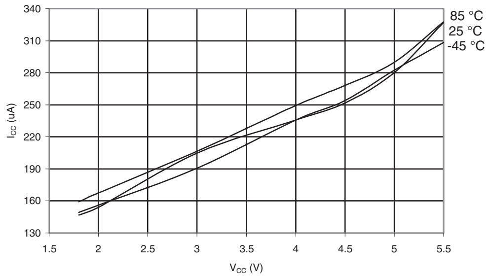
Figure 29-227. ATmega649P: AREF External Reference Current vs. V CC
