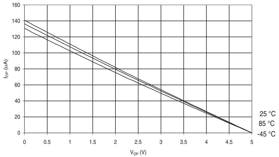
Figure 29-250. ATmega6490P: I/O Pin Pull-up Resistor Current vs. Input Voltage ( V_{CC} = 5V )
