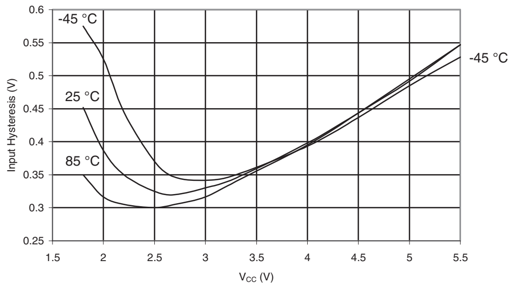
Figure 29-268. ATmega6490P: I/O Pin Input Hysteresis vs. V_{CC}
