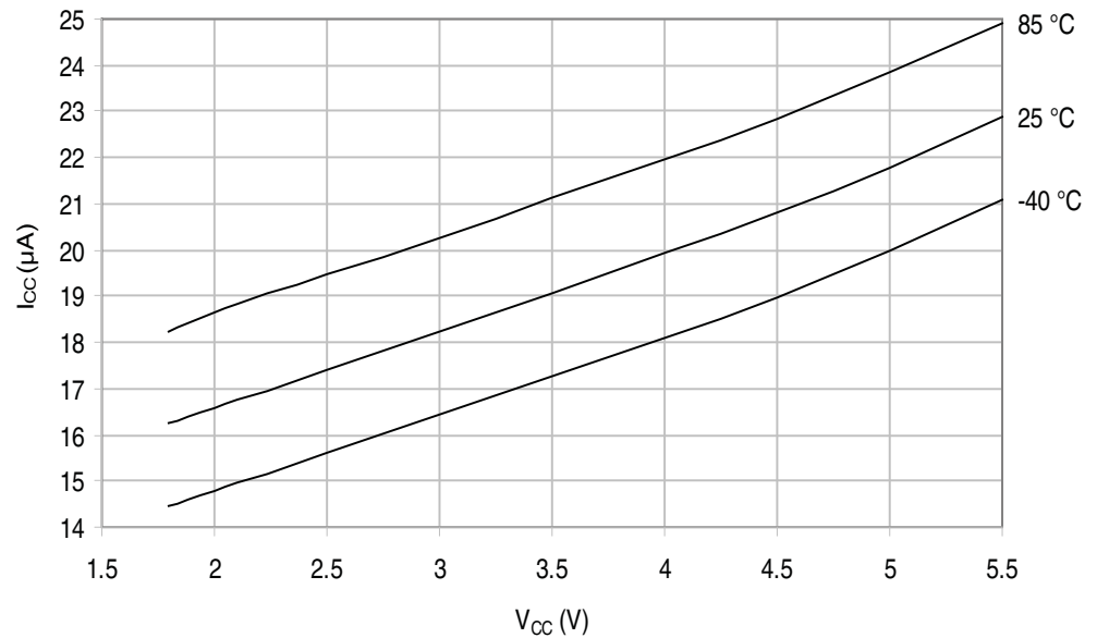
Figure 29-165. ATmega3290P: Brownout Detector Current vs. V_{CC}
