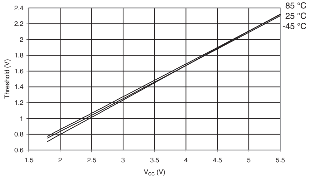
Figure 29-273. ATmega6490P: Reset Input Threshold Voltage vs. V_{CC} ( V_{IL} , IO Pin Read as "0")
