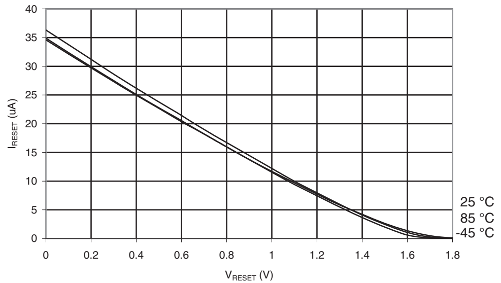
Figure 29-21. ATmega169PA: Reset Pull-up Resistor Current vs. Reset Pin Voltage ( V_{CC}=1.8V )
