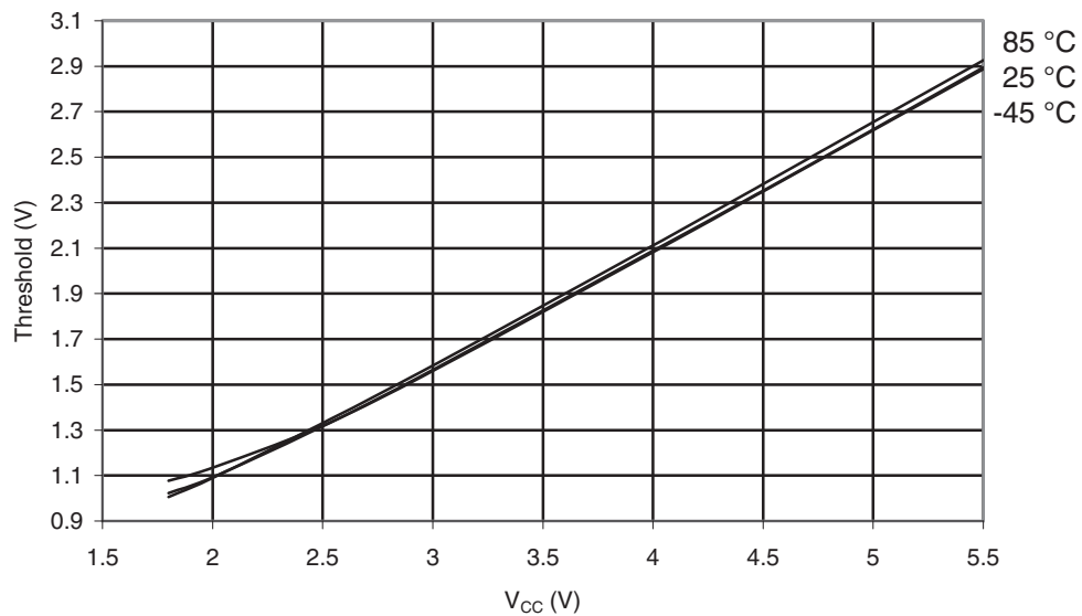
Figure 29-212. ATmega649P: I/O Pin Input Threshold Voltage vs. V_{CC} , ( V_{IH} , IO Pin Read as "1")
