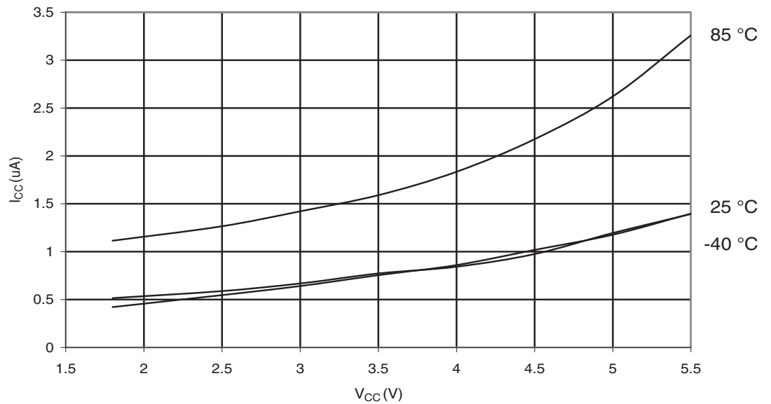
Figure 29-74. ATmega329P: Power-save Supply Current vs. V_{CC} (Watchdog Timer Disabled)
