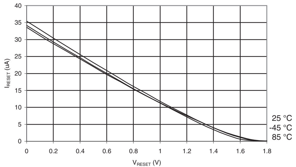
Figure 29-251. ATmega6490P: Reset Pull-up Resistor Current vs. Reset Pin Voltage ( V_{CC} = 1.8V )
