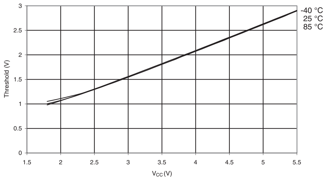
Figure 29-97. ATmega329P: I/O Pin Input Threshold Voltage vs. V_{CC} , Port A,C,D,E,F,G,H,J ( V_{IH} , IO Pin Read as "1")
