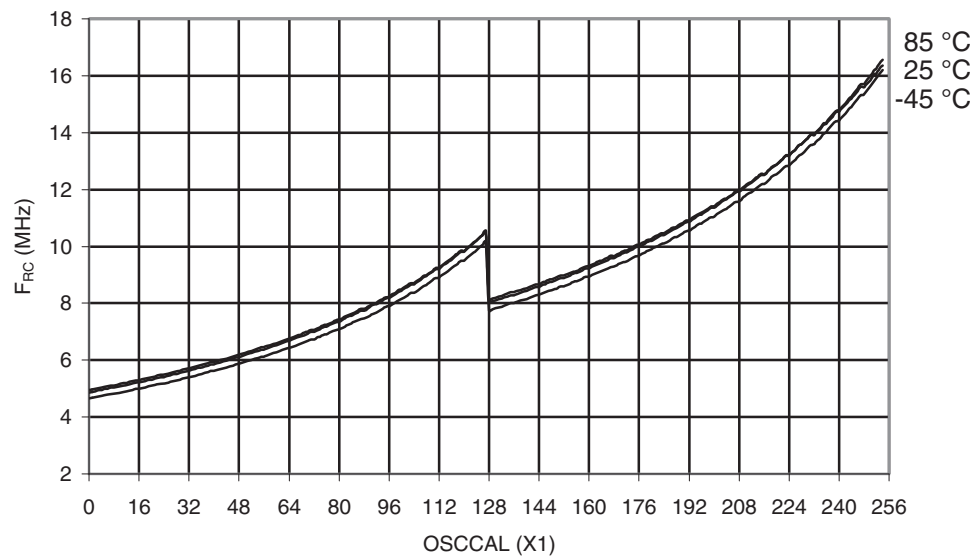
Figure 29-279. ATmega6490P: Calibrated 8MHz RC Oscillator Frequency vs. OSCAL Value
