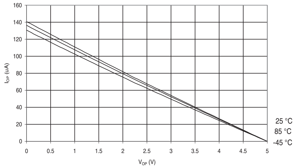
Figure 29-193. ATmega649P: I/O Pin Pull-up Resistor Current vs. Input Voltage ( V_{CC} = 5V )
