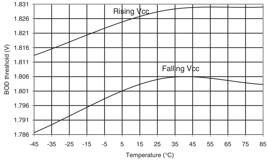
Figure 29-42. ATmega169PA: BOD Thresholds vs. Temperature (BOD Level is 1.8V)
