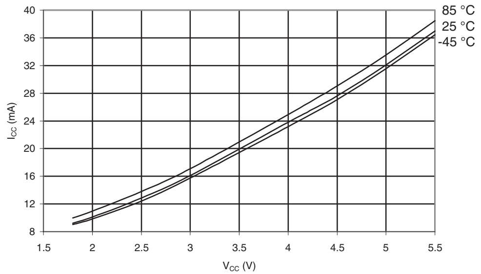
Figure 29-181. ATmega649P: Active Supply Current vs. V_{CC} (32kHz Watch Crystal)
