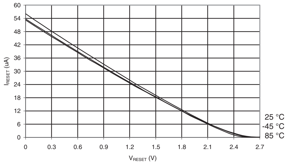
Figure 29-252. ATmega6490P: Reset Pull-up Resistor Current vs. Reset Pin Voltage ( V_{CC} = 2.7V )
