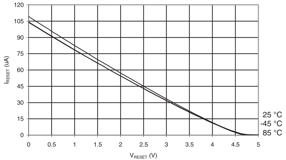
Figure 29-196. ATmega649P: Reset Pull-up Resistor Current vs. Reset Pin Voltage ( V_{CC} = 5V )
