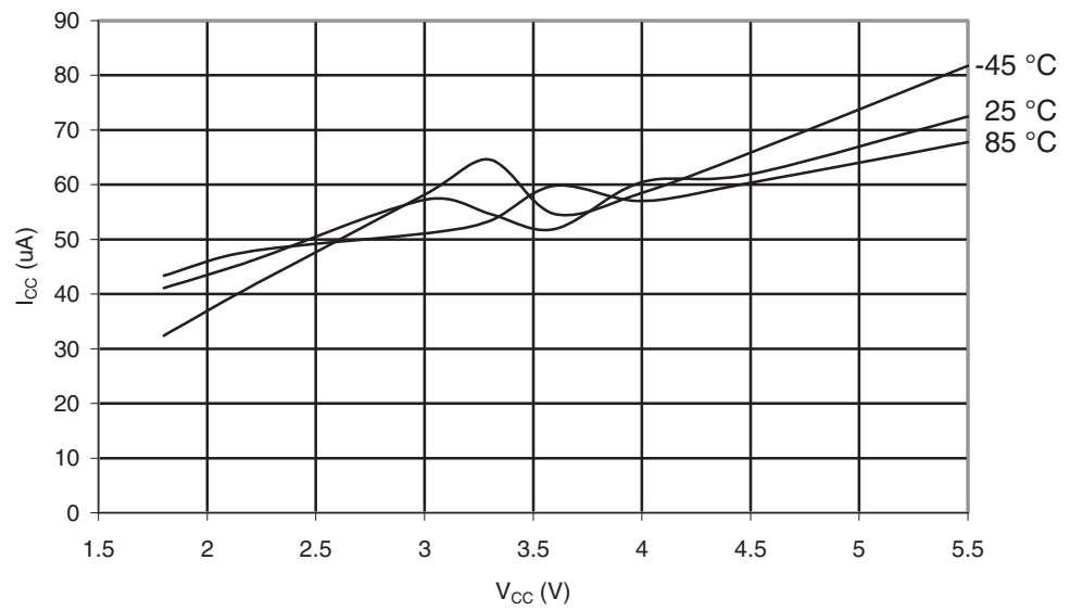
Figure 29-58. ATmega169PA: Analog Comparator Current vs. V_{CC}
