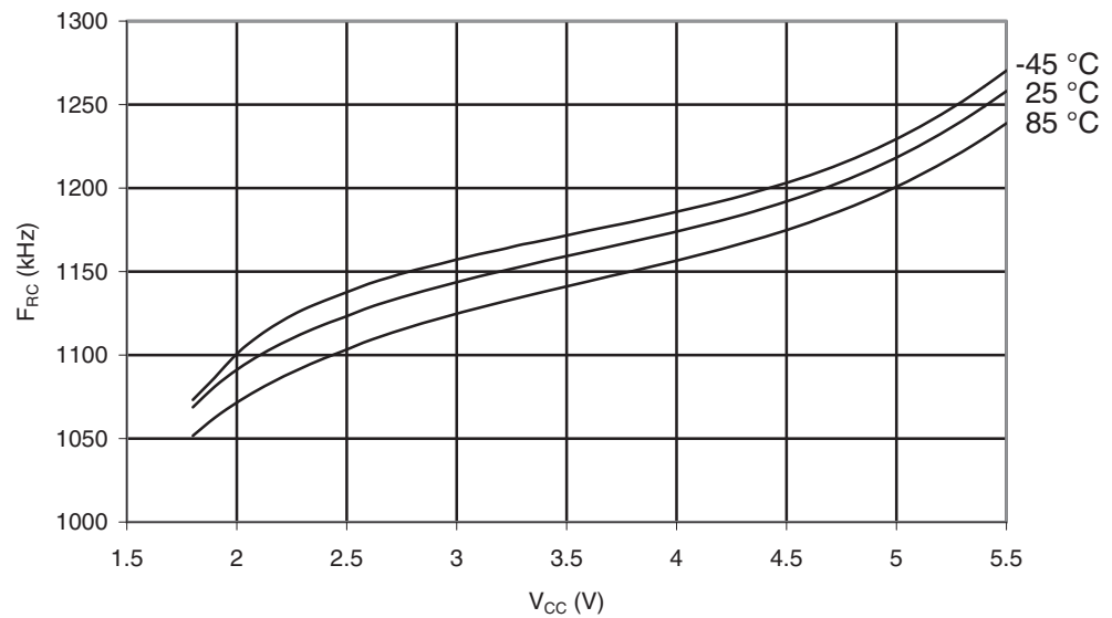
Figure 29-47. ATmega169PA: Watchdog Oscillator Frequency vs. V_{CC}
