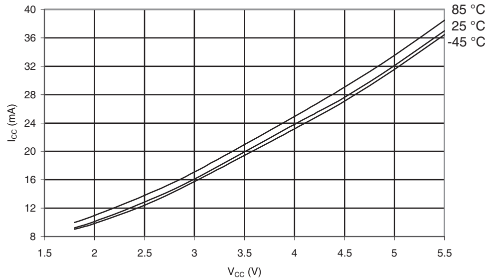
Figure 29-238. ATmega6490P: Active Supply Current vs. V_{CC} (32kHz Watch Crystal)
