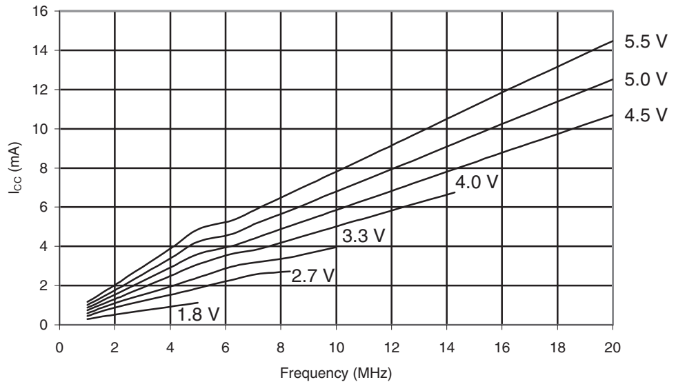
Figure 29-235. ATmega6490P: Active Supply Current vs. Frequency (1 - 20MHz)
