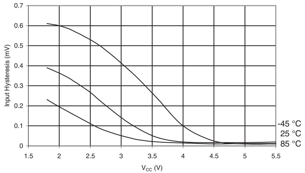
Figure 29-274. ATmega6490P: Reset Pin Input Hysteresis vs. V_{CC}
