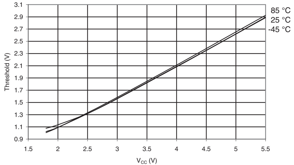
Figure 29-266. ATmega6490P: I/O Pin Input Threshold Voltage vs. V_{CC} , ( V_{IH} , IO Pin Read as "1")
