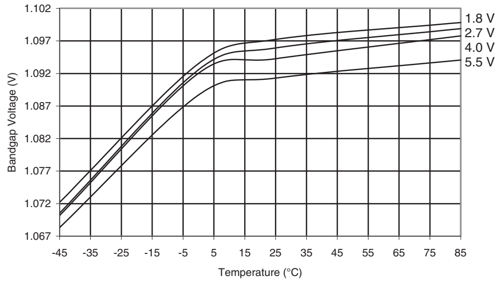
Figure 29-44. ATmega169PA: Bandgap Voltage vs. Temperature
