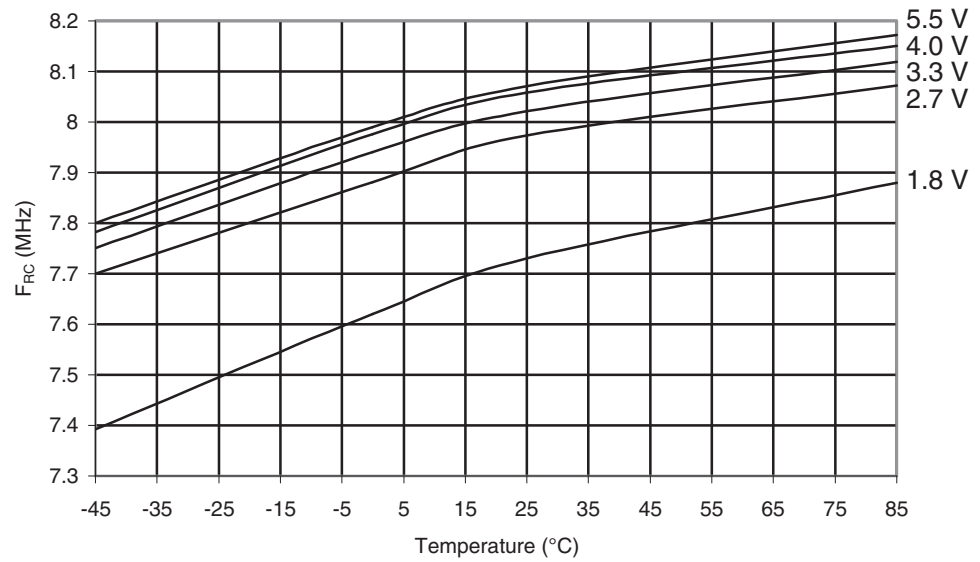
Figure 29-221. ATmega649P: Calibrated 8MHz RC Oscillator Frequency vs. Temperature
