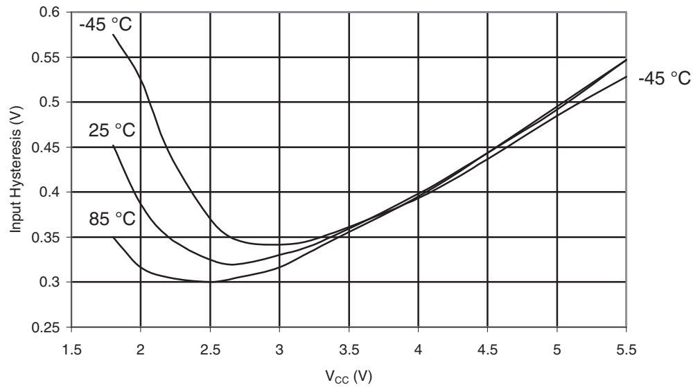
Figure 29-271. ATmega6490P: I/O Pin Hysteresis vs. V_{CC} , Port A,C,D,E,F,G,H,J
