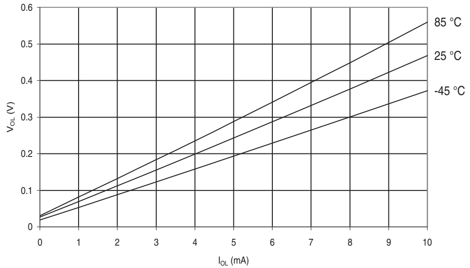
Figure 29-202. ATmega649P: I/O Pin Output Voltage vs. Sink Current, Port A,C,D,E,F,G ( V_{CC}=5V )
