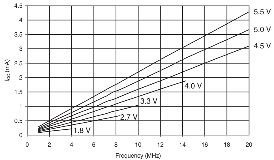
Figure 29-240. ATmega6490P: Idle Supply Current vs. Frequency (1 - 20MHz)
