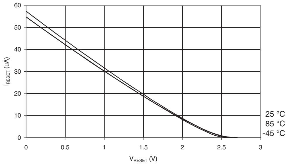
Figure 29-20. ATmega169PA: Reset Pull-up Resistor Current vs. Reset Pin Voltage ( V_{CC}=2.7V )
