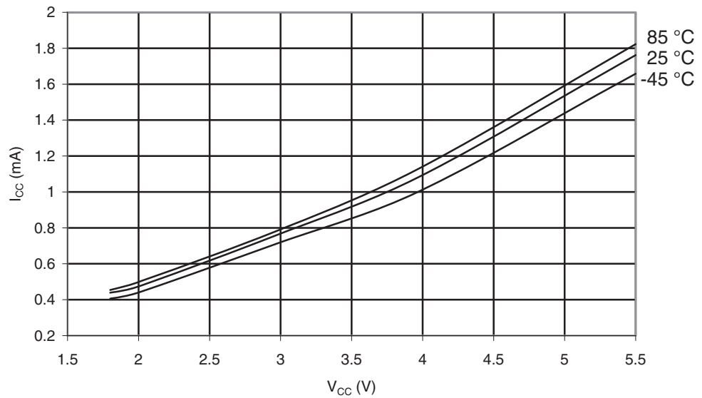
Figure 29-241. ATmega6490P: Idle Supply Current vs. V_{CC} (Internal RC Oscillator, 8MHz)
