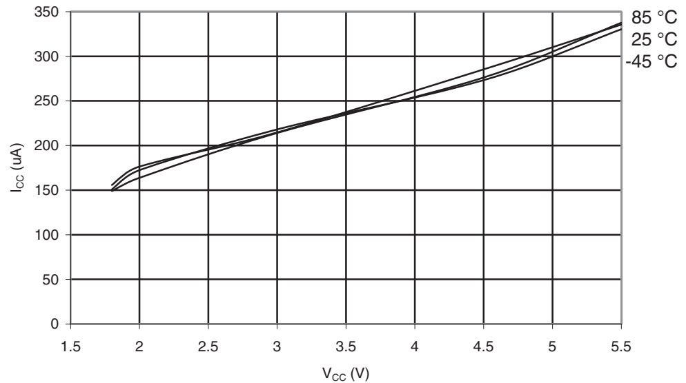
Figure 29-55. ATmega169PA: Active Supply Current with ADC at 1MHz vs. V_{CC}
