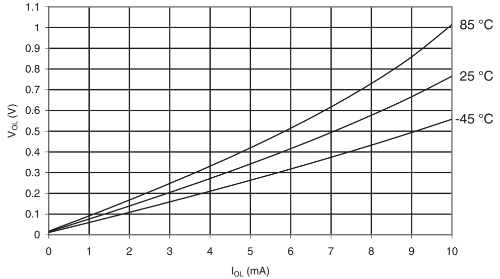
Figure 29-29. ATmega169PA: I/O Pin Output Voltage vs. Sink Current, Ports A, C, D, E, F, G ( V_{CC} = 2.7V )
