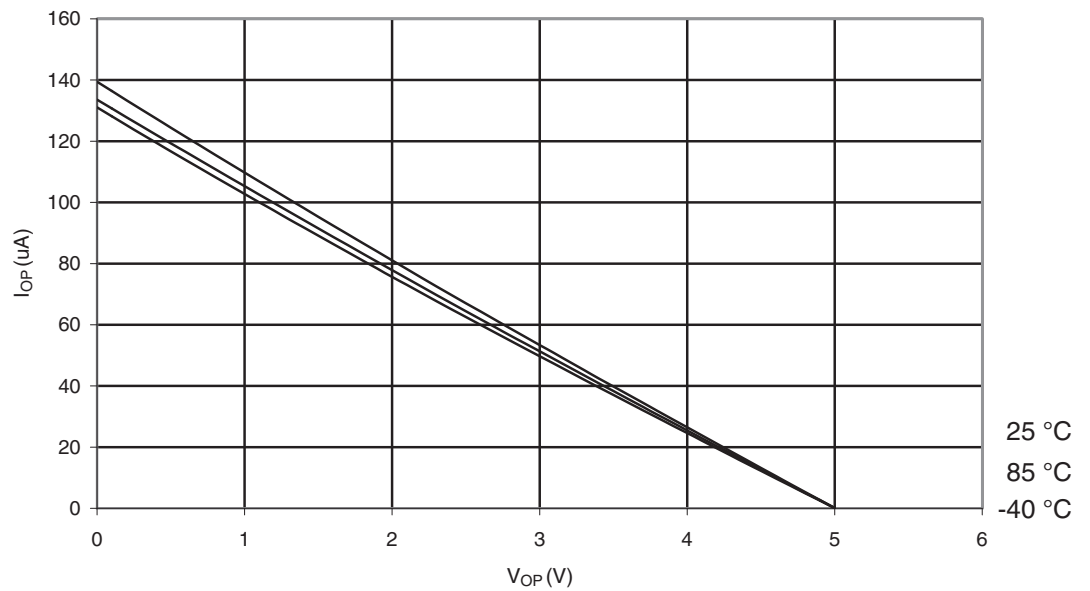
Figure 29-78. ATmega329P: I/O Pin Pull-up Resistor Current vs. Input Voltage ( V_{CC} = 5V )
