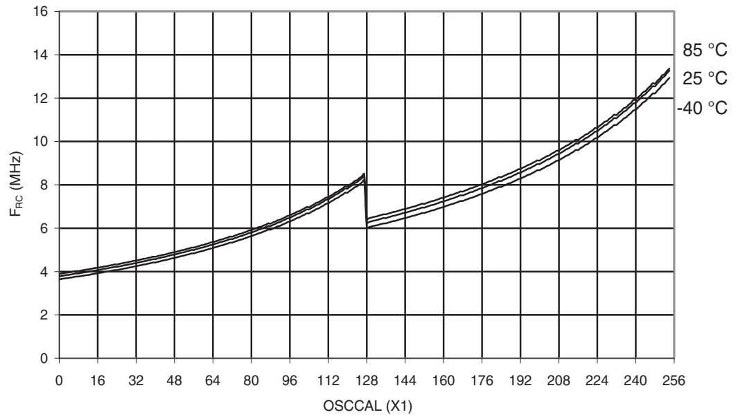
Figure 29-107. ATmega329P: Calibrated 8MHz RC Oscillator Frequency vs. Oscscal Value
