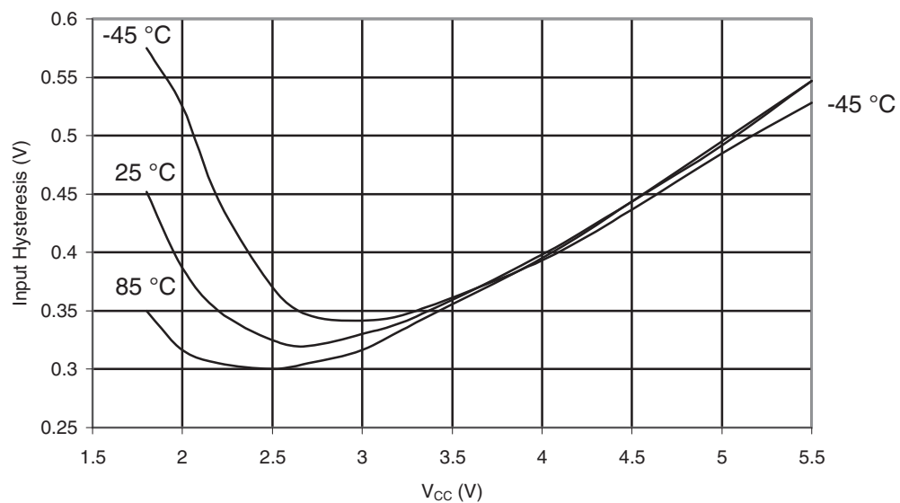
Figure 29-211. ATmega649P: I/O Pin Input Hysteresis vs. V_{CC}
