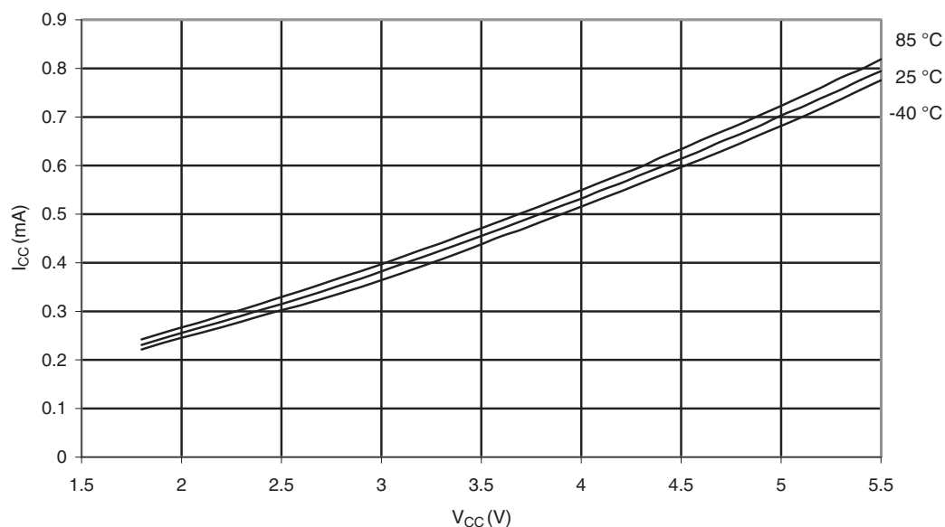
Figure 29-71. ATmega329P: Idle Supply Current vs. V_{CC} (Internal RC Oscillator, 1MHz)
