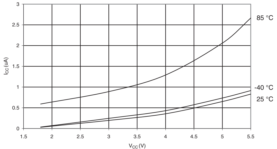
Figure 29-72. ATmega329P: Power-down Supply Current vs. V_{CC} (Watchdog Timer Disabled)
