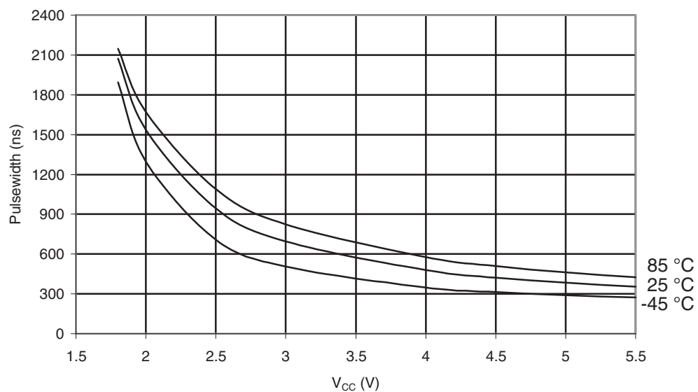
Figure 29-233. ATmega649P: Minimum Reset Pulse Width vs. V_{CC}
