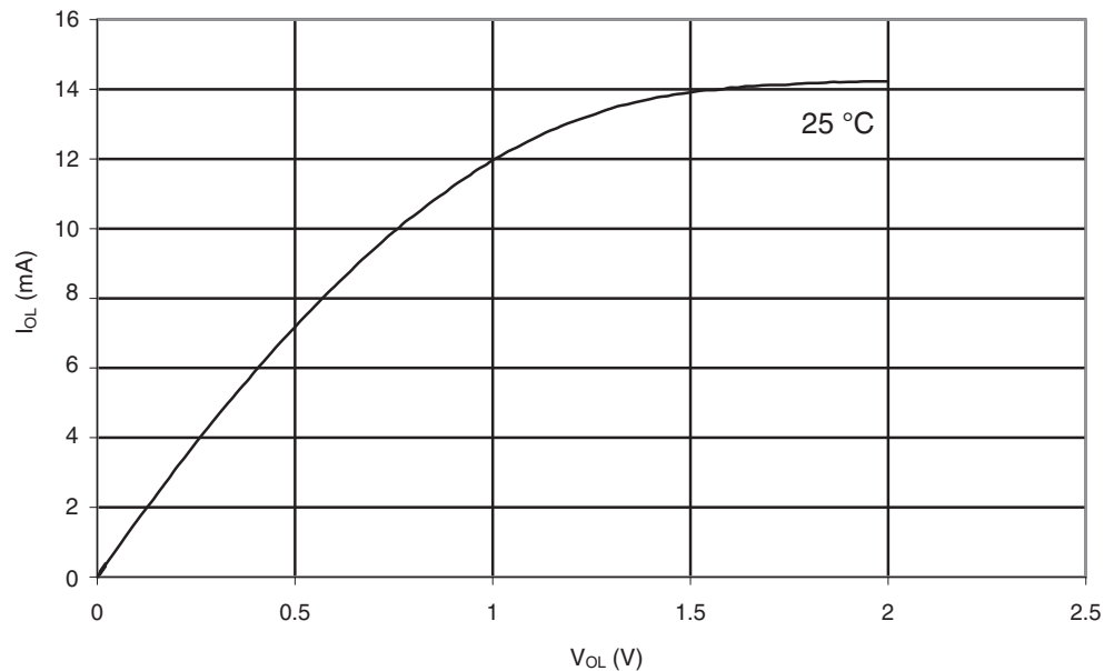
Figure 29-86. ATmega329P: I/O Pin Sink Current vs. Output Voltage, Port A,C,D,E,F,G,H,J ( V_{CC} = 2.7\text{ V} )
