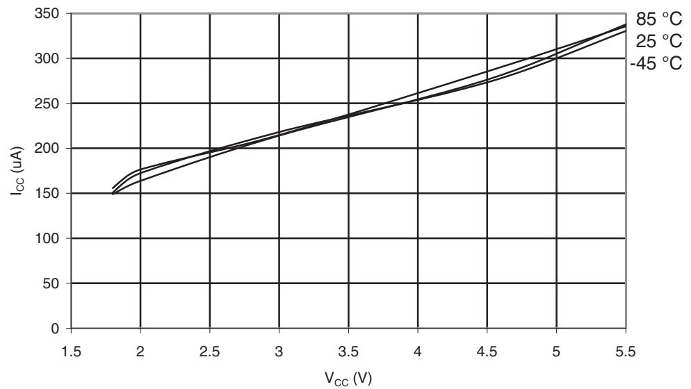
Figure 29-168. ATmega3290P: Active Supply Current with ADC at 1MHz vs. V_{CC}
