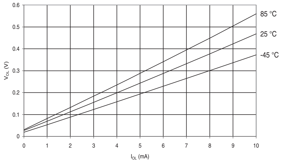
Figure 29-259. ATmega6490P: I/O Pin Output Voltage vs. Sink Current, Port A,C,D,E,F,G ( V_{CC}=5V )
