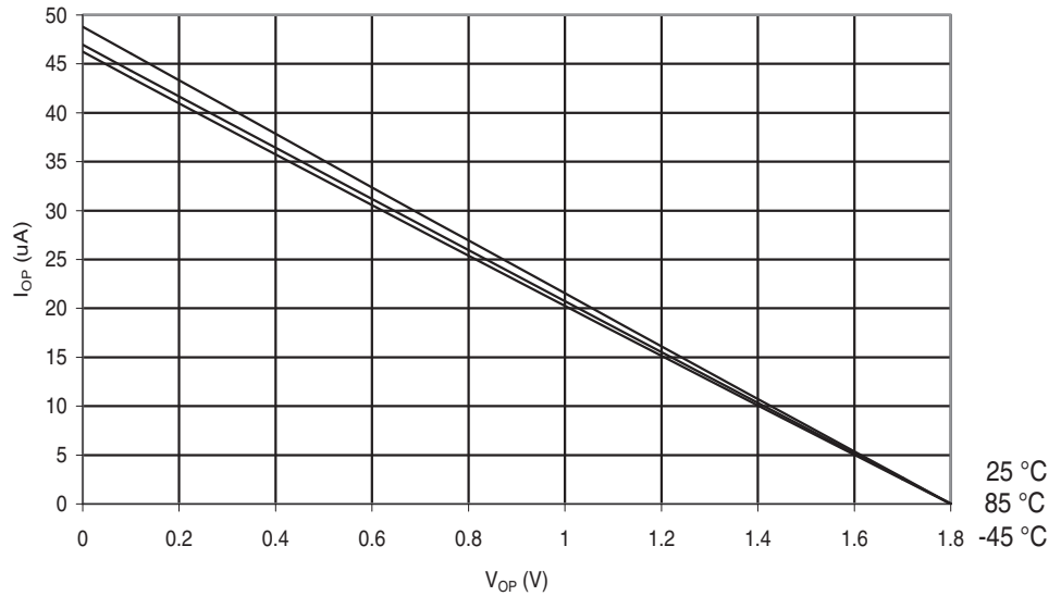
Figure 29-248. ATmega6490P: I/O Pin Pull-up Resistor Current vs. Input Voltage ( V_{CC} = 1.8V )
