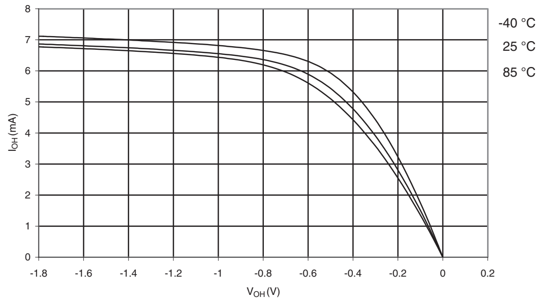
Figure 29-88. ATmega329P: I/O Pin Source Current vs. Output Voltage, Port B ( V_{CC} = 1.8\text{V} )
