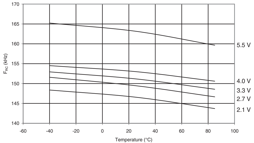
Figure 29-104. ATmega329P: Watchdog Oscillator Frequency vs. Temperature
