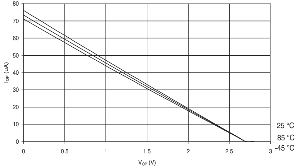
Figure 29-192. ATmega649P: I/O Pin Pull-up Resistor Current vs. Input Voltage ( V_{CC} = 2.7V )
