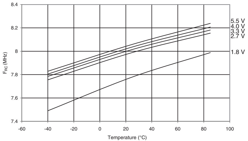
Figure 29-106. ATmega329P: Calibrated 8MHz RC Oscillator Frequency vs. Temperature
