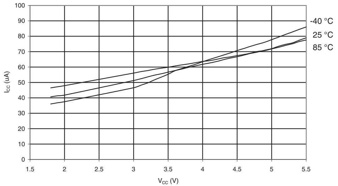
Figure 29-115. ATmega329P: Analog Comparator Current vs. V_{CC}
