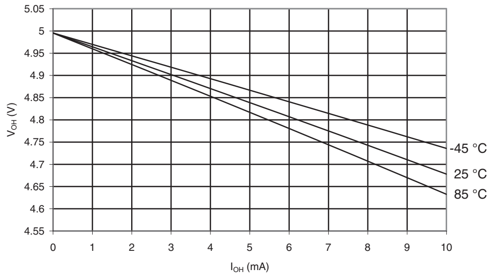
Figure 29-22. ATmega169PA: I/O Pin Output Voltage vs. Source Current, Ports A, C, D, E, F, G ( V_{CC} = 5V )
