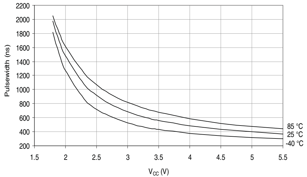
Figure 29-176. ATmega3290P: Minimum Reset Pulse Width vs. V_{CC}
