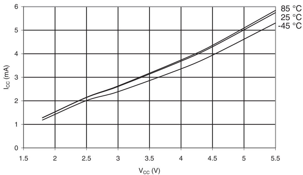
Figure 29-3. ATmega169PA: Active Supply Current vs. V_{CC} (Internal RC Oscillator, 8MHz)
