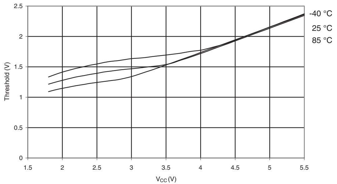
Figure 29-157. ATmega3290P: Reset Input Threshold Voltage vs. V_{CC} ( V_{IH} , IO Pin Read as "1")
