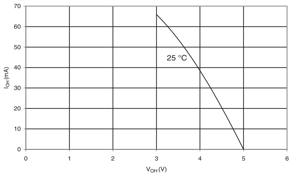
Figure 29-147. ATmega3290P: I/O Pin Source Current vs. Output Voltage, Port B ( V_{CC} = 5V )
