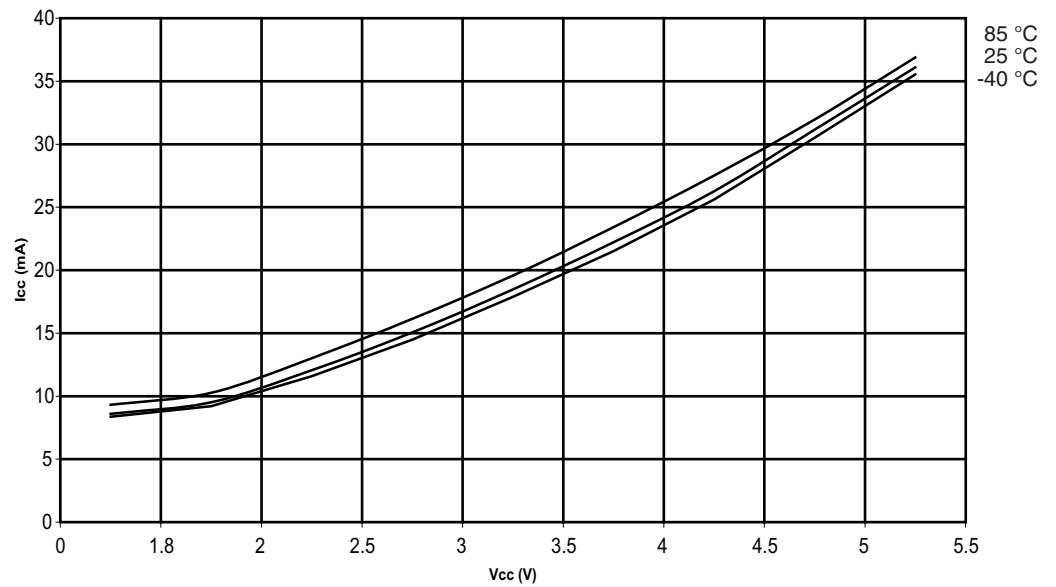
Figure 29-67. ATmega329P: Active Supply Current vs. V_{CC} (32kHz Watch Crystal)
