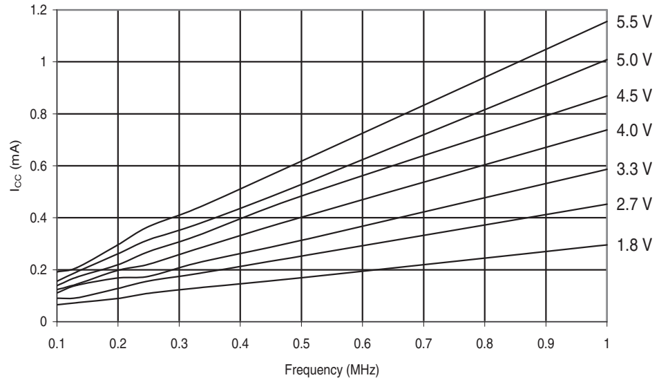
Figure 29-234. ATmega6490P: Active Supply Current vs. Low Frequency (0.1 - 1.0MHz)
