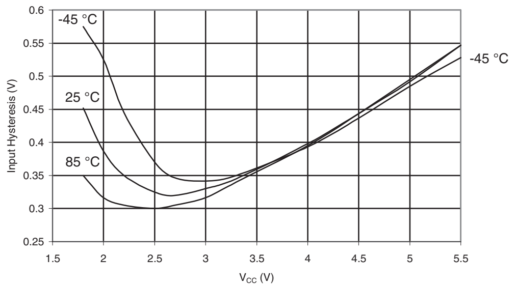
Figure 29-214. ATmega649P: I/O Pin Hysteresis vs. V_{CC} , Port A,C,D,E,F,G,H,J
