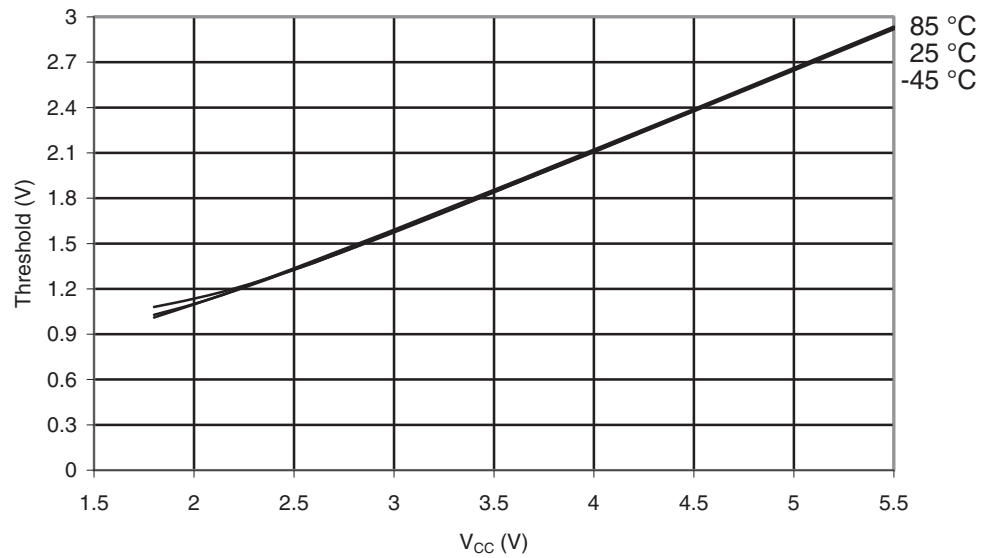
Figure 29-34. ATmega169PA: I/O Pin Input Threshold Voltage vs. V_{CC} ( V_{IH} , I/O Pin Read as “1”)
