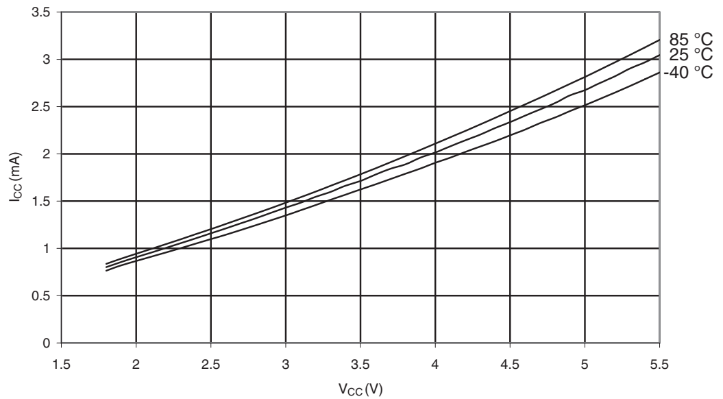
Figure 29-127. ATmega3290P: Idle Supply Current vs. V_{CC} (Internal RC Oscillator, 8MHz)
