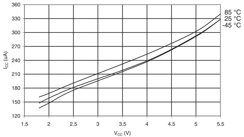
Figure 29-225. ATmega649P: Active Supply Current with ADC at 200kHz vs. V_{CC}
