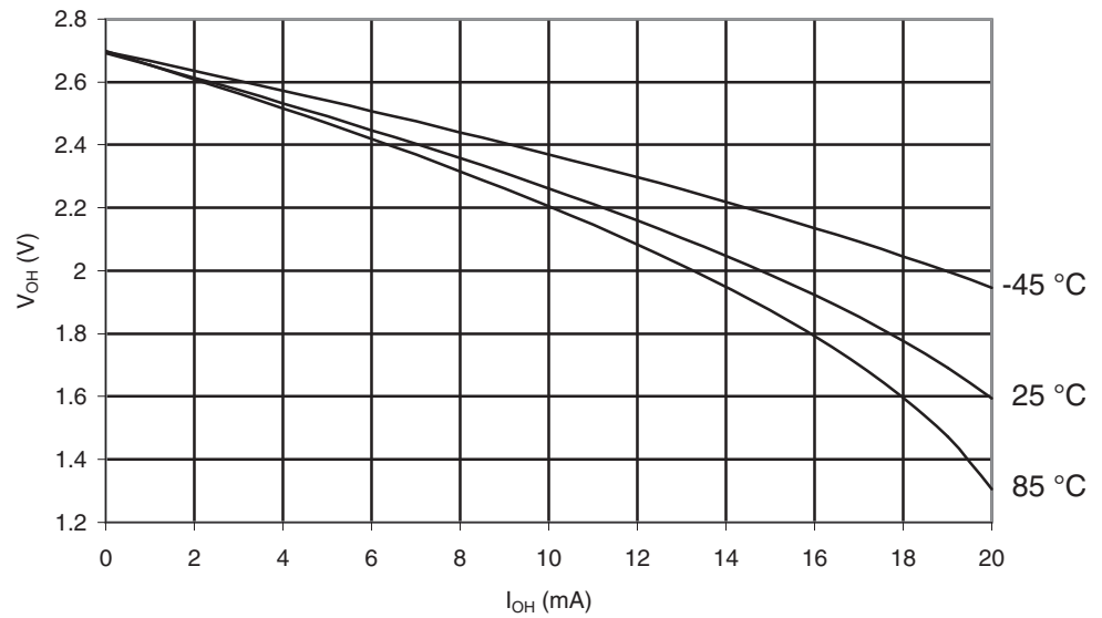
Figure 29-261. ATmega6490P: I/O Pin Output Voltage vs. Source Current, Port B ( V_{CC} = 2.7V )
