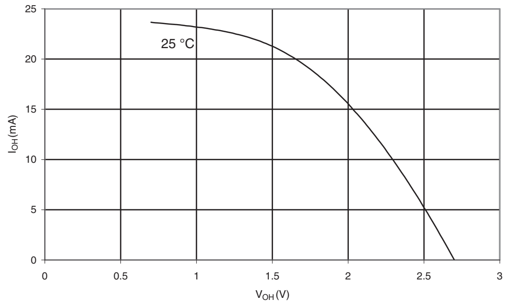
Figure 29-89. ATmega329P: I/O Pin Source Current vs. Output Voltage, Port B ( V_{CC} = 2.7V )
