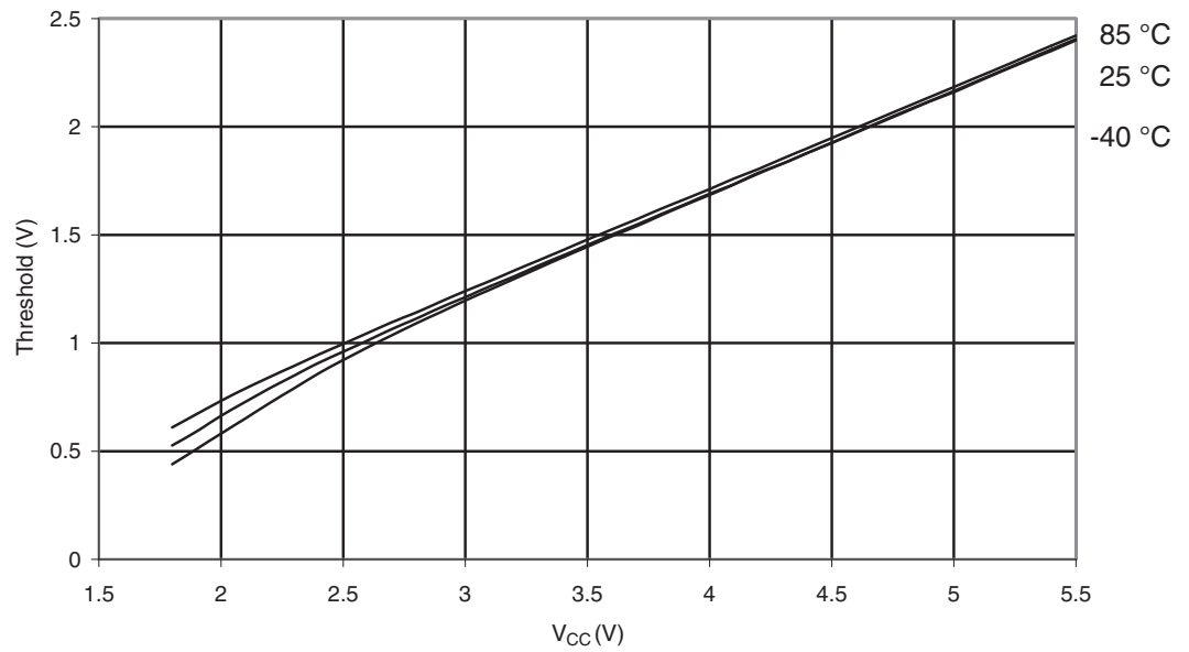
Figure 29-95. ATmega329P: I/O Pin Input Threshold Voltage vs. V_{CC} , Port B ( V_{IL} , IO Pin Read as "0")
