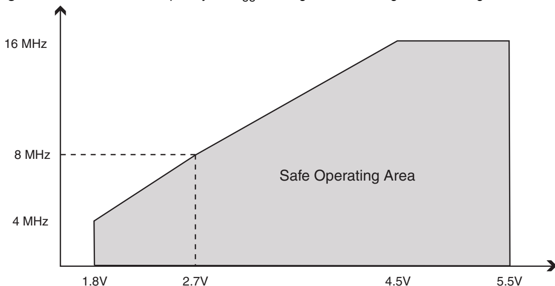
Figure 28-1. Maximum Frequency vs. V_{CC} , ATmega169PA/ATmega329P/ATmega3290P
