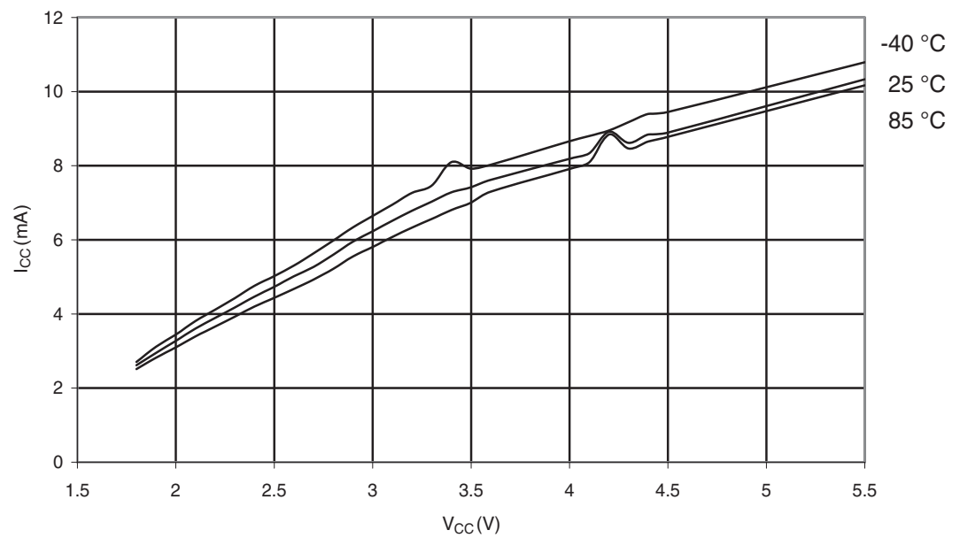
Figure 29-173. ATmega3290P: Programming Current vs. V_{CC}
