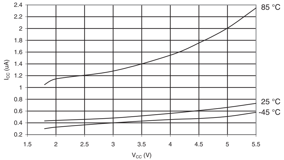
Figure 29-187. ATmega649P: Power-down Supply Current vs. V_{CC} (Watchdog Timer Disabled)
