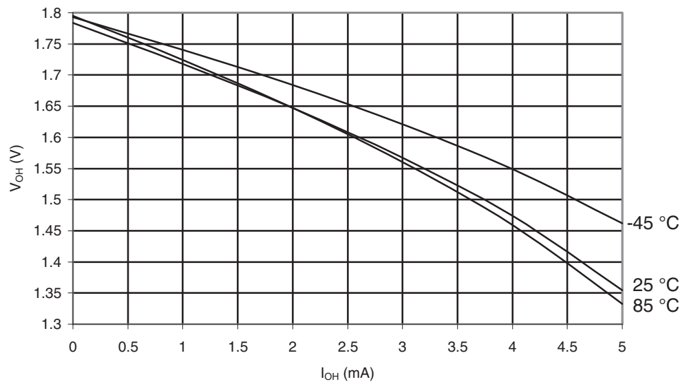
Figure 29-203. ATmega649P: I/O Pin Output Voltage vs. Source Current, Port B ( V_{CC} = 1.8V )
