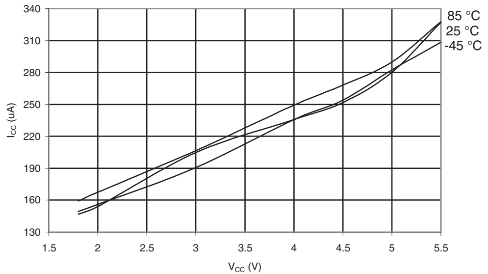
Figure 29-283. ATmega6490P: Active Supply Current with ADC at 1MHz vs. V_{CC}
