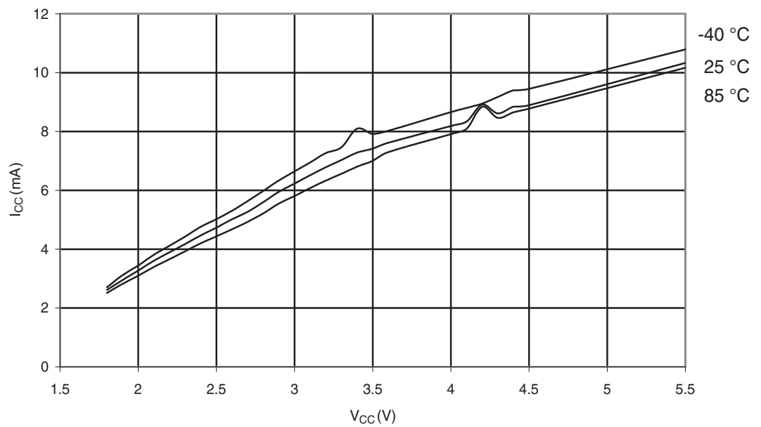
Figure 29-116. ATmega329P: Programming Current vs. V_{CC}
