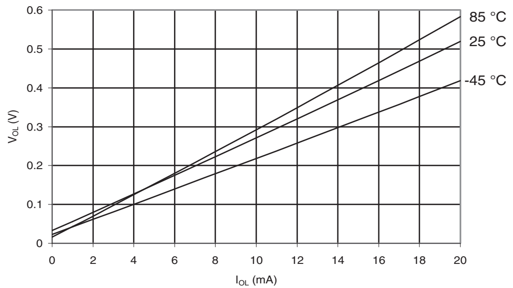
Figure 29-256. ATmega6490P: I/O Output Voltage vs. Pin Sink Current, Port B ( V_{CC} = 5V )
