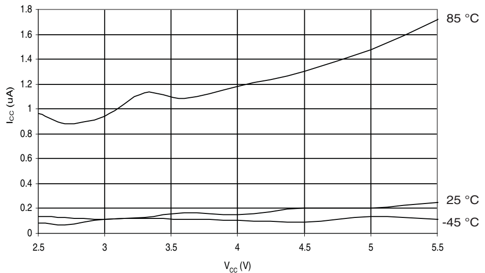
Figure 29-11. ATmega169PA: Power-down Supply Current vs. V_{CC} (Watchdog Timer Disabled)
