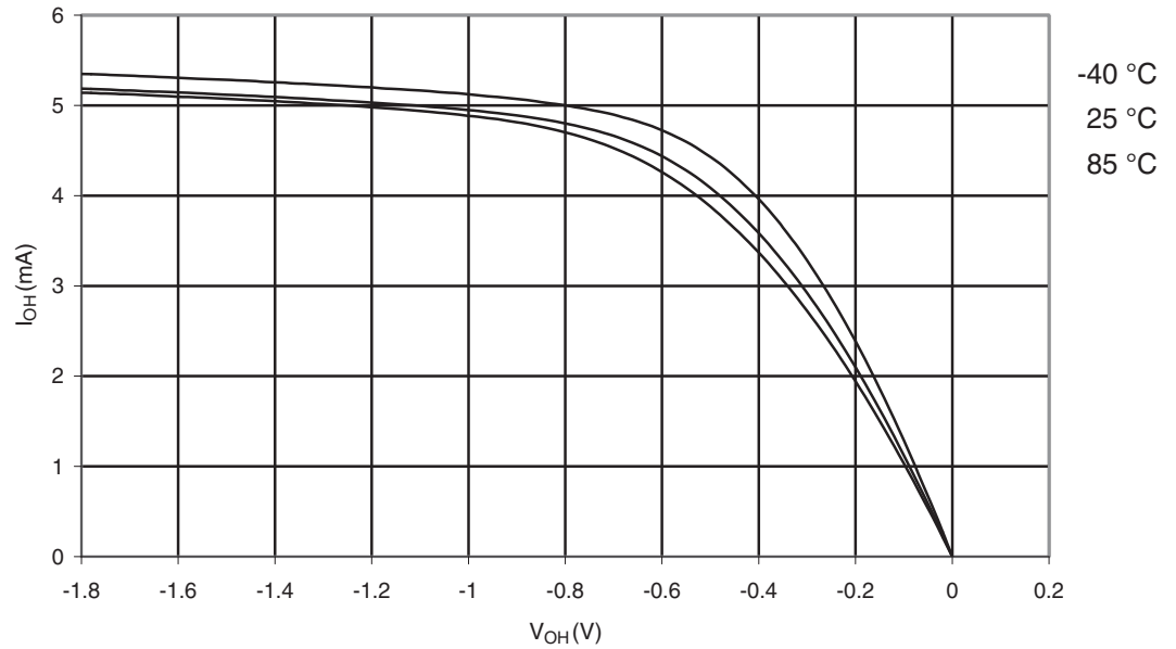
Figure 29-91. ATmega329P: I/O Pin Source Current vs. Output Voltage, Port A,C,D,E,F,G,H,J ( V_{CC}=1.8V )
