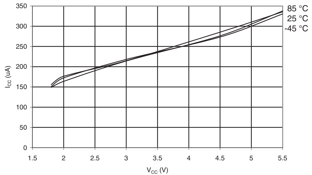
Figure 29-111. ATmega329P: Active Supply Current with ADC at 1MHz vs. V_{CC}
