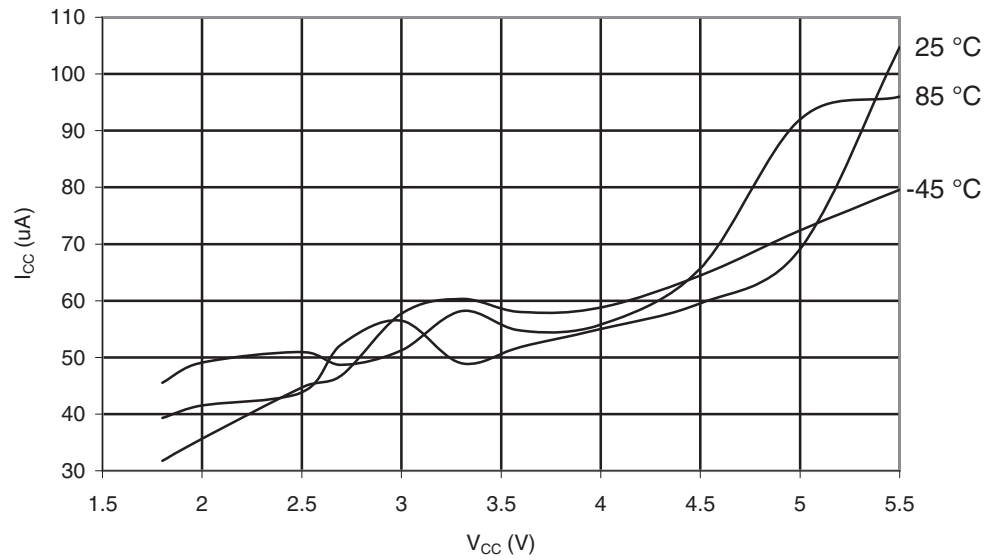
Figure 29-229. ATmega649P: Analog Comparator Current vs. V_{CC}
