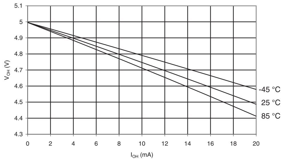
Figure 29-25. ATmega169PA: I/O Pin Output Voltage vs. Source Current, Port B ( V_{CC} = 5V )
