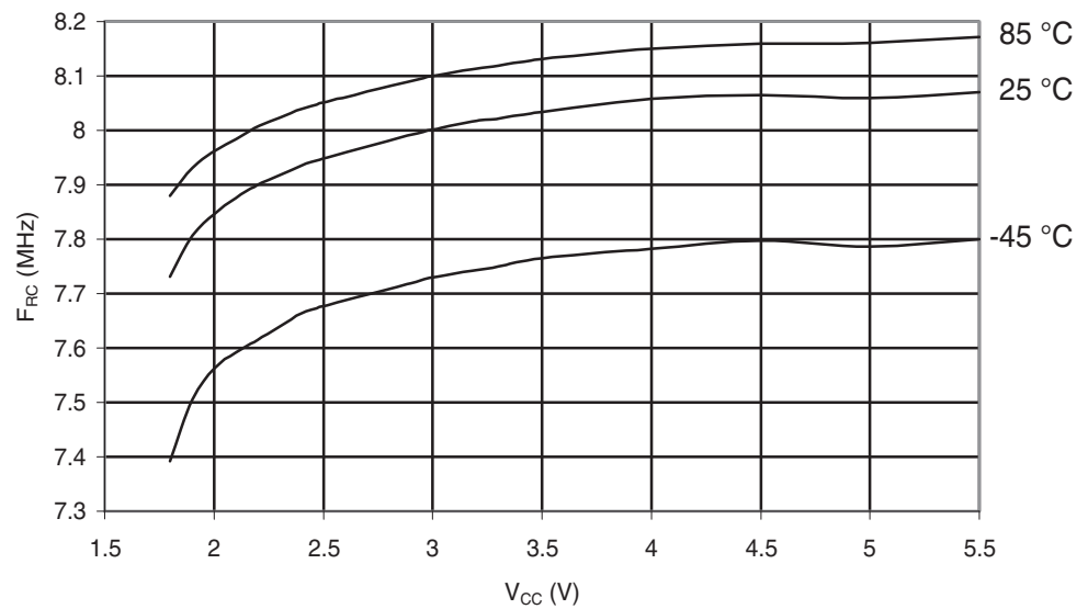
Figure 29-220. ATmega649P: Calibrated 8MHz RC Oscillator Frequency vs. V_{CC}
