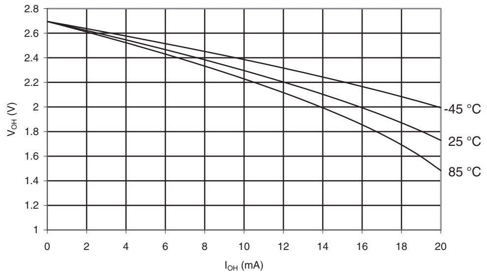
Figure 29-26. ATmega169PA: I/O Pin Output Voltage vs. Source Current, Port B ( V_{CC} = 2.7V )
