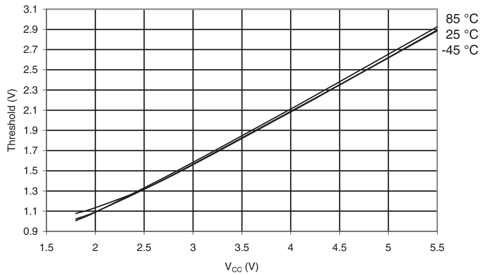
Figure 29-269. ATmega6490P: I/O Pin Input Threshold Voltage vs. V_{CC} , ( V_{IH} , IO Pin Read as "1")
