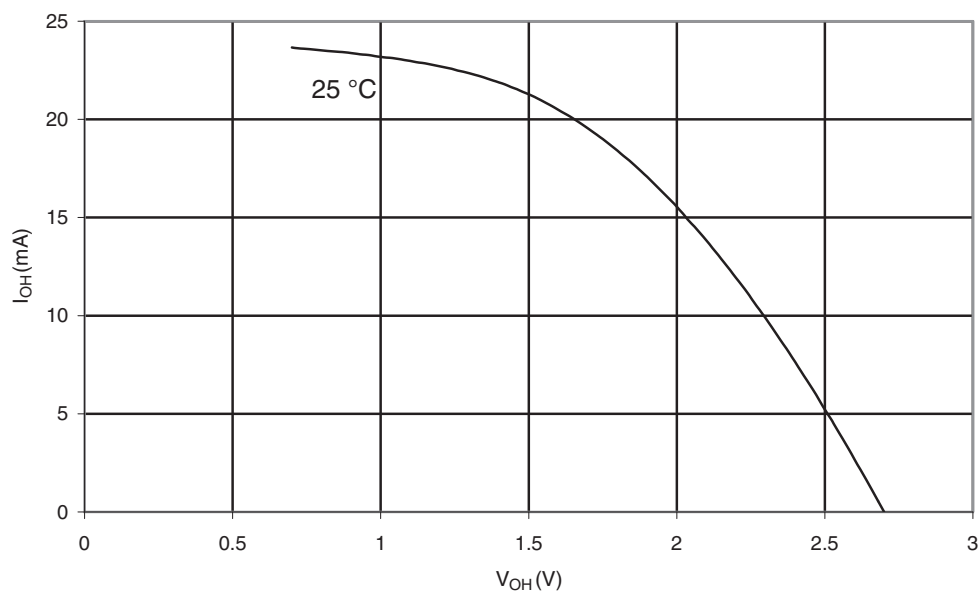
Figure 29-146. ATmega3290P: I/O Pin Source Current vs. Output Voltage, Port B ( V_{CC} = 2.7V )
