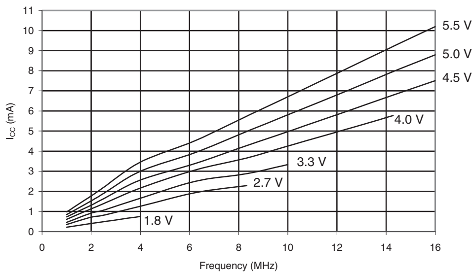
Figure 29-2. ATmega169PA: Active Supply Current vs. Frequency (1 - 16MHz)
