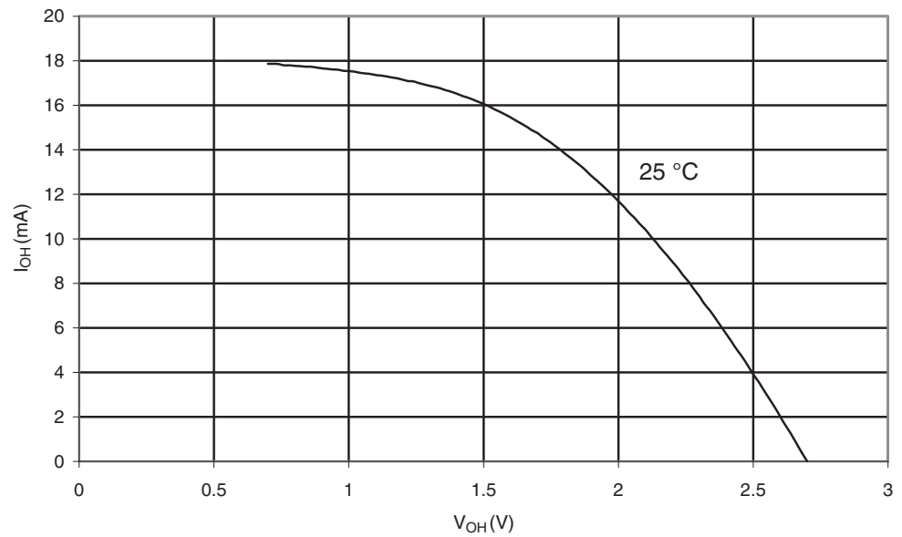
Figure 29-149. ATmega3290P: I/O Pin Source Current vs. Output Voltage, Port A,C,D,E,F,G,H,J ( V_{CC}=2.7V )
