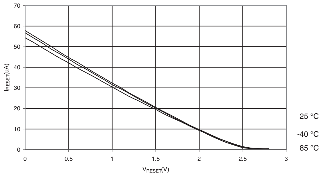
Figure 29-137. ATmega3290P: Reset Pull-up Resistor Current vs. Reset Pin Voltage ( V_{CC} = 2.7V )
