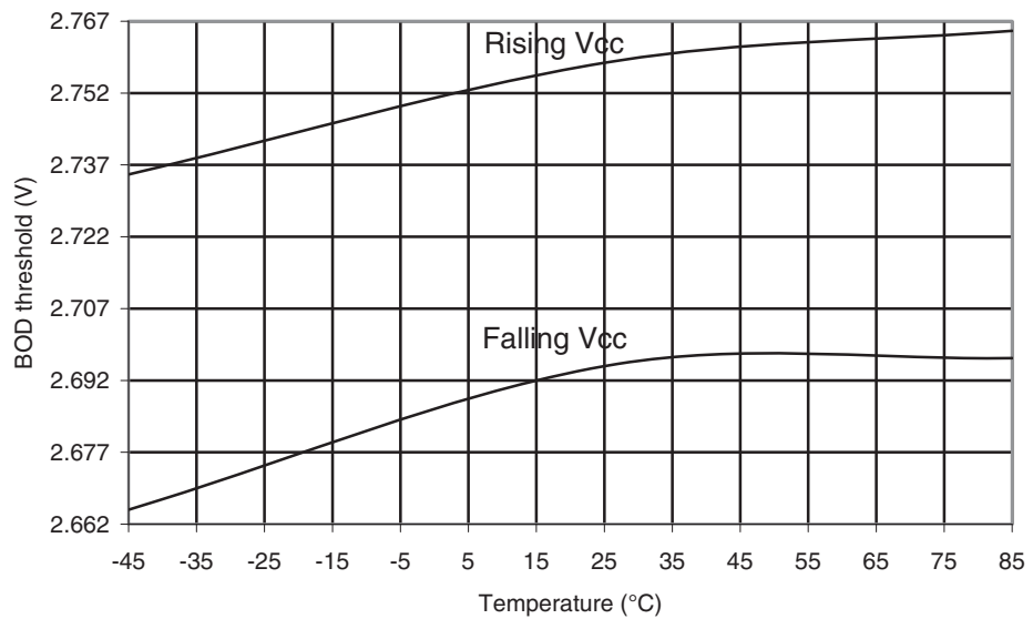
Figure 29-41. ATmega169PA: BOD Thresholds vs. Temperature (BOD Level is 2.7V)
