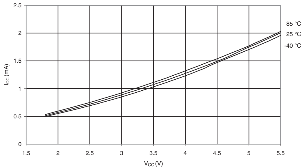
Figure 29-123.) ATmega3290P: Active Supply Current vs. V_{CC} (Internal RC Oscillator, 1MHz)
