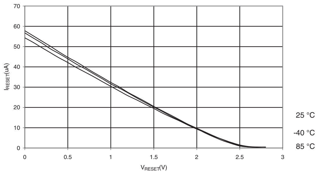
Figure 29-80. ATmega329P: Reset Pull-up Resistor Current vs. Reset Pin Voltage ( V_{CC} = 2.7V )
