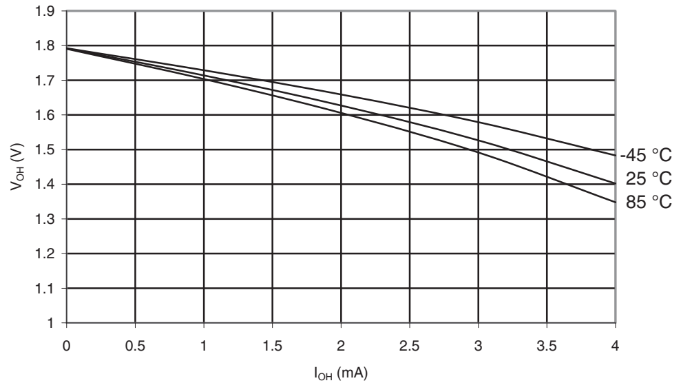
Figure 29-24. ATmega169PA: I/O Pin Output Voltage vs. Source Current, Ports A, C, D, E, F, G ( V_{CC} = 1.8V )
