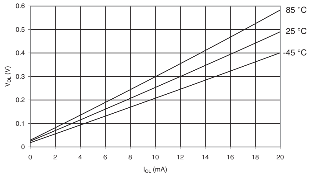
Figure 29-31. ATmega169PA: I/O Pin Output Voltage vs. Sink Current, Port B ( V_{CC} = 5V )
