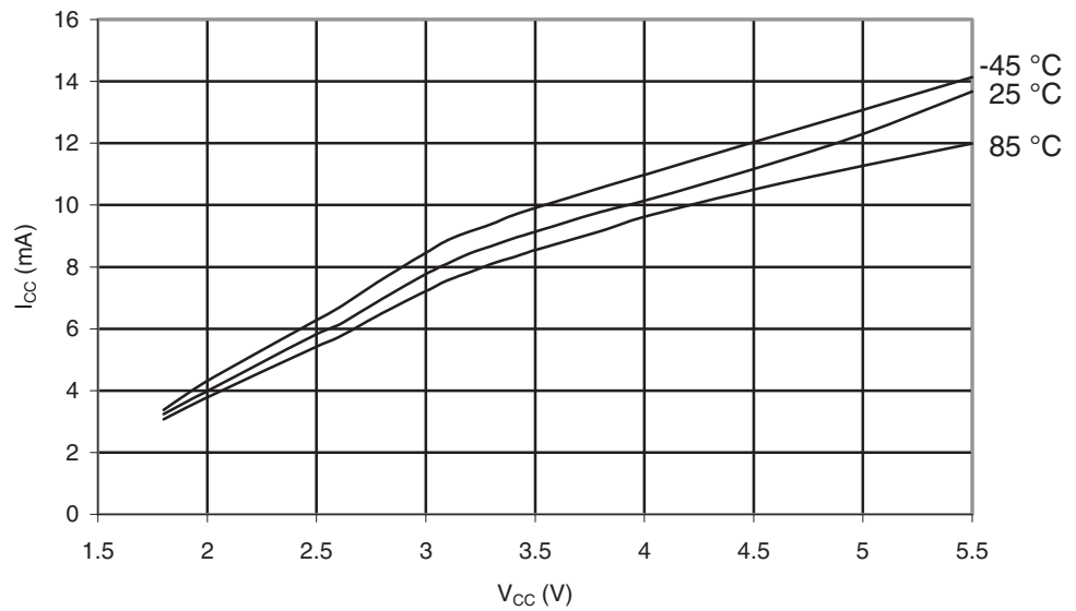
Figure 29-59. ATmega169PA: Programming Current vs. V_{CC}
