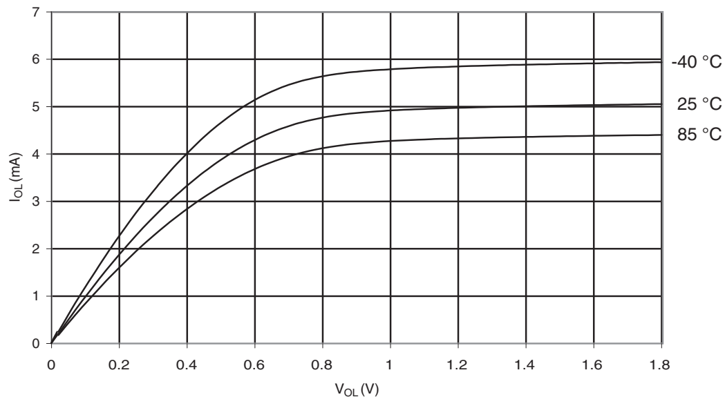
Figure 29-85. ATmega329P: I/O Pin Sink Current vs. Output Voltage, Port A,C,D,E,F,G,H,J ( V_{CC} = 1.8\text{ V} )
