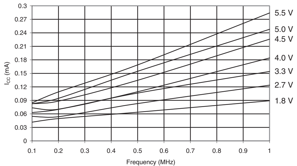
Figure 29-239. ATmega6490P: Idle Supply Current vs. Low Frequency (0.1 - 1.0MHz)
