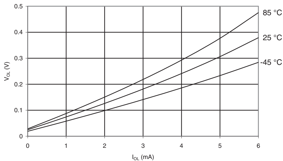
Figure 29-33. ATmega169PA: I/O Pin Output Voltage vs. Sink Current, Port B ( V_{CC} = 1.8V )
