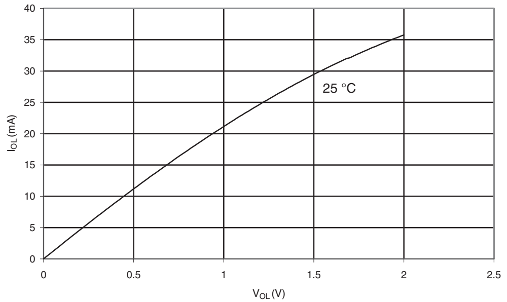
Figure 29-144. ATmega3290P: I/O Pin Sink Current vs. Output Voltage, Port A,C,D,E,F,G,H,J ( V_{CC}=5V )
