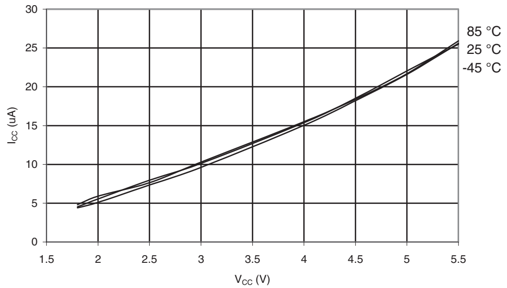
Figure 29-57. ATmega169PA: Watchdog Timer Current vs. V_{CC}
