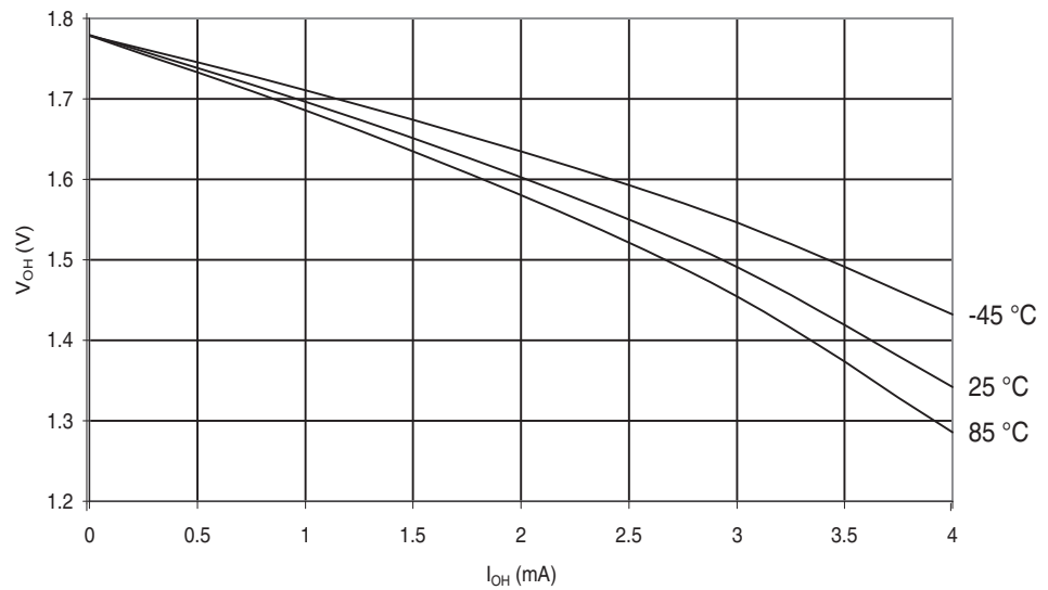
Figure 29-206. ATmega649P: I/O Pin Output Voltage vs. Source Current, Port A,C,D,E,F,G ( V_{CC} = 1.8V )
