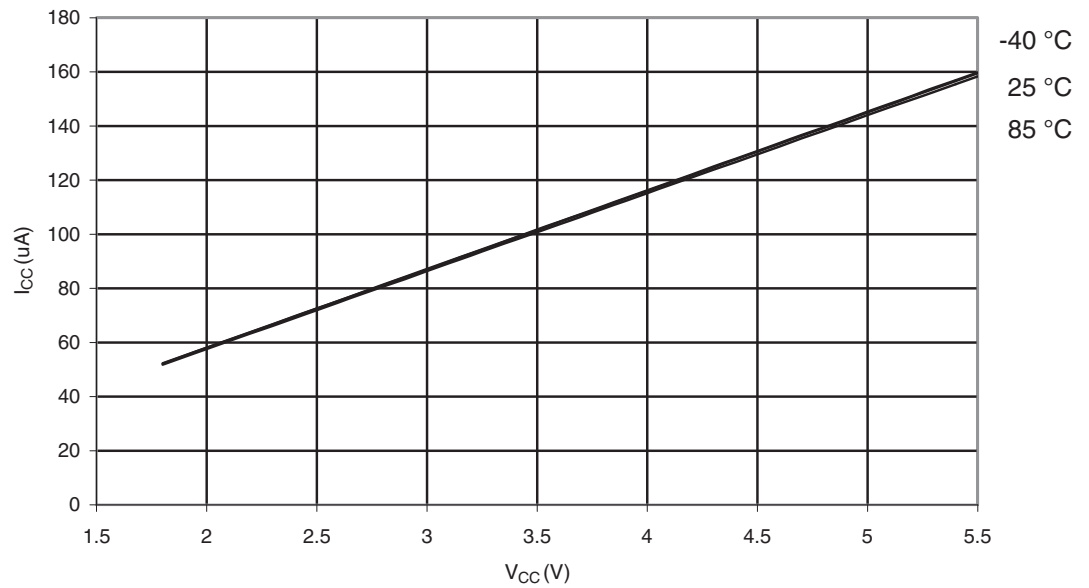
Figure 29-113. ATmega329P: AREF External Reference Current vs. V_{CC}
