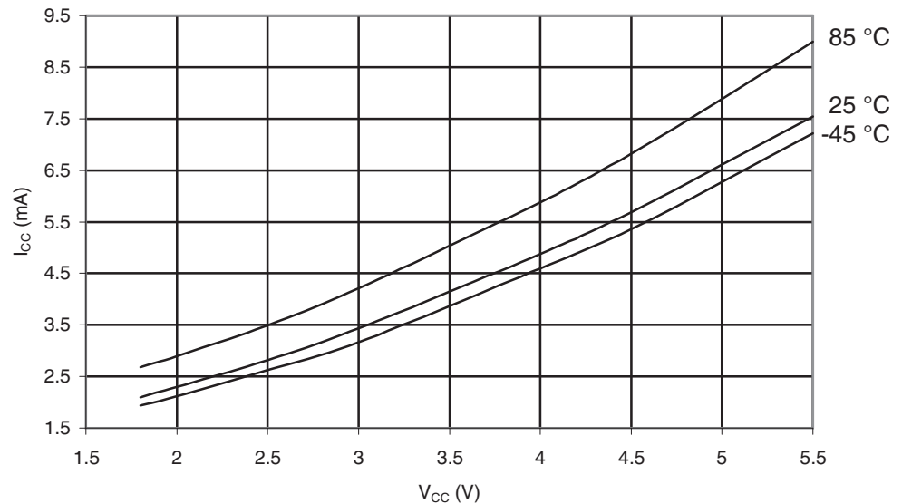
Figure 29-186. ATmega649P: Idle Supply Current vs. V_{CC} (32kHz Watch Crystal)
