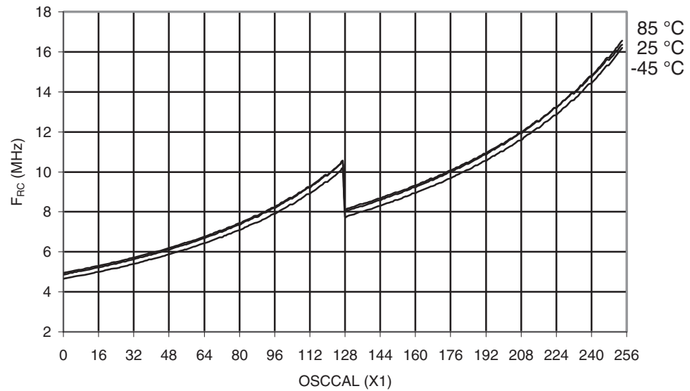
Figure 29-222. ATmega649P: Calibrated 8MHz RC Oscillator Frequency vs. Oscal Value
