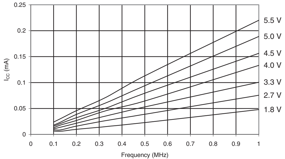
Figure 29-6. ATmega169PA: Idle Supply Current vs. Frequency (0.1 - 1.0MHz)
