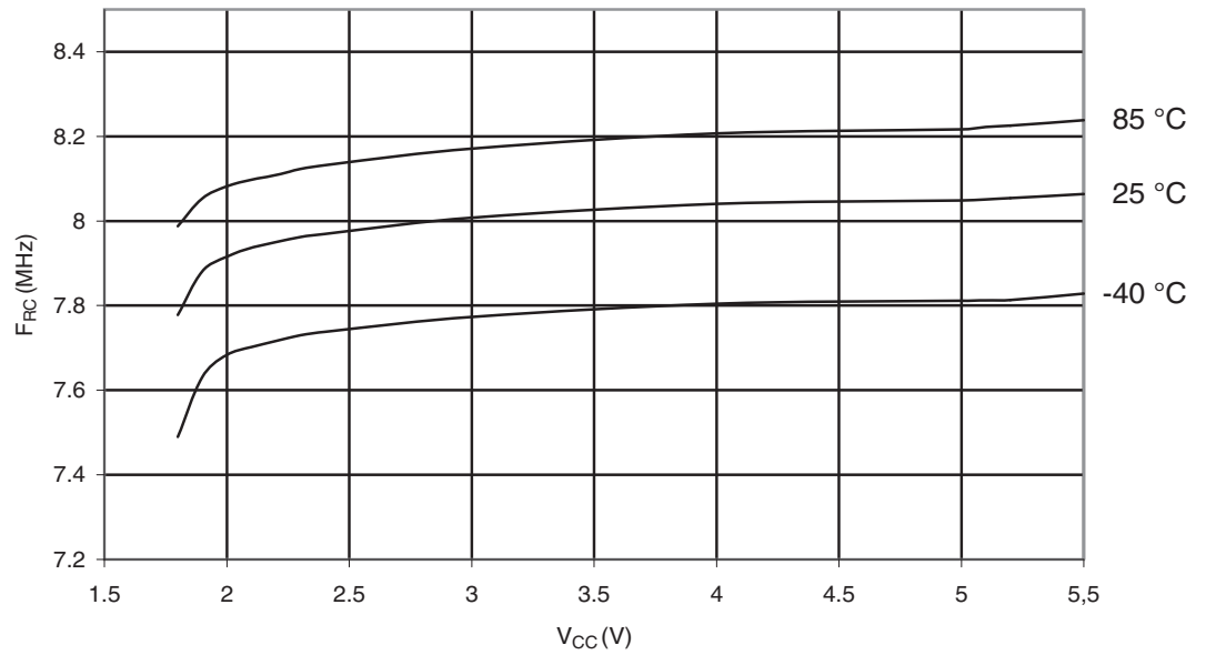
Figure 29-105. ATmega329P: Calibrated 8MHz RC Oscillator Frequency vs. V_{CC}
