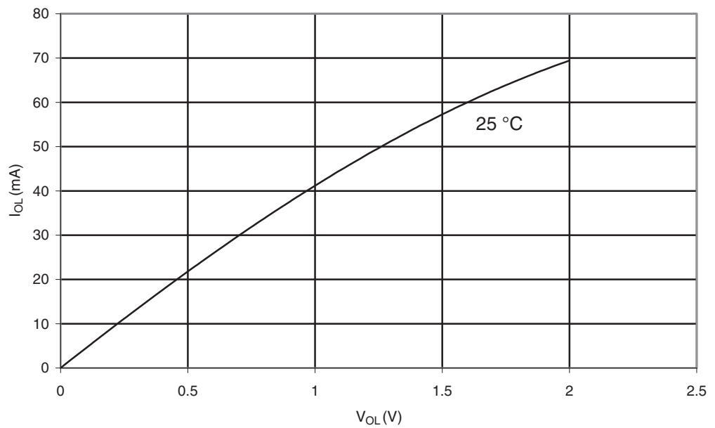
Figure 29-141. ATmega3290P: I/O Pin Sink Current vs. Output Voltage, Port B ( V_{CC} = 5V )
