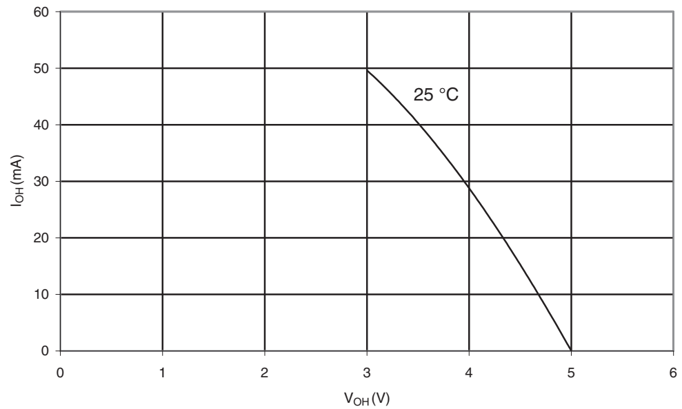
Figure 29-93. ATmega329P: I/O Pin Source Current vs. Output Voltage, Port A,C,D,E,F,G,H,J ( V_{CC}=5V )
