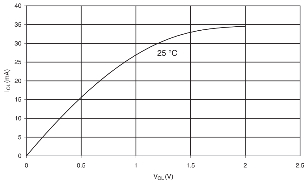
Figure 29-140. ATmega3290P: I/O Pin Sink Current vs. Output Voltage, Port B ( V_{CC} = 2.7V )
