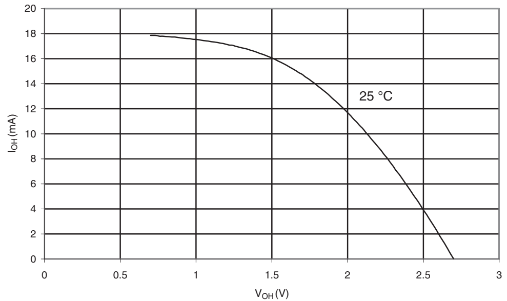
Figure 29-92. ATmega329P: I/O Pin Source Current vs. Output Voltage, Port A,C,D,E,F,G,H,J ( V_{CC}=2.7V )
