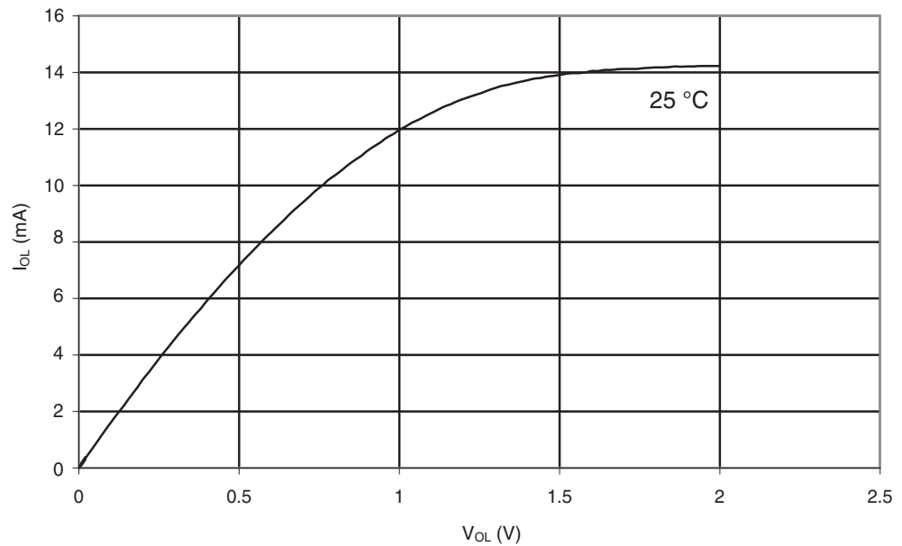
Figure 29-143. ATmega3290P: I/O Pin Sink Current vs. Output Voltage, Port A,C,D,E,F,G,H,J ( V_{CC} = 2.7V )
