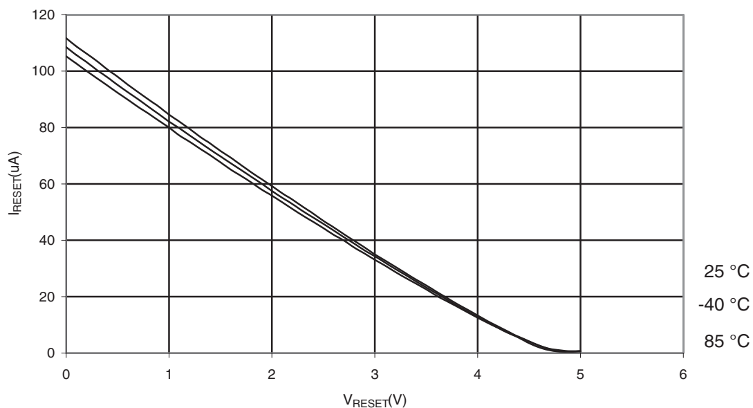
Figure 29-81. ATmega329P: Reset Pull-up Resistor Current vs. Reset Pin Voltage ( V_{CC} = 5V )
