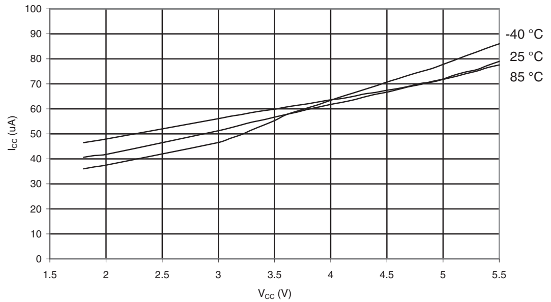
Figure 29-172. ATmega3290P: Analog Comparator Current vs. V_{CC}
