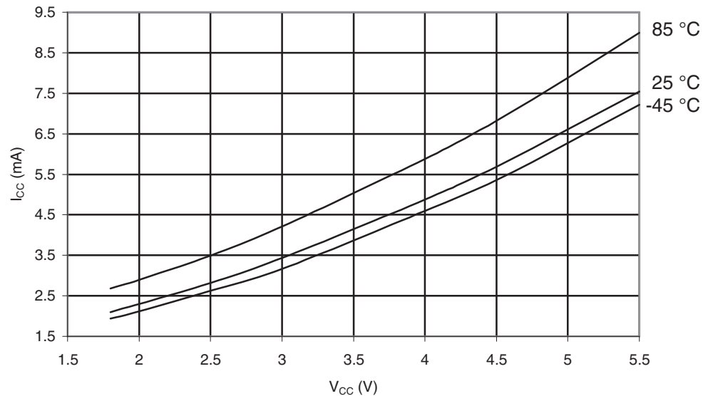
Figure 29-243. ATmega6490P: Idle Supply Current vs. V_{CC} (32kHz Watch Crystal)
