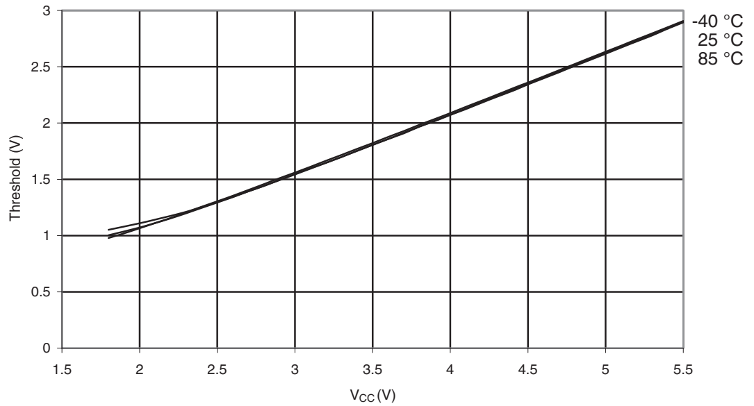
Figure 29-154. ATmega3290P: I/O Pin Input Threshold Voltage vs. V_{CC} , Port A,C,D,E,F,G,H,J ( V_{IH} , IO Pin Read as "1")
