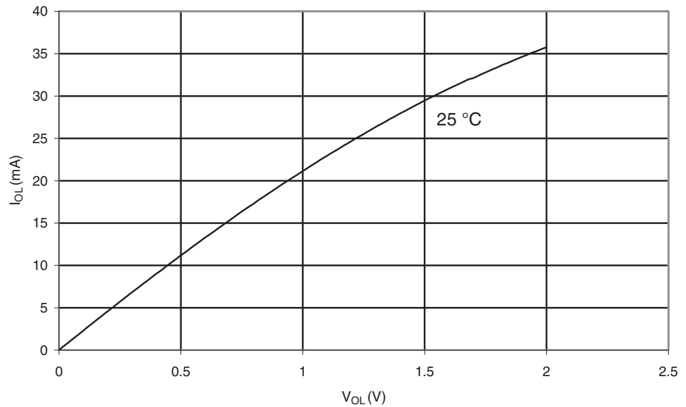
Figure 29-87. ATmega329P: I/O Pin Sink Current vs. Output Voltage, Port A,C,D,E,F,G,H,J ( V_{CC} = 5\text{ V} )
