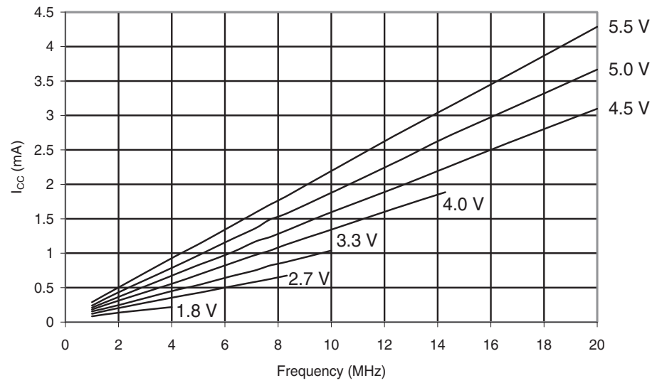
Figure 29-183. ATmega649P: Idle Supply Current vs. Frequency (1 - 20MHz)
