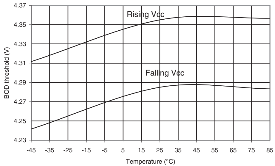
Figure 29-40. ATmega169PA: BOD Thresholds vs. Temperature (BOD Level is 4.3V)
