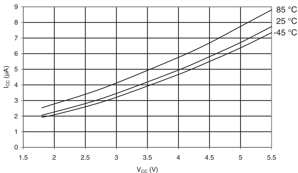
Figure 29-10. ATmega169PA: Idle Supply Current vs. V_{CC} (32kHz Watch Crystal)
