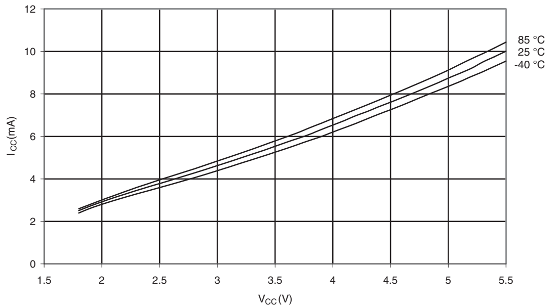
Figure 29-65. ATmega329P: Active Supply Current vs. V_{CC} (Internal RC Oscillator, 8MHz)
