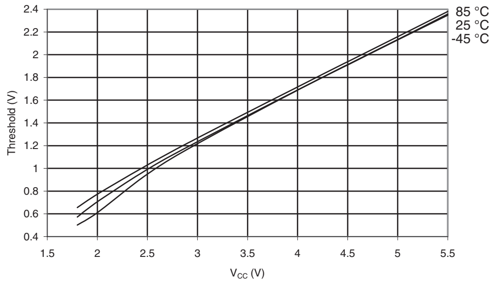
Figure 29-213. ATmega649P: I/O Pin Input Threshold Voltage vs. V_{CC} ( V_{IL} , IO Pin Read as "0")
