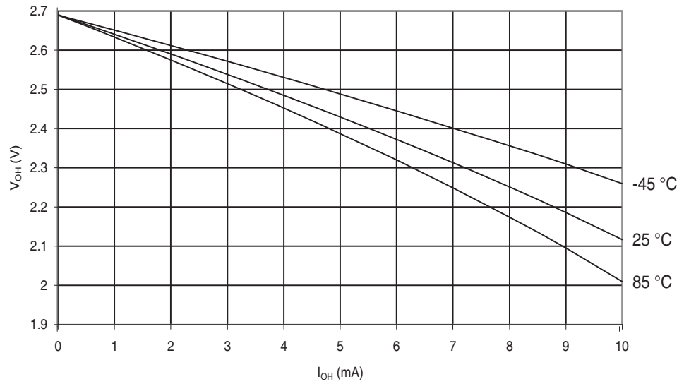
Figure 29-264. ATmega6490P: I/O Pin Output Voltage vs. Source Current, Port A,C,D,E,F,G ( V_{CC}=2.7 )
