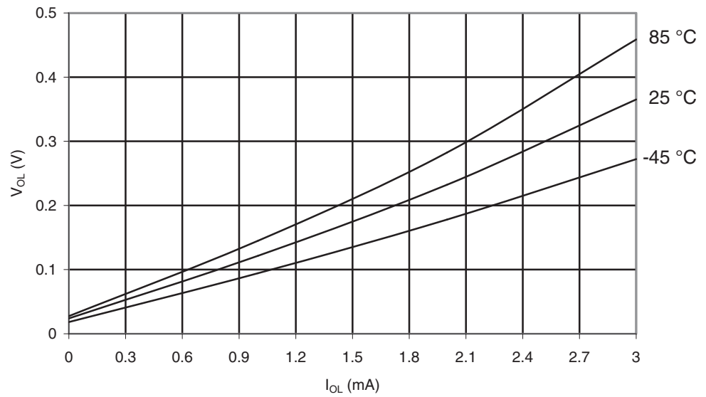
Figure 29-30. ATmega169PA: I/O Pin Output Voltage vs. Sink Current, Ports A, C, D, E, F, G ( V_{CC} = 1.8V )
