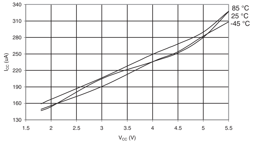
Figure 29-284. ATmega6490P: AREF External Reference Current vs. V CC
