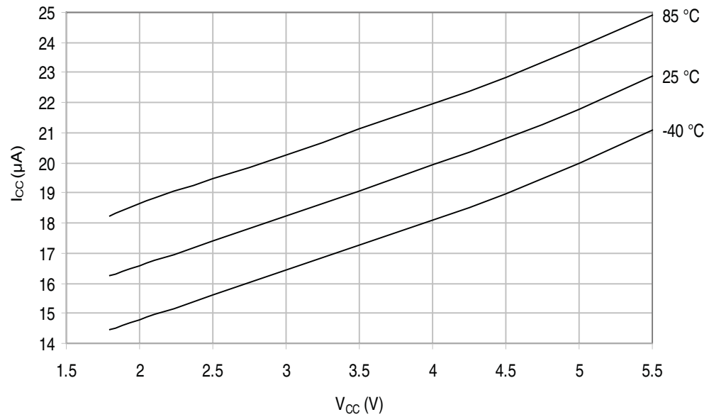
Figure 29-108. ATmega329P: Brownout Detector Current vs. V_{CC}
