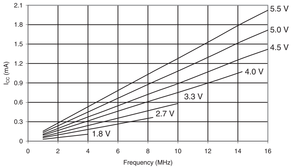
Figure 29-61. ATmega169PA: Reset Supply Current vs. V_{CC} (1 - 16MHz, Excluding Current Through The Reset Pull-up)
