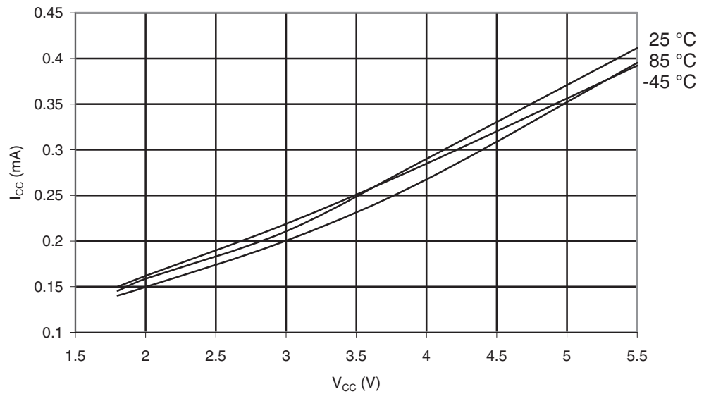
Figure 29-242. ATmega6490P: Idle Supply Current vs. V_{CC} (Internal RC Oscillator, 1MHz)
