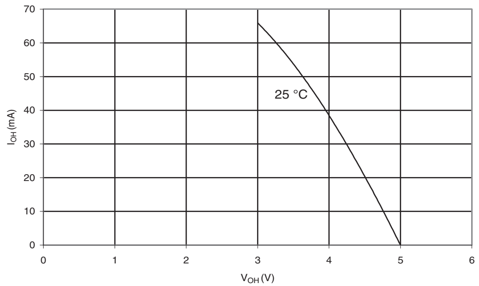
Figure 29-90. ATmega329P: I/O Pin Source Current vs. Output Voltage, Port B ( V_{CC} = 5V )
