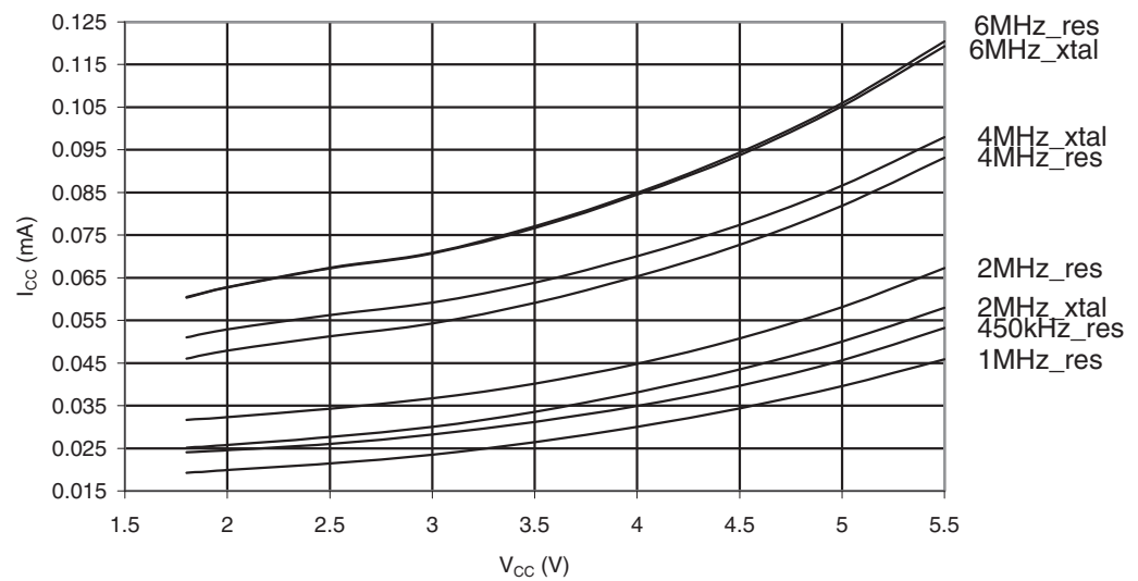
Figure 29-190. ATmega649P: Standby Supply Current vs. V_{CC} (32kHz Watch Crystal, Watchdog Timer Disabled)
