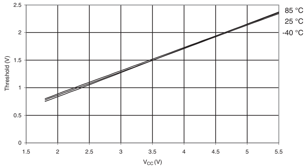
Figure 29-101. ATmega329P: Reset Input Threshold Voltage vs. V_{CC} ( V_{IL} , IO Pin Read as "0")
