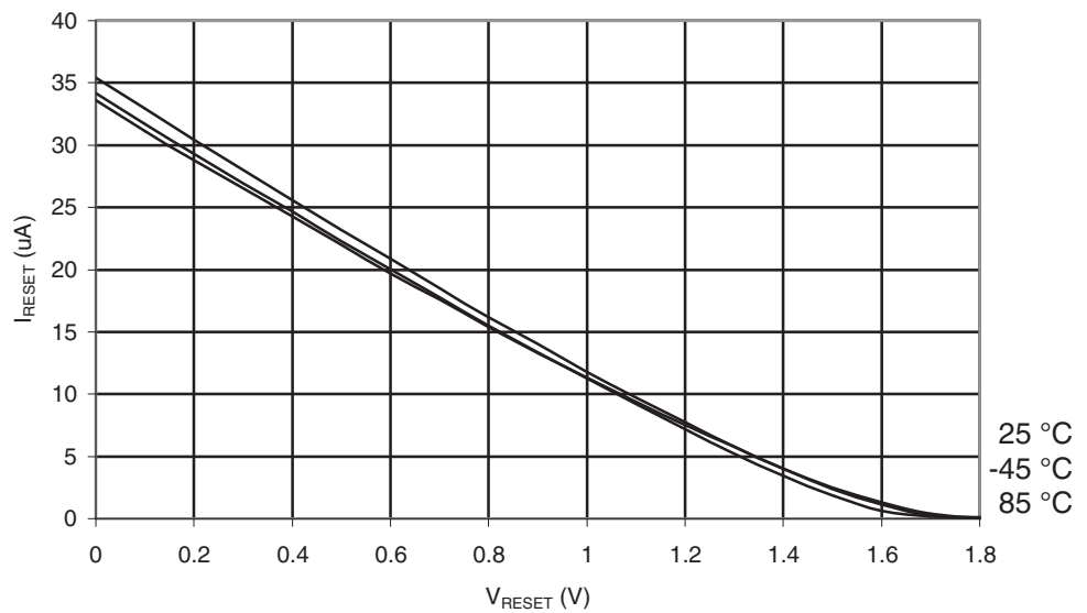
Figure 29-194. ATmega649P: Reset Pull-up Resistor Current vs. Reset Pin Voltage ( V_{CC} = 1.8V )
