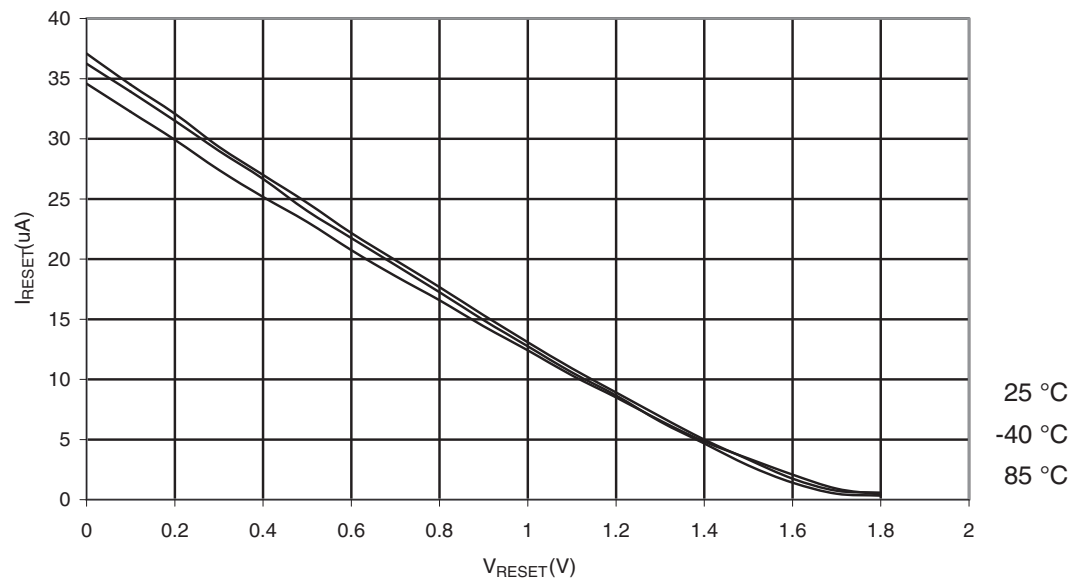
Figure 29-79. ATmega329P: Reset Pull-up Resistor Current vs. Reset Pin Voltage ( V_{CC} = 1.8V )
