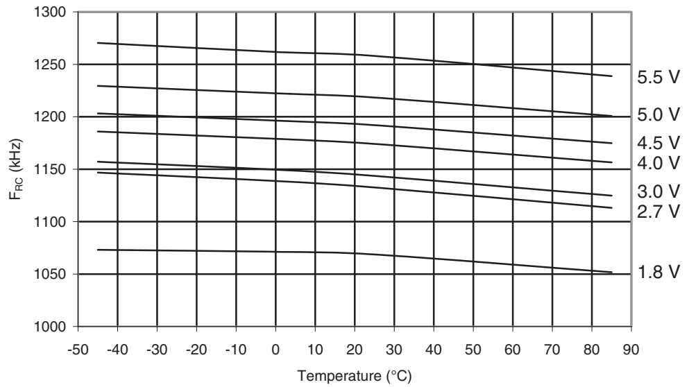
Figure 29-48. ATmega169PA: Watchdog Oscillator Frequency vs. Temperature
