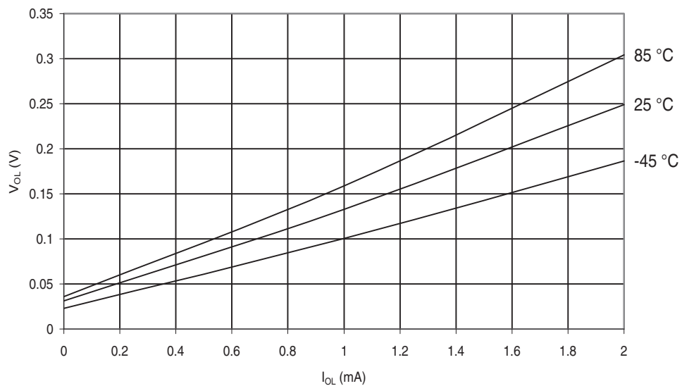
Figure 29-200. ATmega649P: I/O Pin Output Voltage vs. Sink Current, Port A,C,D,E,F,G ( V_{CC} = 1.8V )
