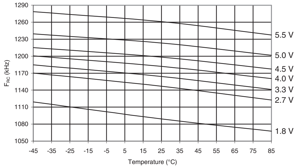
Figure 29-276. ATmega6490P: Watchdog Oscillator Frequency vs. Temperature
