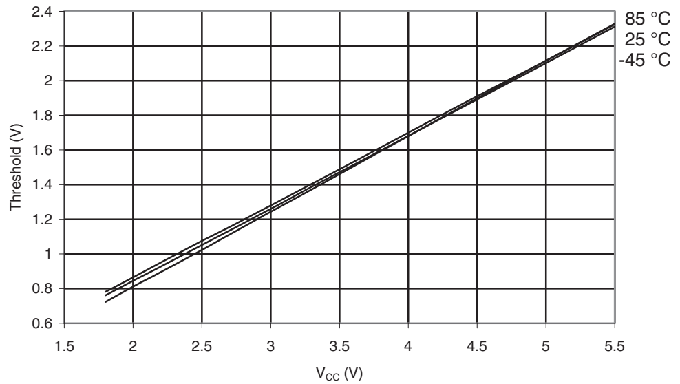
Figure 29-38. ATmega169PA: Reset Input Threshold Voltage vs. V_{CC} ( V_{IL} , Reset Pin Read as “0”)
