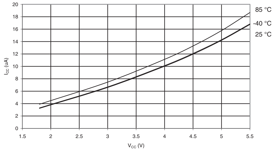
Figure 29-73. ATmega329P: Power-down Supply Current vs. V_{CC} (Watchdog Timer Enabled)
