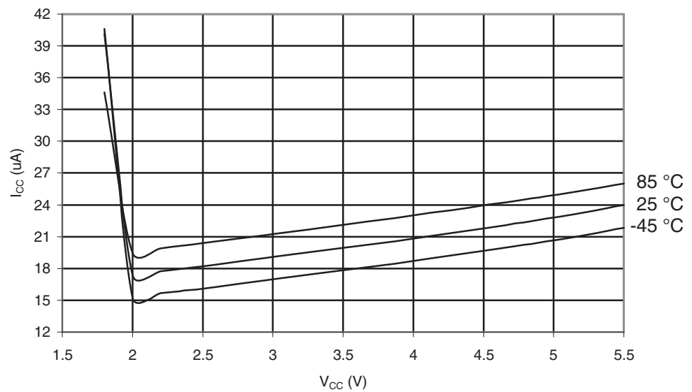
Figure 29-280. ATmega6490P: Brownout Detector Current vs. V_{CC}
