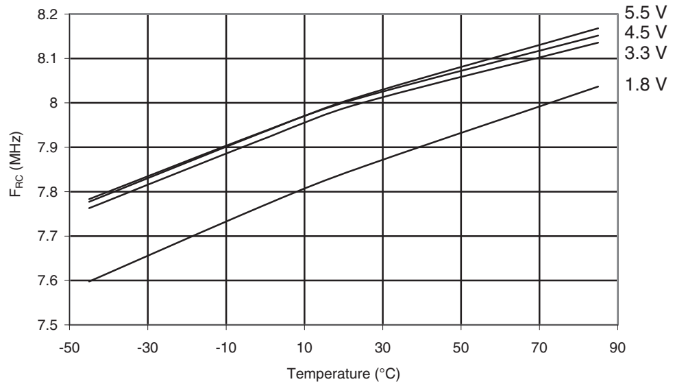
Figure 29-49. ATmega169PA: Calibrated 8MHz RC Oscillator Frequency vs. Temperature
