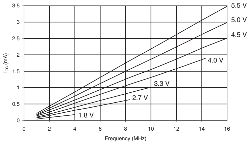
Figure 29-7. ATmega169PA: Idle Supply Current vs. Frequency (1 - 16MHz)
