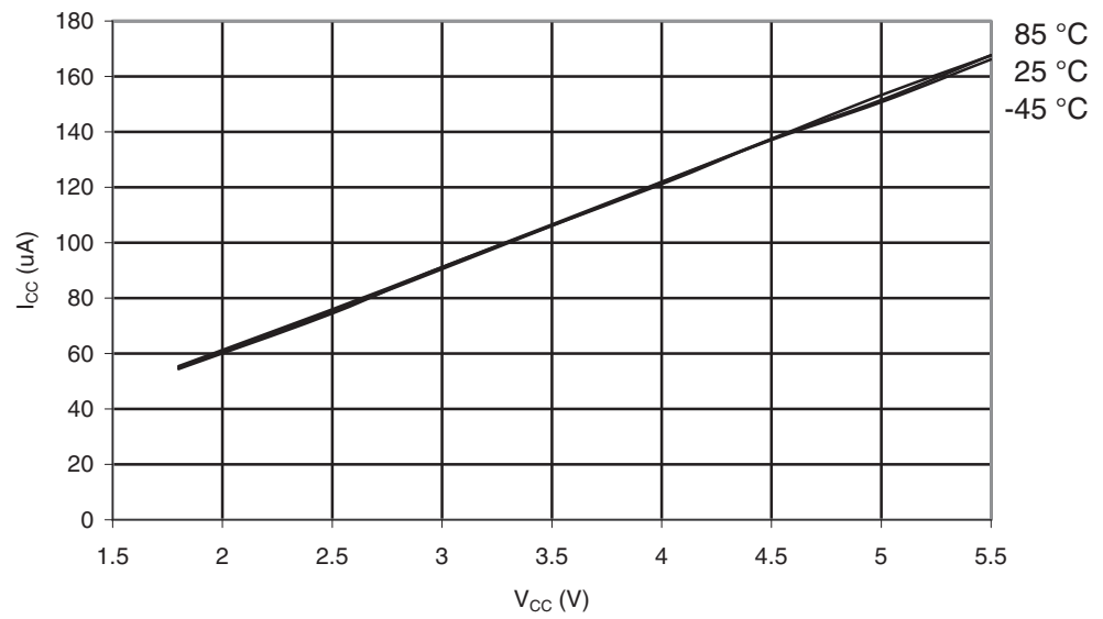
Figure 29-56. ATmega169PA: AREF External Reference Current vs. V_{CC}
