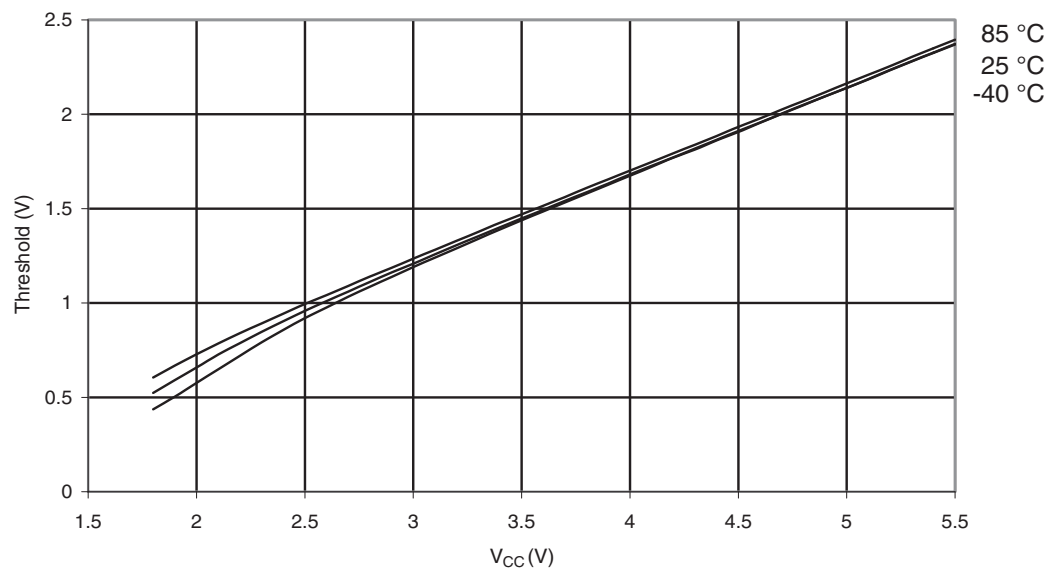
Figure 29-98. ATmega329P: I/O Pin Input Threshold Voltage vs. V_{CC} , Port A,C,D,E,F,G,H,J ( V_{IL} , IO Pin Read as "0")
