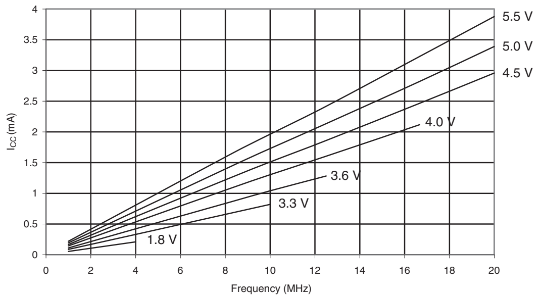
Figure 29-175. ATmega3290P: Reset Supply Current vs. Frequency (1 - 20MHz)
