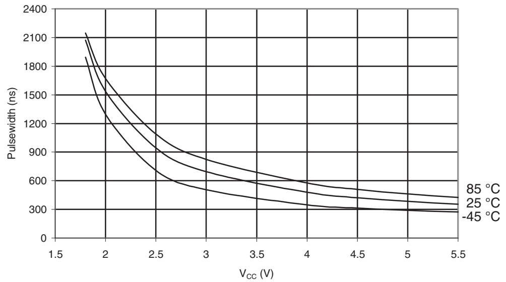
Figure 29-290. ATmega6490P: Minimum Reset Pulse Width vs. V_{CC}
