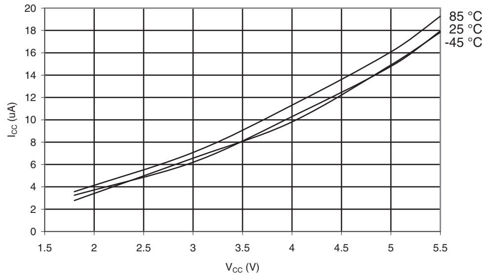
Figure 29-12. ATmega169PA: Power-down Supply Current vs. V_{CC} (Watchdog Timer Enabled)
