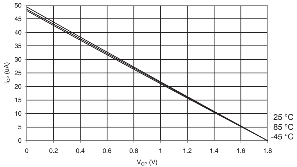
Figure 29-18. ATmega169PA: I/O Pin Pull-up Resistor Current vs. Input Voltage ( V_{CC} = 1.8V )
