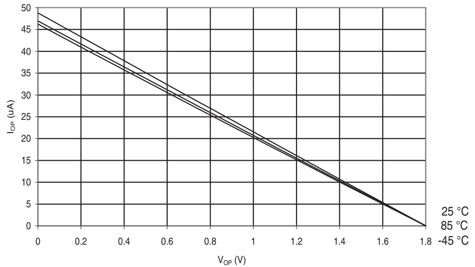
Figure 29-191. ATmega649P: I/O Pin Pull-up Resistor Current vs. Input Voltage ( V_{CC} = 1.8V )
