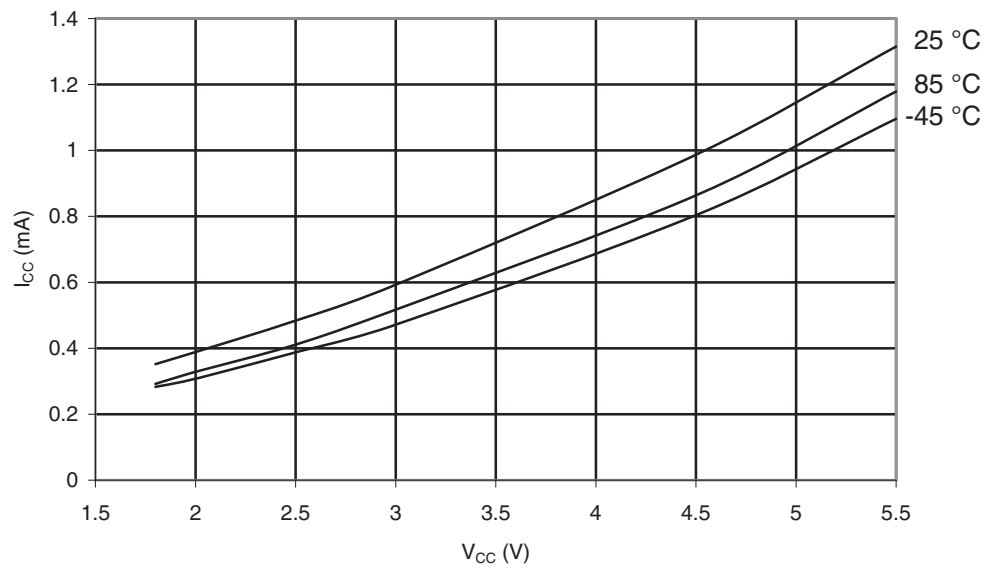
Figure 29-4. ATmega169PA: Active Supply Current vs. V_{CC} (Internal RC Oscillator, 1MHz)
