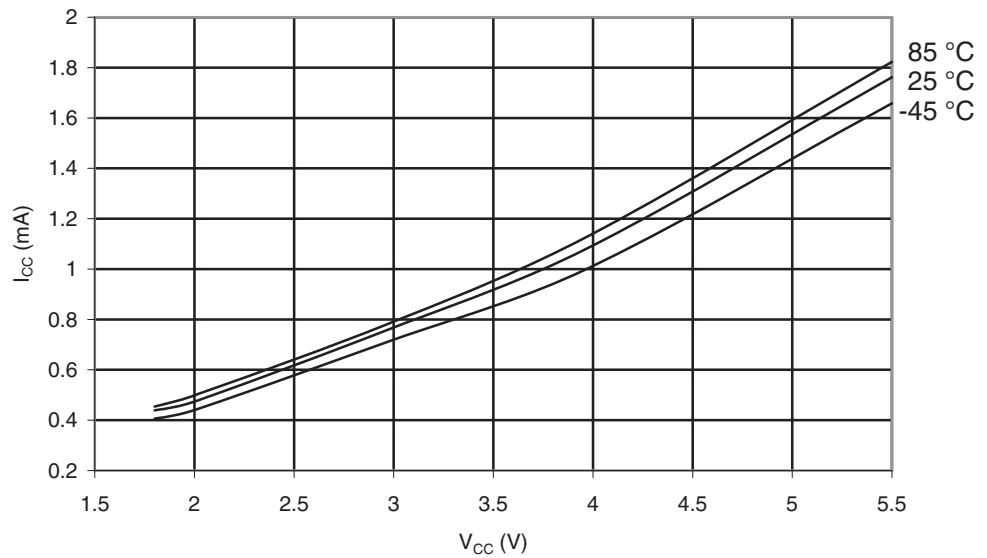
Figure 29-184. ATmega649P: Idle Supply Current vs. V_{CC} (Internal RC Oscillator, 8MHz)
