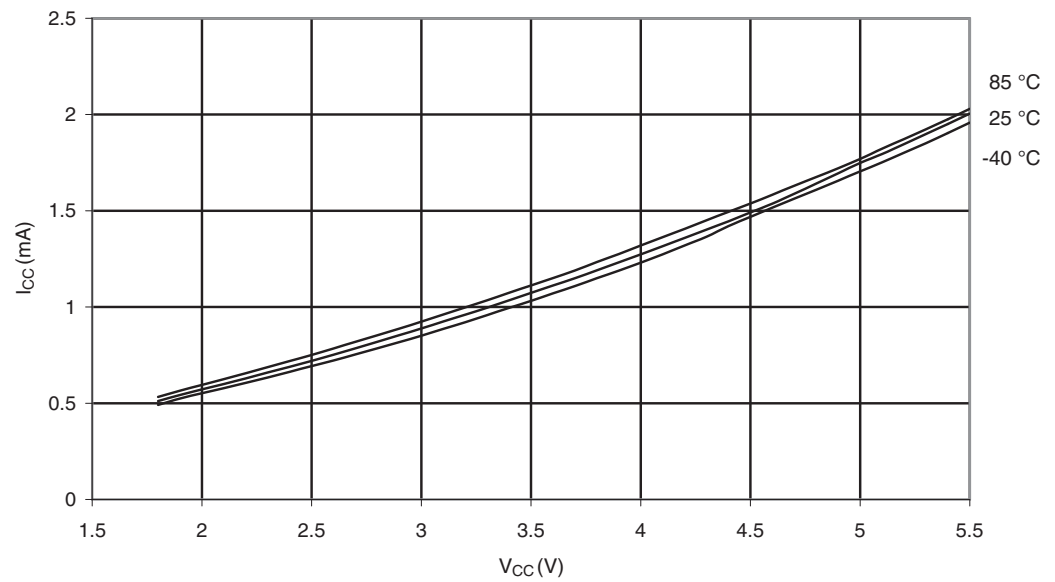
Figure 29-66. ATmega329P: Active Supply Current vs. V_{CC} (Internal RC Oscillator, 1MHz)
