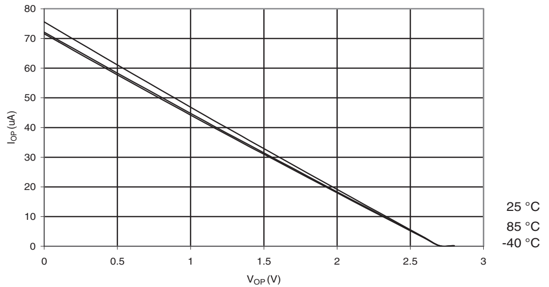
Figure 29-77. ATmega329P: I/O Pin Pull-up Resistor Current vs. Input Voltage ( V_{CC} = 2.7V )
