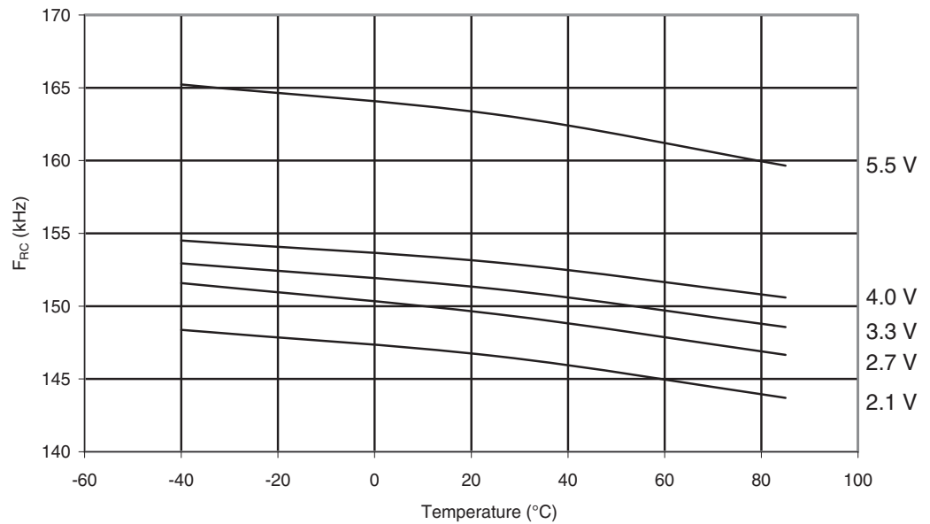
Figure 29-161. ATmega3290P: Watchdog Oscillator Frequency vs. Temperature
