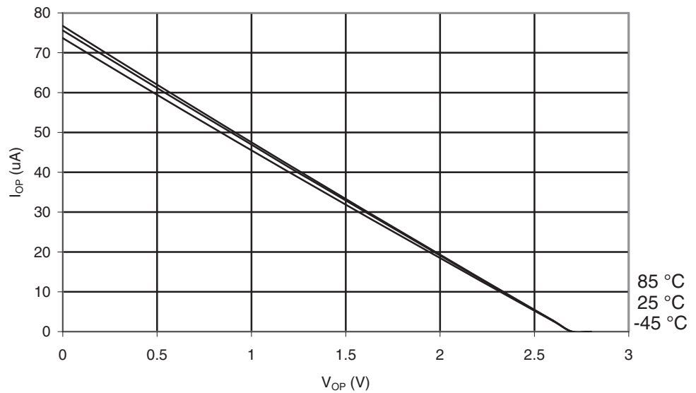
Figure 29-17. ATmega169PA: I/O Pin Pull-up Resistor Current vs. Input Voltage ( V_{CC} = 2.7V )
