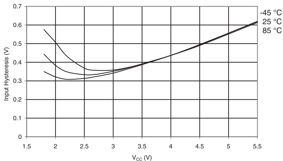
Figure 29-36. ATmega169PA: I/O Pin Input Hysteresis vs. V_{CC}
