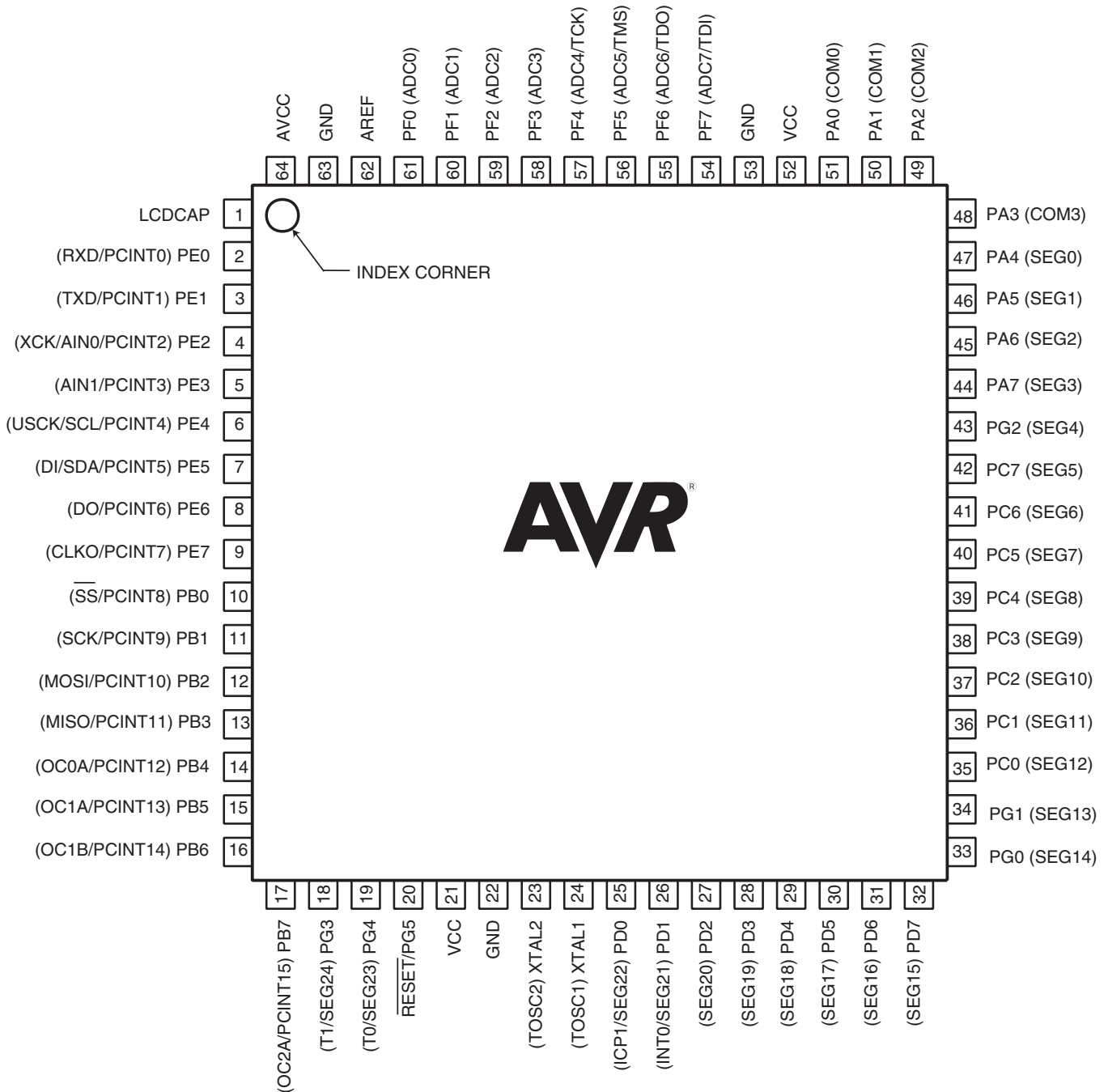
Figure 1-1. MLF/ Pinout ATmega169PA/329P/649P
