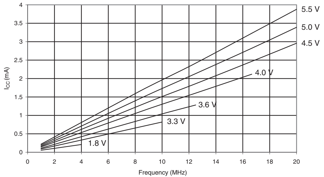
Figure 29-118. ATmega329P: Reset Supply Current vs. Frequency (1 - 20MHz)
