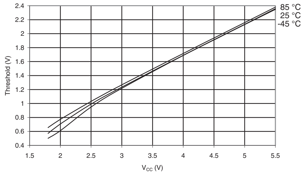
Figure 29-210. ATmega649P: I/O Pin Input Threshold Voltage vs. V_{CC} , Port B ( V_{IL} , IO Pin Read as "0")
