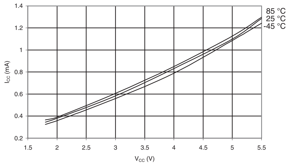
Figure 29-237. ATmega6490P: Active Supply Current vs. V_{CC} (Internal RC Oscillator, 1MHz)
