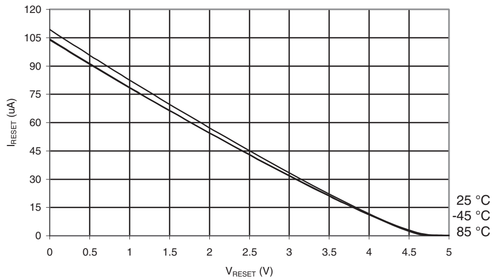
Figure 29-253. ATmega6490P: Reset Pull-up Resistor Current vs. Reset Pin Voltage ( V_{CC} = 5V )
