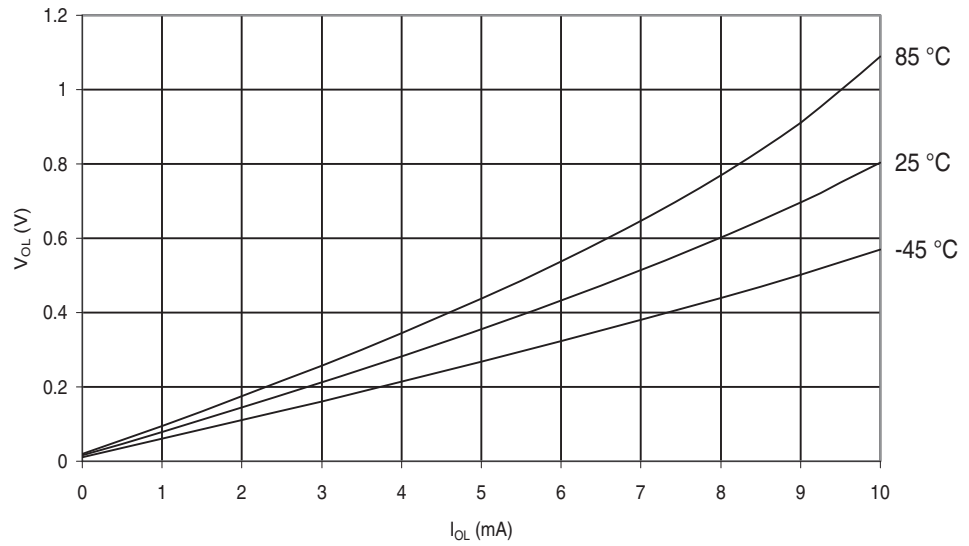
Figure 29-258. ATmega6490P: I/O Pin Output Voltage vs. Sink Current, Port A,C,D,E,F,G ( V_{CC}=2.7V )
