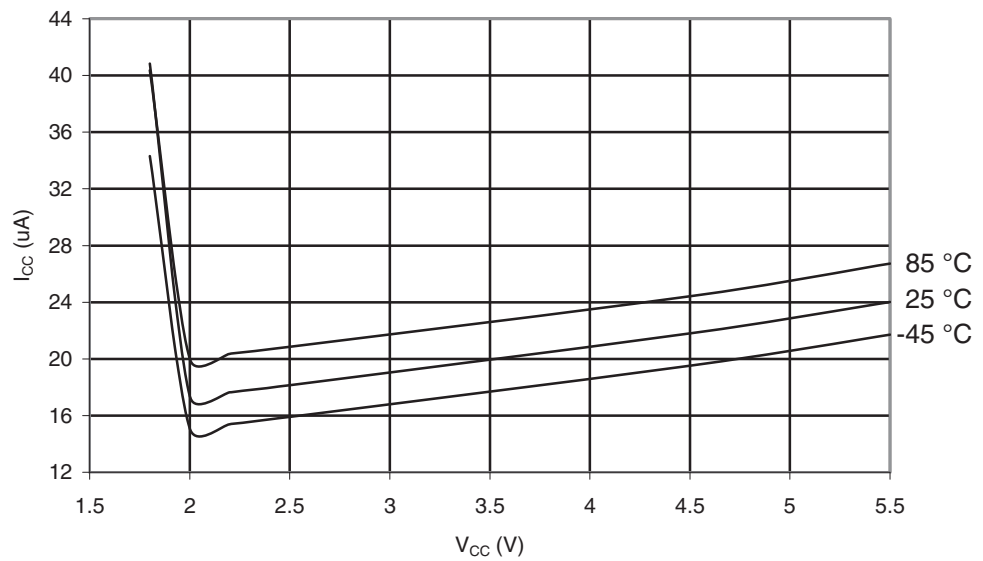
Figure 29-52. ATmega169PA: Brownout Detector Current vs. V_{CC}
