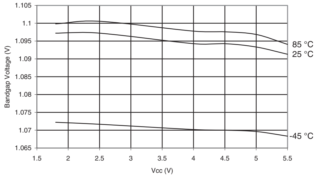
Figure 29-43. ATmega169PA: Bandgap Voltage vs. V_{CC}
