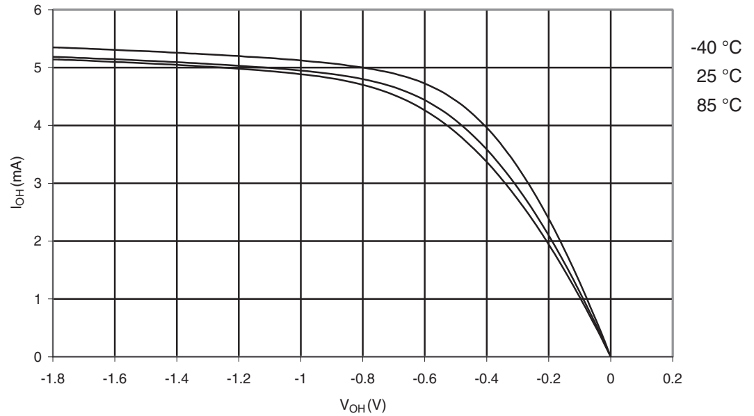
Figure 29-148. ATmega3290P: I/O Pin Source Current vs. Output Voltage, Port A,C,D,E,F,G,H,J ( V_{CC}=1.8V )
