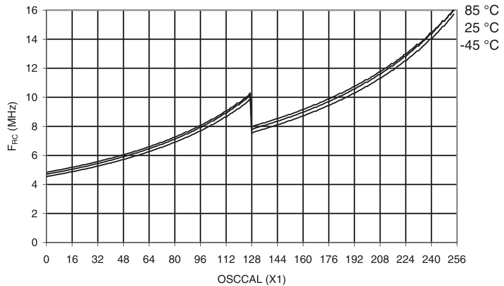
Figure 29-51. ATmega169PA: Calibrated 8MHz RC Oscillator Frequency vs. Oscal Value
