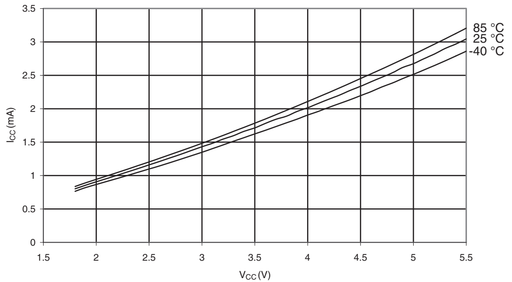
Figure 29-70. ATmega329P: Idle Supply Current vs. V_{CC} (Internal RC Oscillator, 8MHz)
