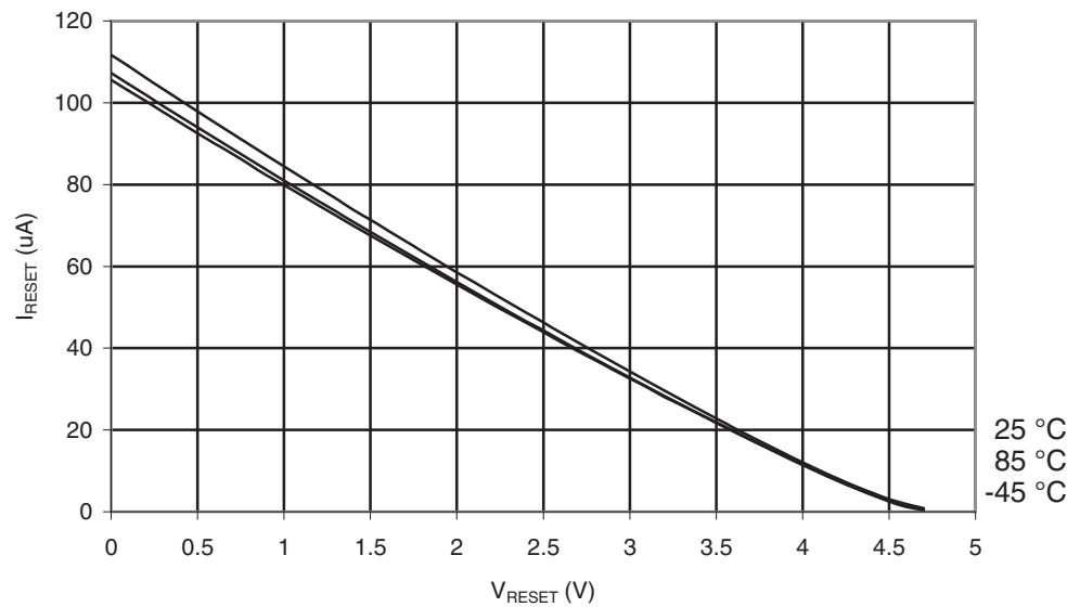
Figure 29-19. ATmega169PA: Reset Pull-up Resistor Current vs. Reset Pin Voltage ( V_{CC} = 5V )
