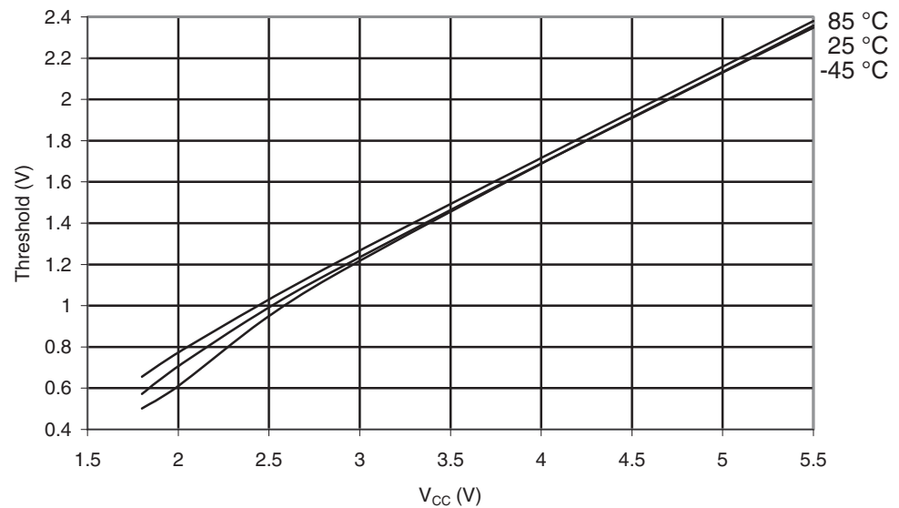
Figure 29-267. ATmega6490P: I/O Pin Input Threshold Voltage vs. V_{CC} , Port B ( V_{IL} , IO Pin Read as "0")
