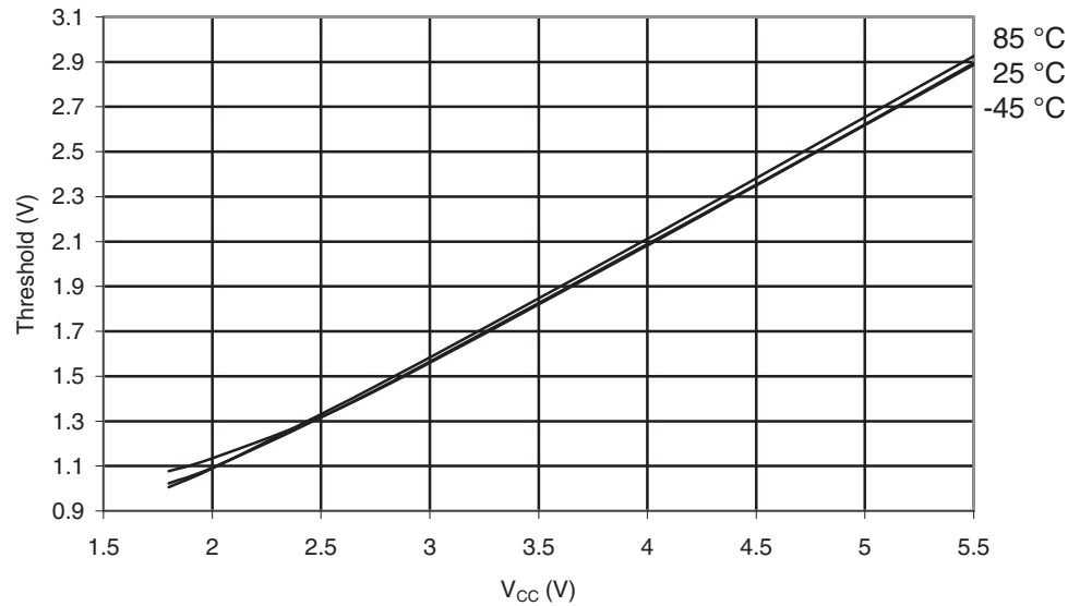
Figure 29-209. ATmega649P: I/O Pin Input Threshold Voltage vs. V_{CC} , ( V_{IH} , IO Pin Read as "1")
