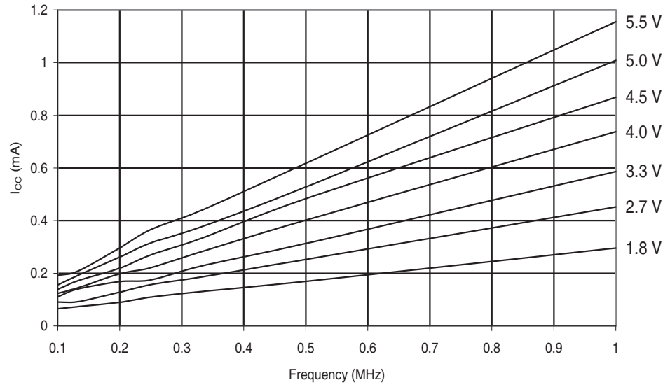
Figure 29-177. ATmega649P: Active Supply Current vs. Low Frequency (0.1 - 1.0MHz)
