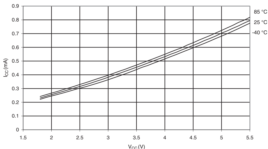
Figure 29-128. ATmega3290P: Idle Supply Current vs. V_{CC} (Internal RC Oscillator, 1MHz)
