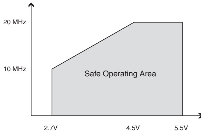
Figure 28-3. Maximum Frequency vs. V_{CC} (10 - 20MHz), ATmega649P/ATmega6490P
