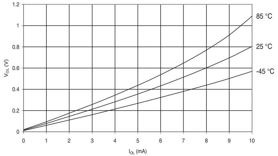
Figure 29-201. ATmega649P: I/O Pin Output Voltage vs. Sink Current, Port A,C,D,E,F,G ( V_{CC}=2.7V )
