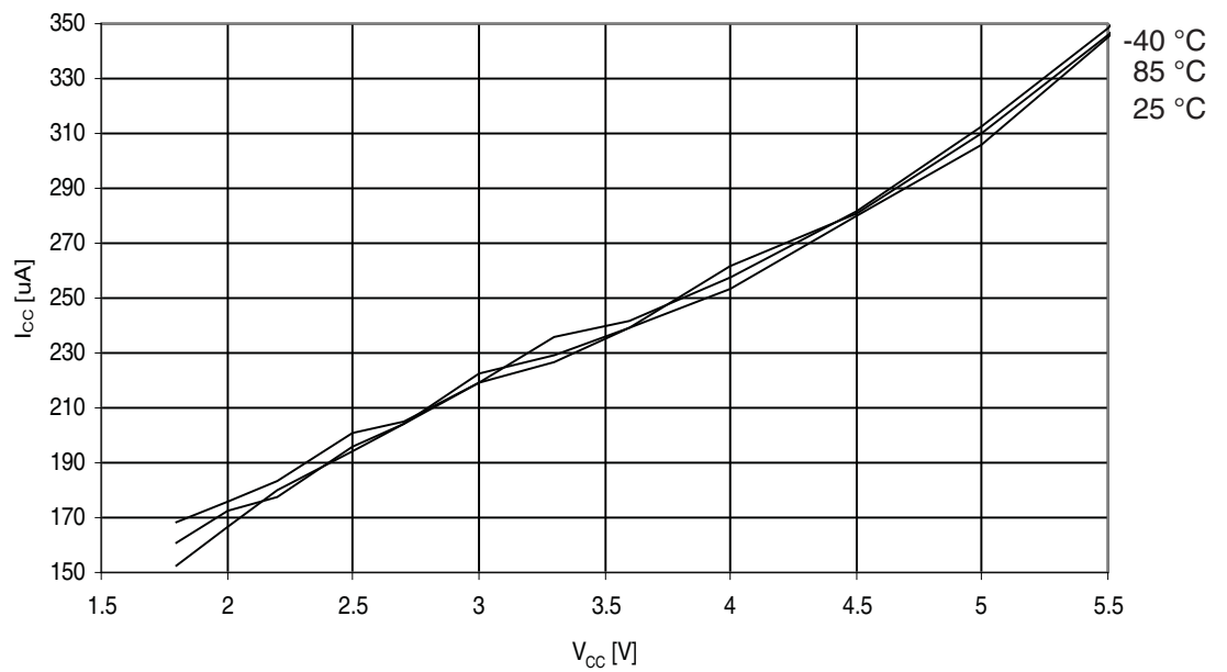
Figure 29-110. ATmega329P: Active Supply Current with ADC at 200kHz vs. V_{CC}
