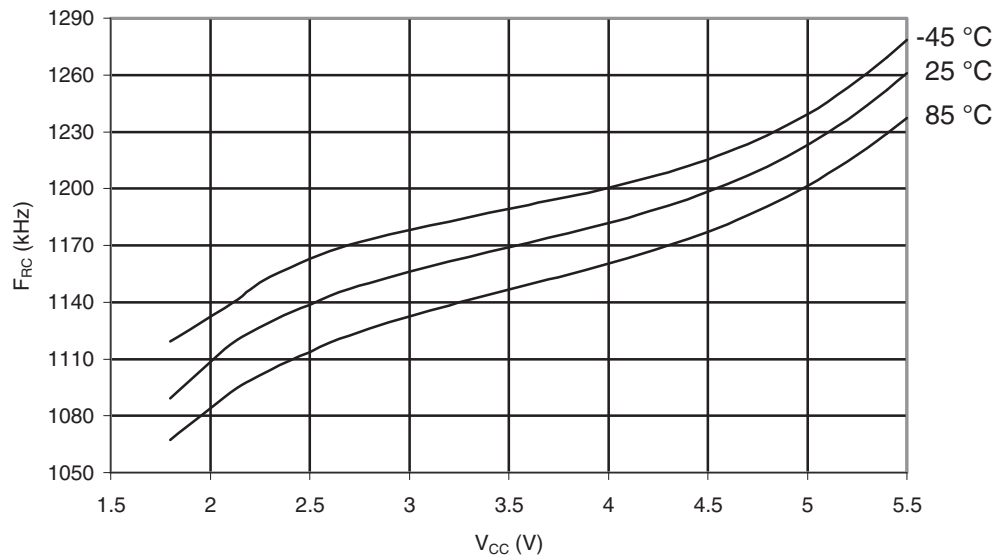
Figure 29-218. ATmega649P: Watchdog Oscillator Frequency vs. V_{CC}
