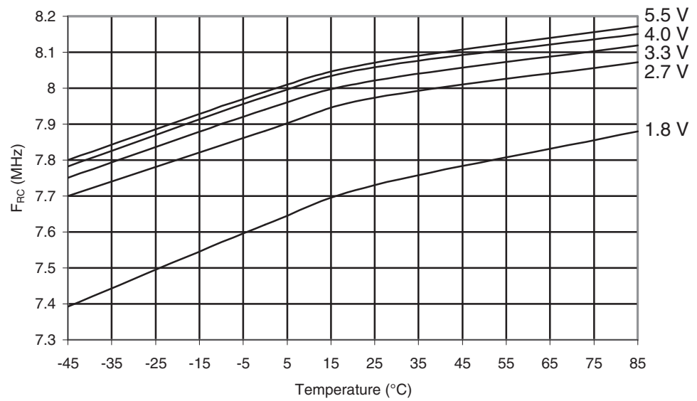
Figure 29-278. ATmega6490P: Calibrated 8MHz RC Oscillator Frequency vs. Temperature
