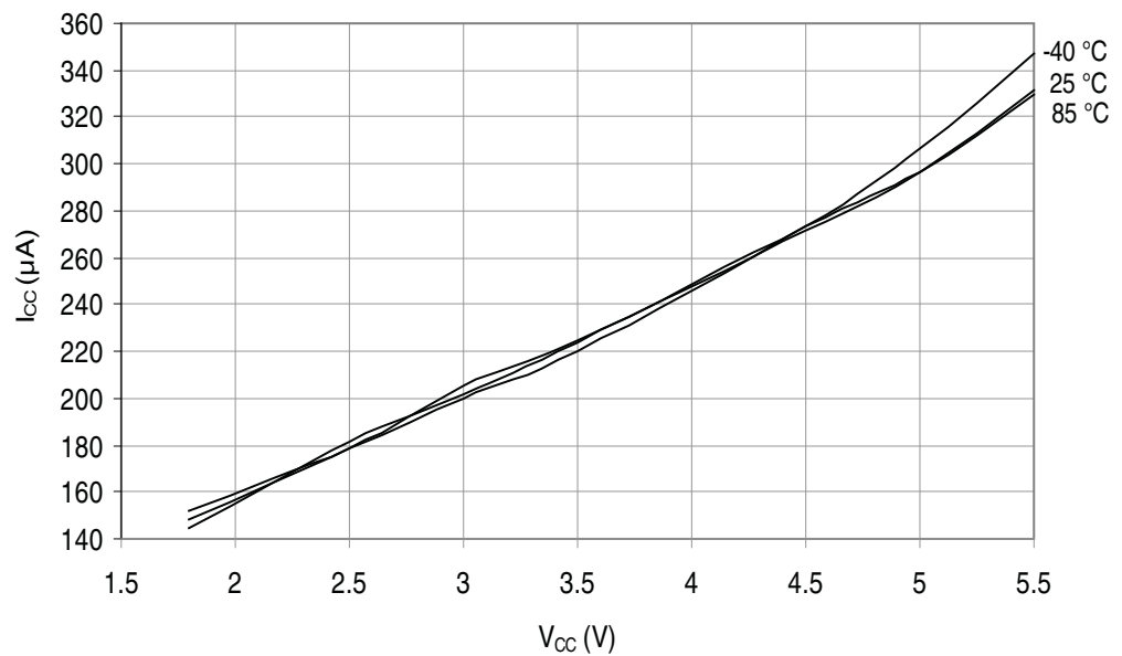
Figure 29-169. ATmega3290P: ADC Current vs. V_{CC} ( A_{REF} = AV_{CC} )
