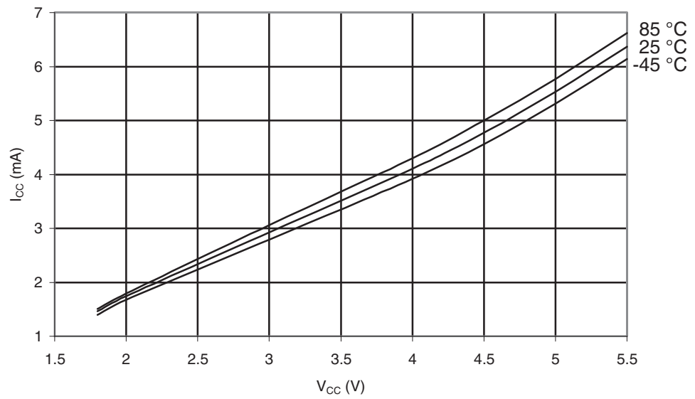
Figure 29-179. ATmega649P: Active Supply Current vs. V_{CC} (Internal RC Oscillator, 8MHz)
