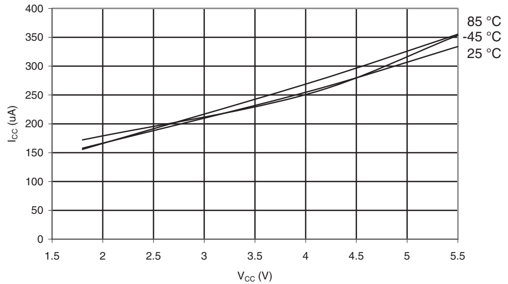
Figure 29-54. ATmega169PA: Active Supply Current with ADC at 200kHz vs. V_{CC}
