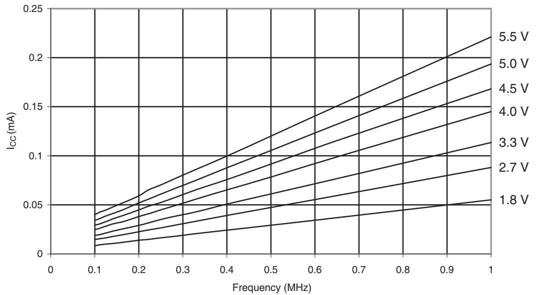
Figure 29-117. ATmega329P: Reset Supply Current vs. Low Frequency (0.1 - 1.0MHz)
