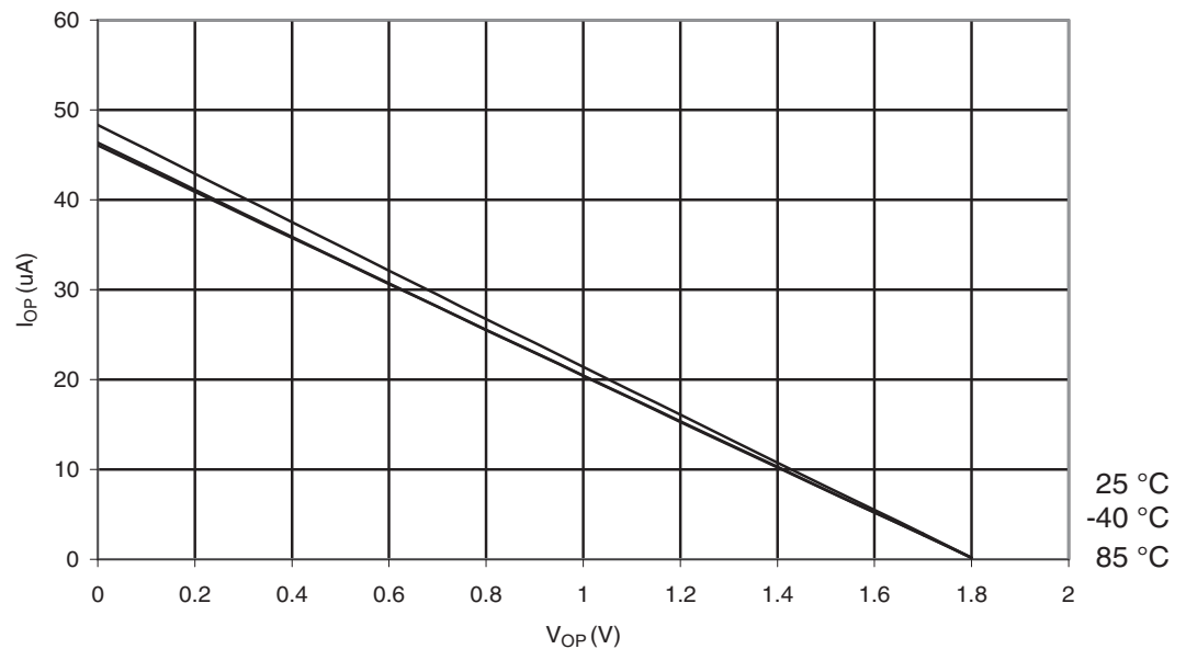
Figure 29-133. ATmega3290P: I/O Pin Pull-up Resistor Current vs. Input Voltage ( V_{CC} = 1.8V )
