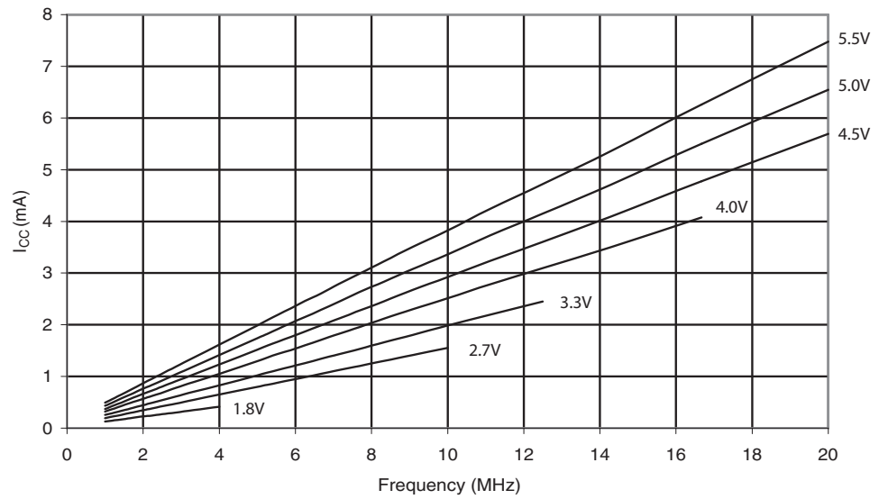
Figure 29-69. ATmega329P: Idle Supply Current vs. Frequency (1 - 20MHz)
