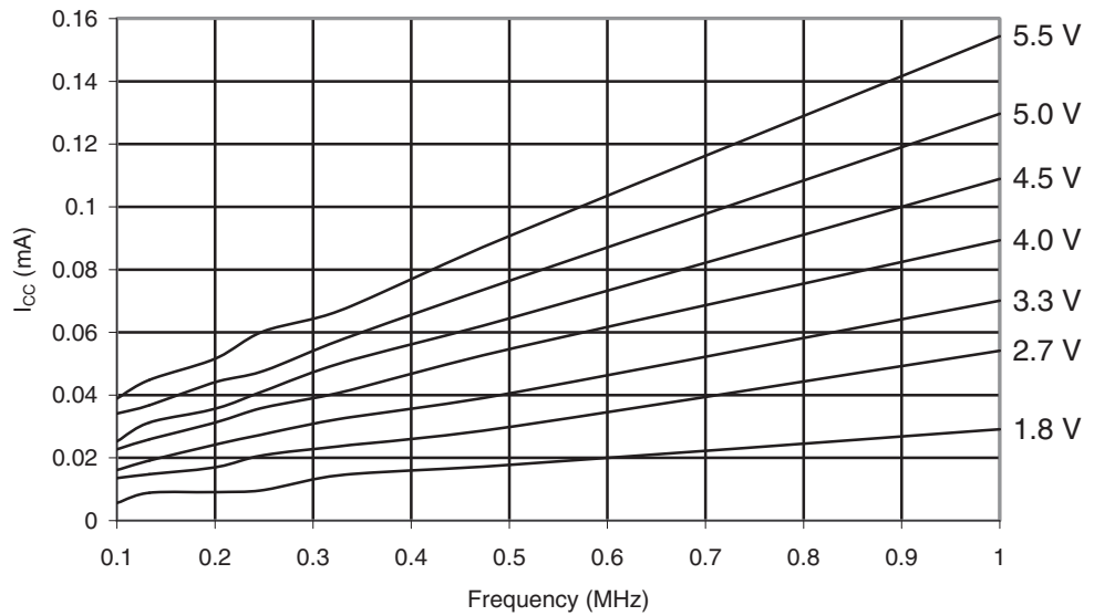
Figure 29-60. ATmega169PA: Reset Supply Current vs. V_{CC} (0.1 - 1.0MHz, Excluding Current Through The Reset Pull-up)
