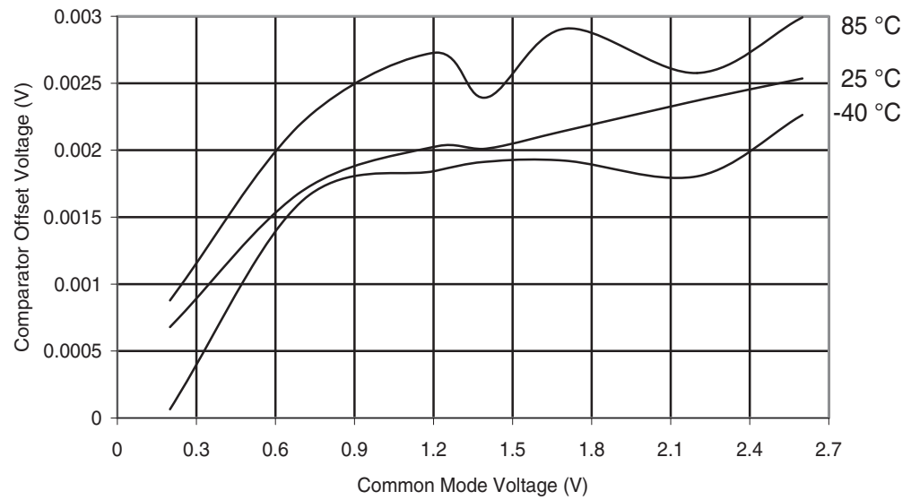
Figure 29-46. ATmega169PA: Analog Comparator Offset Voltage vs. Common Mode Voltage ( V_{CC} = 2.7V )
