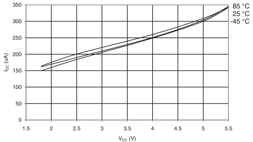
Figure 29-53. ATmega169PA: Active Supply Current with ADC at 50kHz vs. V_{CC}
