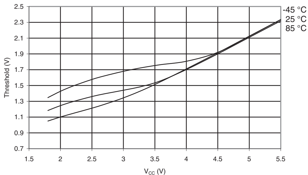
Figure 29-37. ATmega169PA: Reset Input Threshold Voltage vs. V_{CC} ( V_{IH} , Reset Pin Read as “1”)
