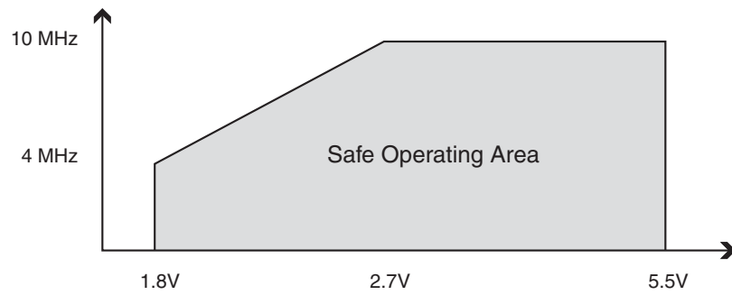
Figure 28-2. Maximum Frequency vs. V_{CC} (4 - 10MHz), ATmega649P/ATmega6490P
