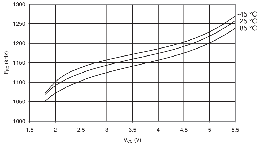
Figure 29-160. ATmega3290P: Watchdog Oscillator Frequency vs. V_{CC}
