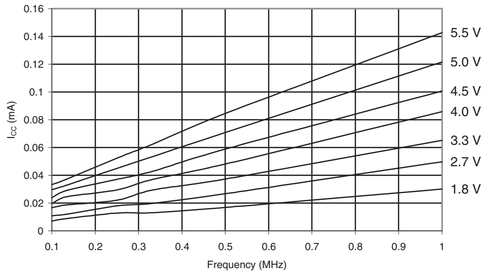
Figure 29-231. ATmega649P: Reset Supply Current vs. Low Frequency (0.1 - 1.0MHz)
