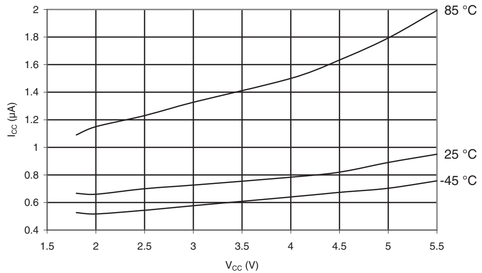
Figure 29-14. ATmega169PA: Standby Supply Current vs. V_{CC} (32kHz Watch Crystal, Watchdog Timer Disabled)
