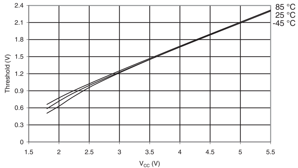
Figure 29-35. ATmega169PA: I/O Pin Input Threshold Voltage vs. V_{CC} ( V_{IL} , I/O Pin Read as “0”)
