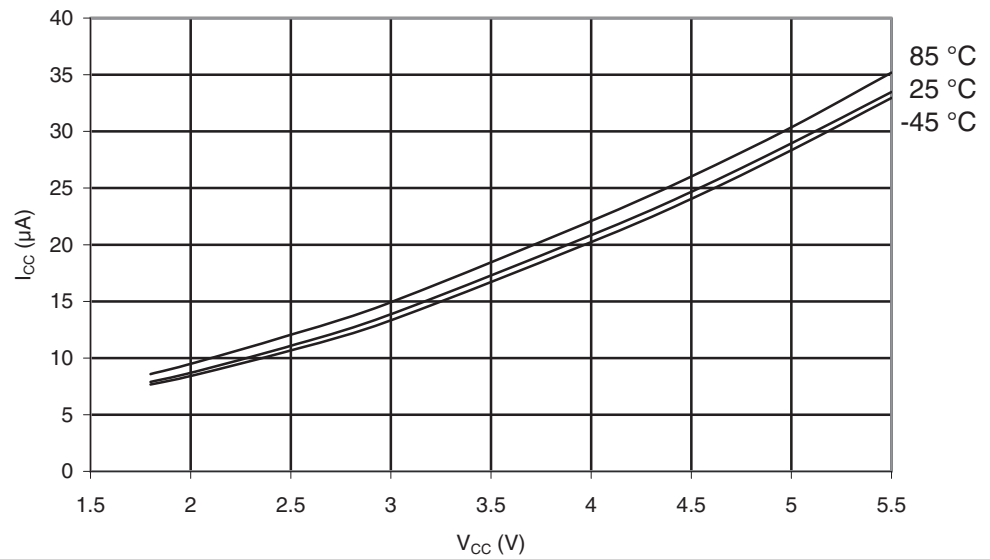
Figure 29-5. ATmega169PA: Active Supply Current vs. V_{CC} (32kHz Watch Crystal)
