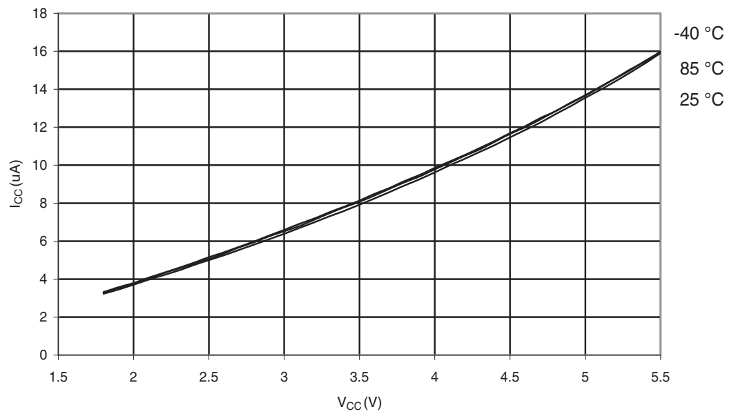
Figure 29-114. ATmega329P: Watchdog Timer Current vs. V_{CC}
