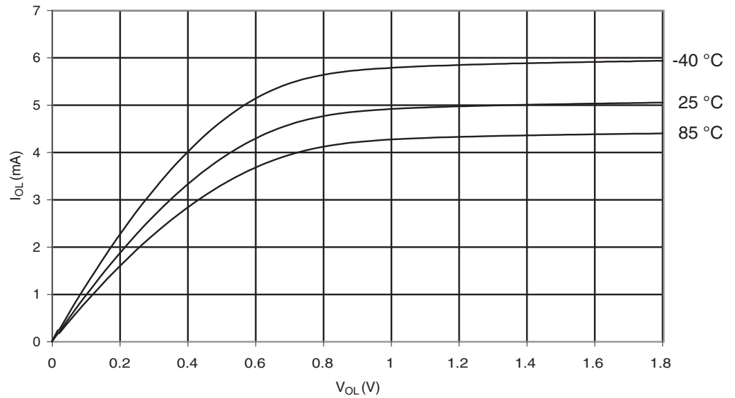
Figure 29-142. ATmega3290P: I/O Pin Sink Current vs. Output Voltage, Port A,C,D,E,F,G,H,J ( V_{CC}=1.8V )
