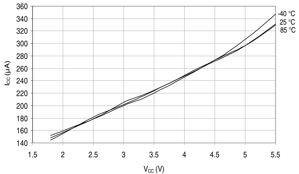
Figure 29-112. ATmega329P: ADC Current vs. V_{CC} (AREF = AV_{CC} )
