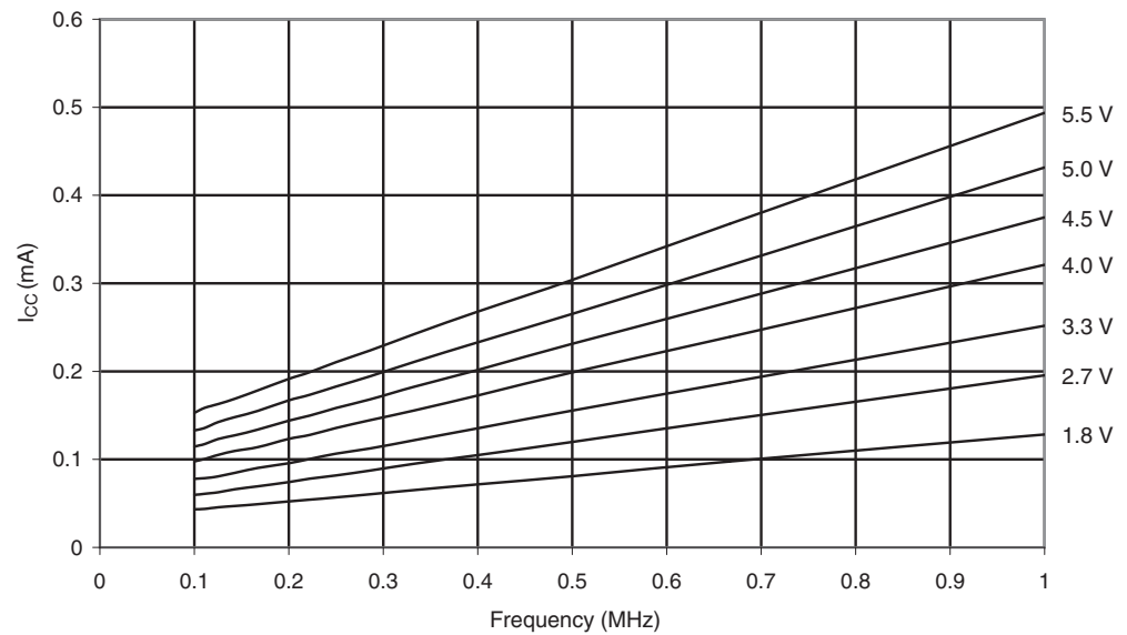
Figure 29-68. ATmega329P: Idle Supply Current vs. Low Frequency (0.1 - 1.0MHz)
