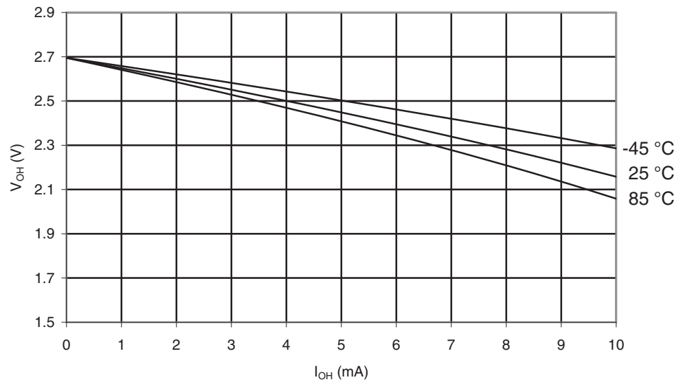
Figure 29-23. ATmega169PA: I/O Pin Output Voltage vs. Source Current, Ports A, C, D, E, F, G ( V_{CC} = 2.7V )
