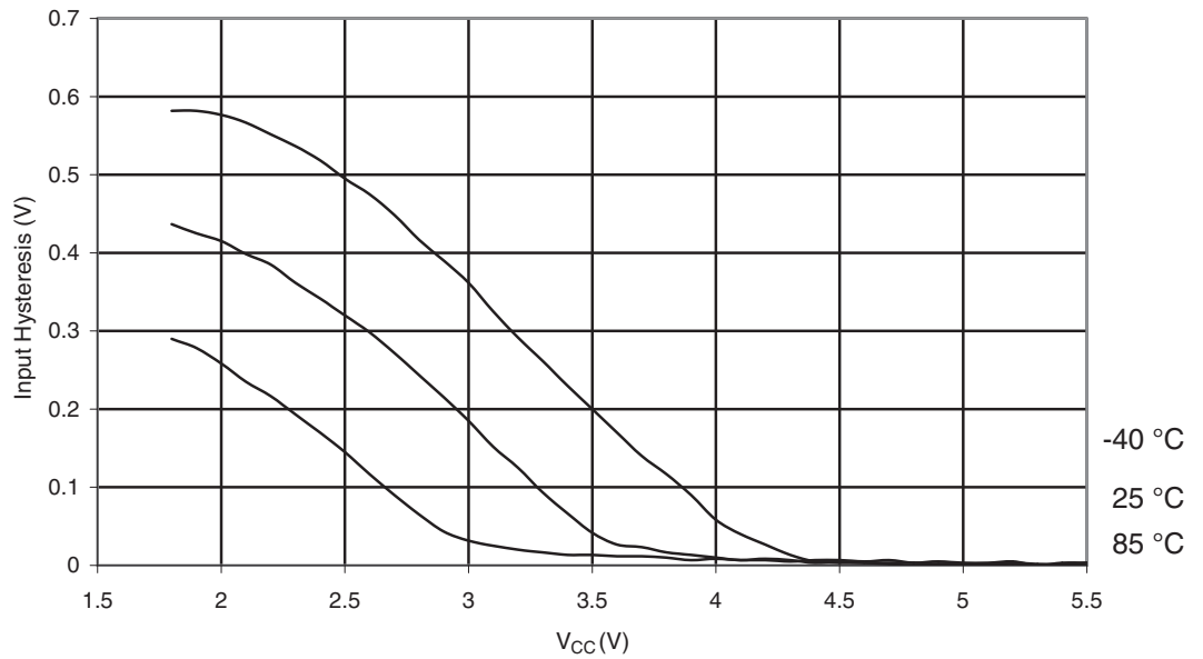
Figure 29-159. ATmega3290P: Reset Pin Input Hysteresis vs. V_{CC}
