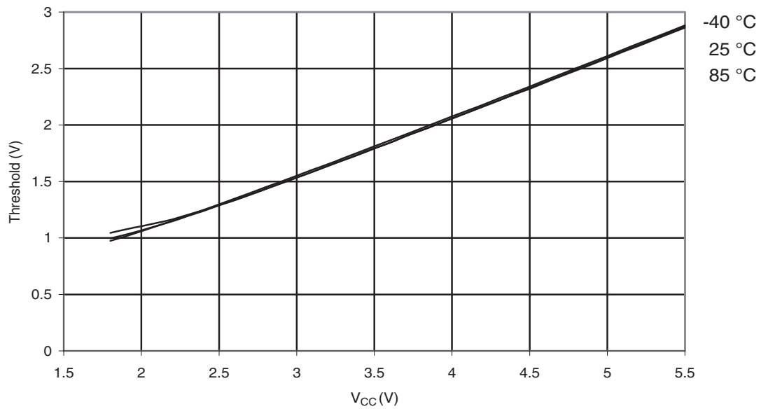
Figure 29-94. ATmega329P: I/O Pin Input Threshold Voltage vs. V_{CC} , Port B ( V_{IH} , IO Pin Read as "1")
