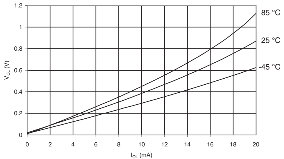
Figure 29-198. ATmega649P: I/O Output Voltage vs. Pin Sink Current, Port B ( V_{CC} = 2.7V )
