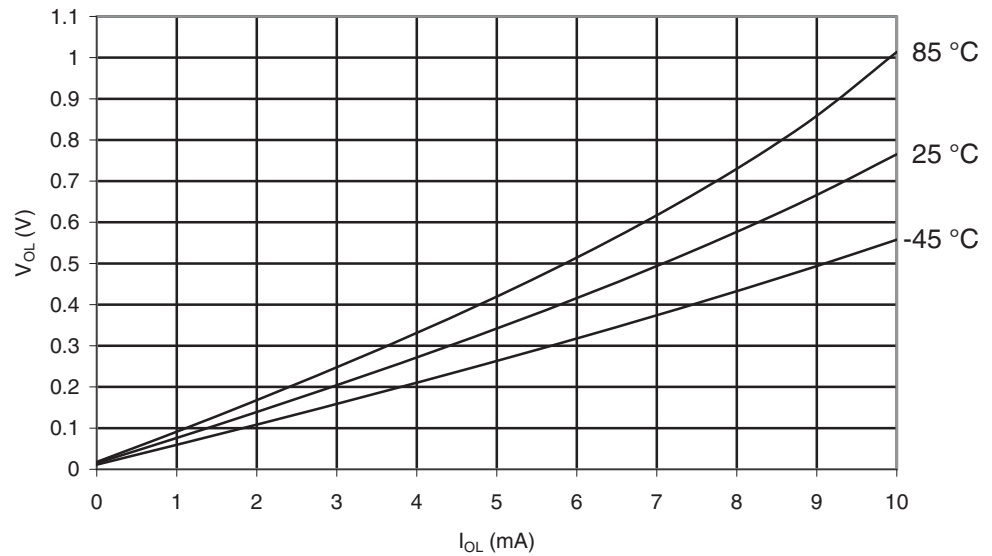
Figure 29-28. ATmega169PA: I/O Pin Output Voltage vs. Sink Current, Ports A, C, D, E, F, G ( V_{CC} = 5V )
