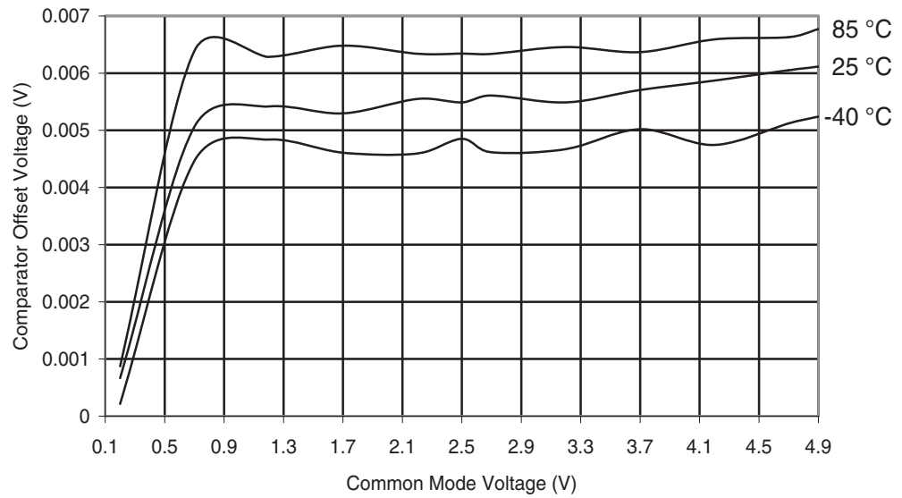
Figure 29-45. ATmega169PA: Analog Comparator Offset Voltage vs. Common Mode Voltage ( V_{CC} = 5V )
