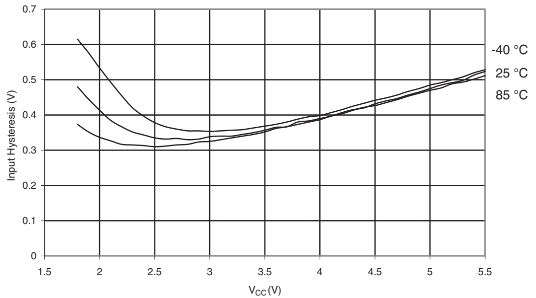
Figure 29-156. ATmega3290P: I/O Pin Hysteresis vs. V_{CC} , Port A,C,D,E,F,G,H,J
