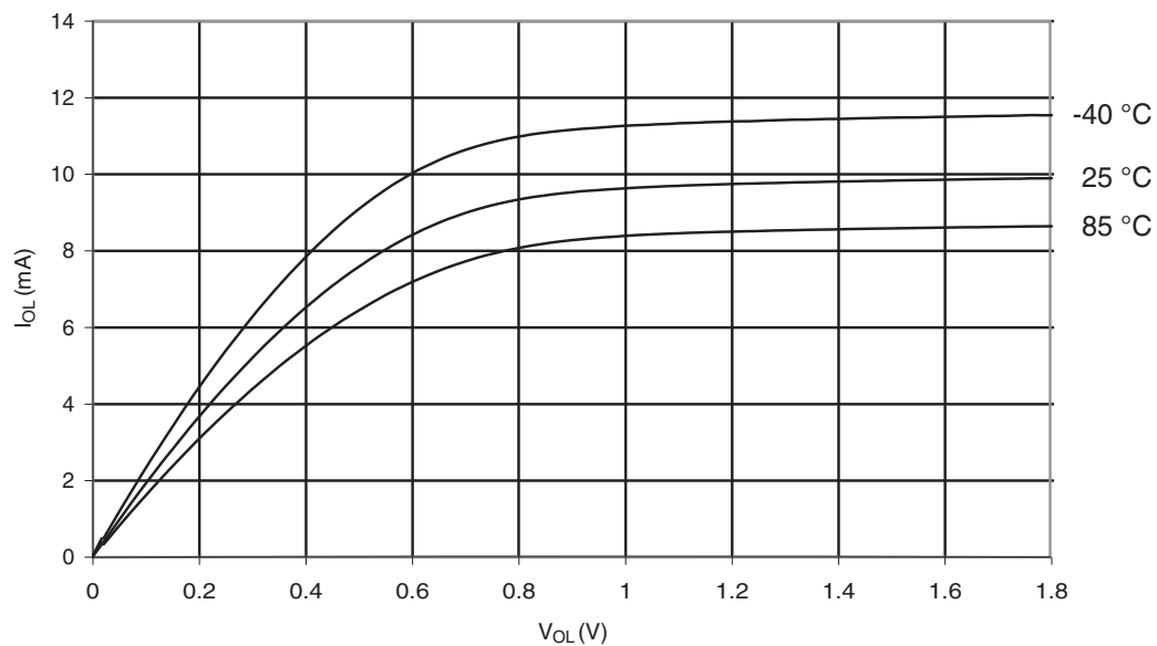
Figure 29-82. ATmega329P: I/O Pin Sink Current vs. Output Voltage, Port B ( V_{CC} = 1.8V )
