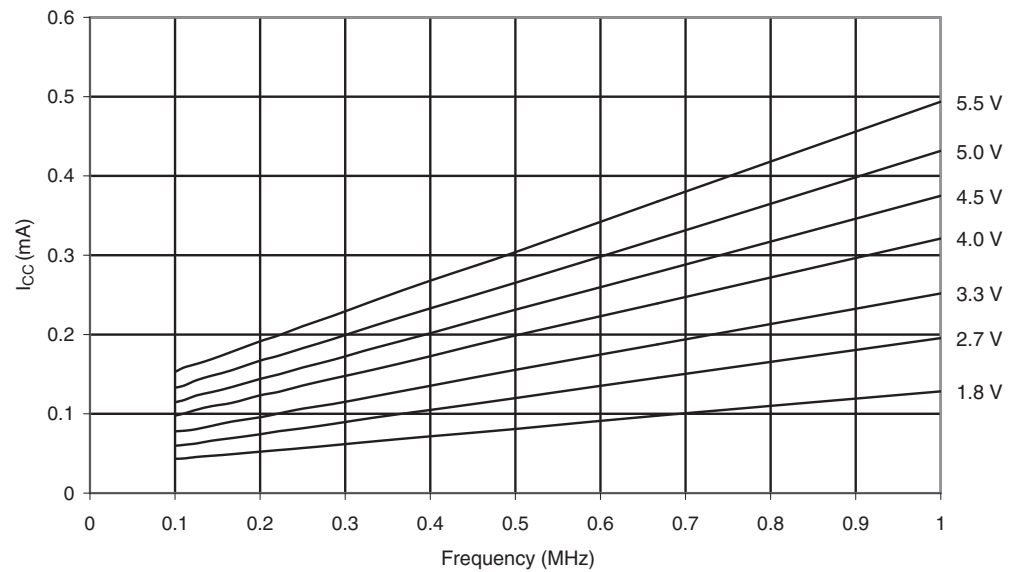
Figure 29-125. ATmega3290P: Idle Supply Current vs. Low Frequency (0.1 - 1.0MHz)
