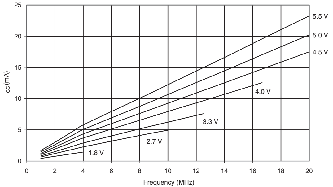
Figure 29-64. ATmega329P: Active Supply Current vs. Frequency (1 - 20MHz)
