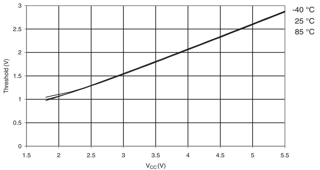
Figure 29-151. ATmega3290P: I/O Pin Input Threshold Voltage vs. V_{CC} , Port B ( V_{IH} , IO Pin Read as "1")
