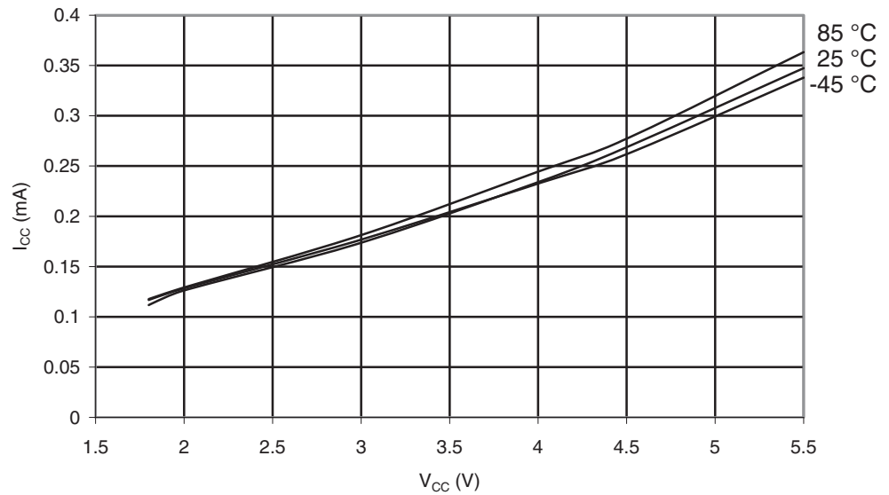
Figure 29-9. ATmega169PA: Idle Supply Current vs. V_{CC} (Internal RC Oscillator, 1MHz)
