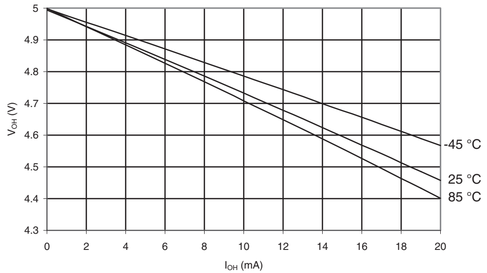
Figure 29-205. ATmega649P: I/O Pin Output Voltage vs. Source Current, Port B ( V_{CC} = 5V )
