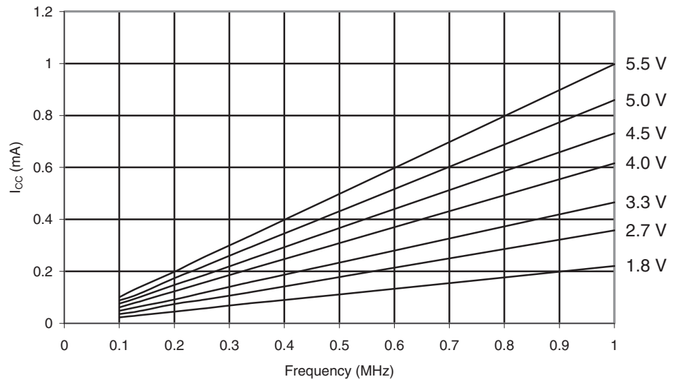
Figure 29-1. ATmega169PA: Active Supply Current vs. Frequency (0.1 - 1.0MHz)
