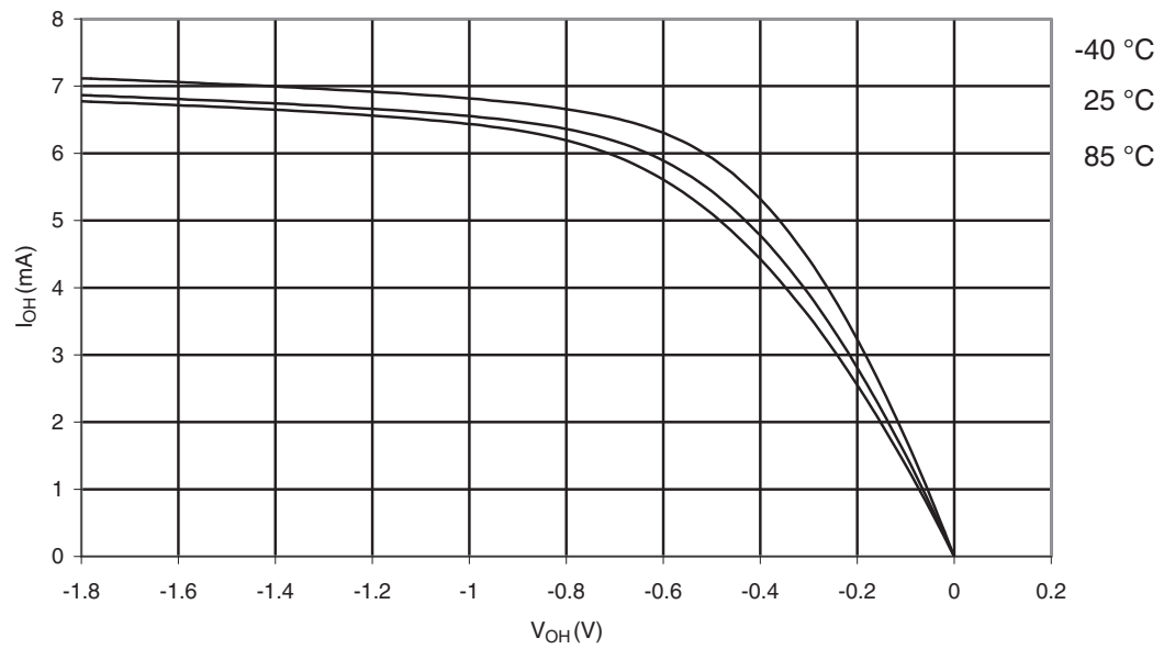
Figure 29-145. ATmega3290P: I/O Pin Source Current vs. Output Voltage, Port B ( V_{CC}=1.8V )
