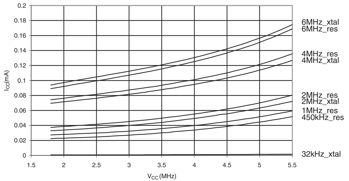
Figure 29-132. ATmega3290P: Standby Supply Current vs. V_{CC} (Watchdog Timer Disabled)
