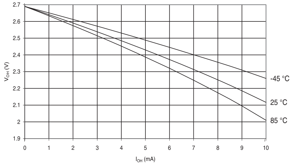
Figure 29-207. ATmega649P: I/O Pin Output Voltage vs. Source Current, Port A,C,D,E,F,G ( V_{CC}=2.7V )
