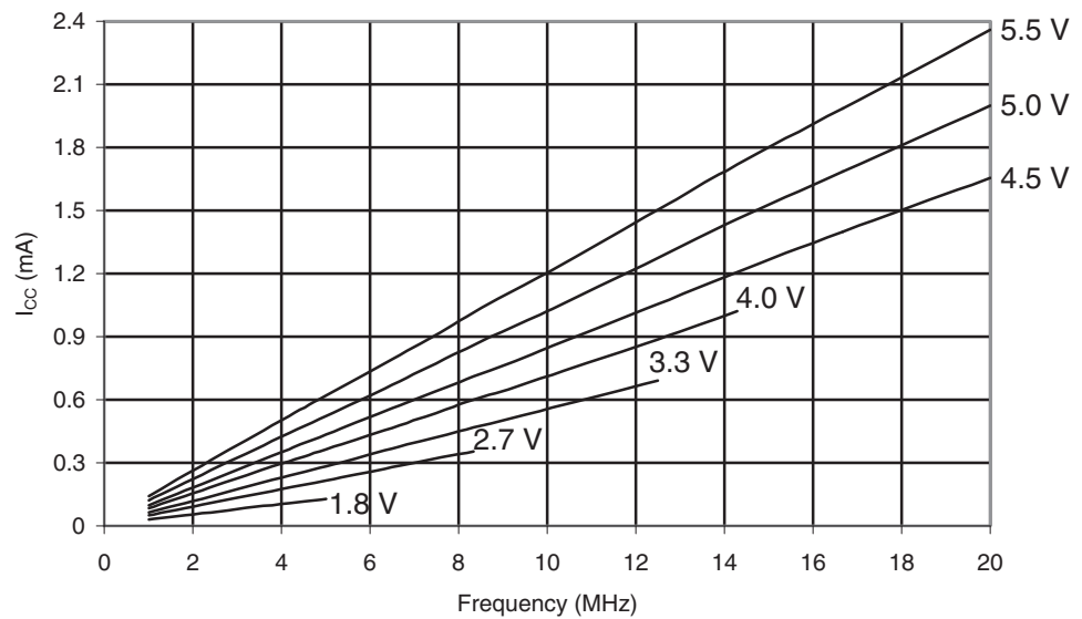
Figure 29-232. ATmega649P: Reset Supply Current vs. Frequency (1 - 20MHz)
