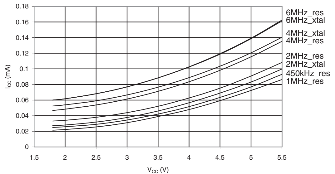
Figure 29-15. ATmega169PA: Standby Supply Current vs. V_{CC} (Xtall and Resonator, Watchdog Timer Disabled)
