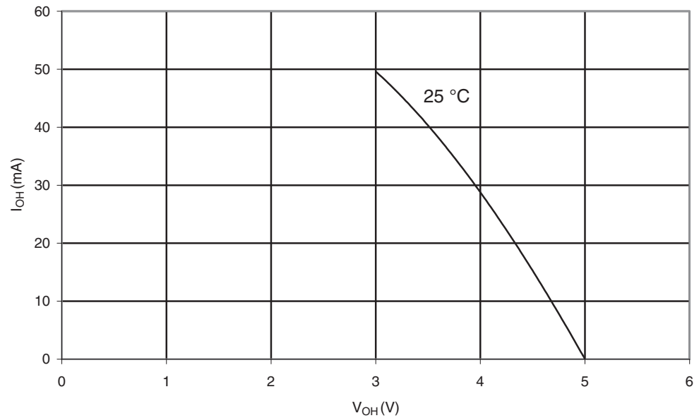
Figure 29-150. ATmega3290P: I/O Pin Source Current vs. Output Voltage, Port A,C,D,E,F,G,H,J ( V_{CC}=5V )
