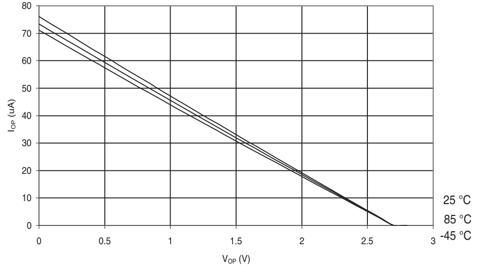
Figure 29-249. ATmega6490P: I/O Pin Pull-up Resistor Current vs. Input Voltage ( V_{CC} = 2.7V )
