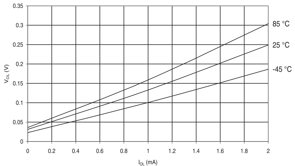
Figure 29-257. ATmega6490P: I/O Pin Output Voltage vs. Sink Current, Port A,C,D,E,F,G ( V_{CC} = 1.8V )
