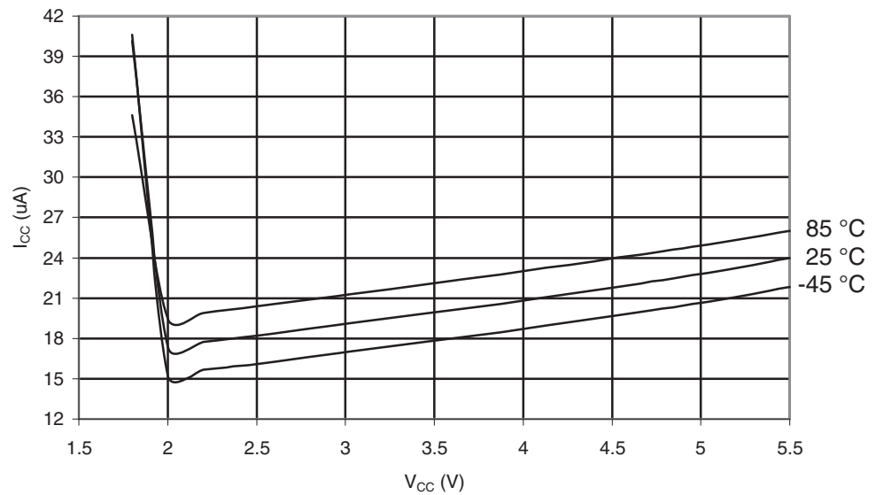
Figure 29-223. ATmega649P: Brownout Detector Current vs. V_{CC}
