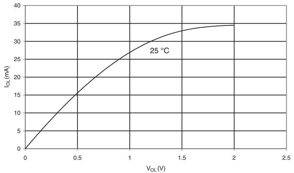
Figure 29-83. ATmega329P: I/O Pin Sink Current vs. Output Voltage, Port B ( V_{CC} = 2.7\text{ V} )
