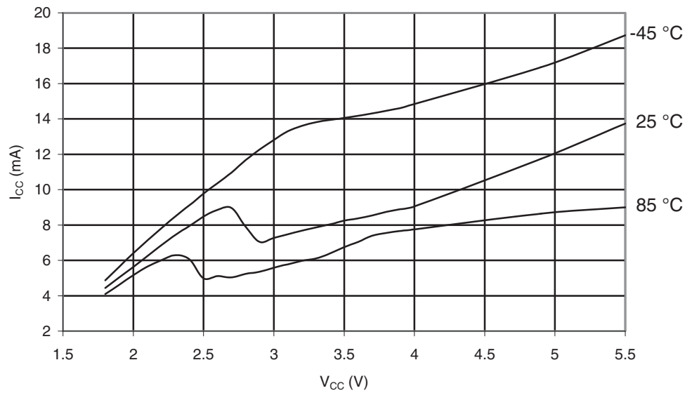
Figure 29-230. ATmega649P: Programming Current vs. V_{CC}
