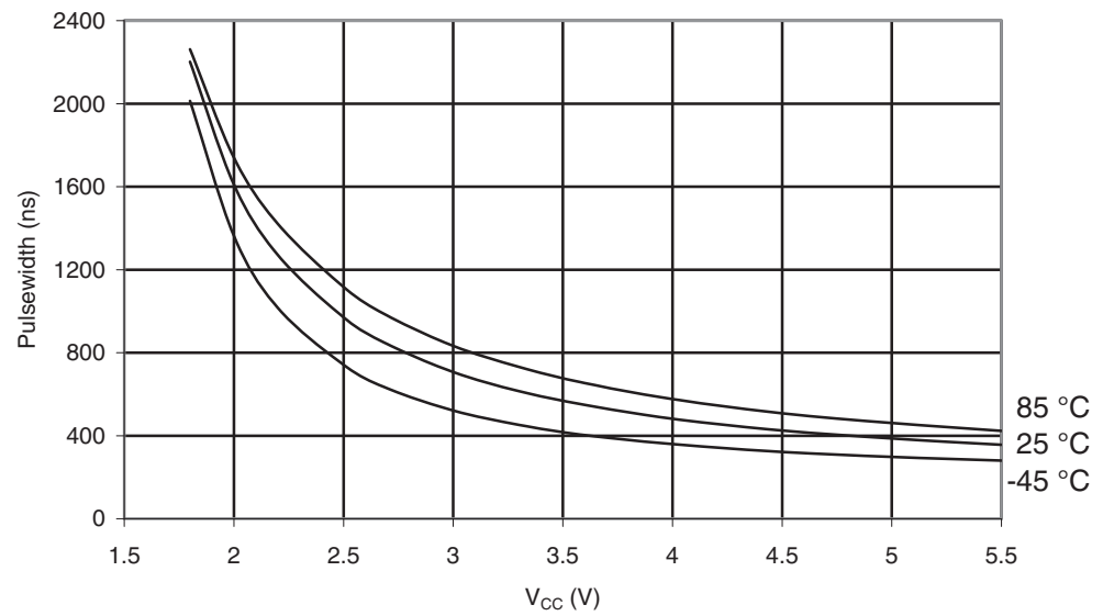
Figure 29-62. ATmega169PA: Minimum Reset Pulse Width vs. V_{CC}
