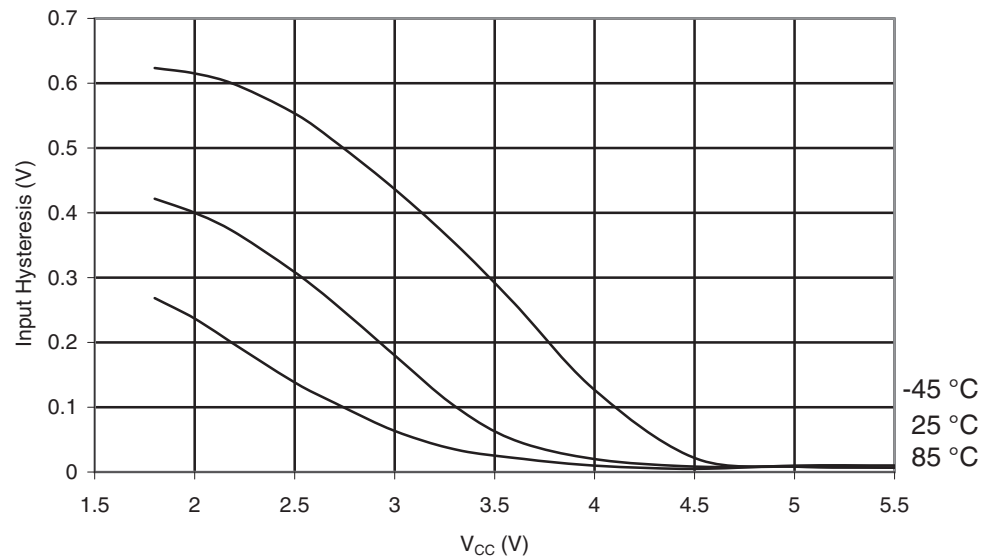
Figure 29-39. ATmega169PA: Reset Input Pin Hysteresis vs. V_{CC}
