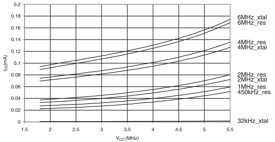
Figure 29-75. ATmega329P: Standby Supply Current vs. V_{CC} (Watchdog Timer Disabled)
