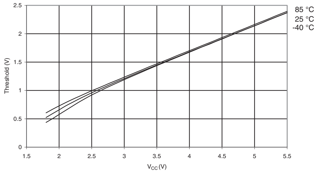
Figure 29-155. ATmega3290P: I/O Pin Input Threshold Voltage vs. V_{CC} , Port A,C,D,E,F,G,H,J ( V_{IL} , IO Pin Read as "0")
