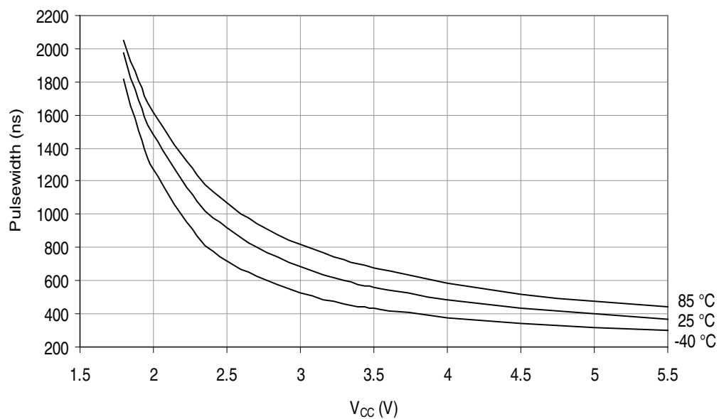
Figure 29-119. ATmega329P: Minimum Reset Pulse Width vs. V_{CC}
