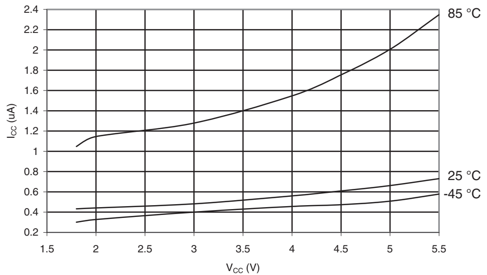
Figure 29-244. ATmega6490P: Power-down Supply Current vs. V_{CC} (Watchdog Timer Disabled)
