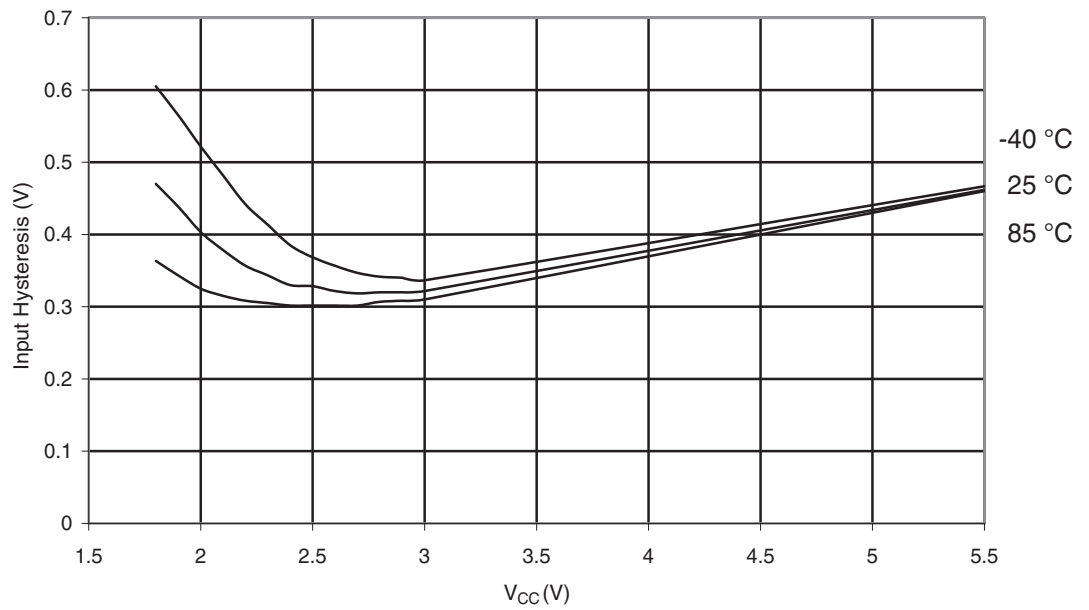
Figure 29-153. ATmega3290P: I/O Pin Input Hysteresis vs. V_{CC} , Port B
