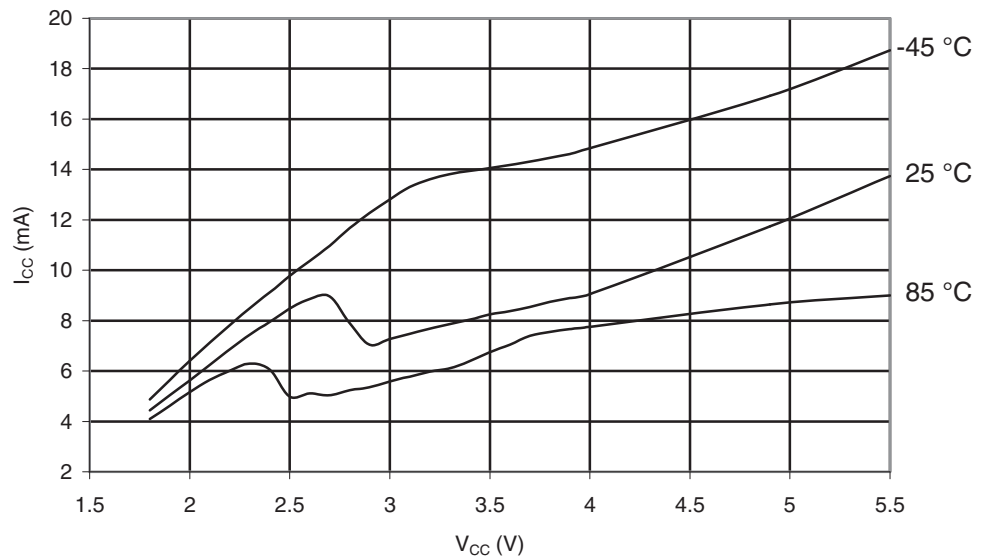
Figure 29-287. ATmega6490P: Programming Current vs. V_{CC}
