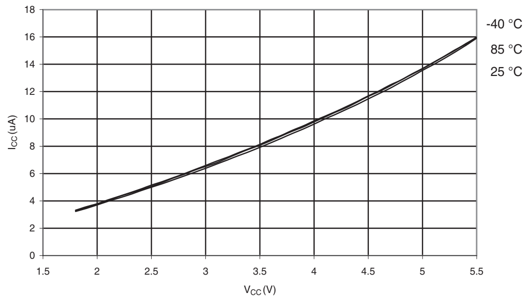
Figure 29-171. ATmega3290P: Watchdog Timer Current vs. V_{CC}
