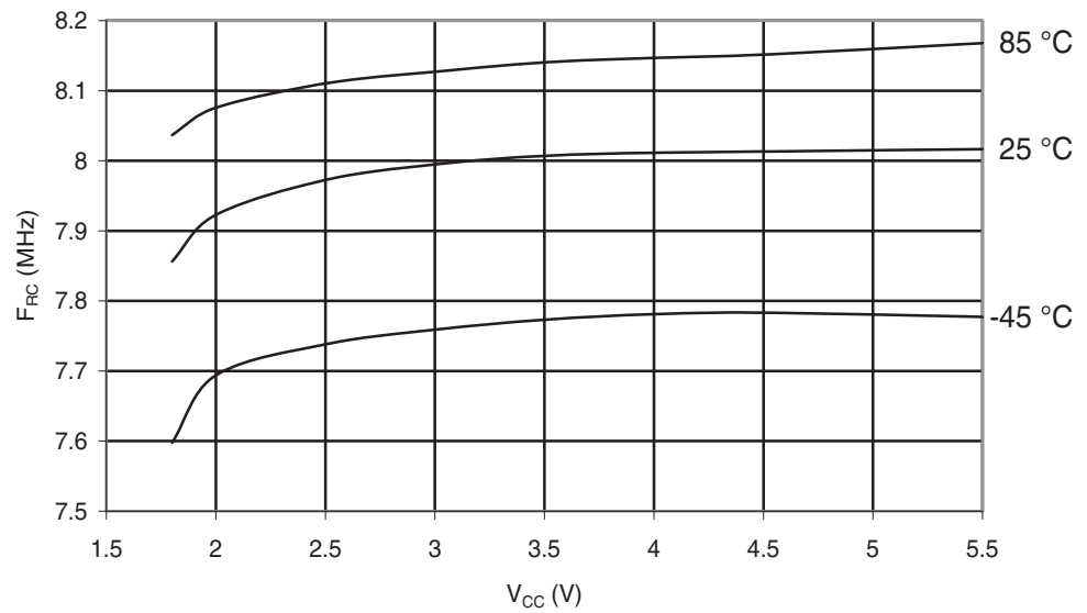
Figure 29-50. ATmega169PA: Calibrated 8MHz RC Oscillator Frequency vs. V_{CC}
