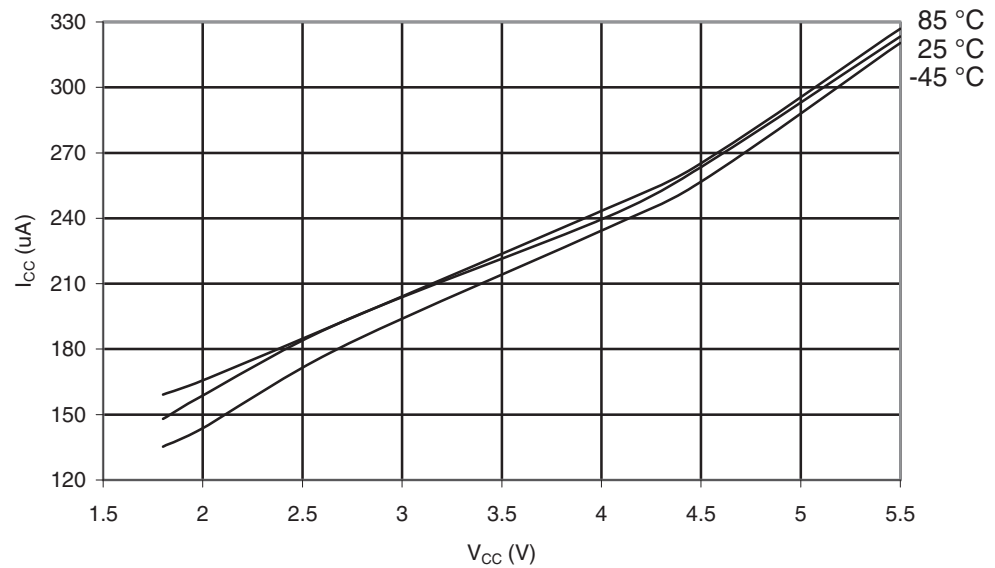
Figure 29-224. ATmega649P: Active Supply Current with ADC at 50kHz vs. V_{CC}
