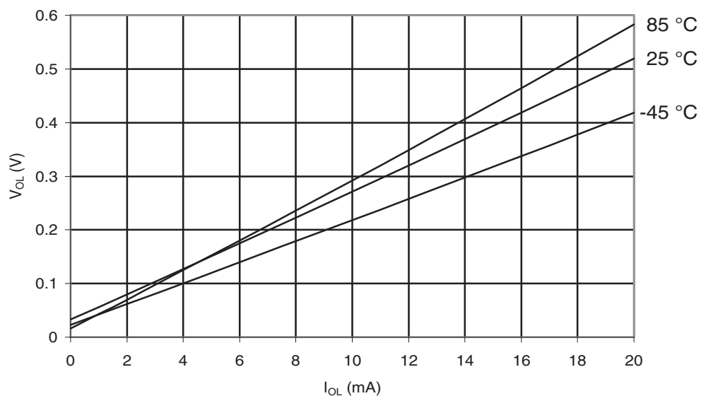
Figure 29-199. ATmega649P: I/O Output Voltage vs. Pin Sink Current, Port B ( V_{CC} = 5V )
