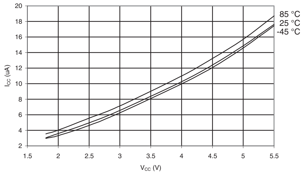
Figure 29-245. ATmega6490P: Power-down Supply Current vs. V_{CC} (Watchdog Timer Enabled)
