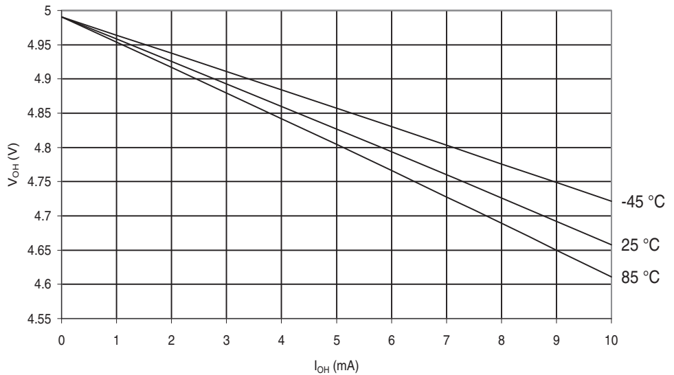
Figure 29-208. ATmega649P: I/O Pin Output Voltage vs. Source Current, Port A,C,D,E,F,G ( V_{CC} = 5V )
