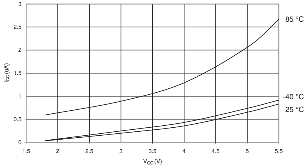
Figure 29-129. ATmega3290P: Power-down Supply Current vs. V_{CC} (Watchdog Timer Disabled)
