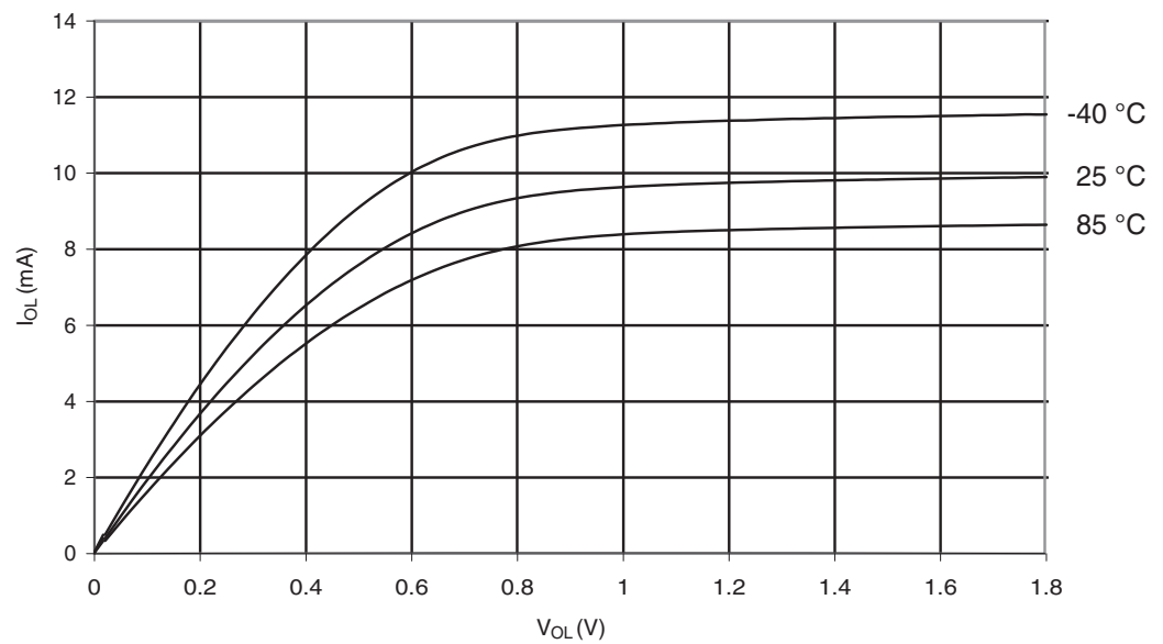
Figure 29-139. ATmega3290P: I/O Pin Sink Current vs. Output Voltage, Port B ( V_{CC} = 1.8V )
