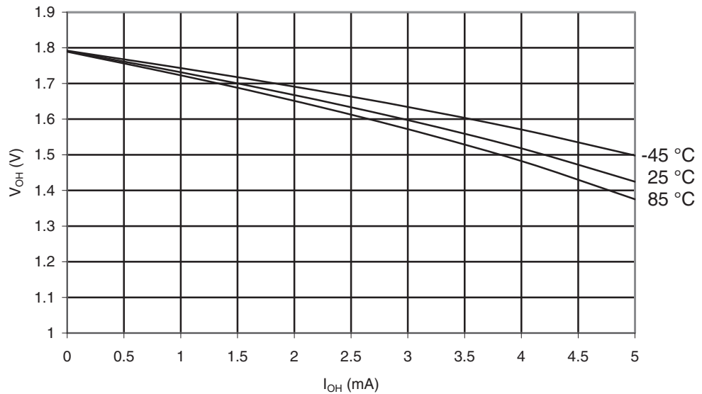
Figure 29-27. ATmega169PA: I/O Pin Output Voltage vs. Source Current, Port B ( V_{CC} = 1.8V )
