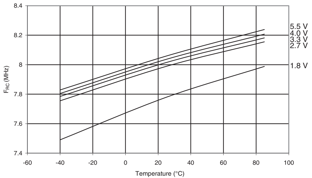
Figure 29-163. ATmega3290P: Calibrated 8MHz RC Oscillator Frequency vs. Temperature
