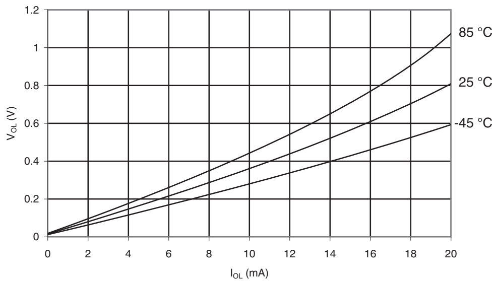
Figure 29-32. ATmega169PA: I/O Pin Output Voltage vs. Sink Current, Port B ( V_{CC} = 2.7V )
