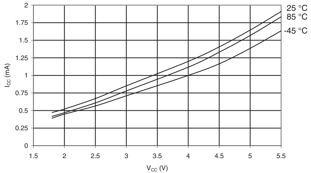
Figure 29-8. ATmega169PA: Idle Supply Current vs. V_{CC} (Internal RC Oscillator, 8MHz)
