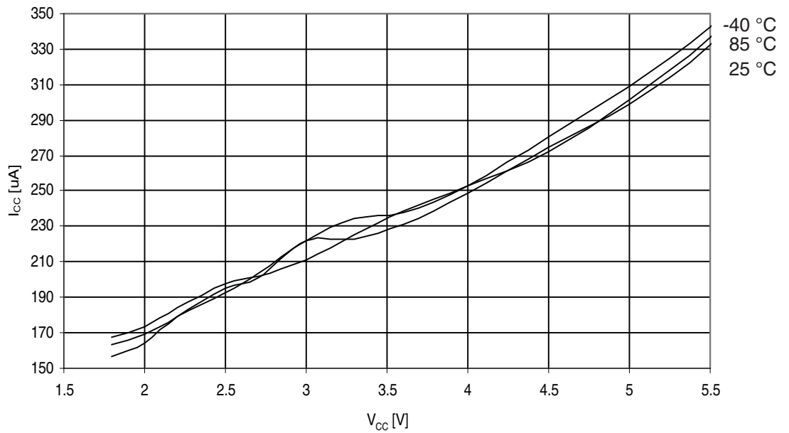
Figure 29-166. ATmega3290P: Active Supply Current with ADC at 50kHz vs. V_{CC}
