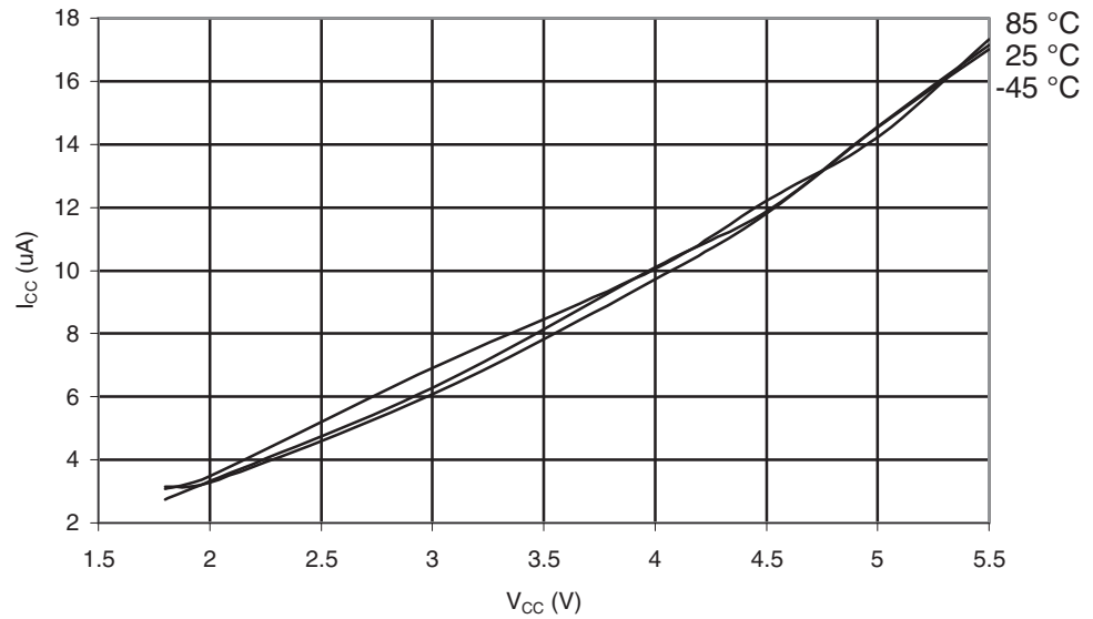
Figure 29-285. ATmega6490P: Watchdog Timer Current vs. V CC
