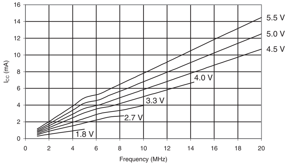
Figure 29-178. ATmega649P: Active Supply Current vs. Frequency (1 - 20MHz)
