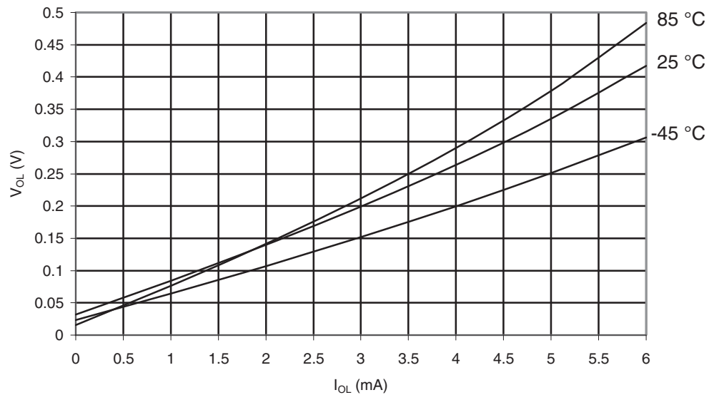
Figure 29-197. ATmega649P: I/O Output Voltage vs., Pin Sink Current Port B ( V_{CC} = 1.8V )
