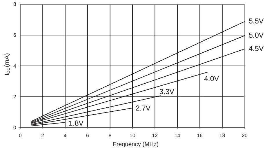
Figure 26-54. Idle Supply Current vs. V_{CC} (1 MHz - 20 MHz).
