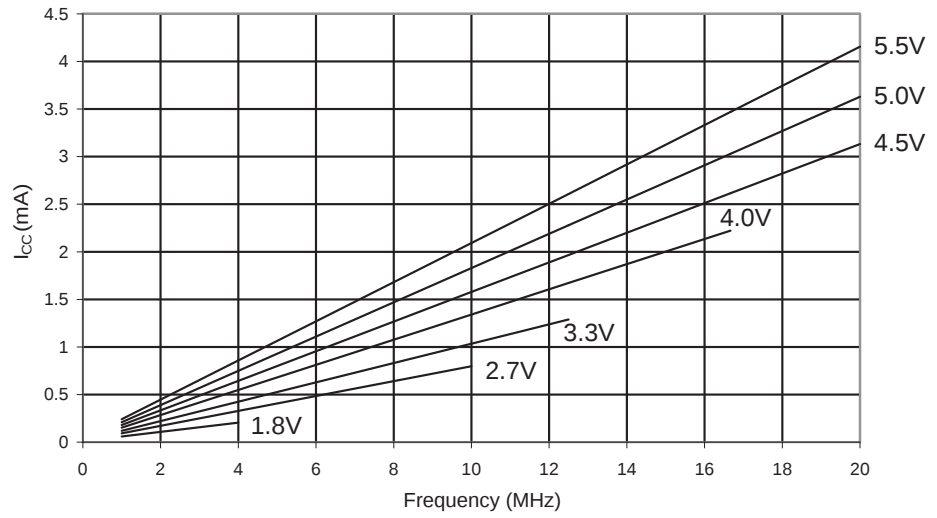
Figure 26-46. Reset Supply Current vs. Frequency (1 MHz - 20 MHz).
