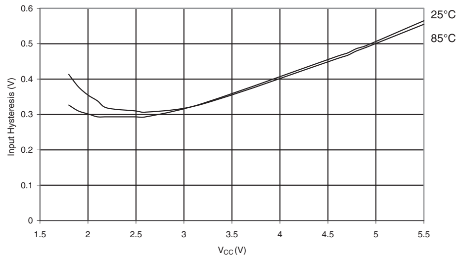
Figure 26-121. I/O Pin Input Hysteresis vs. V_{CC}
