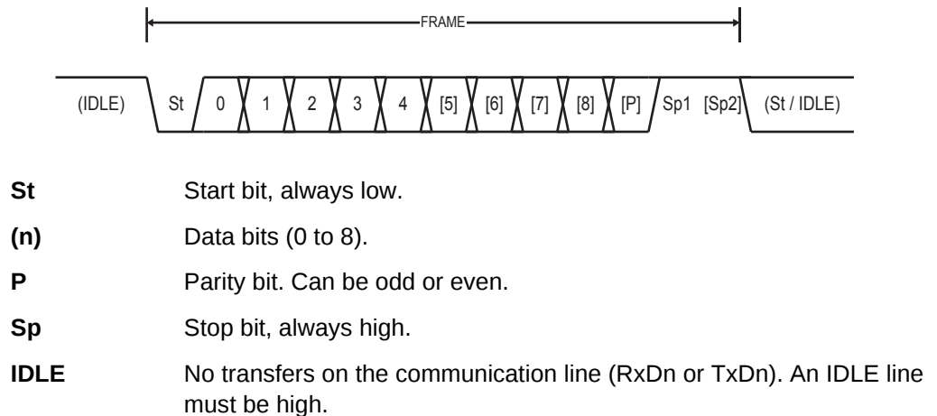
Figure 16-4. Frame Formats
