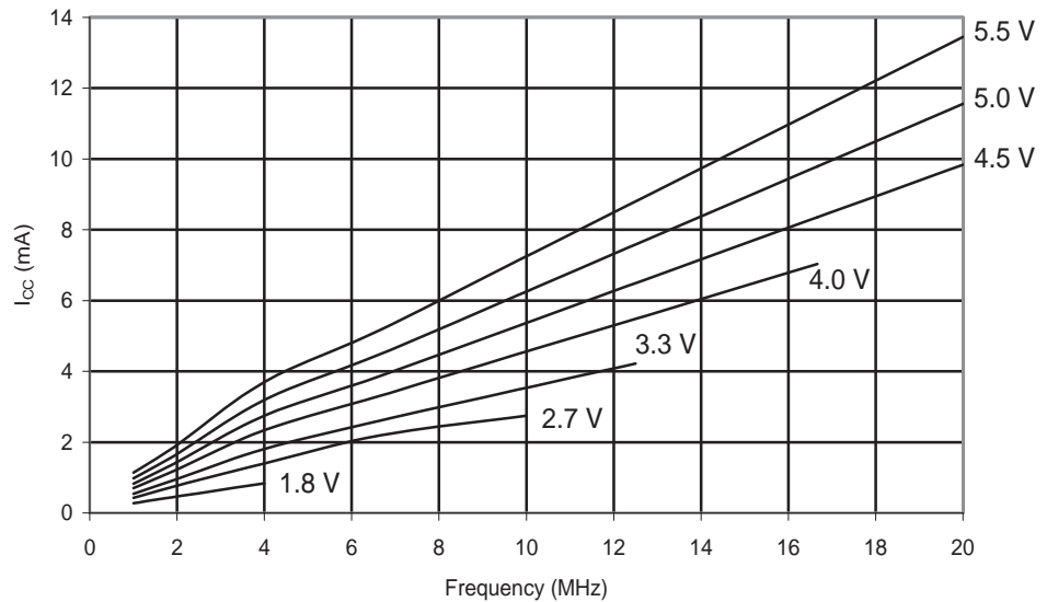
Figure 28-49. ATmega324PA: Active Supply Current vs. Frequency (1 - 20 MHz).
