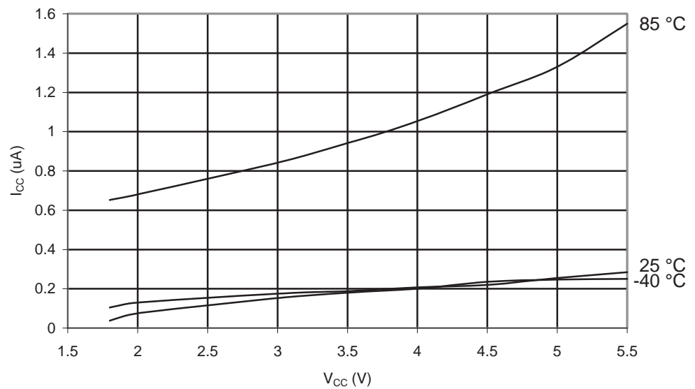
Figure 28-11. ATmega164PA: Power-down Supply Current vs. V_{CC} (Watchdog Timer Disabled).
