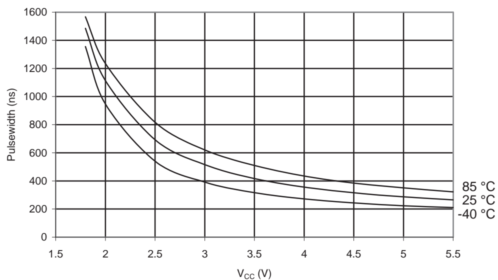
Figure 28-47. ATmega164PA: Minimum Reset Pulsewidth vs. V_{CC}
