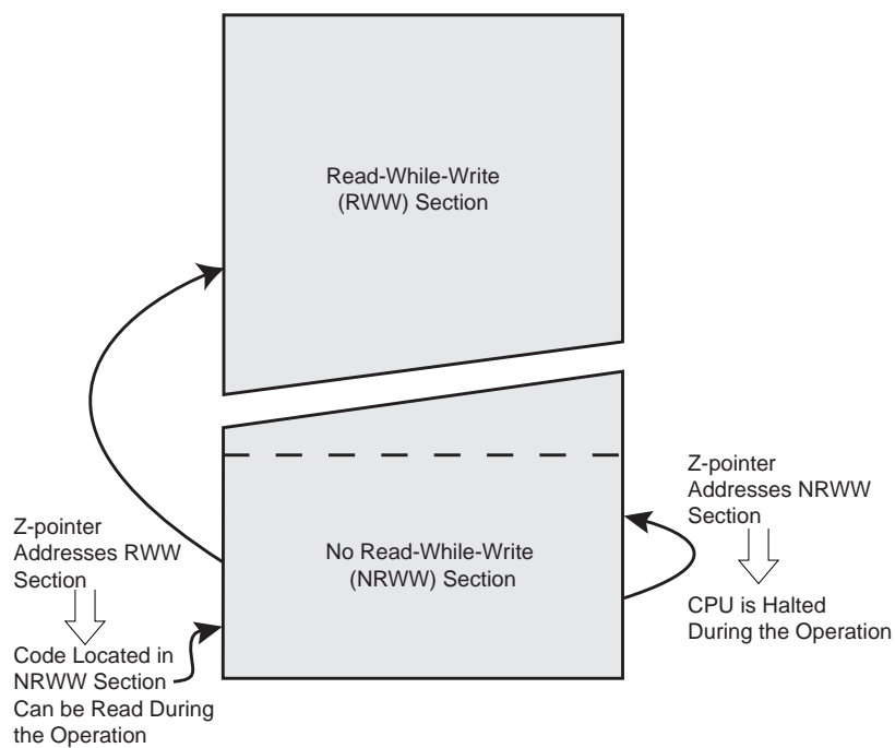
Figure 25-1. Read-While-Write vs. No Read-While-Write
