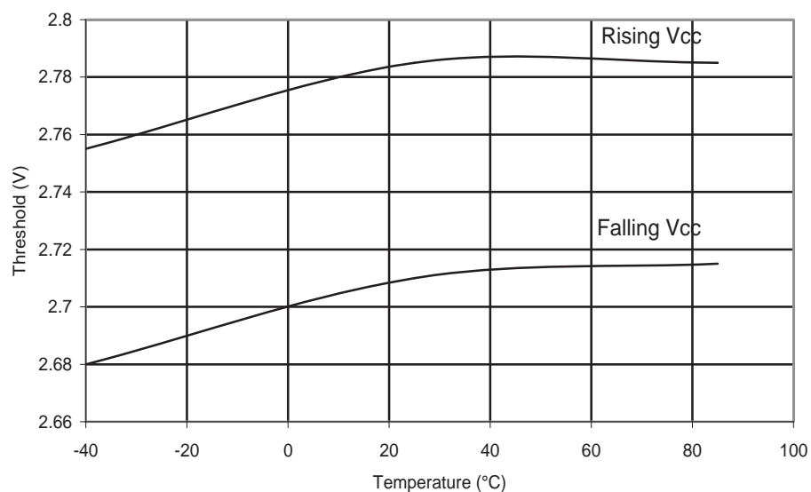
Figure 28-79. ATmega324PA: BOD Threshold vs. Temperature ( V_{BOT} = 2.7V )
