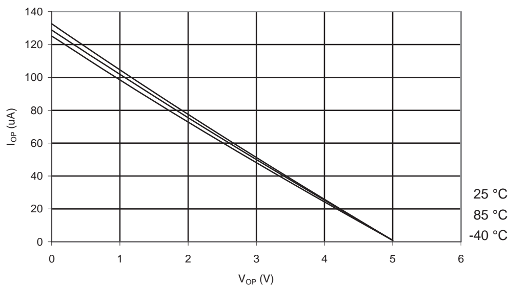
Figure 28-17. ATmega164PA: I/O Pin Pull-up Resistor Current vs. Input Voltage ( V_{CC} = 5V ).
