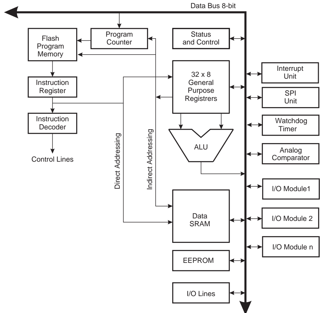
Figure 6-1. Block Diagram of the AVR Architecture
