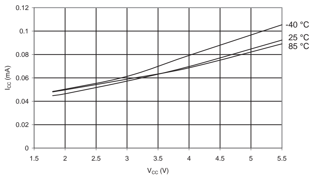
Figure 28-10. ATmega164PA: Idle Supply Current vs. V_{CC} (Internal RC Oscillator, 128 kHz).
