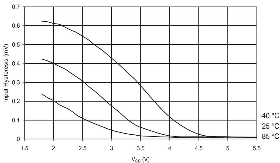
Figure 28-77. ATmega324PA: Reset Pin Input Hysteresis vs. V_{CC}
