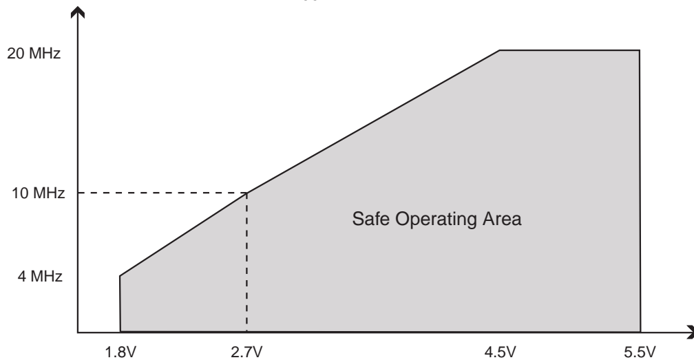
Figure 27-1. Maximum Frequency vs. V_{CC} , ATmega164PA/324PA/644PA
