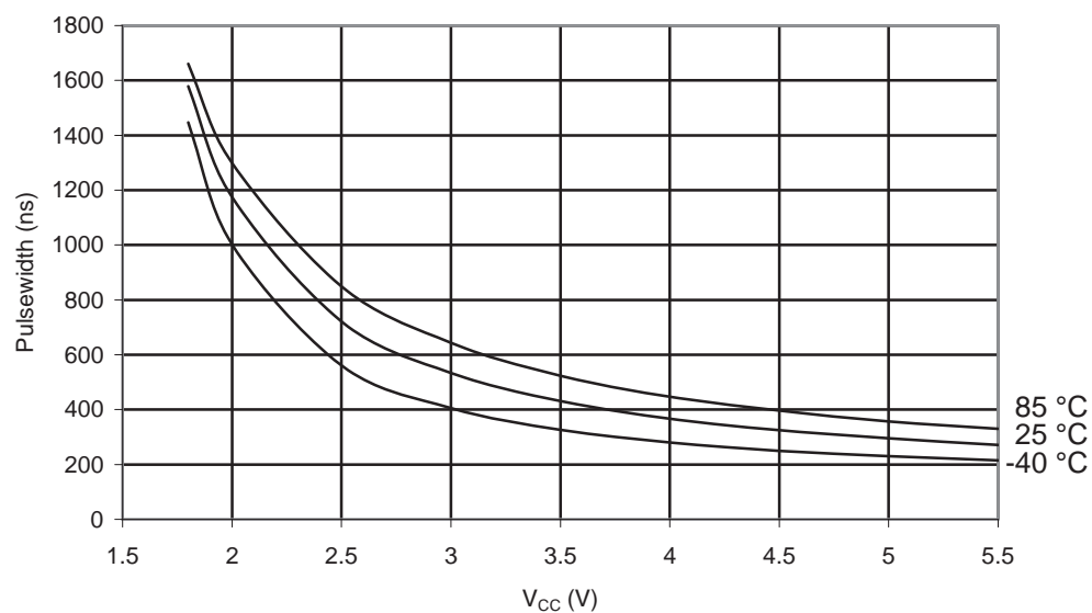
Figure 28-141. ATmega644PA: Minimum Reset Pulsewidth vs. V_{CC}
