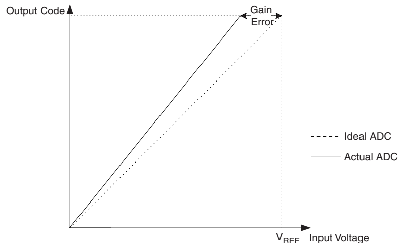
Figure 22-11. Gain Error
