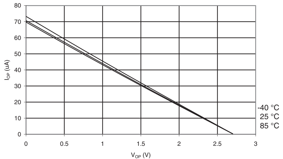
Figure 28-157. ATmega1284P: I/O Pin Pull-up Resistor Current vs. Input Voltage ( V_{CC} = 2.7V )
