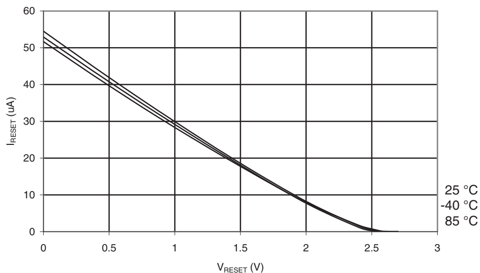
Figure 28-160. ATmega1284P: Reset Pull-up Resistor Current vs. Reset Pin Voltage ( V_{CC} = 2.7V )
