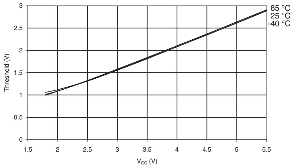
Figure 28-167. ATmega1284P: I/O Pin Input Threshold vs. V_{CC} ( V_{IH} , I/O Pin Read as '1')
