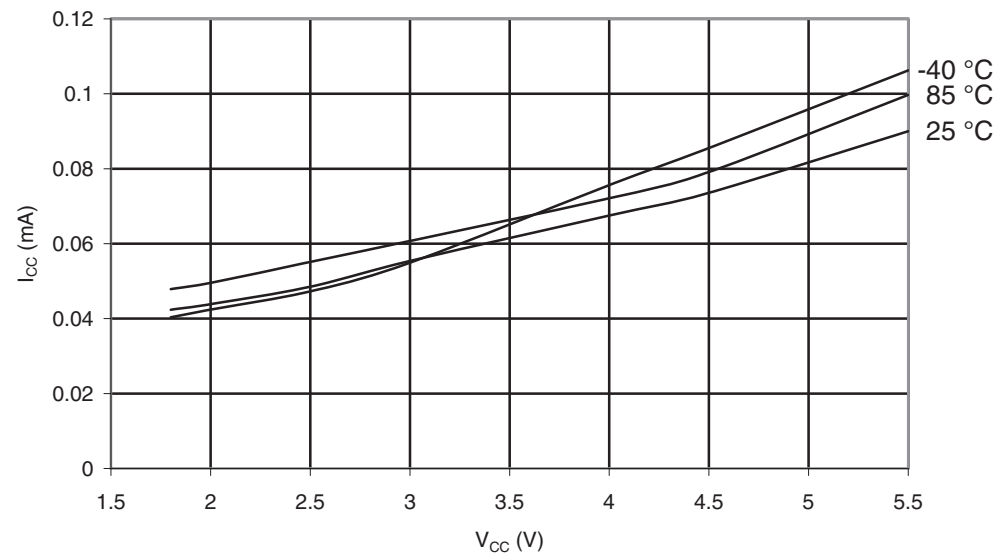
Figure 28-151. ATmega1284P: Idle Supply Current vs. V_{CC} (Internal RC Oscillator, 128 kHz)
