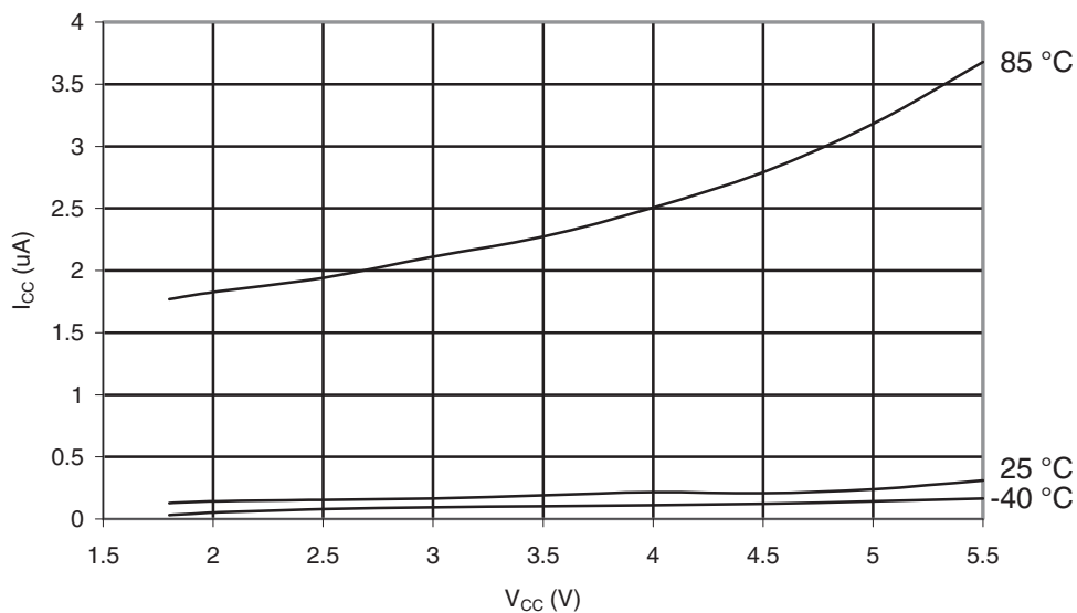
Figure 28-153. ATmega1284P: Power-down Supply Current vs. V_{CC} (Watchdog Timer Enabled)
