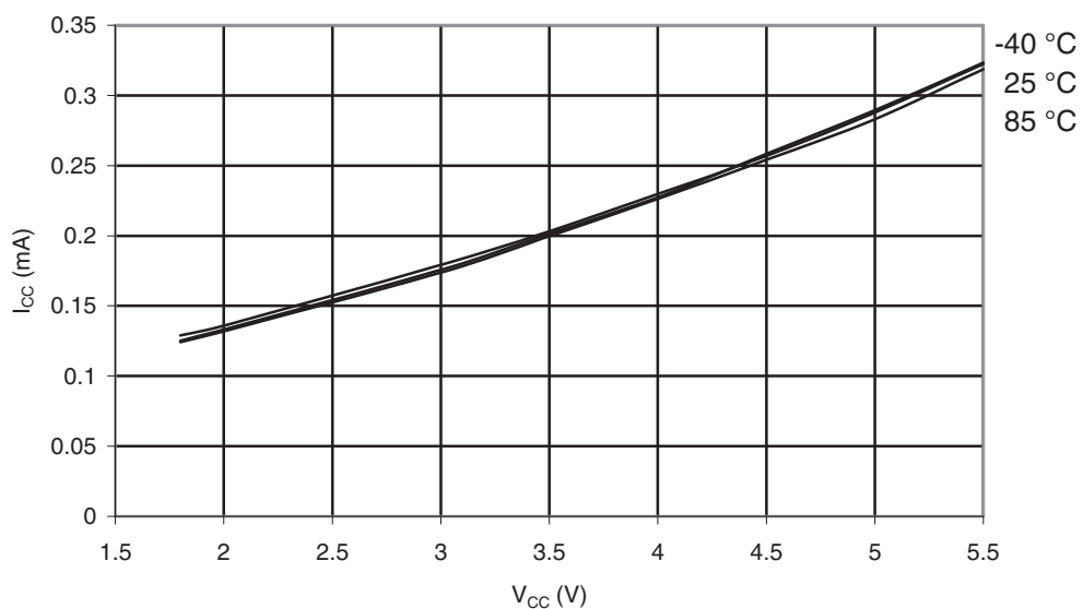
Figure 28-9. ATmega164PA: Idle Supply Current vs. V_{CC} (Internal RC Oscillator, 1 MHz).
