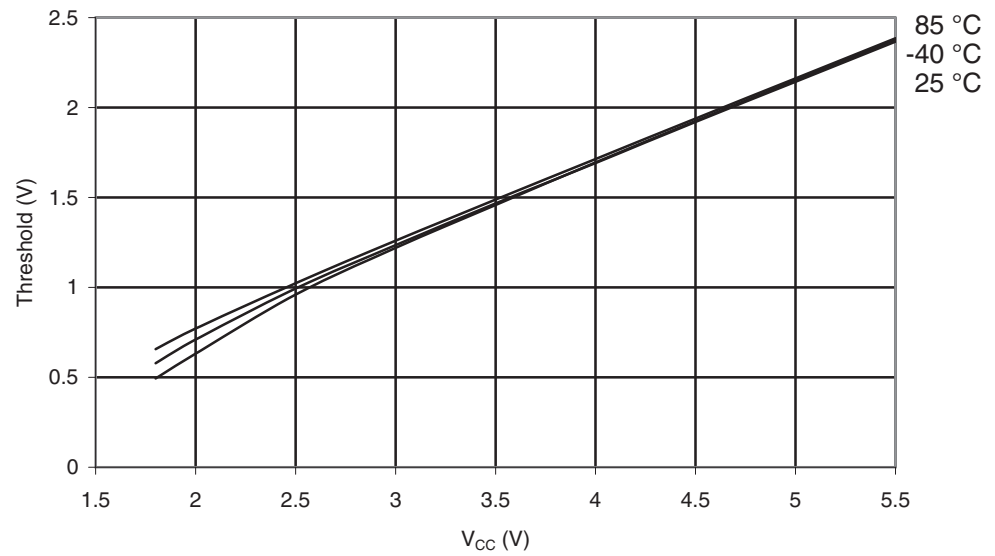
Figure 28-168. ATmega1284P: I/O Pin Input Threshold vs. V_{CC} ( V_{IL} , I/O Pin Read as '0')
