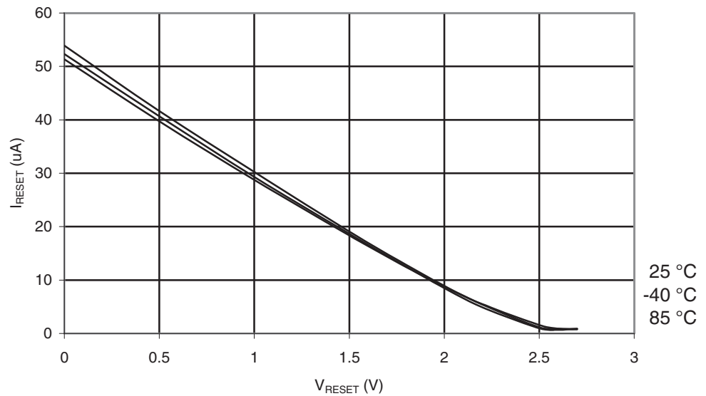
Figure 28-19. ATmega164PA: Reset Pull-up Resistor Current vs. Reset Pin Voltage ( V_{CC} = 2.7V ).
