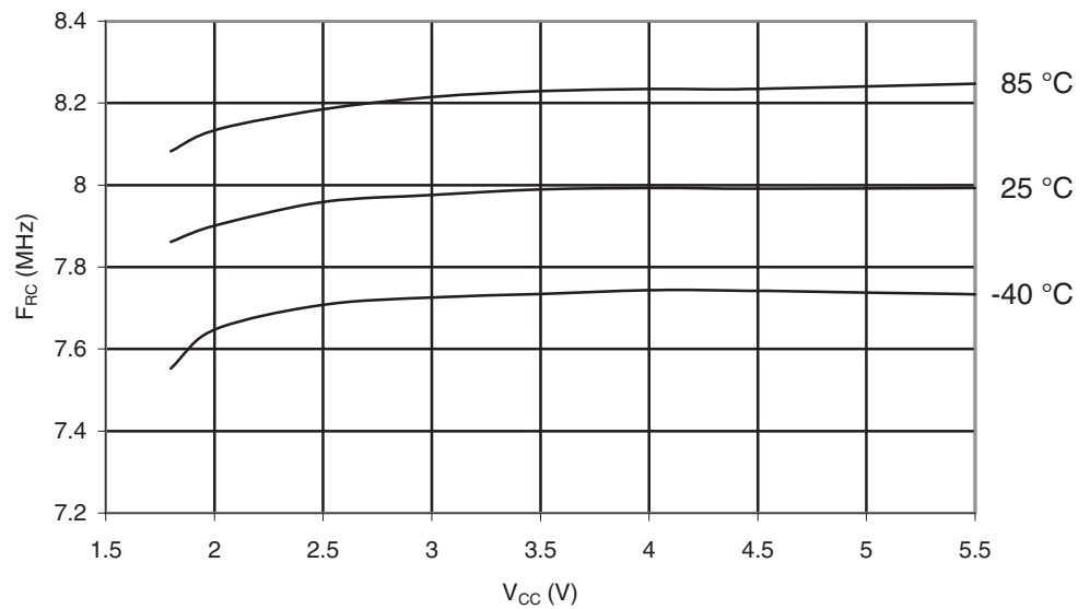
Figure 28-36. ATmega164PA: Calibrated 8 MHz RC Oscillator vs. V_{CC}
