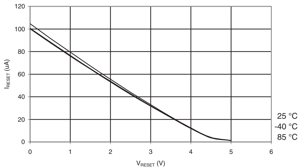
Figure 28-20. ATmega164PA: Reset Pull-up Resistor Current vs. Reset Pin Voltage ( V_{CC} = 5V ).
