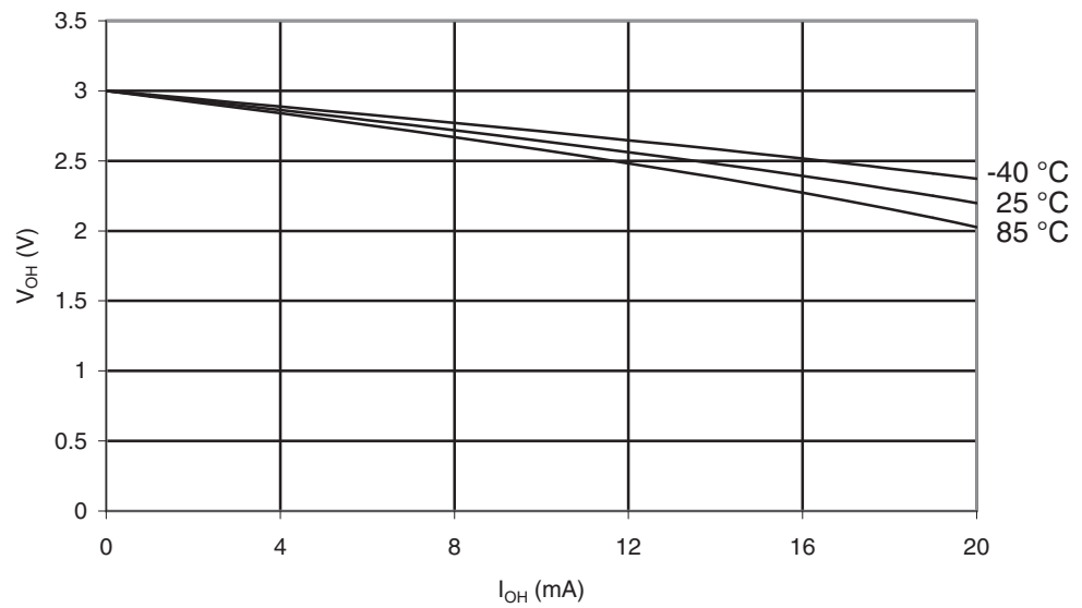
Figure 28-23. ATmega164PA: I/O Pin Output Voltage vs. Source Current ( V_{CC} = 3V ).
