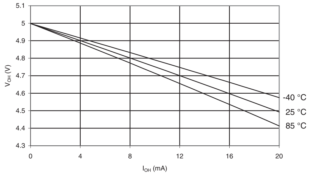
Figure 28-24. ATmega164PA: I/O Pin Output Voltage vs. Source Current ( V_{CC} = 5V ).
