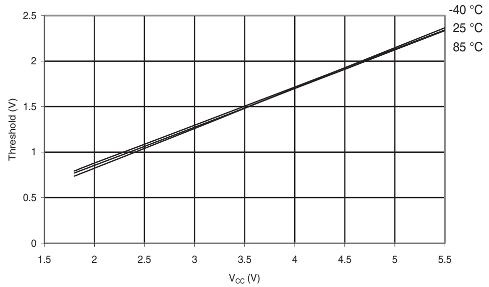
Figure 28-76. ATmega324PA: Reset Pin Input Threshold vs. V_{CC} ( V_{IL} , I/O Pin Read as '0').
