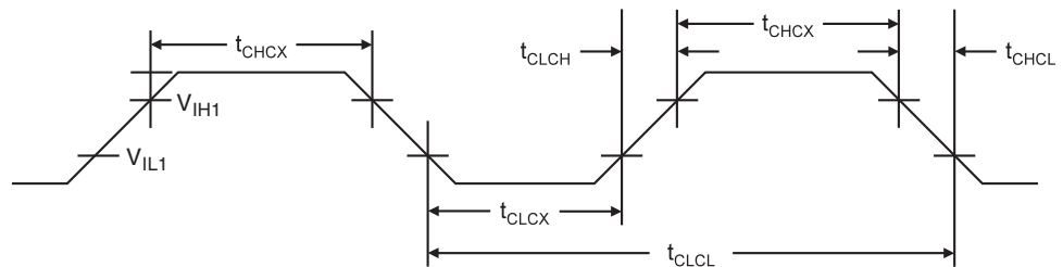
Figure 27-2. External Clock Drive Waveforms
