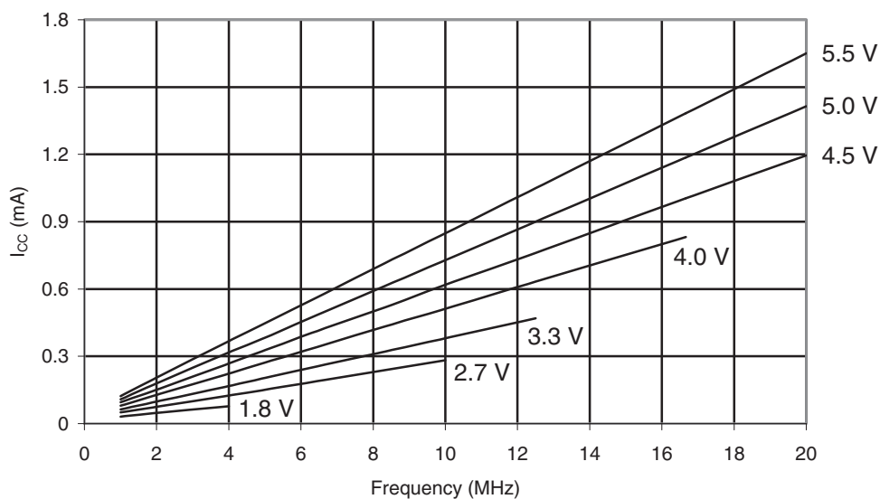
Figure 28-46. ATmega164PA: Reset Supply Current vs. Frequency (1 - 20 MHz).
