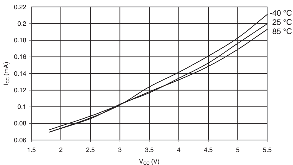
Figure 28-99. ATmega644PA: Active Supply Current vs. V_{CC} (Internal RC Oscillator, 128 kHz).
