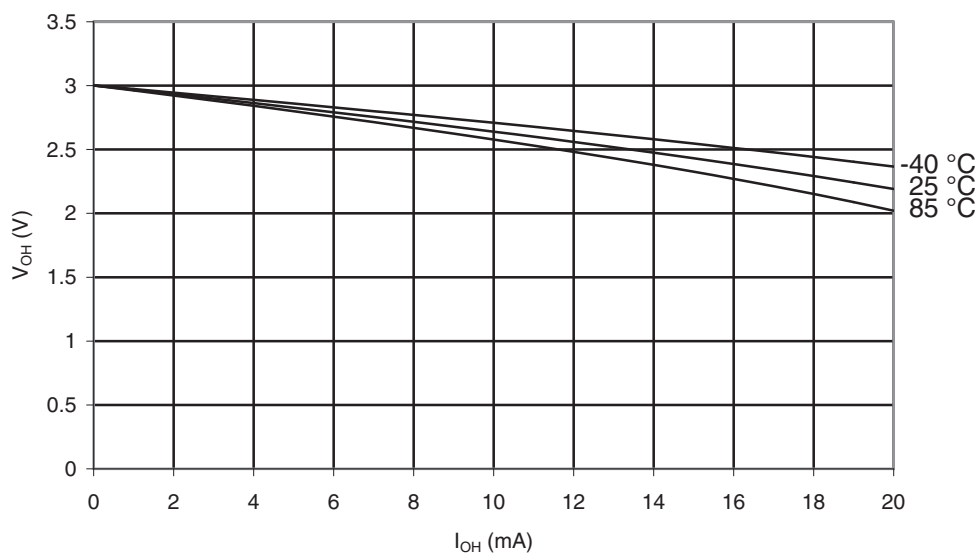
Figure 28-166. ATmega1284P: I/O Pin Output Voltage vs. Source Current ( V_{CC} = 3V )
