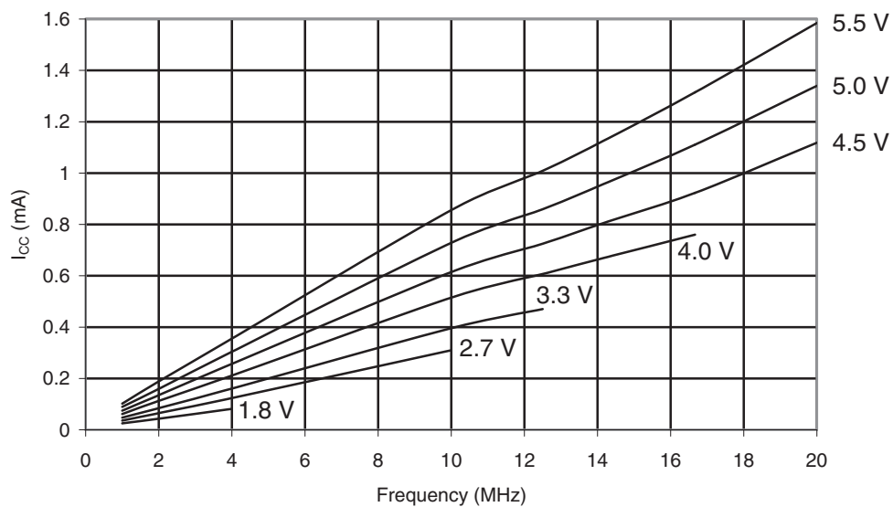
Figure 28-188. ATmega1284P: Reset Supply Current vs. Frequency (1 - 20 MHz)
