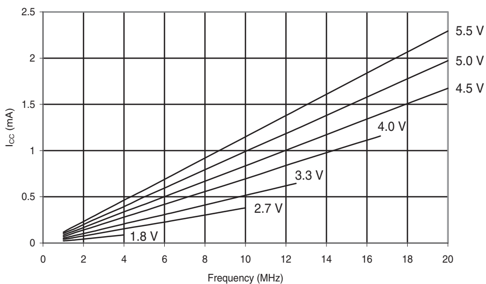
Figure 28-93. ATmega324PA: Reset Supply Current vs. Frequency (1 - 20 MHz)
