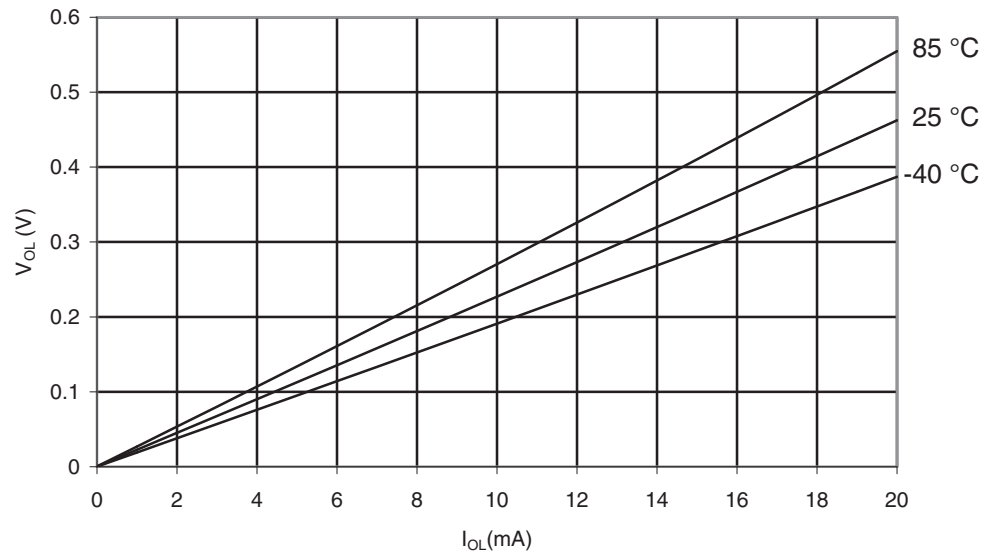
Figure 28-164. ATmega1284P: I/O Pin Output Voltage vs. Sink Current ( V_{CC} = 5V )
