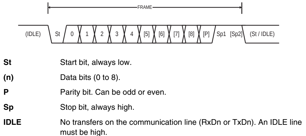
Figure 18-4. Frame Formats
