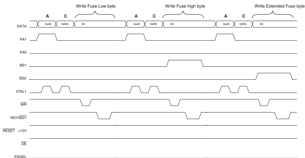
Figure 26-5. Programming the FUSES Waveforms
