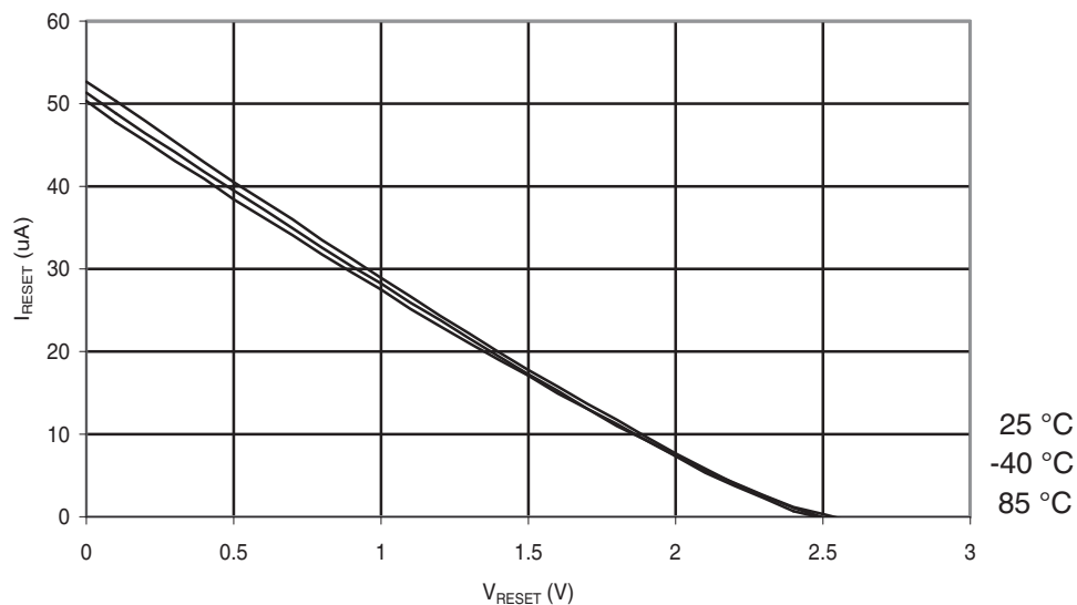
Figure 28-114. ATmega644PA: Reset Pull-up Resistor Current vs. Reset Pin Voltage ( V_{CC} = 5V ).
