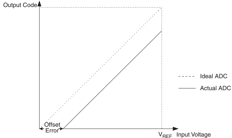
Figure 22-10. Offset Error
