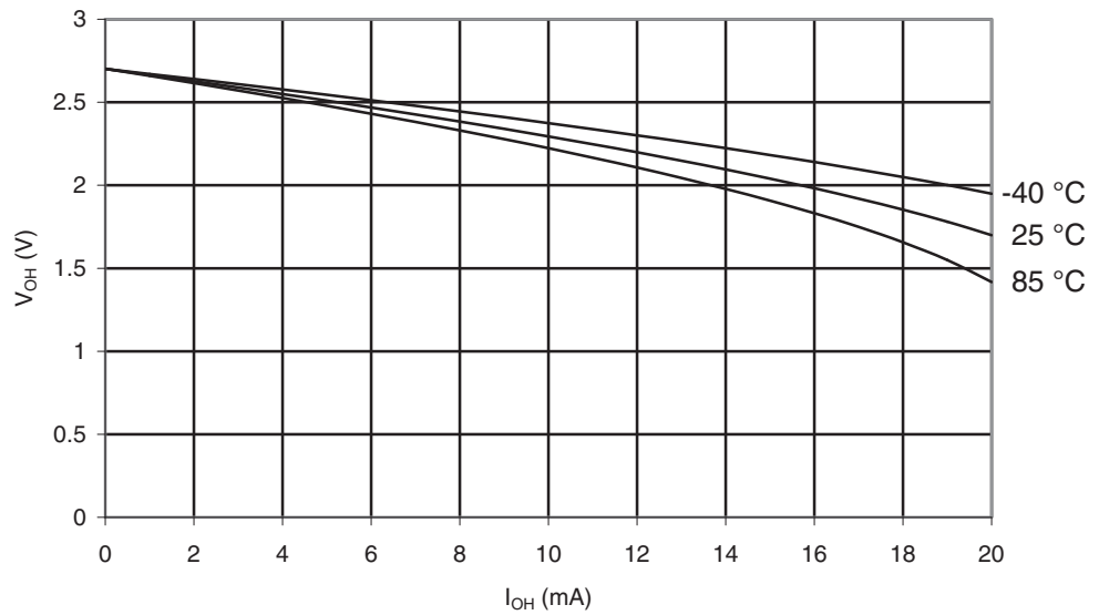
Figure 28-165. ATmega1284P: I/O Pin Output Voltage vs. Source Current ( V_{CC} = 2.7V )
