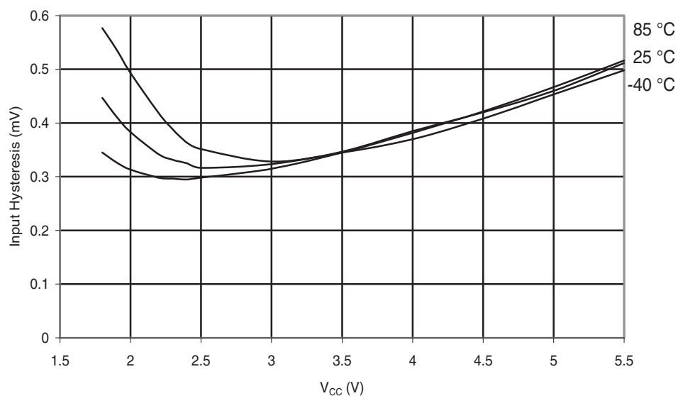
Figure 28-74. ATmega324PA: I/O Pin Input Hysteresis vs. V_{CC}
