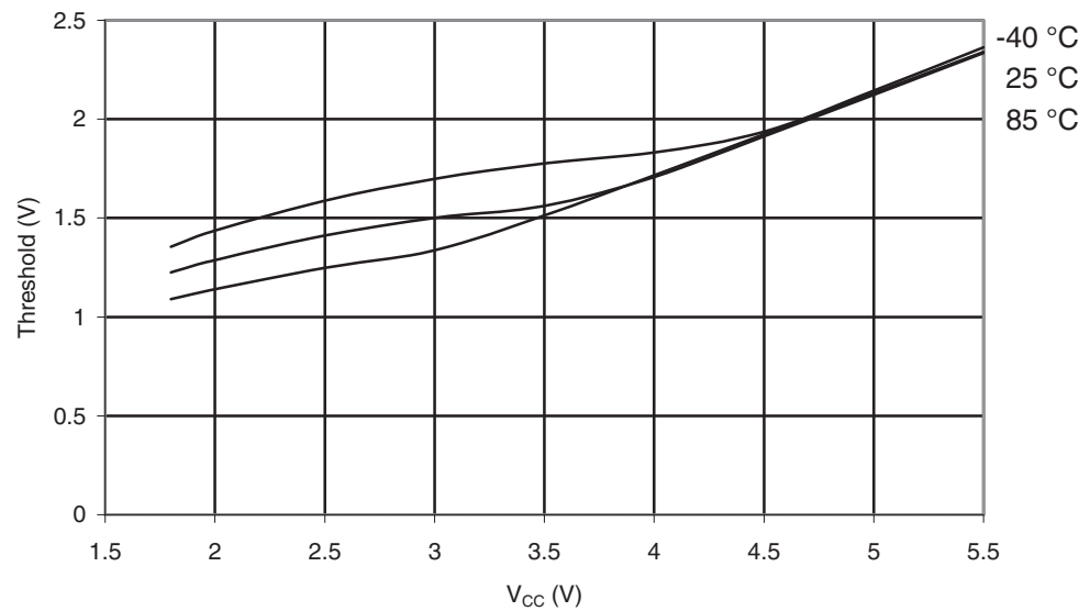
Figure 28-28. ATmega164PA: Reset Pin Input Threshold vs. V_{CC} ( V_{IH} , I/O Pin Read as '1').
