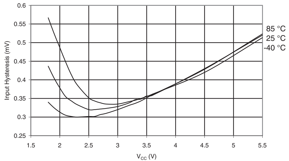
Figure 28-169. ATmega1284P: I/O Pin Input Hysteresis vs. V_{CC}
