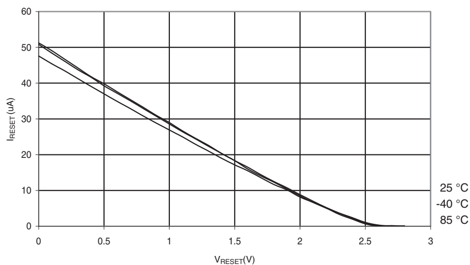
Figure 28-53. Reset Pull-up Resistor Current vs. Reset Pin Voltage ( V_{CC} = 2.7V )
