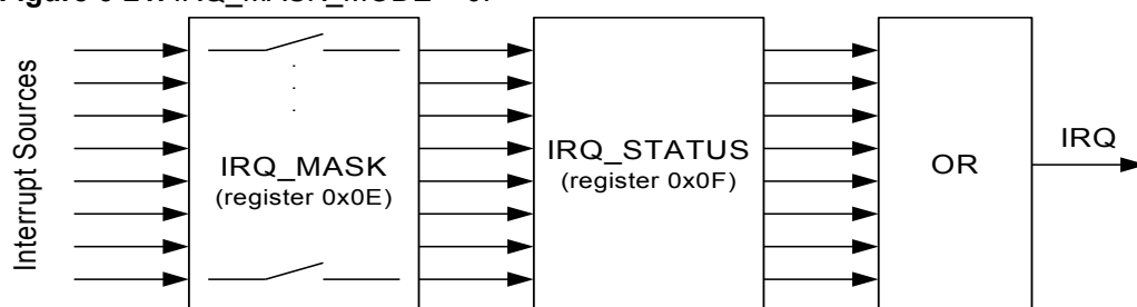
Figure 6-21. IRQ_MASK_MODE = 0 .
