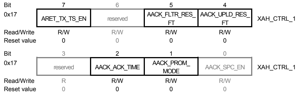
Figure 7-20. Register XAH_CTRL_1.
