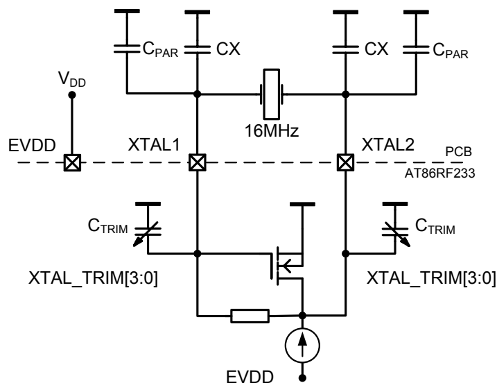
Figure 9-11. Simplified XOSC Schematic with External Components.
