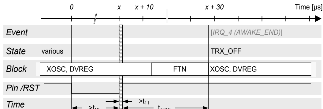
Figure 7-8. Reset Procedure.
