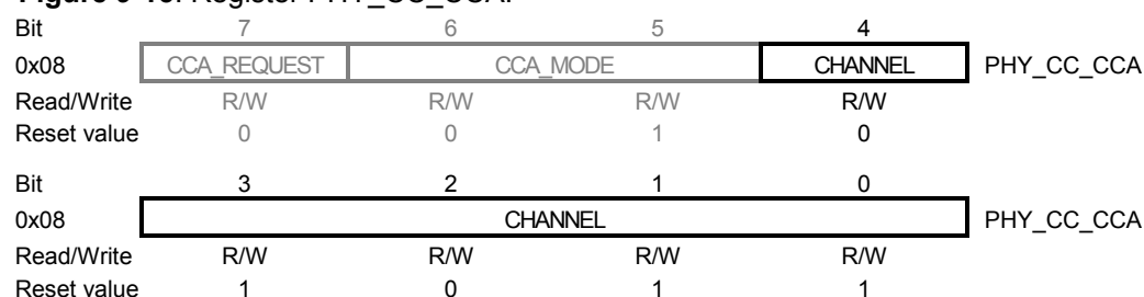
Figure 9-15. Register PHY_CC_CCA.
