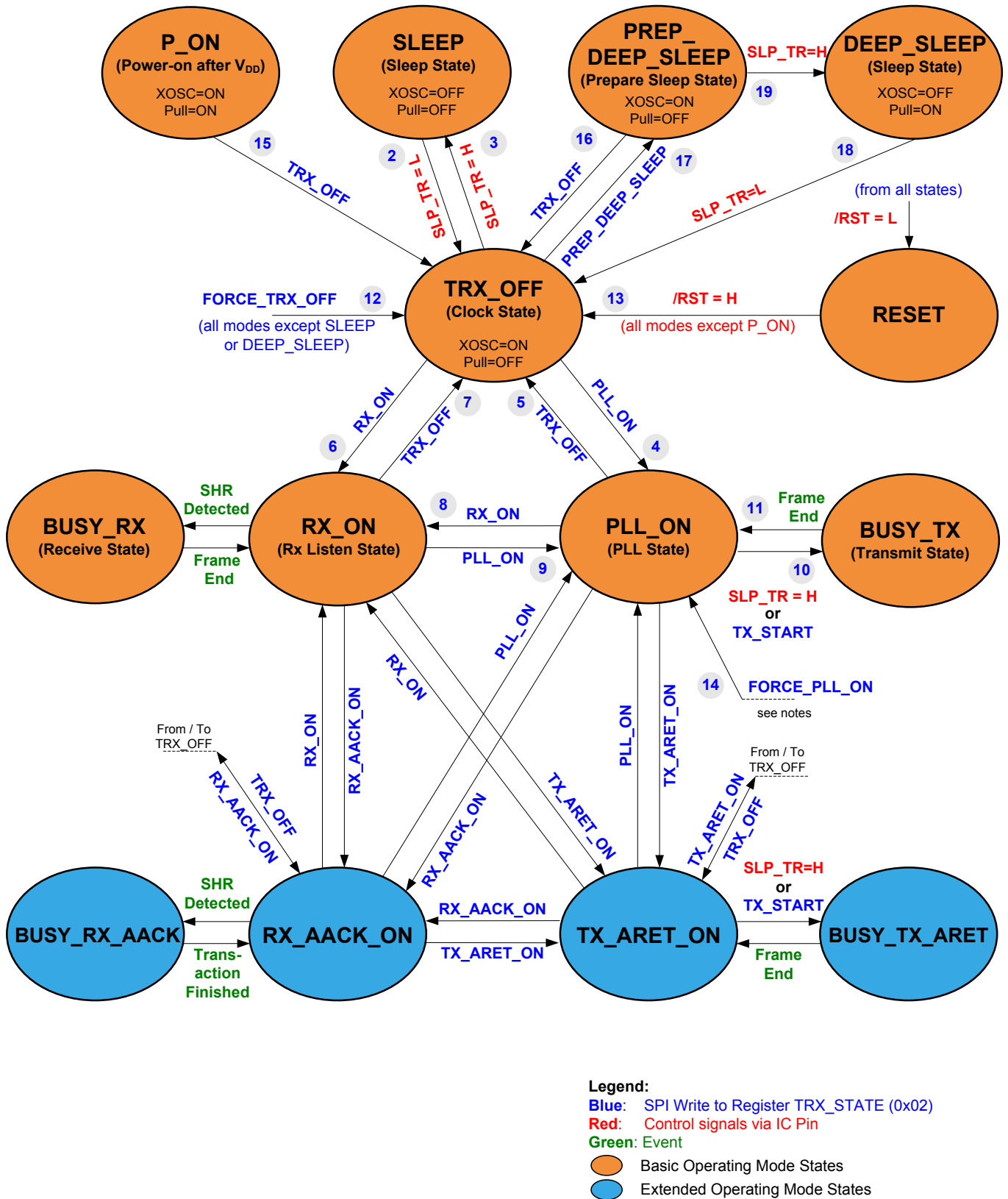
Figure 7-11. Extended Operating Mode State Diagram.
