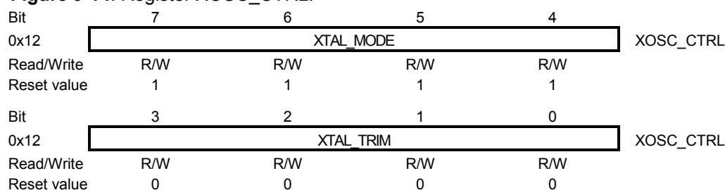
Figure 9-14. Register XOSC_CTRL.
