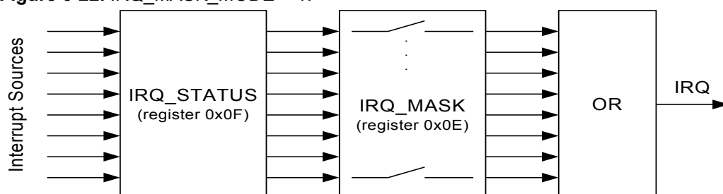
Figure 6-22. IRQ_MASK_MODE = 1 .
