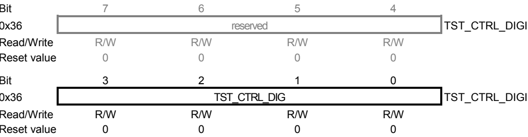
Figure 0-1. Register TST_CTRL_DIGI.
