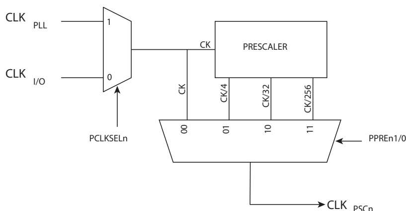
Figure 12-42. Clock selection
