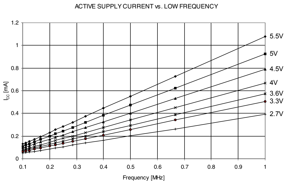
Figure 23-1. Active Supply Current vs. Frequency (0.1 - 1.0 MHz)
