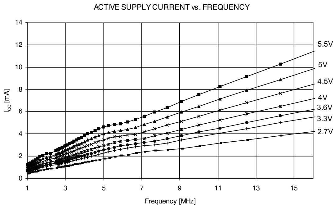
Figure 23-2. Active Supply Current vs. Frequency (1 - 16 MHz)
