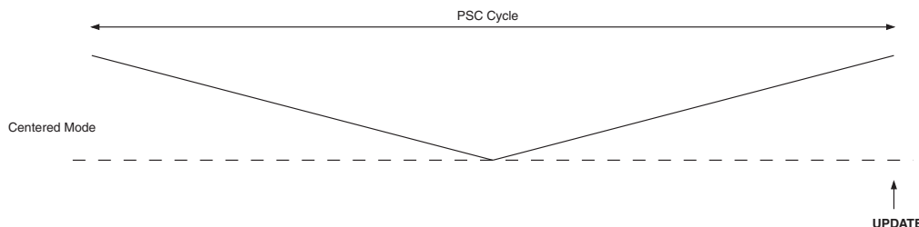
Figure 12-5. Cycle Presentation in Centered Mode
