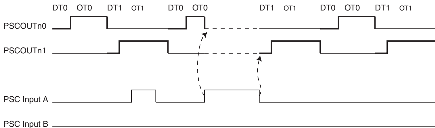
Figure 12-22. PSCn behavior versus PSCn Input A in Fault Mode 1
