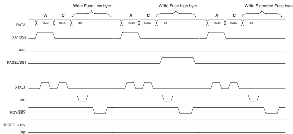
Figure 21-5. Programming the FUSES Waveforms
