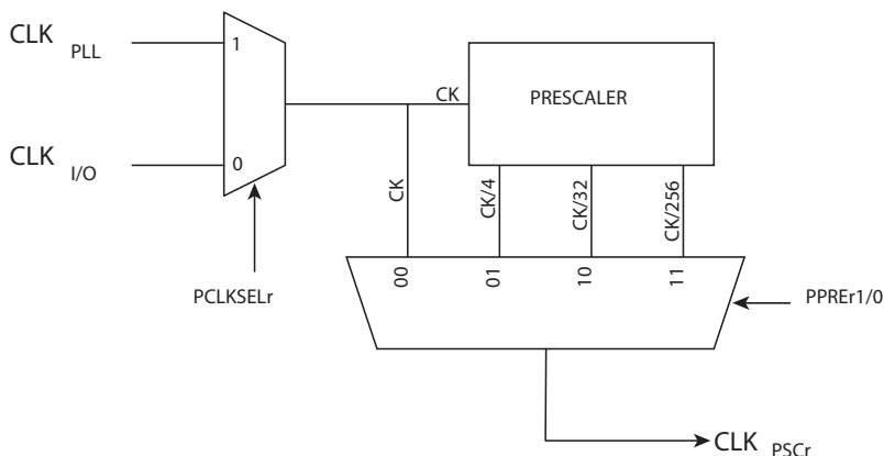
Figure 13-31. Clock selection
