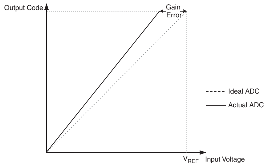
Figure 17-11. Gain Error
