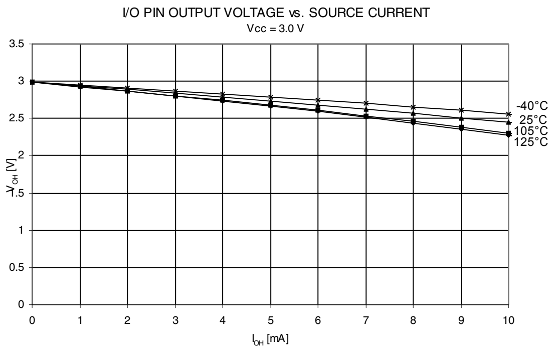
Figure 23-18. I/O Pin Output Voltage vs. Source current ( V_{CC} = 3V )
