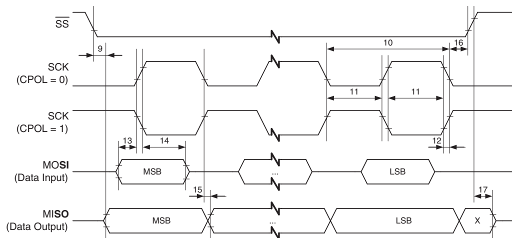
Figure 22-4. SPI Interface Timing Requirements (Slave Mode)
