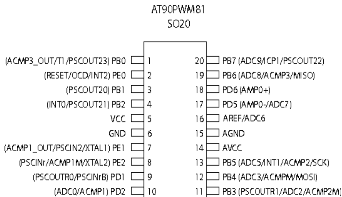
Figure 2-1. 20 Pin Packages
