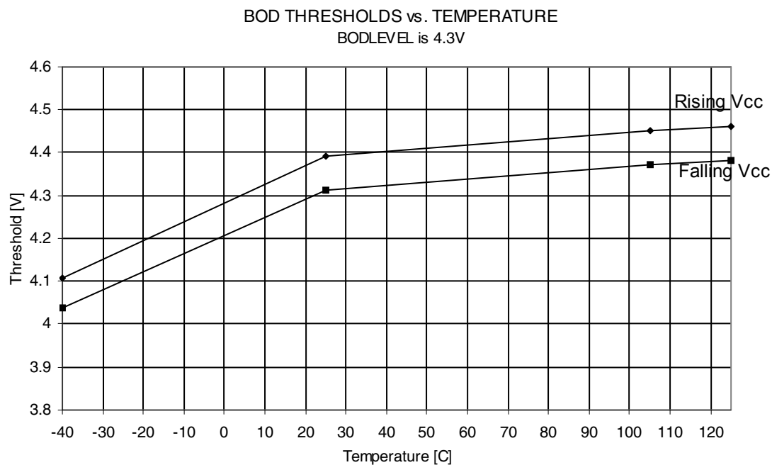
Figure 23-23. BOD Thresholds vs. Temperature (BODLEVEL is 4.3V)
