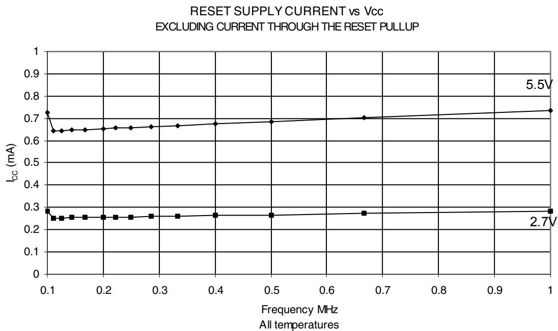
Figure 23-31. Reset Supply Current vs. V_{CC} (0.1 - 1.0 MHz, Excluding Current through the Reset Pull-up)
