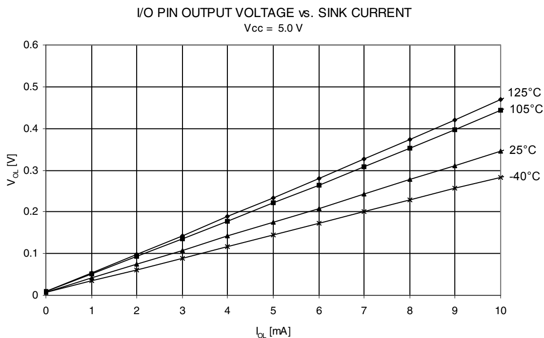
Figure 23-19. I/O Pin Output Voltage vs. Sink current ( V_{CC} = 5V )
