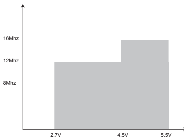
Figure 22-2. Maximum Frequency vs. V_{CC} , AT90PWM81
