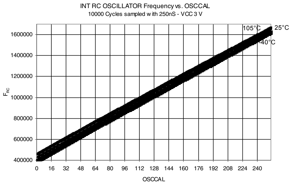
Figure 23-30. Calibrated 8 MHz RC Oscillator Frequency vs. Oscal Value
