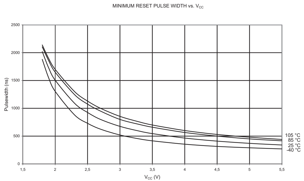
Figure 2-43. Minimum Reset Pulse Width vs. V_{CC}
