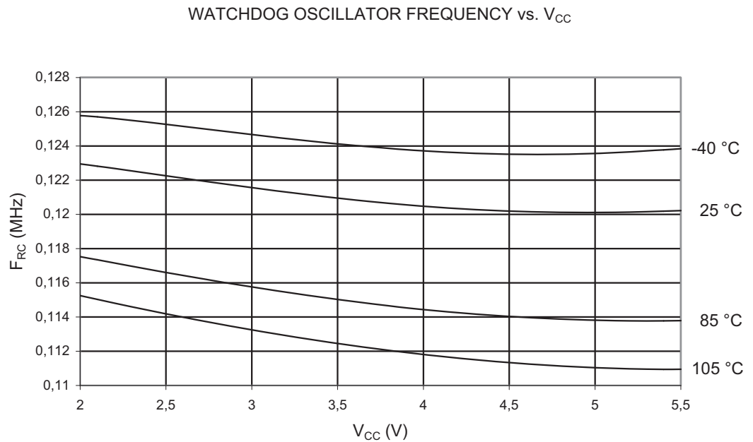
Figure 2-34. Watchdog Oscillator Frequency vs. V_{CC}
