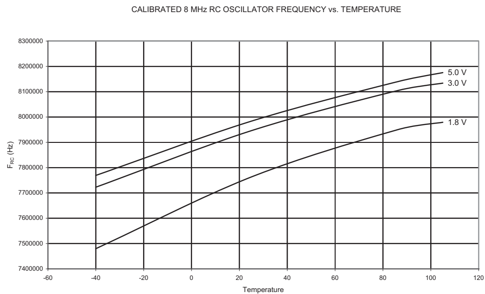
Figure 2-37. Calibrated 8 MHz RC Oscillator Frequency vs. Temperature
