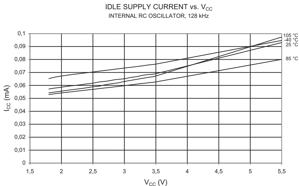
Figure 2-6. Idle Supply Current vs. V_{CC} (Internal RC Oscillator, 128 kHz)
