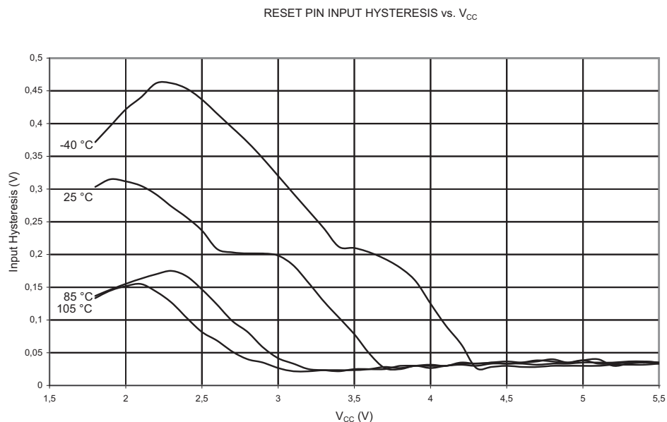
Figure 2-28. Reset Pin Input Hysteresis vs. V_{CC}
