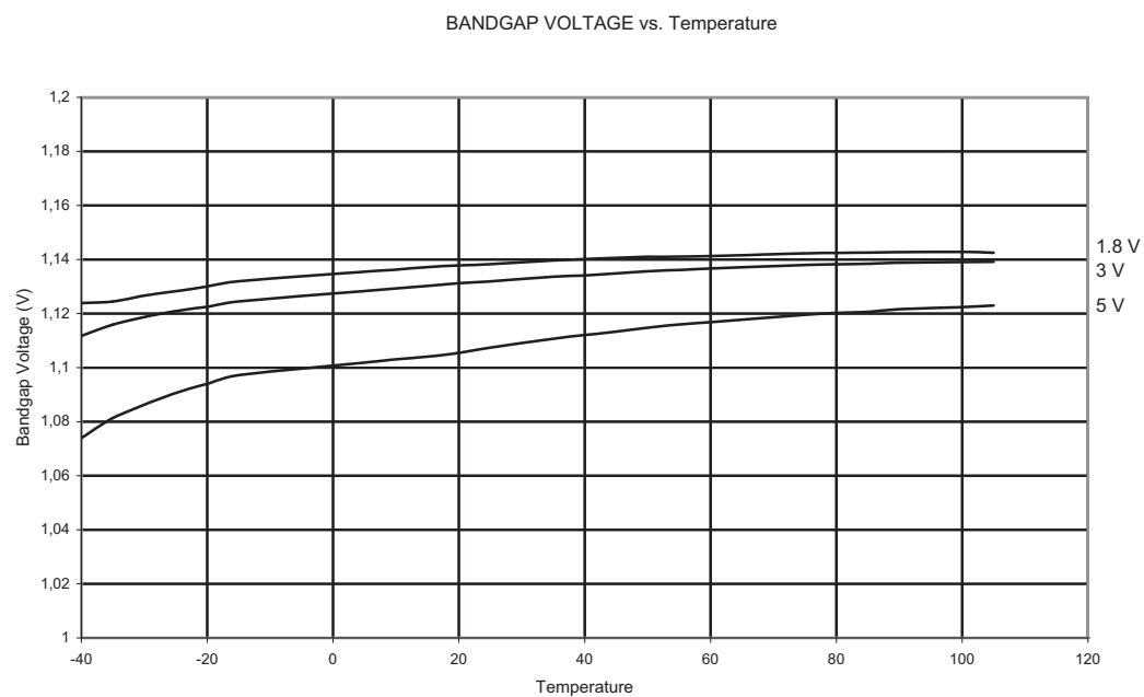
Figure 2-33. Bandgap Voltage vs. Temperature
