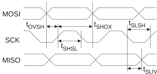
Figure 1-2. Serial Programming Timing
