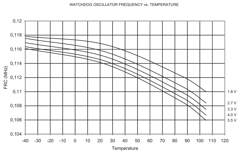
Figure 2-35. Watchdog Oscillator Frequency vs. Temperature
