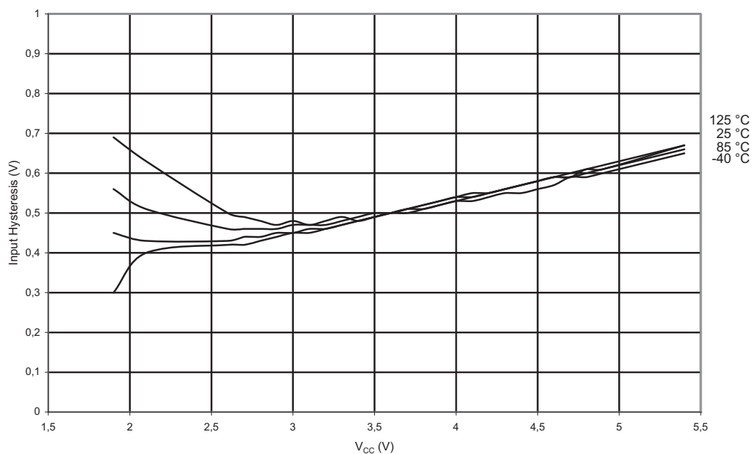
Figure 3-122. V_{IH}-V_{IL} : Input Hysteresis vs. V_{CC} (Reset Pin as I/O)
