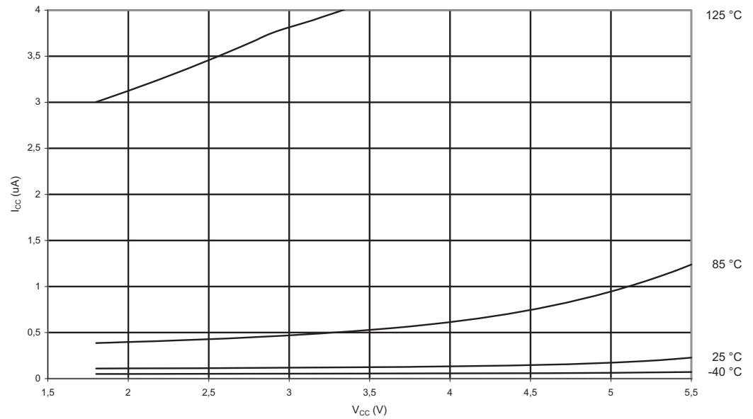
Figure 3-100. Power-down Supply Current vs. V_{CC} (Watchdog Timer Enabled)
