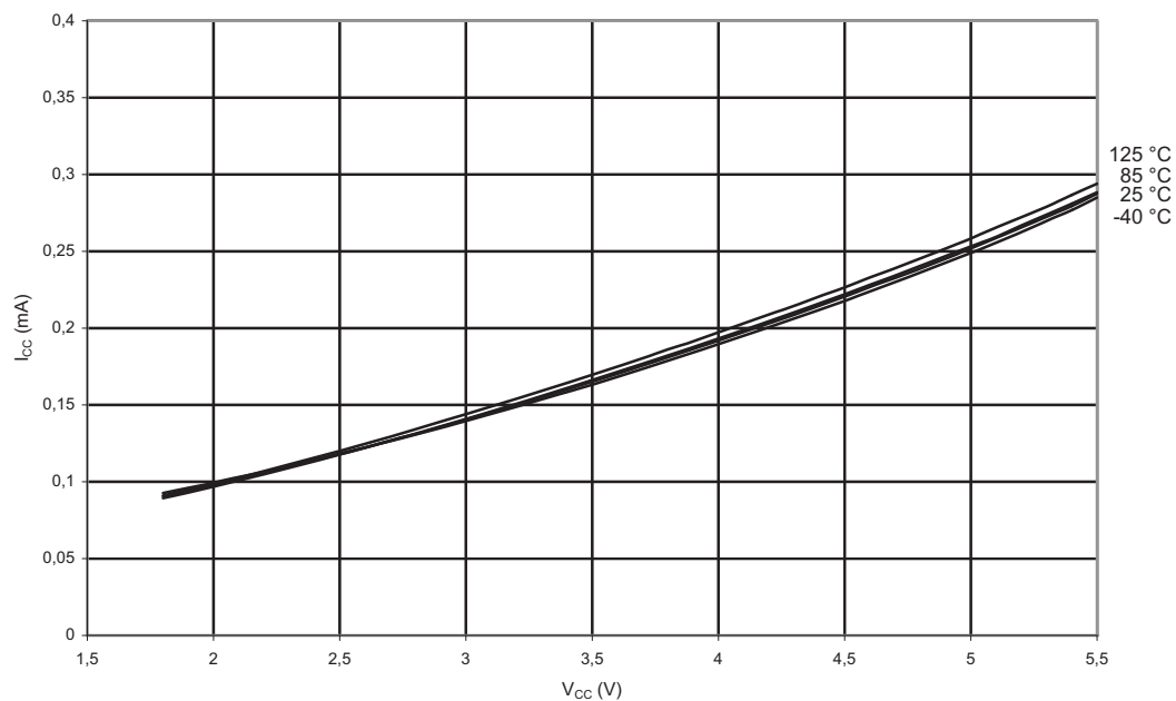
Figure 3-98. Idle Supply Current vs. V_{CC} (Internal RC Oscillator, 128 kHz)
