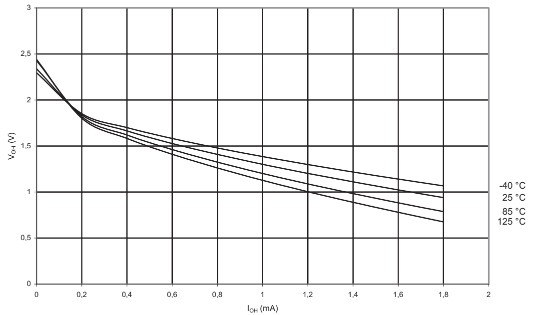
Figure 3-116. V_{OH} : Output Voltage vs. Source Current (Reset Pin as I/O, V_{CC} = 5V )
