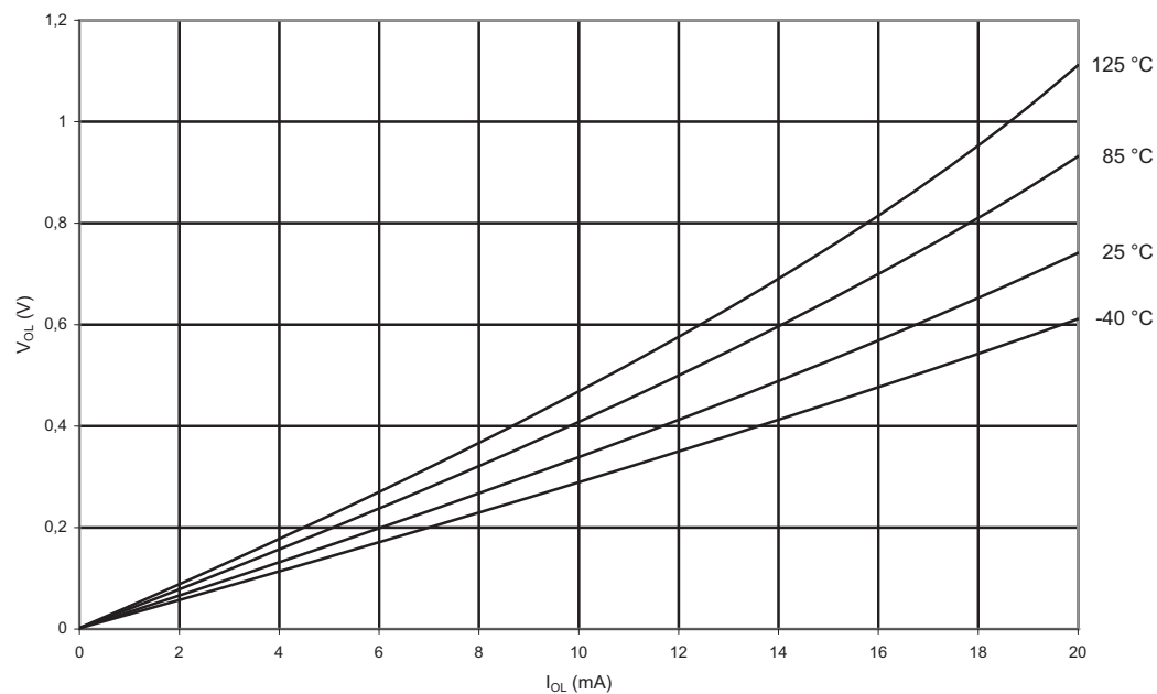
Figure 3-110. V_{OL} : Output Voltage vs. Sink Current (I/O Pin, V_{CC} = 5V )
