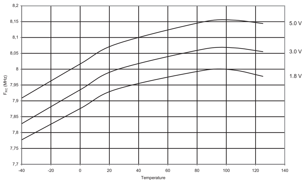
Figure 3-134. Calibrated 8 MHz RC Oscillator Frequency vs. Temperature
