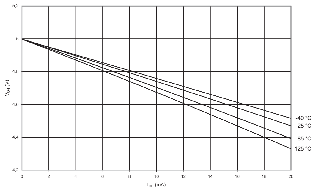
Figure 3-112. V_{OH} : Output Voltage vs. Source Current (I/O Pin, V_{CC} = 5V )
