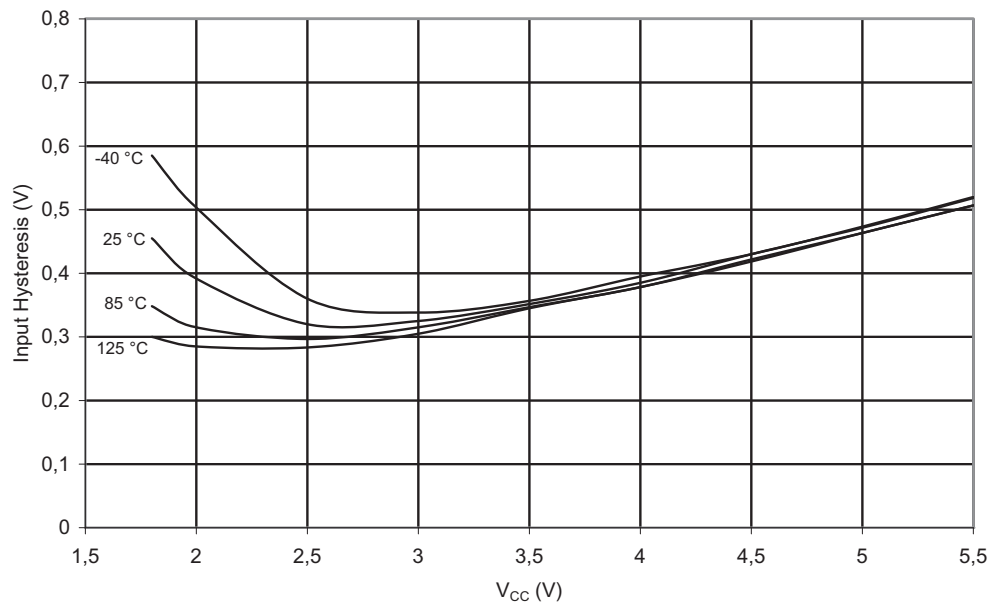
Figure 3-76. V_{IH}-V_{IL} : Input Hysteresis vs. V_{CC} (I/O Pin)
