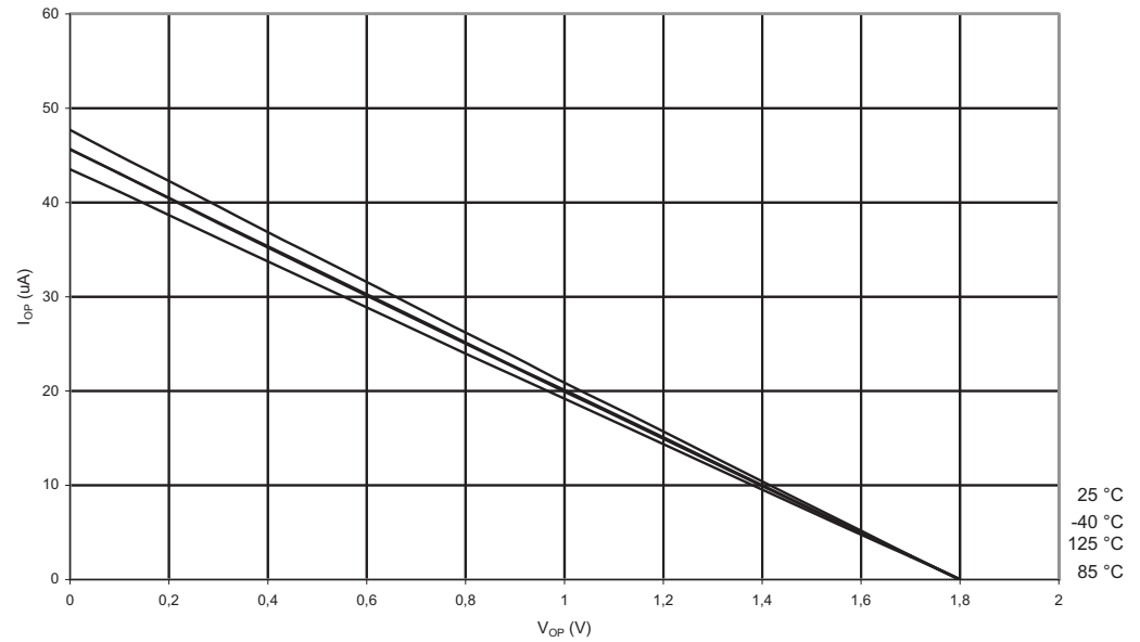
Figure 3-104. Pull-up Resistor Current vs. Input Voltage (I/O Pin, V_{CC} = 2.7V )
