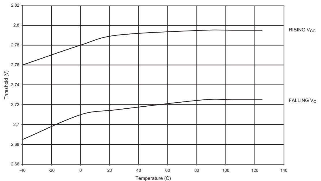
Figure 3-124. BOD Threshold vs. Temperature (BODLEVEL = 2.7V)
