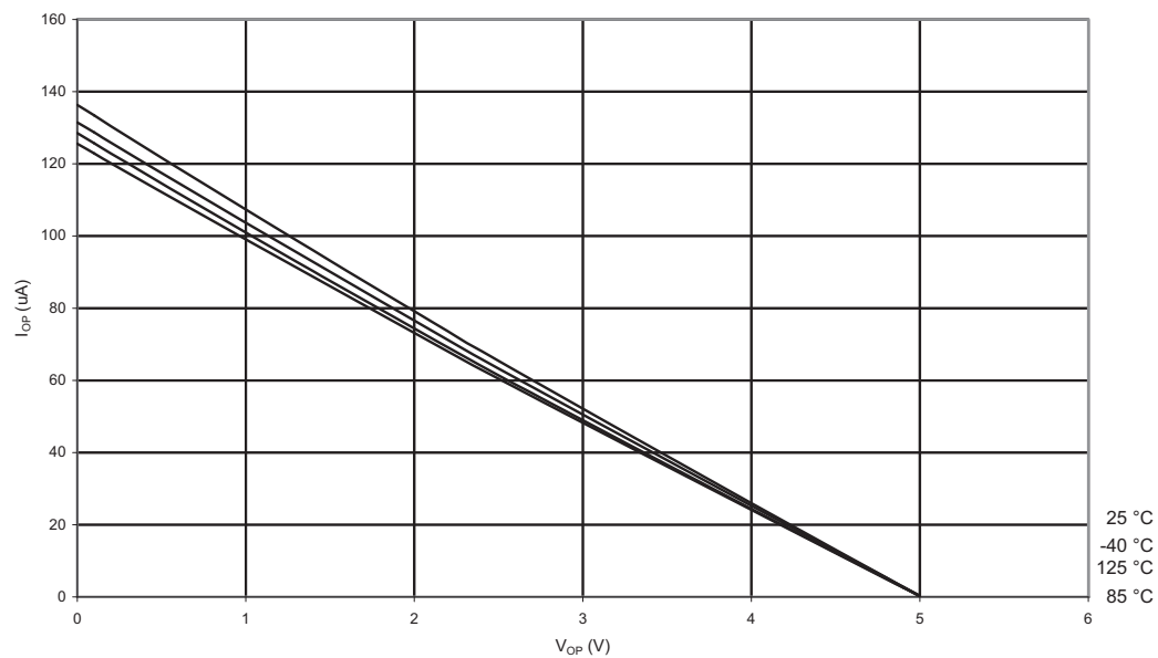
Figure 3-106. Reset Pull-up Resistor Current vs. Reset Pin Voltage ( V_{CC} = 1.8V )
