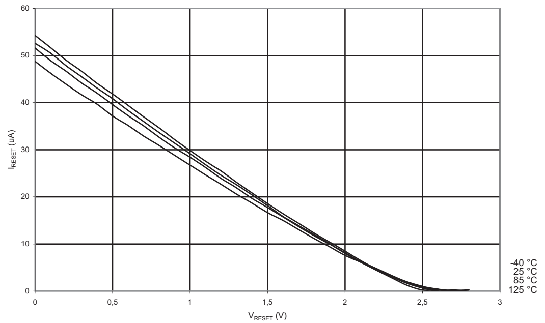
Figure 3-108. Reset Pull-up Resistor Current vs. Reset Pin Voltage ( V_{CC} = 5V )
