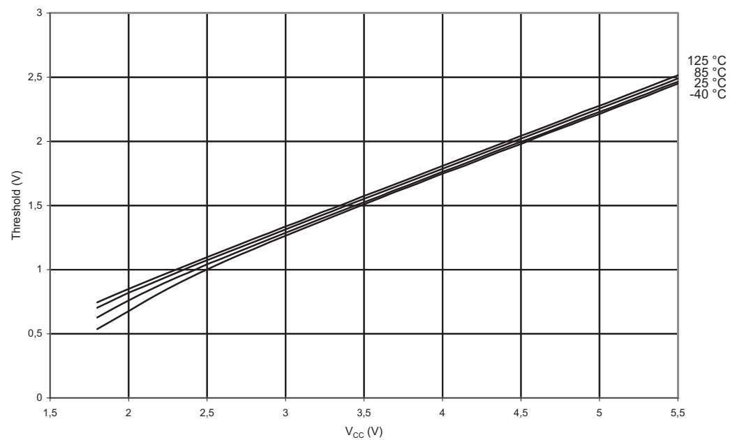
Figure 3-118. V_{IL} : Input Threshold Voltage vs. V_{CC} (I/O Pin, Read as '0')
