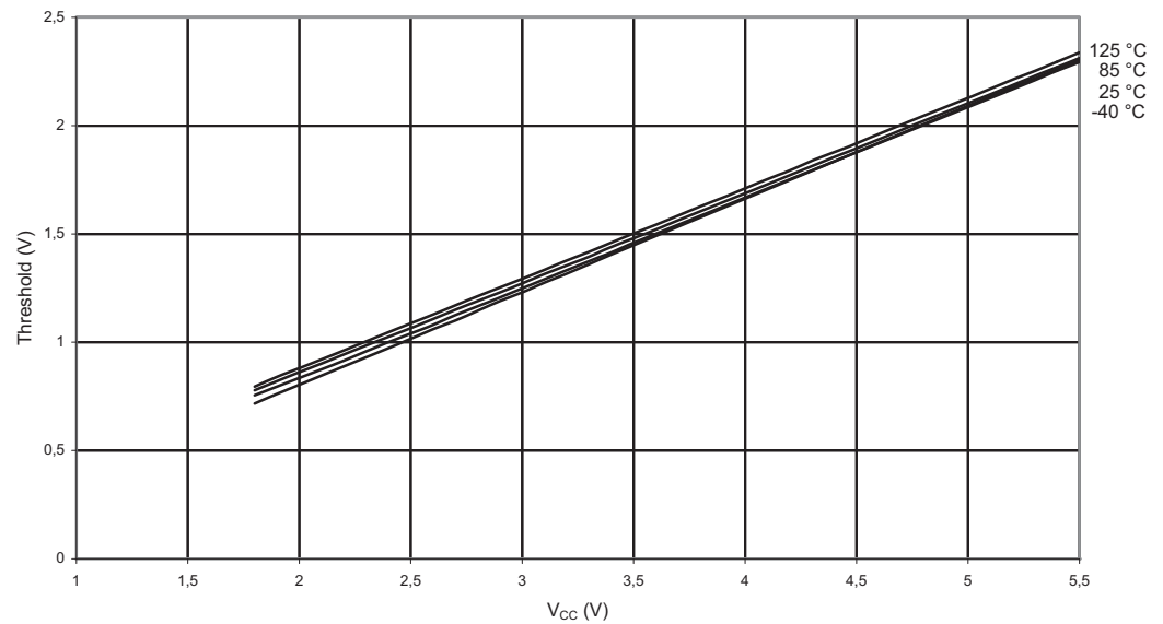
Figure 3-40. V_{IH}-V_{IL} : Input Hysteresis vs. V_{CC} (Reset Pin)
