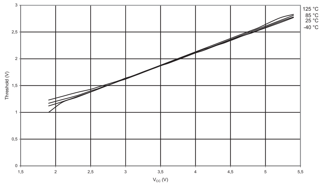
Figure 3-120. V_{IH} : Input Threshold Voltage vs. V_{CC} (Reset Pin as I/O, Read as '1')
