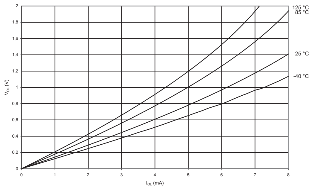
Figure 3-114. V_{OL} : Output Voltage vs. Sink Current (Reset Pin as I/O, V_{CC} = 5V )
