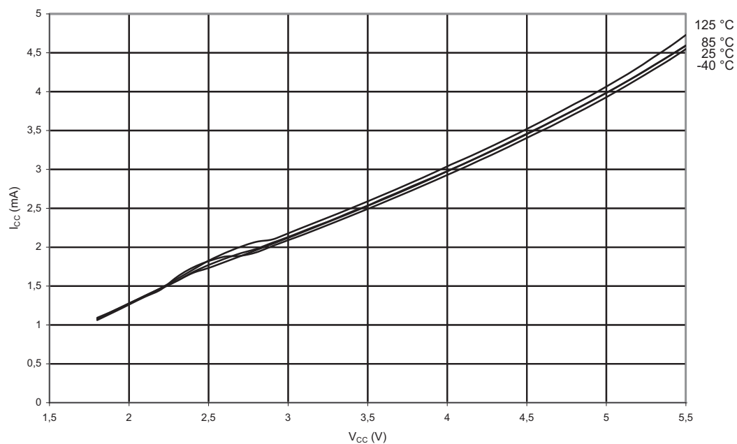
Figure 3-94. Active Supply Current vs. V_{CC} (Internal RC Oscillator, 1 MHz)
