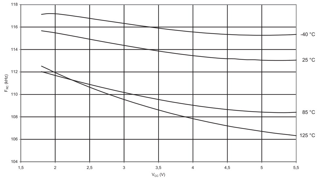
Figure 3-132. Watchdog Oscillator Frequency vs. Temperature
