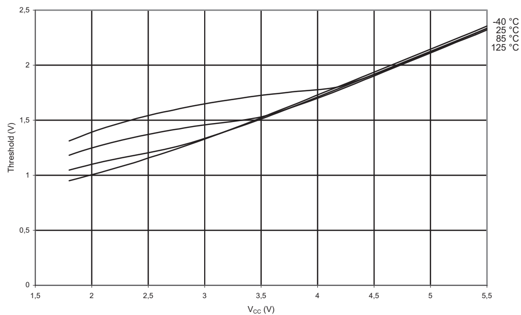
Figure 3-126. V_{IH} : Input Threshold Voltage vs. V_{CC} (Reset Pin, Read as '1')
