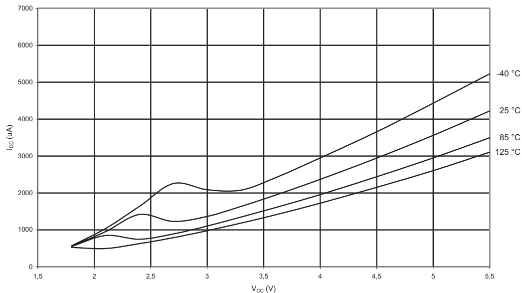
Figure 3-102. Brownout Detector Current vs. V_{CC} (BOD Level = 1.8V)
