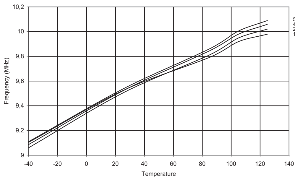
Figure 2-53. Calibrated 9.6 MHz Oscillator Frequency vs. Temperature CALIBRATED 9.6MHz OSCILLATOR FREQUENCY vs. TEMPERATURE
