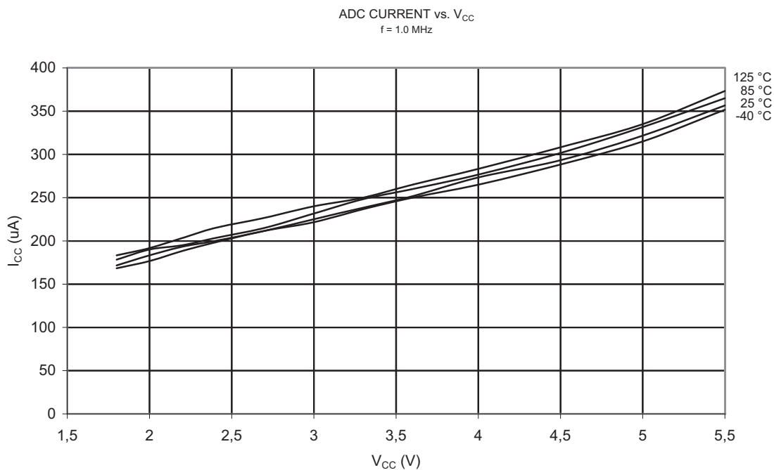
Figure 2-12. ADC Current vs. V_{CC}
