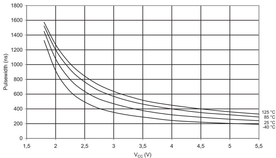
Figure 2-52. Minimum Reset Pulse Width vs. V_{CC} MINIMUM RESET PULSE WIDTH vs. V_{CC}
