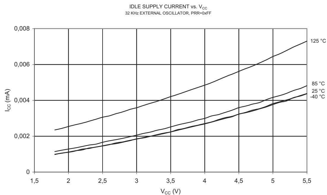
Figure 2-8. Idle Supply Current vs. V_{CC} (32 kHz External Clock)
