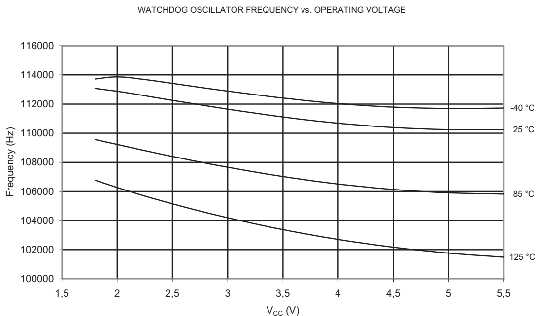
Figure 2-58. 128 kHz Watchdog Oscillator Frequency vs. V_{CC}
