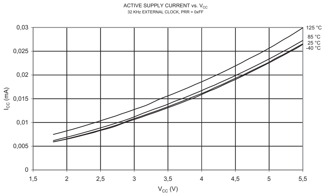
Figure 2-4. Active Supply Current vs. V_{CC} (32 kHz External Clock)
