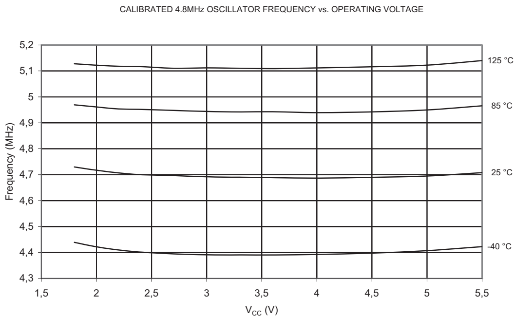
Figure 2-56. Calibrated 4.8 MHz Oscillator Frequency vs. V_{CC}
