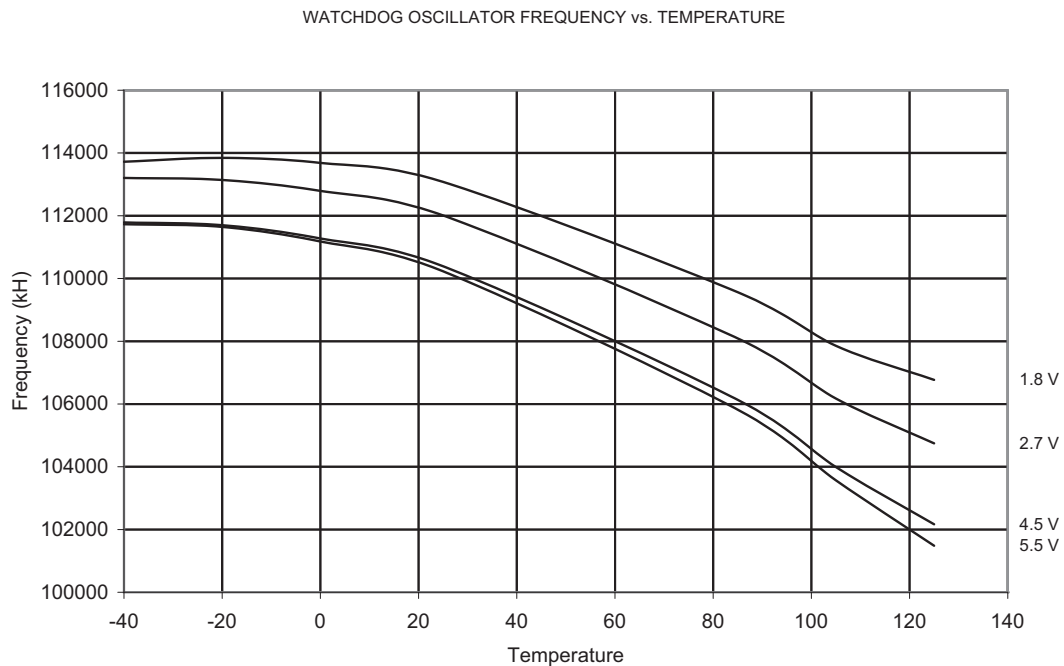
Figure 2-57. 128 kHz Watchdog Oscillator Frequency vs. Temperature
