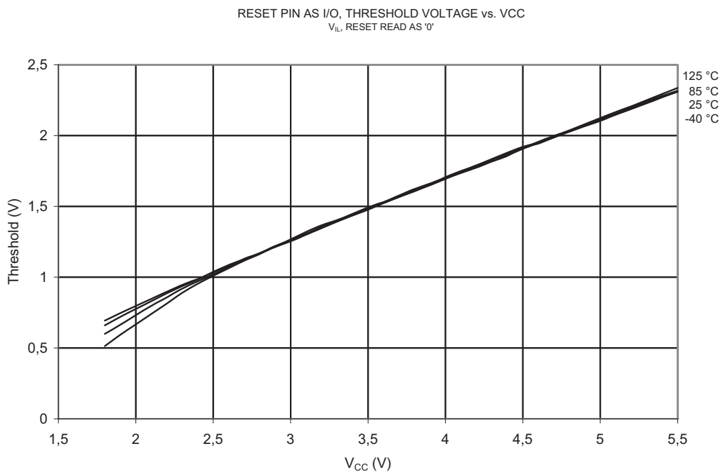
Figure 2-43. V_{IL} : Input Threshold Voltage vs. V_{CC} (Reset Pin as I/O, Read as '0')
