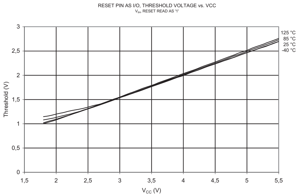
Figure 2-42. V_{IH} : Input Threshold Voltage vs. V_{CC} (Reset Pin as I/O, Read as '1')
