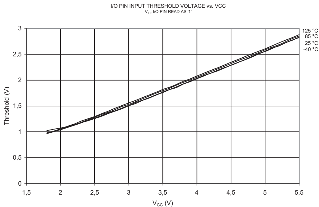
Figure 2-39. V_{IH} : Input Threshold Voltage vs. V_{CC} (I/O Pin, Read as '1')
