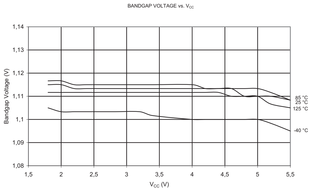
Figure 2-48. Bandgap Voltage vs. V_{CC}
