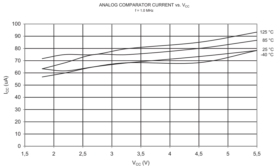
Figure 2-13. Analog Comparator Current vs. V_{CC}
