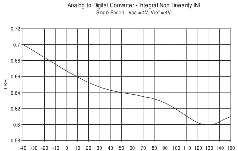
Figure 29. Analog to Digital Converter INL vs. Temperature, Single Ended
