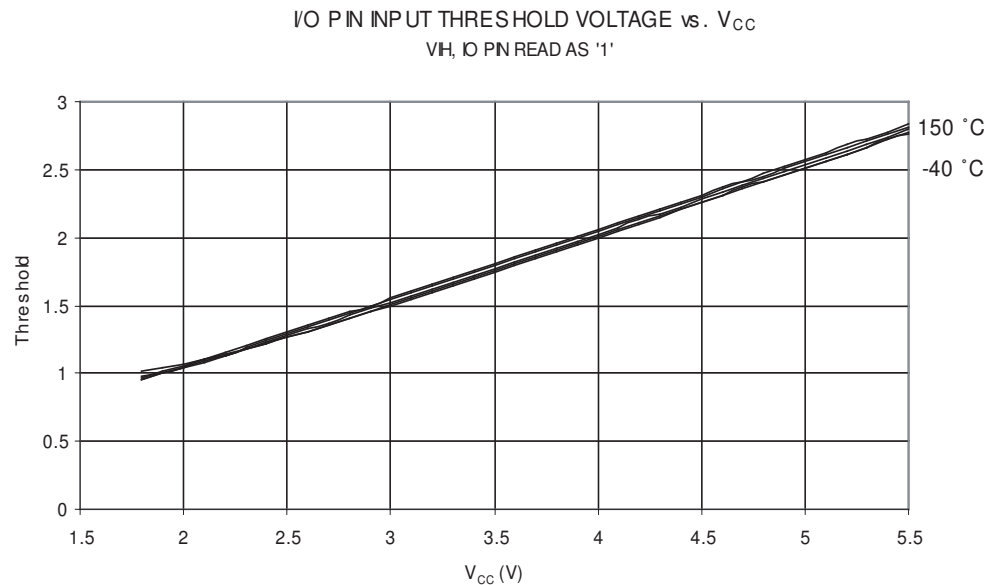
Figure 12. I/O Pin Input Threshold vs. V_{CC} ( V_{IH} , I/O Pin Read as '1')
