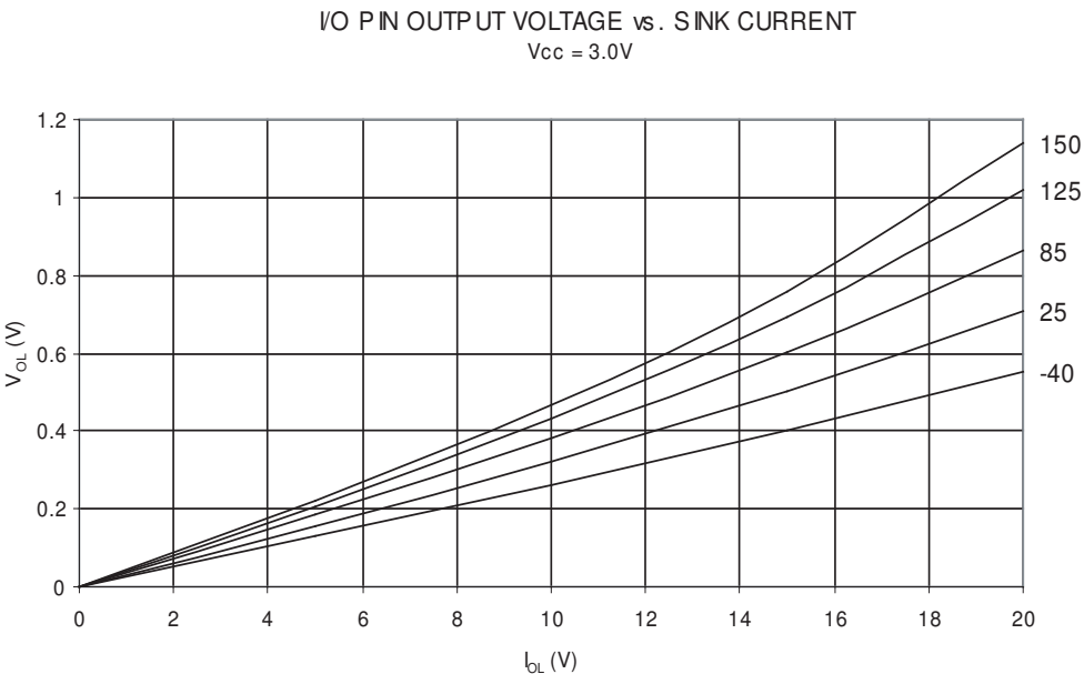
Figure 8. Output Low Voltage vs. Output Low Current ( V_{CC} = 3V )
