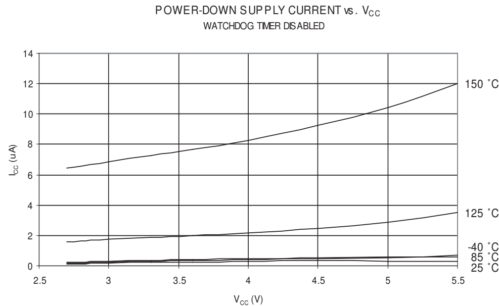
Power-Down Supply Current Figure 4. Power-Down Supply Current vs. V_{CC} (Watchdog Timer Disabled)
