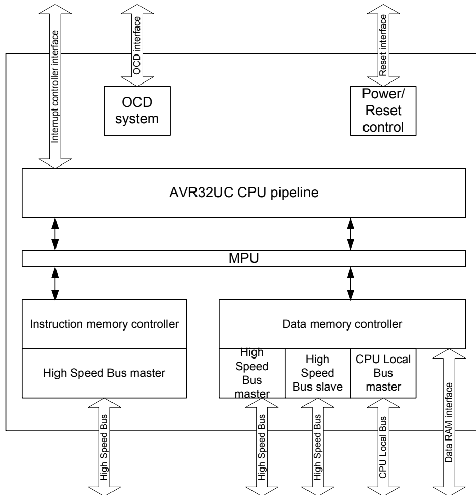
Figure 1-1. Overview of AVR32UC.
