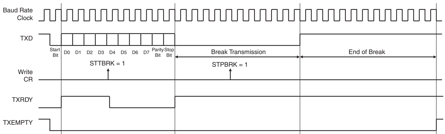
Figure 19-14. Break Transmission
