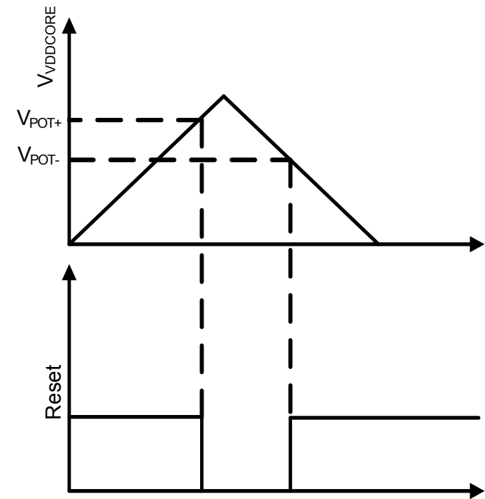
Figure 32-5. POR18 Operating Principles
