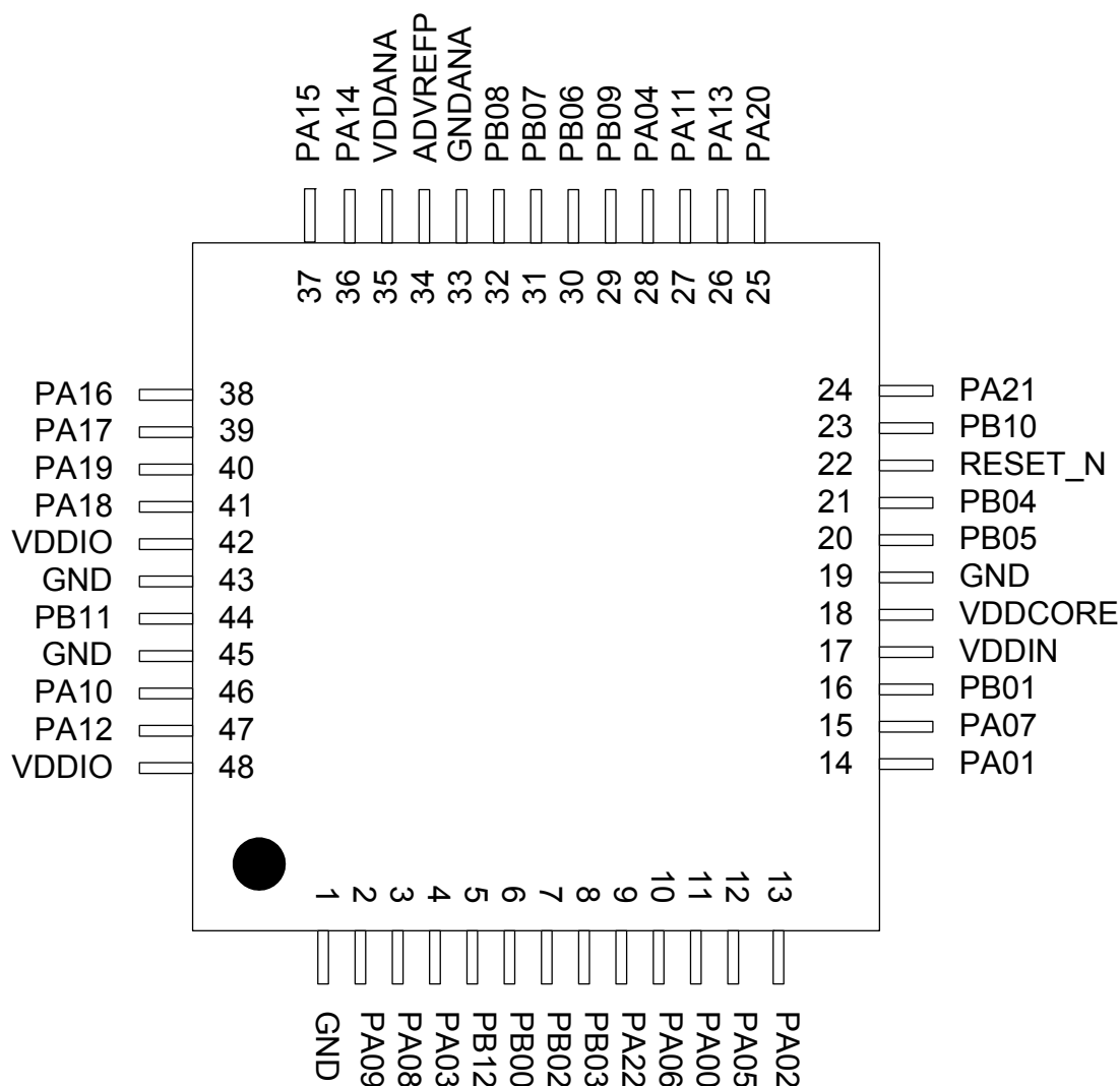
Figure 3-2. TLLGA48 Pinout
