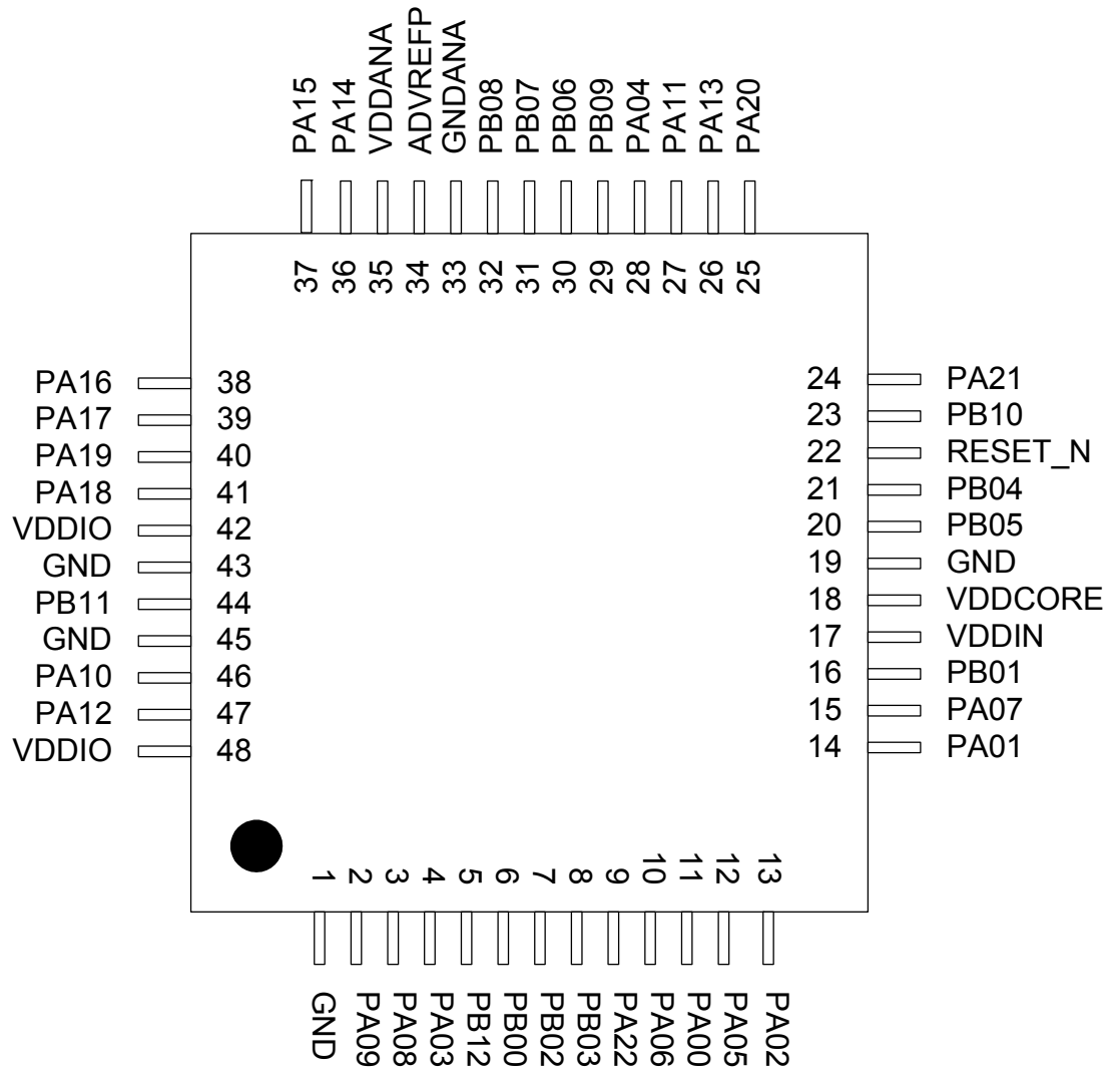
Figure 3-2. TLLGA48 Pinout
