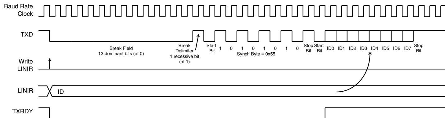
Figure 19-21. Header Transmission
