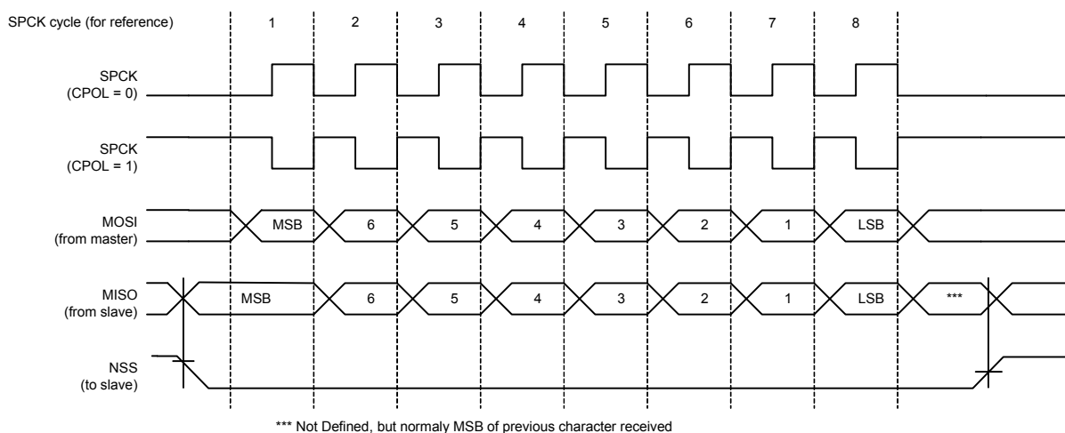
Figure 20-3. SPI Transfer Format (NCPHA = 1, 8 bits per transfer)
