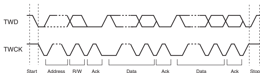
Figure 21-4. Transfer Format
