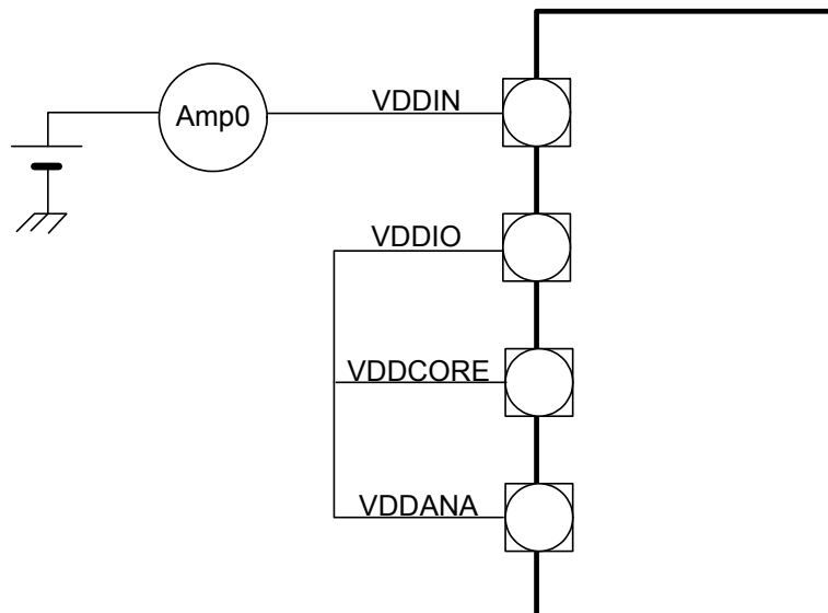
Figure 32-1. Measurement Schematic, Internal Core Supply
