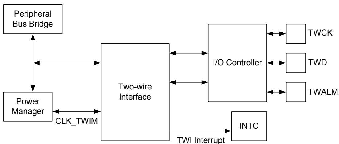
Figure 21-1. Block Diagram
