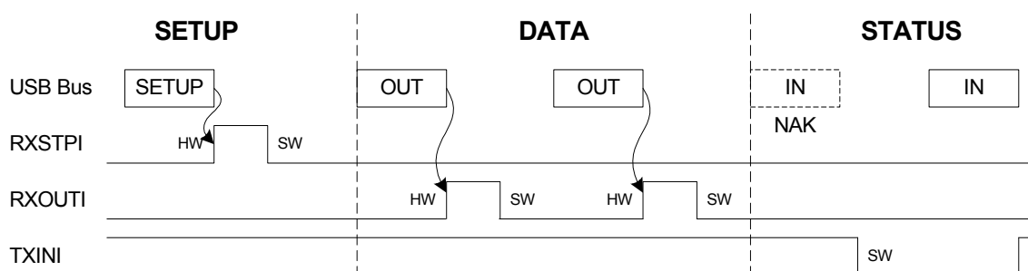
Figure 19-6. Control Write
