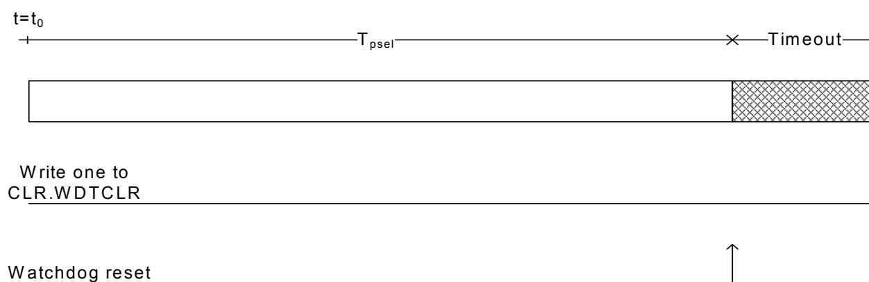
Figure 15-3. Basic Mode WDT Timing Diagram, no clear within T_{psel} .
