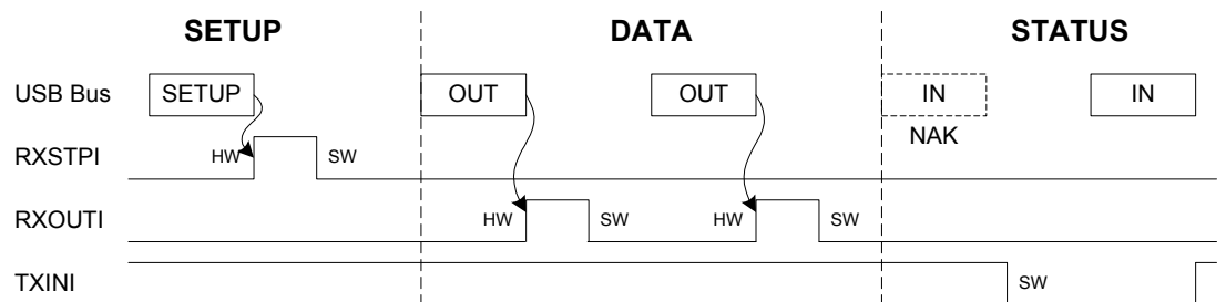
Figure 26-14. Control Write
