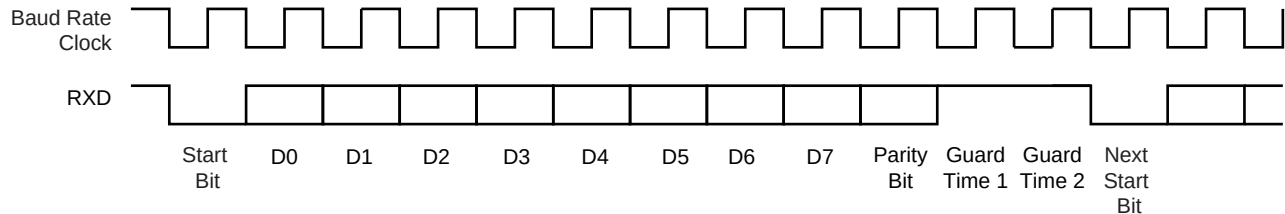
Figure 25-30. T=0 Protocol without Parity Error
