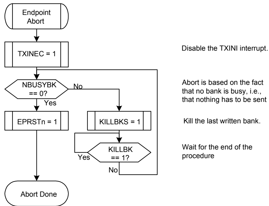
Figure 26-18. Abort Algorithm
