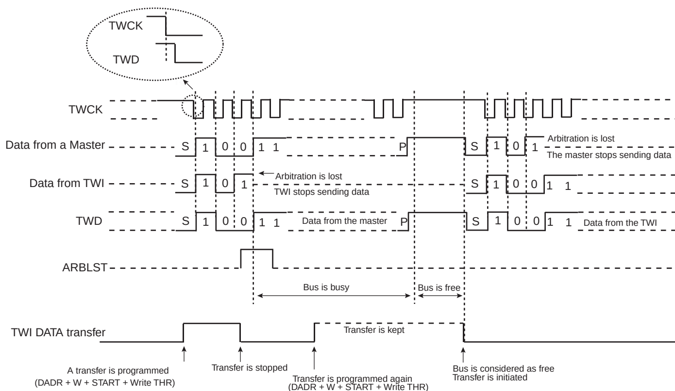
Figure 23-11. Arbitration Cases
