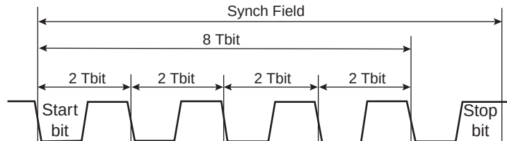
Figure 25-41. Sync Field
