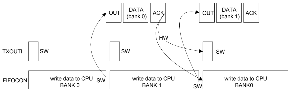
Figure 26-28. Example of an OUT Pipe with two Data Banks and a Bank Switching Delay
