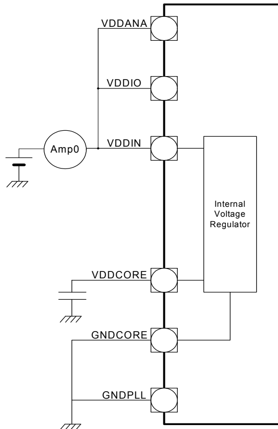
Figure 35-6. Measurement Setup
