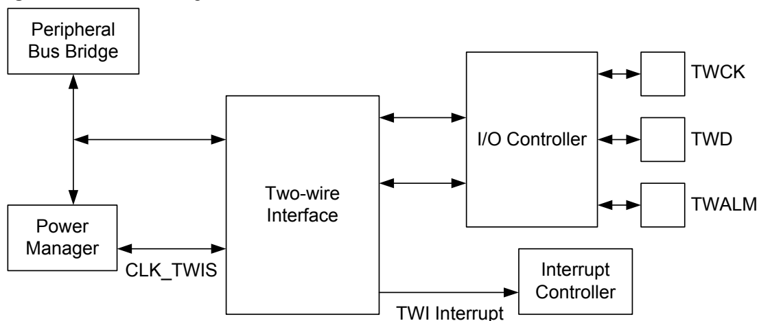
Figure 22-1. Block Diagram
