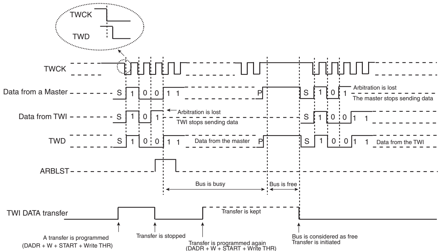
Figure 22-11. Arbitration Cases
