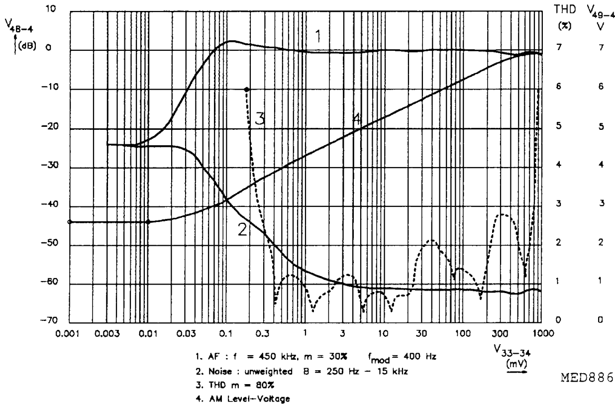
Fig.19 Signal, noise and distortion of AM AF output voltage and AM level voltage (typical curve).
