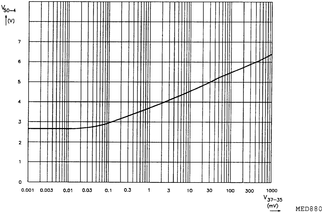
Fig.13 Level unweighted voltage (typical curve).
