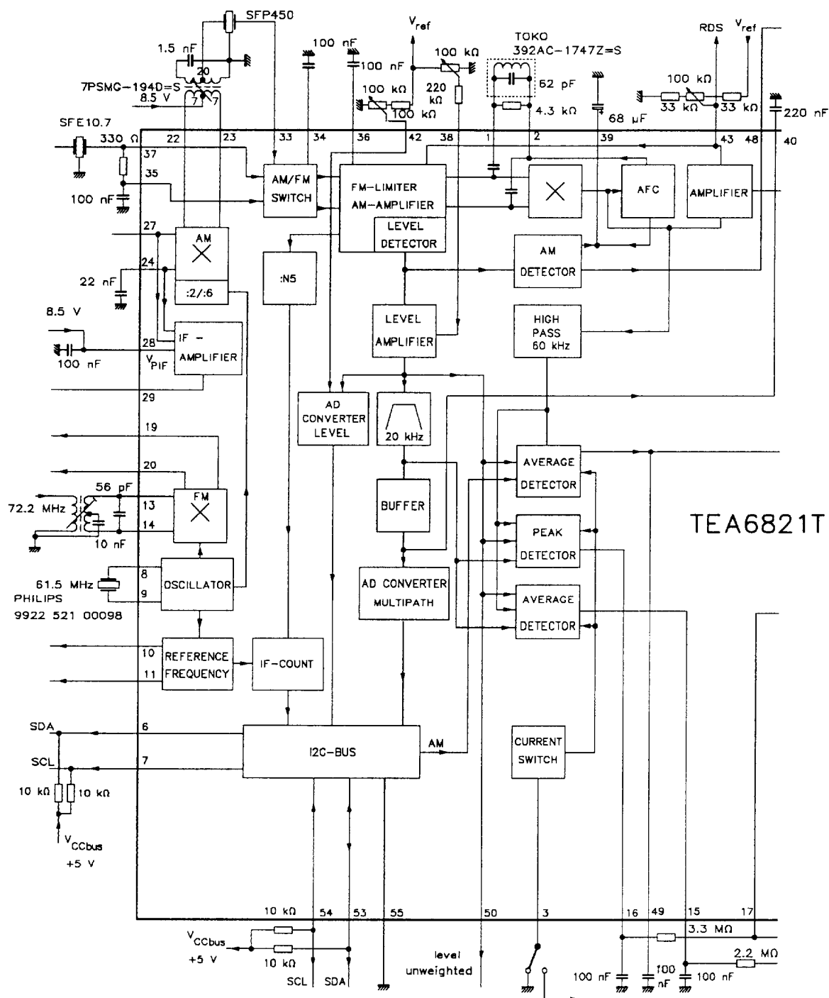
Fig.1 Block diagram (continued in Fig.2).
