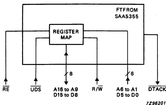
Fig.20 Microprocessor access to register map.
