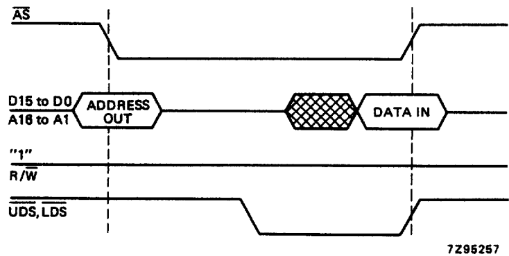
Fig.18 Bus timing for display memory access.
