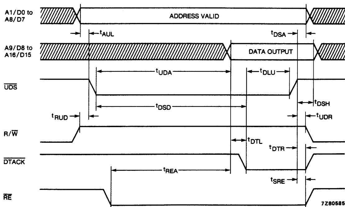
Fig.9 Timing of microprocessor read from FTFROM.
