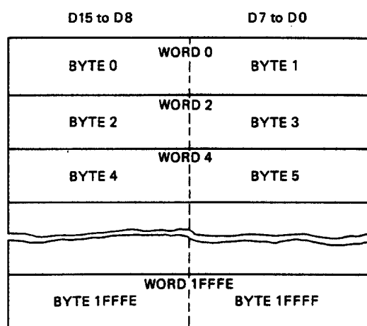
Fig.19 Display memory word/byte organization.
