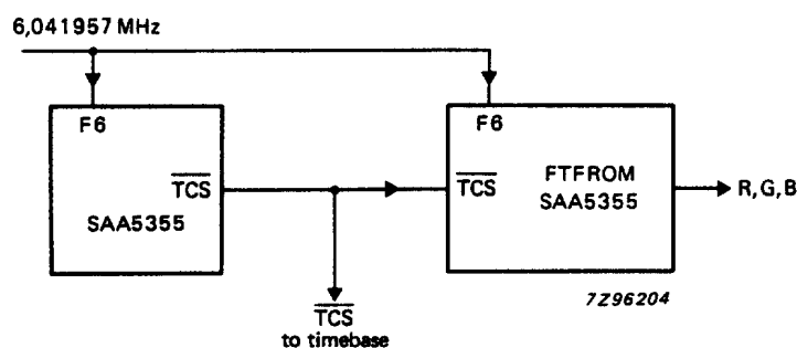
Fig.25 Simple-slave (direct sync) mode.
