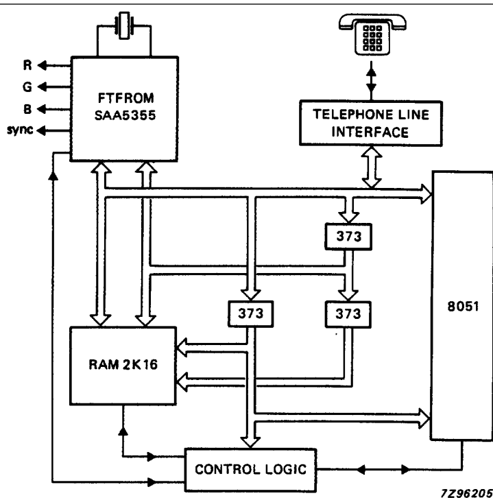
Fig.14 Basic videotex decoder configuration.
