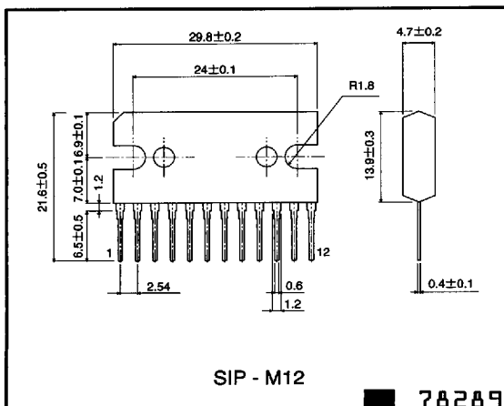
● External dimensions (Units: mm)
